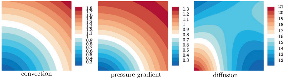
Figure 3.2: Magnitude of convection, pressure and diffusion terms [ \text{N m}^{-3} ] corresponding to the manufactured solution of Case 1.
