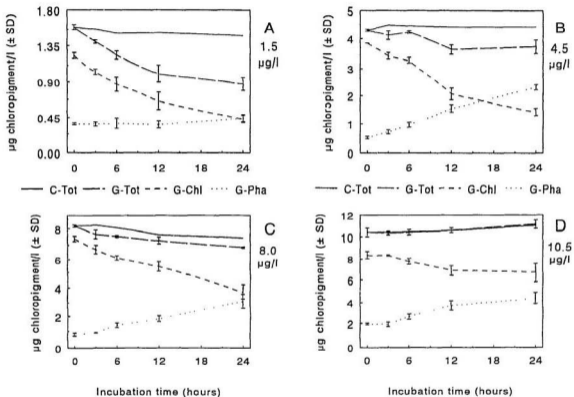
Figure 3.5. Chlorophyll levels in control (C) and grazing (G) bottles following incubation at 4 seston chlorophyll concentrations (A-D) for 3, 6, 12 and 24 hr. Tot-total, Chl-chlorophyll a and Pha-phaeopigments. Note: Y-scales differ.
