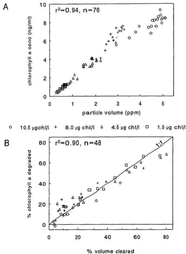
Figure 3.8. Relationships between (A) particle volume and chlorophyll a concentration in control and grazing bottles, and (B) % particle volume cleared and % chlorophyll a degraded in grazing bottles, with C. finmarchicus and 4 seston chloropigment concentrations.
