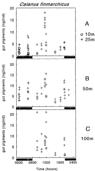
Figure 5.7. Diel chloropigment levels (ng/ind, chl a wt equiv.) in the digestive tracts of adult ♀ Calanus finmarchicus collected at various depths (A-C) during April 18-22, 1989. Each point represents an estimate determined from an extract of 5-20 copepods. See Appendix 5.1 for mean \pm SD values.
