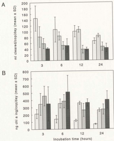
Figure 3.1. Particle clearance rates (A) and chlorophyll a ingestion rates (B) of adult ♀ Calanus finmarchicus , determined from particle spectra and chloropigment concentrations in bottle incubations at 4 initial seston chloropigment concentrations.
