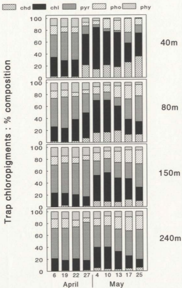
Figure 6.4. Chlorophyll composition of trap contents during April and May, 1988. X-axis: dates of initial trap deployment. Legend: chd (chlorophyllide a ), chl (chlorophyll a -types), pyr (pyropheophorbide a ), pho (other phaeophorbides) and phy (phaeophytin a -types).
