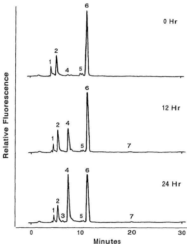
Figure 3.7. HPLC profiles of initial seston and representative bottle samples removed after 12 hr and 24 hr of incubation in C. finmarchicus grazing in Experiment 4. Peak identities are: 1-chlorophyllide a , 2-chlorophyll c , 3-phaeophorbide a , 4-pyropheophorbide a , 5-chlorophyll a allomers, 6-chlorophyll a , and 7-phaeophytin a . Note: Y-scales constant.
