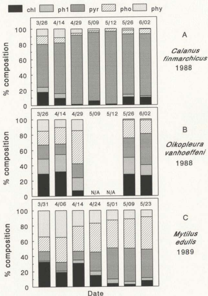
Figure 5.13. The seasonal chloropigment composition in A) Calanus finmarchicus digestive tracts, B) Oikopleura vanhoffeni faecal pellets, and in C) Mytilus edulis faeces. Legend: chl (chlorophyll a -types), ph1 (phaeophorbide a ), pyr (pyropheophorbide a ), pho (less polar phaeophorbide a -types) and phy (phaeophytin a -types). Data represent mean values.
