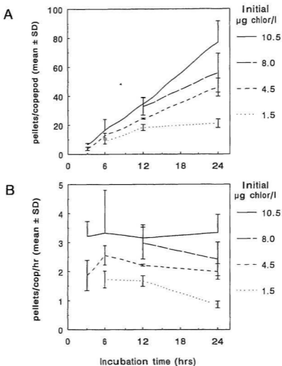
Figure 3.4. C. finmarchicus faecal pellet production (cumulative, A) and pellet production rate (B) following incubation at 4 seston chlorophyll concentrations for 3, 6, 12 and 24 hr.
