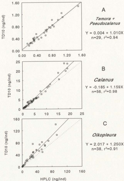
Figure 5.14. Relationships between standard fluorometric (TD10) and HPLC determinations of total chlorophyll concentration (chl a wt equiv.) in extracts of copepods (A,B) and oikopleurids (C) collected during the spring of 1988. Dotted lines represent a 1:1 relationship.
