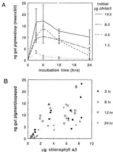
Figure 3.2. Adult ♀ C. finmarchicus gut chloropigments (ng/copepod) in grazing bottles following incubation at 4 initial seston chloropigment concentrations for 3, 6, 12 and 24 hr: A) gut pigments vs incubation time, and B) gut pigments vs chlorophyll a concentration remaining in each grazing bottle. Copepods prestarved overnight. Data represent extractions of approximately 10 animals from each of 3 grazing bottles.
