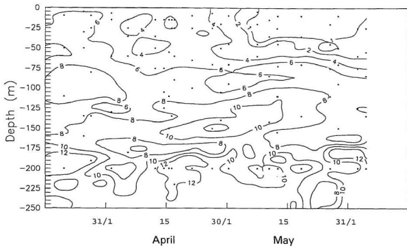
Figure 4.7. Time-depth plot of dissolved silicate concentration ( \mu\text{M/l} ) at the Conception Bay sampling site during mid-March to early June, 1988.
