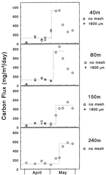
Figure 6.1. Mean carbon flux ( \text{mg}/\text{m}^2/\text{day} ) to 40, 80, 150 and 240 m during April and May 1988, as determined by replicate sediment traps ( N=4 ) at each depth. Step function fitted from the intercepts of the slopes of cumulative carbon flux in Figure 6.6.
