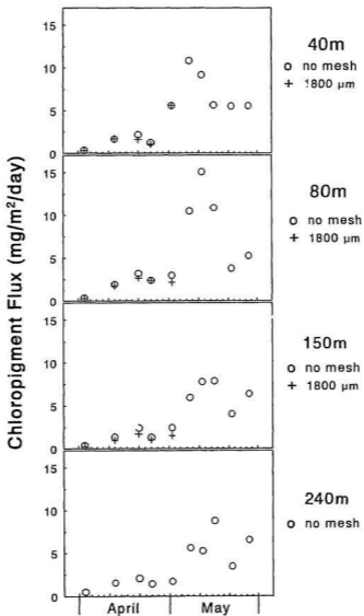
Figure 6.2. Mean chlorophyll flux (mg/m 2 /day, chl a wt. equiv.) to 40, 80, 150 and 240 m during April and May 1988, as determined by replicate sediment traps (N=4) at each depth.
