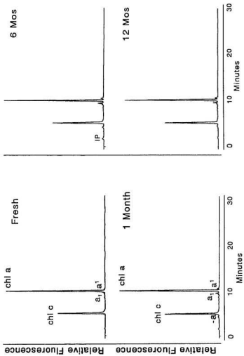
Figure 2-4. HPLC chlorophyll profiles of Thalassiosira weissflogii extracted fresh and following 1 month, 6 mos and 12 mos of storage at -20^{\circ}\text{C} . Peak identities: chl c (chlorophyll c), chl a (chlorophyll a), a 1 (chl a allomers), a 1 ' (C-10 epimer), -a (chlorophyllide a), IP (injection peak). Identical scaling of Y axes.
