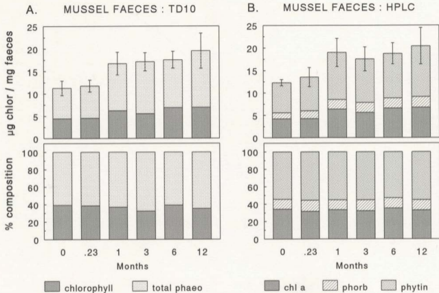
Figure 2.7. Chlorophyll concentration (chlor a wt. equiv. \pm SD of total) and percent composition in mussel faeces extracts using A) the TD10 fluorometer and B) HPLC. Legend as in Fig. 2.5.
