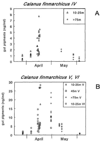
Figure 5.1. Total chloropigment concentrations (ng/ind, chl a wt equiv.) in the gut tracts of Calanus finmarchicus (Stages IV, V and VI) collected at various depths during March to June 1988. Each point represents an estimate of gut pigment per copepod determined fluorometrically (TD10) from an extract of 5-20 animals.
