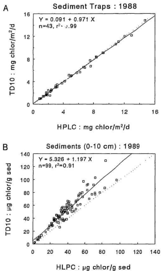
Figure 6.10. Relationships between standard fluorometric (TD10) and HPLC determinations of chloropigments in (A) sediment trap collections and (B) surface sediments. Dotted line represents a 1:1 relationship.
