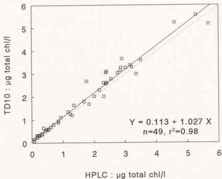
Figure 4.17. Relationship between standard fluorometric (TD10) and HPLC measurements of total chloropigments ( \mu\text{g/l} ) in seston <505\mu\text{m} collected during the spring 1988. Dotted line represents a 1:1 ratio.
