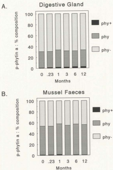
Figure 2.10. Percent composition of phaeophytin a -type pigments in A) mussel digestive gland and B) mussel faeces : phy (phaeophytin a plus isomer), phy+ (more polar types), phy- (less polar types).
