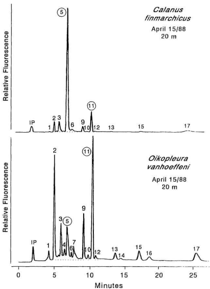
Figure 5.4. HPLC fluorescence profiles of chloropigments in the digestive tracts of Calanus finmarchicus and Oikopleura vanhoeffeni . Animals collected from the same net tow during full bloom conditions on April 15, 1988. Peak identities shown in Table 5.1.
