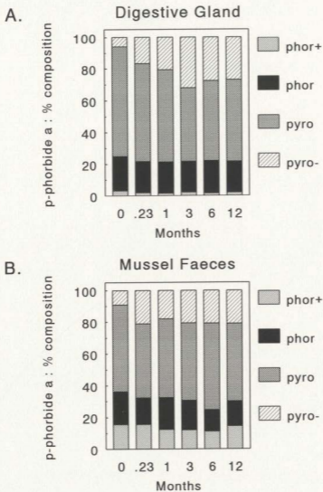
Figure 2.11. Percent composition of phaeophorbide a -type pigments in A) mussel digestive gland and B) mussel faeces : phor (phaeophorbide a ), phor+ (more polar types), pyro (pyropheophorbide a ), pyro- (less polar types than pyro).
