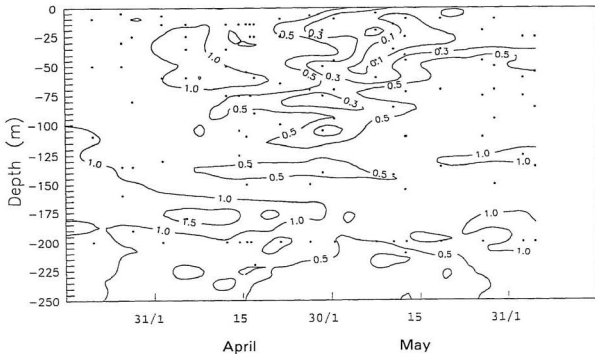
Figure 4.6. Time-depth plot of reactive phosphate concentration ( \mu\text{M:l} ) at the Conception Bay sampling site during mid-March to early June, 1988.
