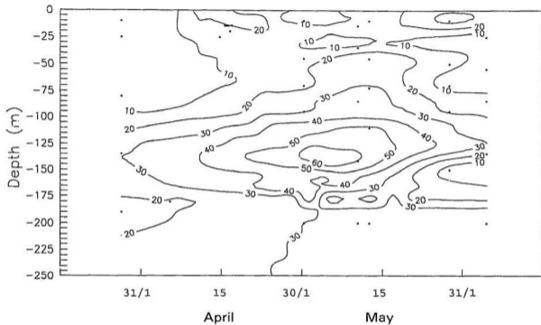
Figure 4.13. Time-depth plot of percent chlorophyll a in seston 15-70 \mu\text{m} at the Conception Bay sampling site during mid-March to early June, 1988. Measurements determined from extracts of filtered samples of fractionated seston.
