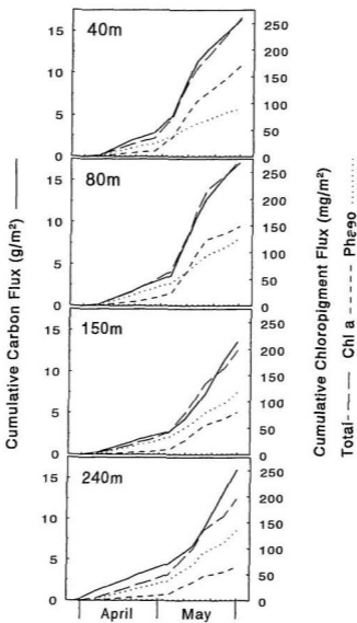
Figure 6.6. Cumulative flux of carbon ( \text{g}/\text{m}^2 ), total chlorophylls ( \text{mg}/\text{m}^2 ), chlorophyll a ( \text{mg}/\text{m}^2 ) and phaeopigments ( \text{mg}/\text{m}^2 ) to depths of 40, 80, 150 and 240 m during April and May 1988.
