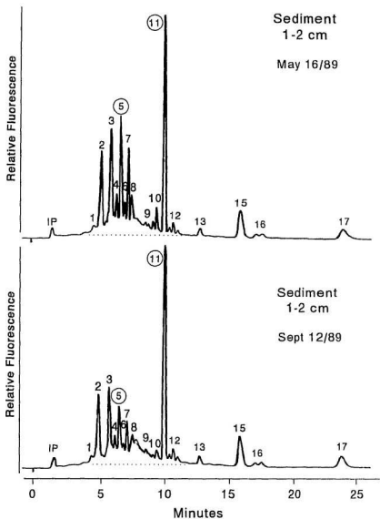
Figure 6.9. HPLC fluorescence profiles of chloropigments extracted from surface sediments (1-2 cm) during May and Sept., 1989. Peak identities are shown in Table 5.1.
