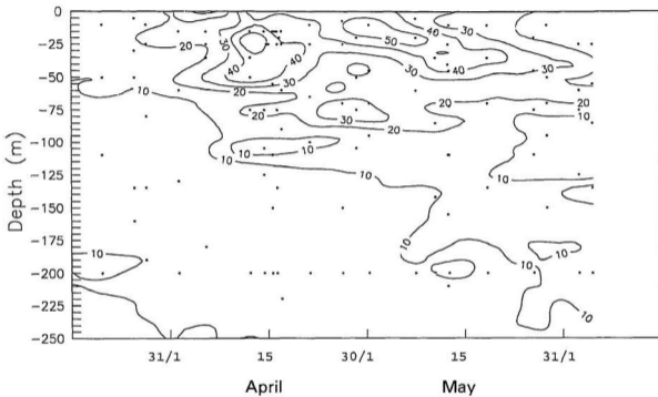
Figure 4.9. Time-depth plot of particulate organic nitrogen concentration ( \mu\text{g/l} ) in seston < 505 \mu\text{m} at the Conception Bay sampling site during mid-March to early June, 1988.
