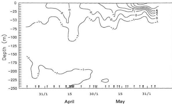
Figure 4.3. Time-depth plot of temperature ( ^{\circ}\text{C} ) at the Conception Bay sampling site during mid-March to early June, 1988. Measurements were determined using a Seabird SBE 20 CTD. Arrows indicate dates of CTD casts.
