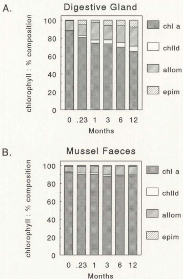
Figure 2.9. Percent composition of chlorophyll a -type pigments in A) mussel digestive gland and B) mussel faeces : chl a (chlorophyll a ), chlld (chlorophyllide a ), allom (allomers), epim (epimers).
