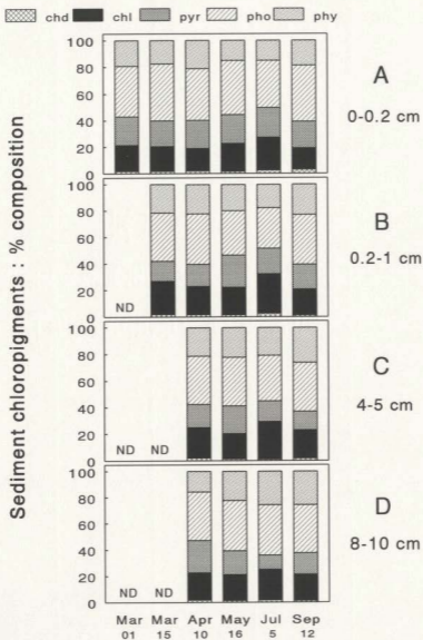
Figure 6.8. Chlorophyll composition of sediments collected at depths of 0-0.2 cm, 0.2-1 cm, 4-5 cm and 8-10 cm during March to September, 1989. Legend: chd (chlorophyllide a ), chl (chlorophyll a -types), pyr (pyropheophorbide a ), pho (other phaeophorbides) and phy (phaeophytin a -types).
