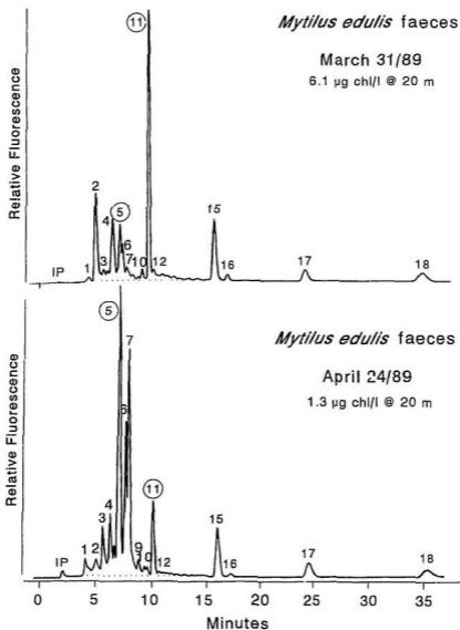
Figure 5.12. HPLC fluorescence profiles of chloropigments in the faeces of the blue mussel Mytilus edulis , suspended at a depth of 20 m during high and low seston chlorophyll concentrations in the spring of 1989. Peak identities are shown in Table 5.1.
