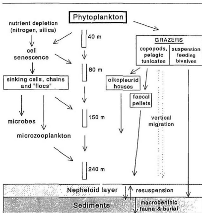
Figure 1.3. Schematic of some pathways of chlorophyll flux during the spring phytoplankton bloom in Conception Bay. Chlorophyll analyses were conducted on phytoplankton samples, grazer gut tracts and faecal material, sediment trap collections at various depths, surface sediments and overlying flocculent material.
