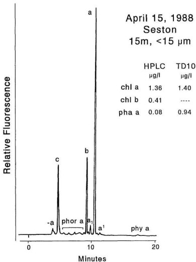
Figure 4.16. HPLC fluorescence profile of pigments extracted from seston <15 \mu m collected from a depth of 15 m on April 15, 1988. Peak identities are: -a (chlorophyllide a), c (chlorophyll c), b (chlorophyll b), a (chlorophyll a), a 1 (allomers of a), a' (epimers of a), phor a (phaeophorbide a-types), phy a (phaeophytin a). Note the TD10 overestimation of phaeopigments (pha) in the presence of high levels of chlorophyll b.
