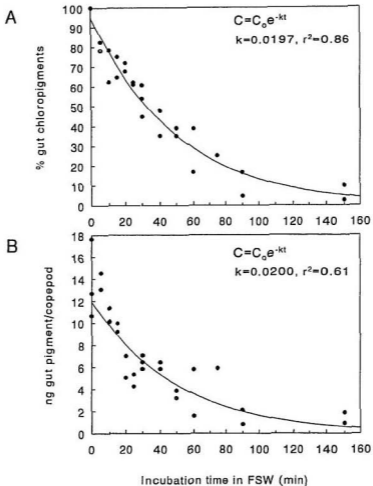
Figure 3.3. Gut clearance rates of chloropigments following transfer of adult ♀ C. finmarchicus to FSW. Rates determined using A) % gut chloropigments and B) gut chloropigment content at each interval. Incubations conducted at 0-1°C. Each point represents data collected from 5-10 copepods. All data fitted to an exponential curve: C = C_0 e^{-kt} , where C = gut pigment level, k = defecation rate constant, and t = time (min).
