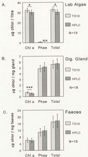
Figure 2.13. Comparative TD10 and HPLC estimates (mean \pm SD) of chlorophyll a -type pigments, phaeopigments and total chloropigments in extracts of A) laboratory algae, B) mussel digestive gland and C) mussel faeces. ANOVA: *( p < 0.05 ), ***( p < 0.001 ).
