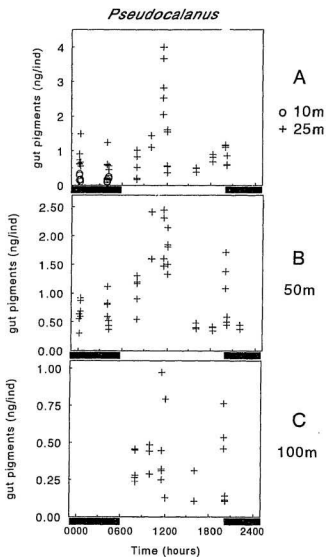
Figure 5.10. Diel chloropigment levels (ng/ind, chl a wt equiv.) in the digestive tracts of adult Pseudocalanus minutus collected at various depths (A-C) during April 18-22, 1989. Each point represents an estimate determined from an extract of 20-50 copepods. Note: Y-scale differs with depth. See Appendix 5.1 for mean \pm SD values.
