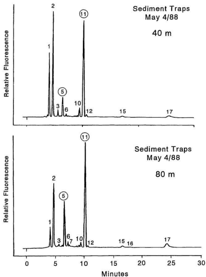
Figure 6.3. HPLC fluorescence profiles of chloropigments extracted from material collected in sediment traps at 40 m, 80 m, 150 m and 240 m. Traps retrieved on May 4, 1988 following a 7 day deployment period. Peak identities are shown in Table 5.1.
