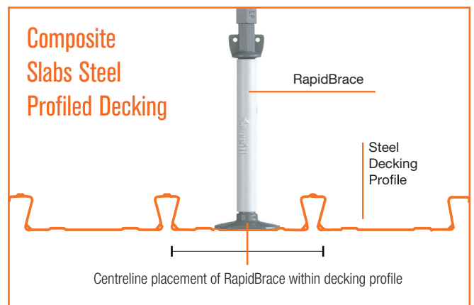
Figure 3: Centreline placement of RapidBrace within trough of steel decking profile, equidistant from each rib.
