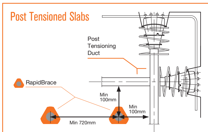
Figure 2: RapidBrace clearances to post tensioning ducts.
