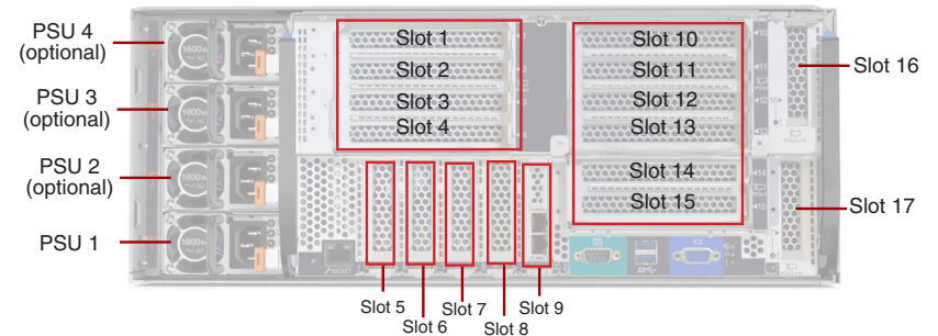
Note: All riser cards, expansion cards, and LOM adapters are optional.
