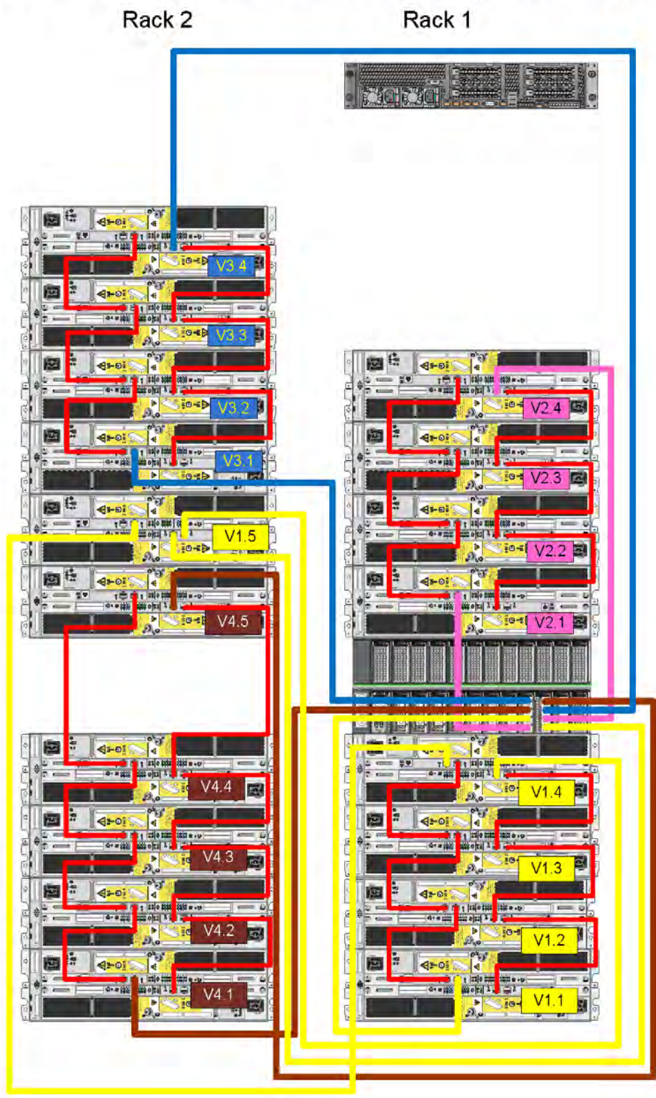
Figure 96. Recommended cabling for DD7200 integrated with Avamar
