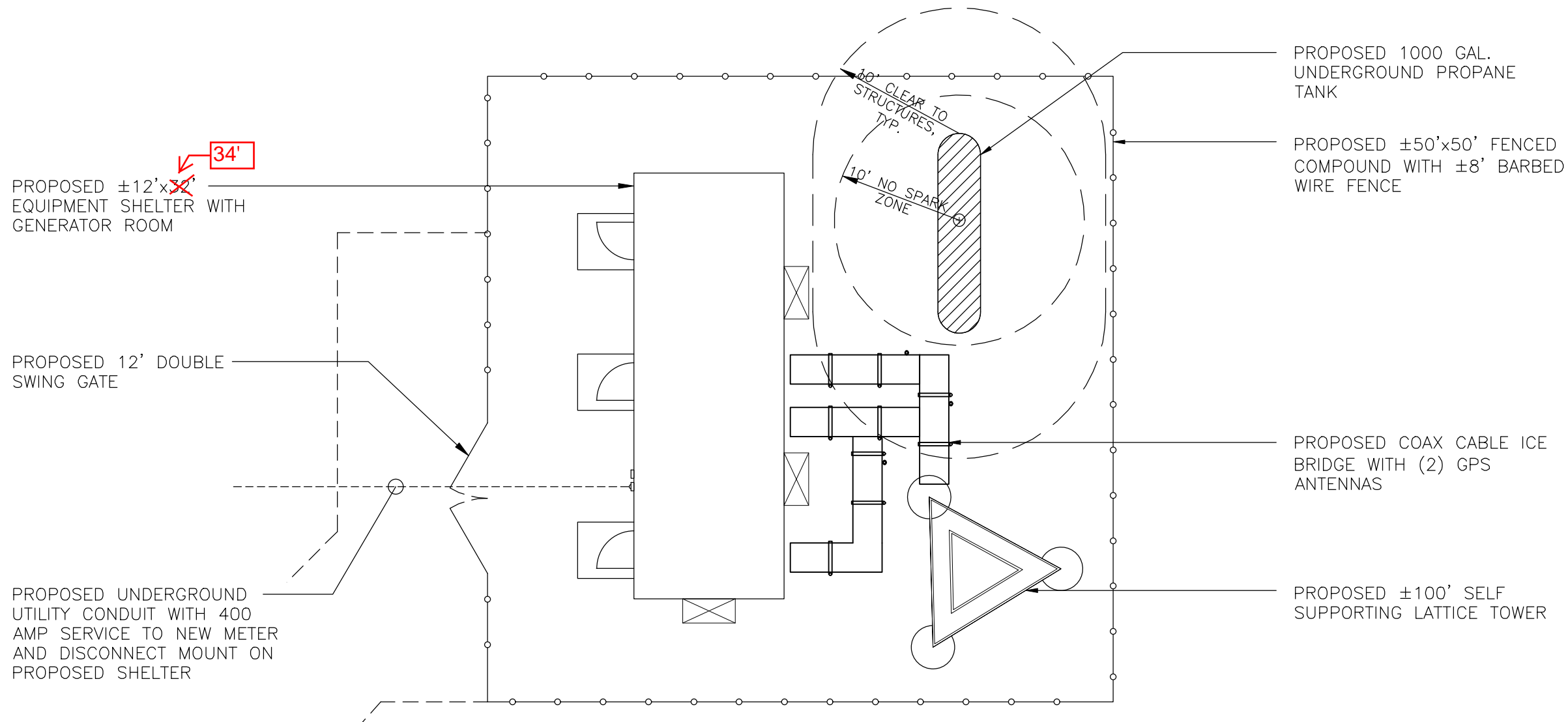
1 L-3 COMPOUND PLAN SCALE: 1" = 10'-0"
