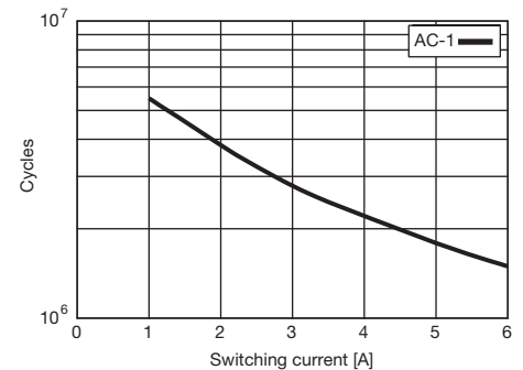
Fig.1 AC voltage endurance
