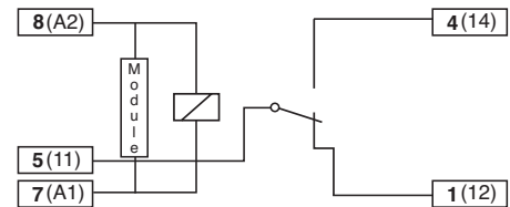
S7-16 for relays C7-A10 (16 A)
