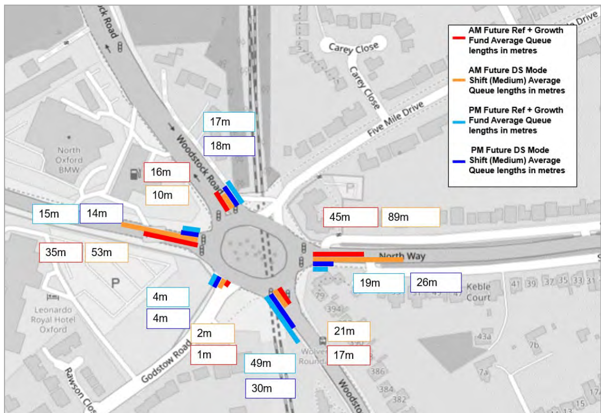
Figure 4.6: Wolvercote Average Queue lengths (0800-0900 and 1700-1800)
