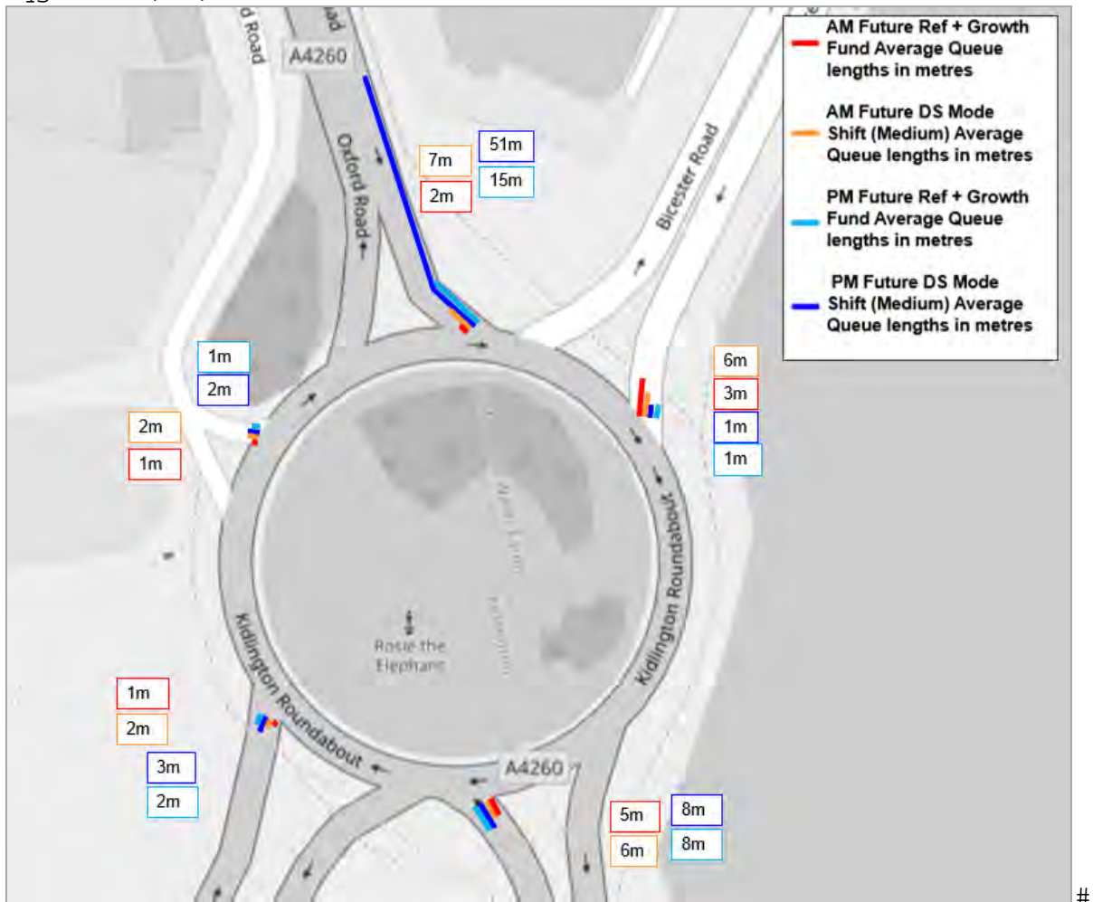
Figure 4.3: Oxford Road/Bicester Road Roundabout Average Queue lengths +3 ; 33 03 < 33 # dgg# : 33 04 ; 33 ,
