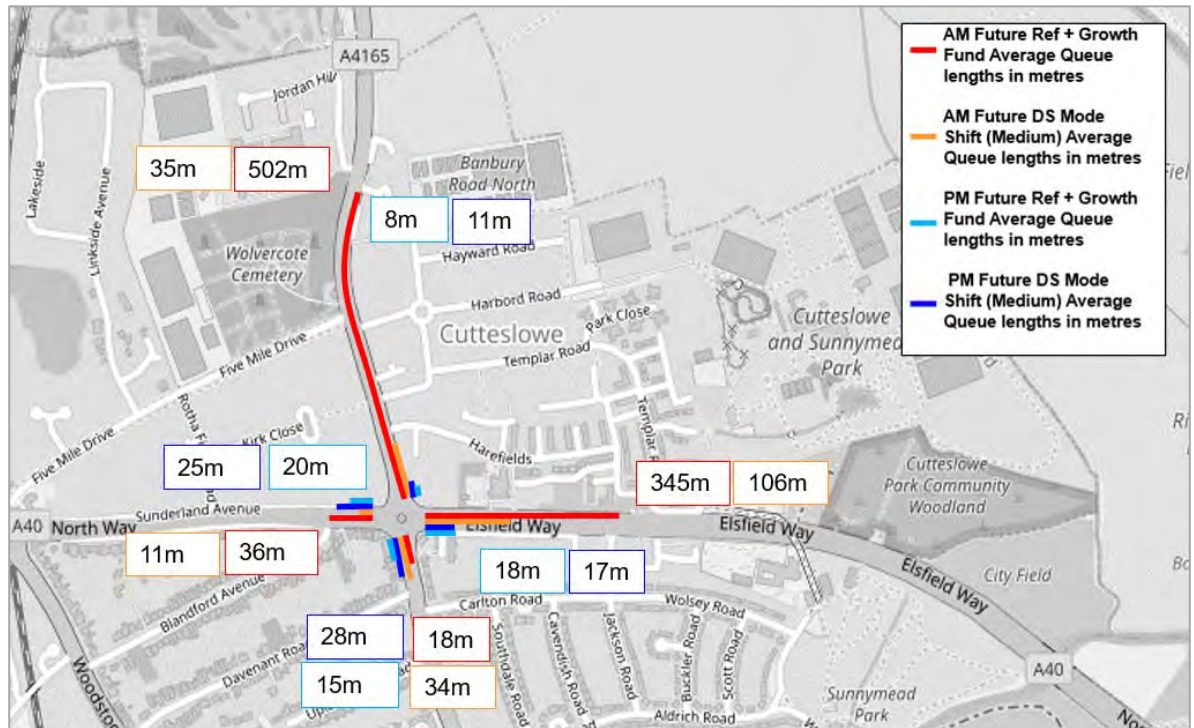
Figure 4.7: Cutteslowe Roundabout Average Queue lengths (0800-0900 and 1700-1800)#
