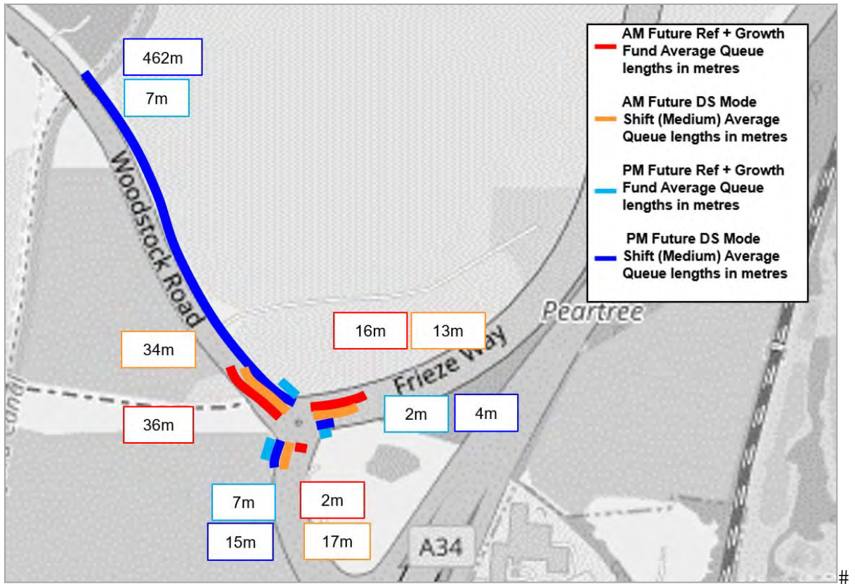
Figure 4.3: Loop Farm Roundabout Average Queue lengths (0800-0900 and 1700-1800)
