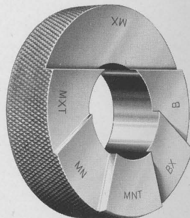
6 Step Major Diameter Ring Gage
