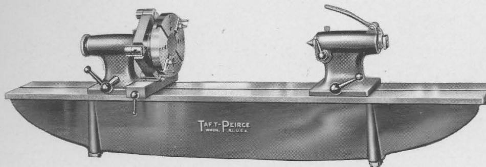
STYLE 9205-SB
