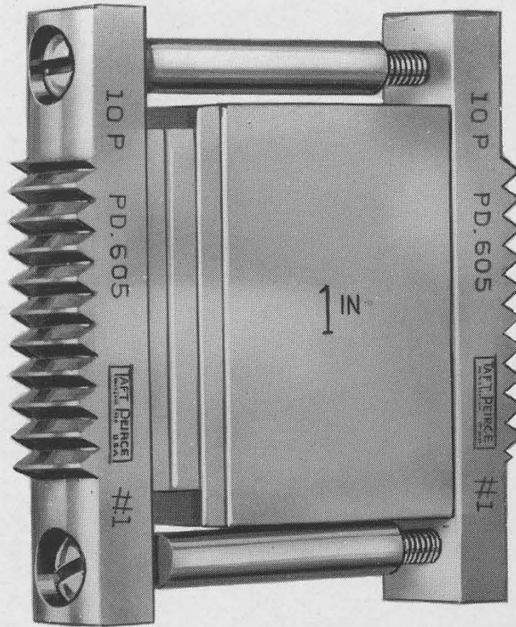
TAFT-PEIRCE STYLE 9431
