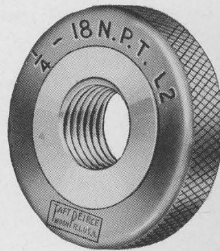
L2 Taper Thread Ring Gage
