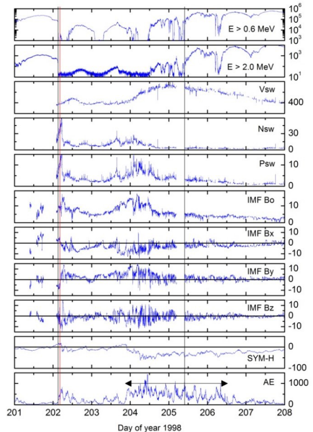
Figure 12. A relativistic electron decrease (RED) event and later acceleration. Taken from Tsurutani et al. (2016b).
