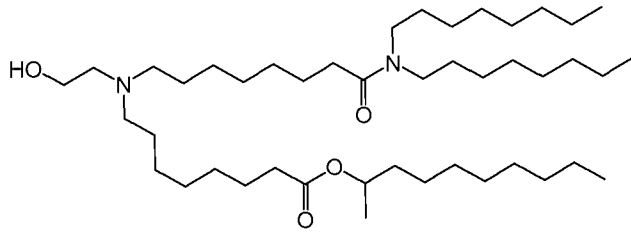
(Compound 130),
