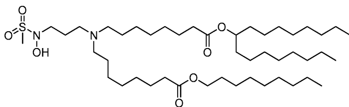
(Compound 206),
