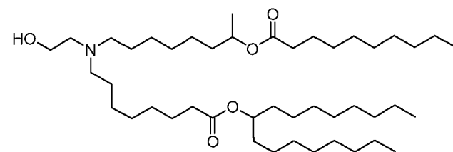
(Compound 98),
