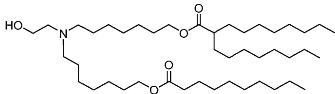
(Compound 150),
