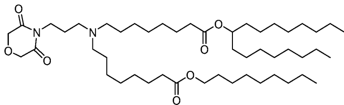
(Compound 202),
