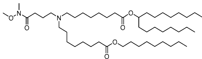
(Compound 228),
