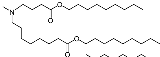
(Compound 126),
