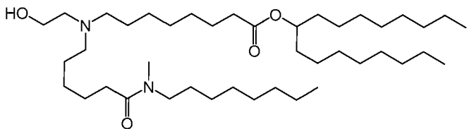
(Compound 146),
