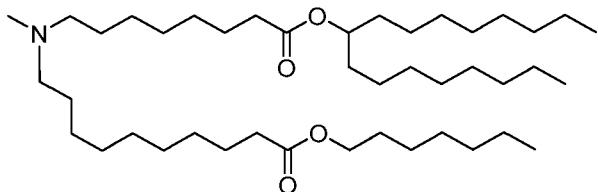
(Compound 149),
