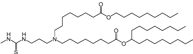
(Compound 113),
