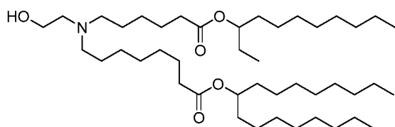
(Compound 75),
