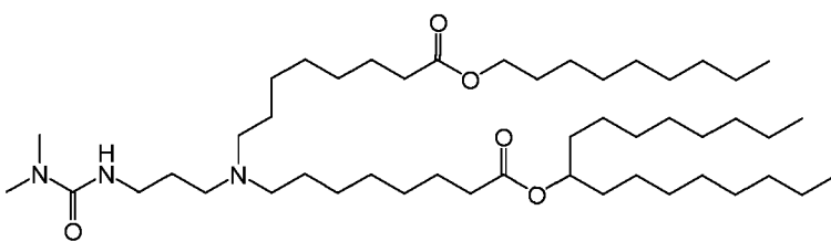
(Compound 110),
