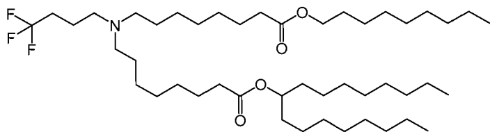
(Compound 107),
