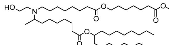
(Compound 192),
