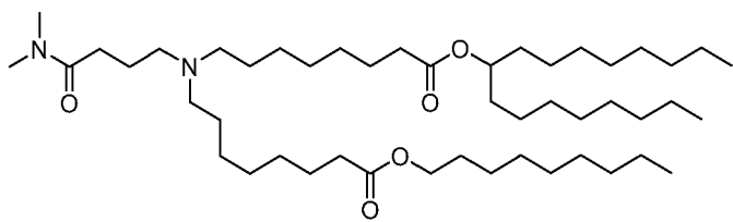
(Compound 224),
