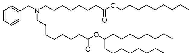
(Compound 94),
