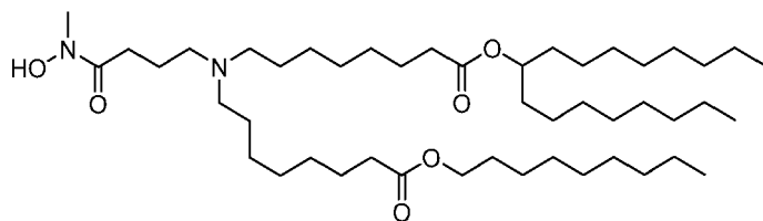
(Compound 227),
