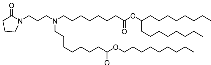
(Compound 195),
