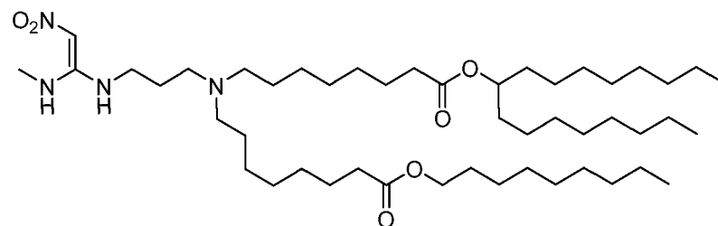
(Compound 170),
