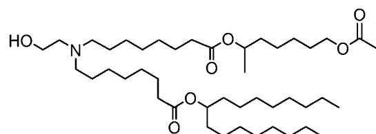
(Compound 214),
