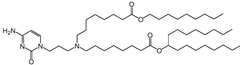
(Compound 115),
