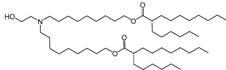
(Compound 133).
