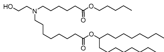
(Compound 104),
