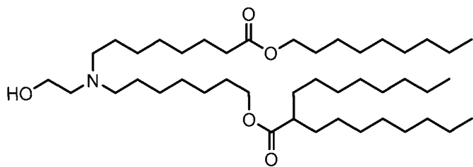
(Compound 30),
