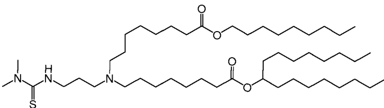
(Compound 111),
