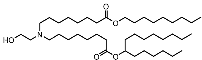
(Compound 32),
