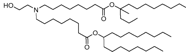
(Compound 87),
