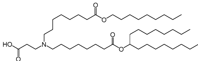
(Compound 124),
