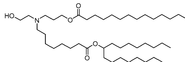
(Compound 97),
