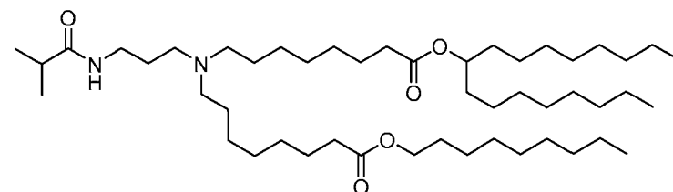
(Compound 194),
