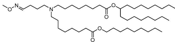
(Compound 229),
