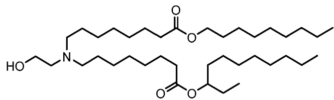
(Compound 35),
