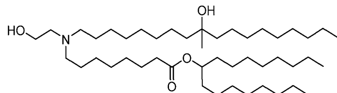
(Compound 171),
