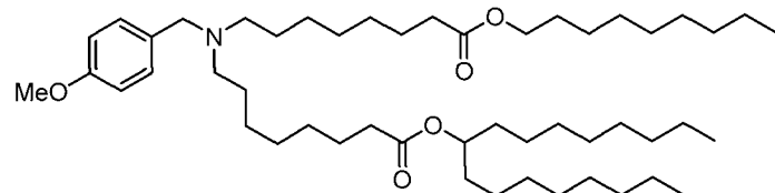
(Compound 94),
