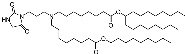
(Compound 174),
