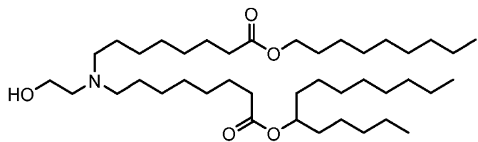
(Compound 33),
