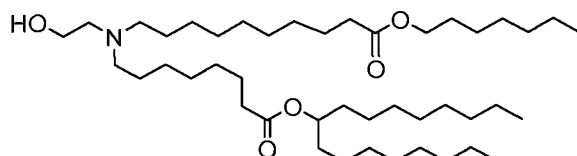
(Compound 189),
