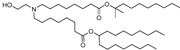
(Compound 85),
