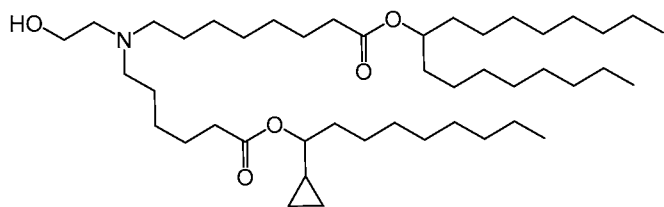
(Compound 128),
