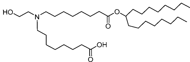
(Compound 166),
