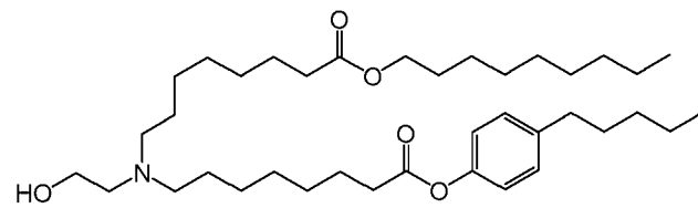
(Compound 119),
