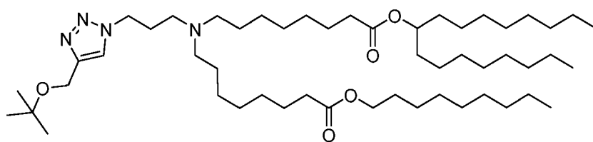
(Compound 176),
