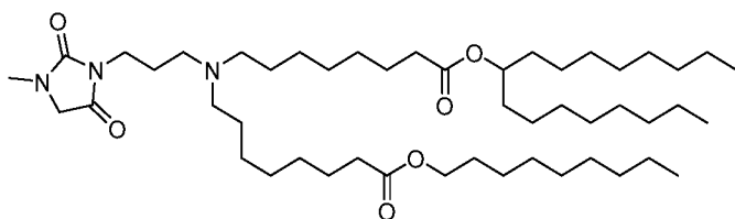
(Compound 201),
