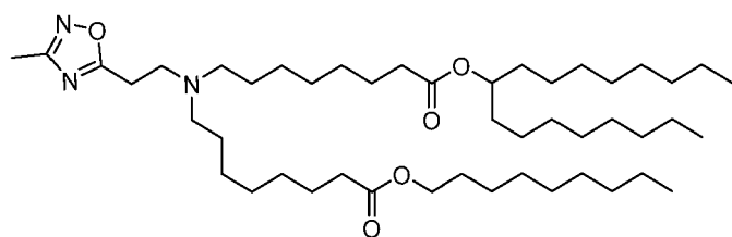
(Compound 230),
