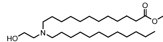
(Compound 137),
