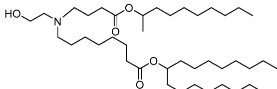
(Compound 70),
