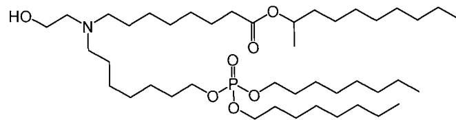
(Compound 132),
