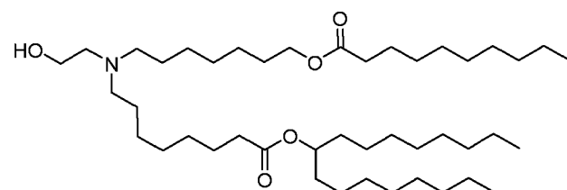
(Compound 96),
