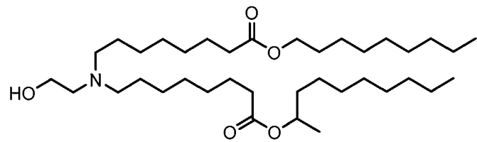
(Compound 36),
