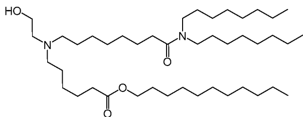
(Compound 129),
