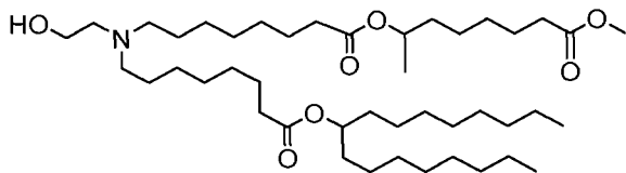
(Compound 187),
