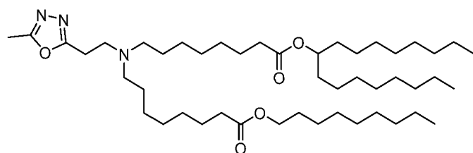
(Compound 231),
