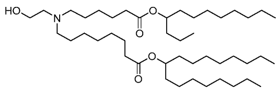
(Compound 76),
