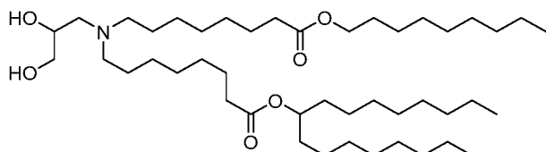
(Compound 69),
