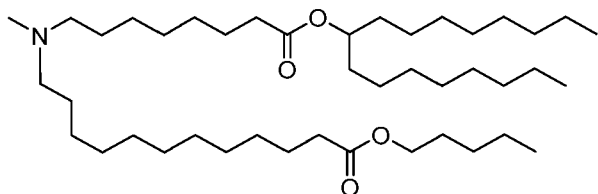
(Compound 150),
