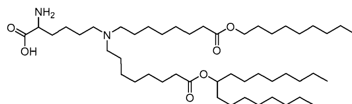
(Compound 105),
