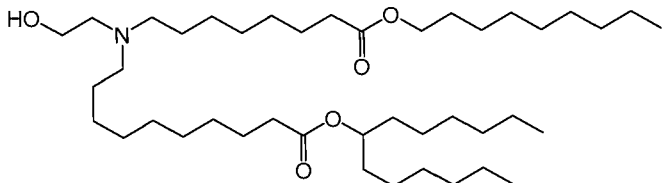
(Compound 147),
