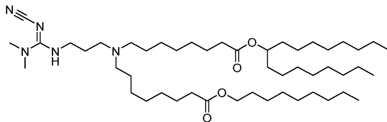
(Compound 167),
