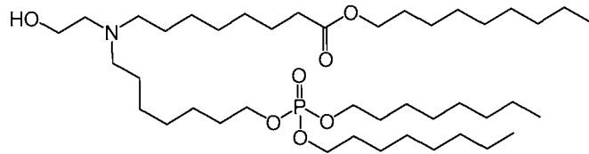
(Compound 131),
