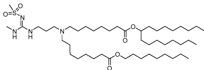
(Compound 212),
