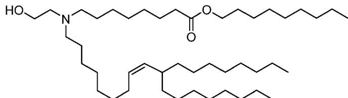
(Compound 152),
