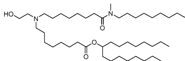
(Compound 105),
