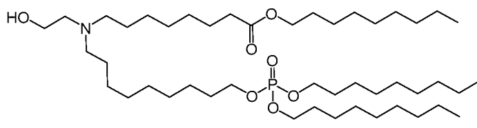
(Compound 126),
