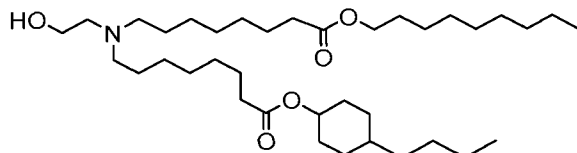
(Compound 188),
