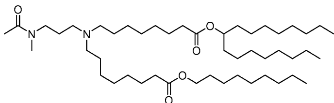
(Compound 196),
