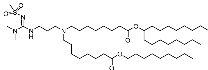
(Compound 213),
