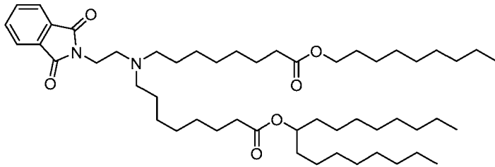
(Compound 100),
