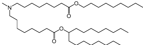
(Compound 123),
