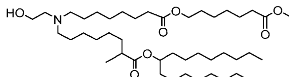
(Compound 190),
