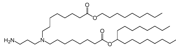
(Compound 121).
