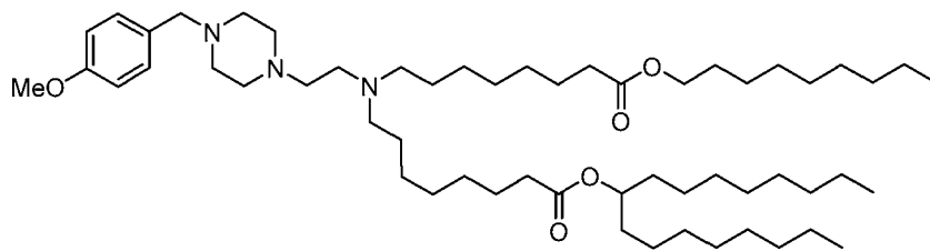
(Compound 101),
