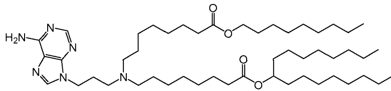
(Compound 116),
