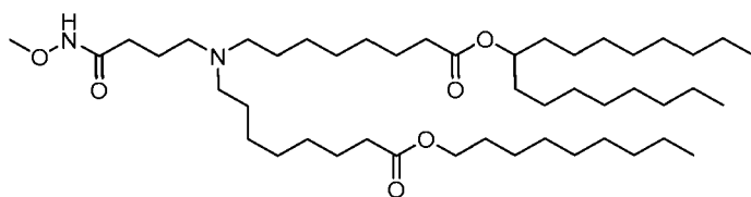
(Compound 226),
