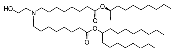
(Compound 172),
