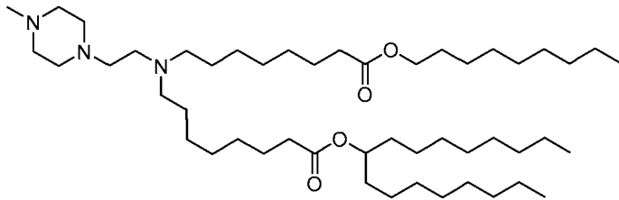
(Compound 101),
