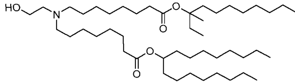
(Compound 86),
