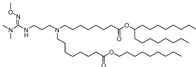
(Compound 211),
