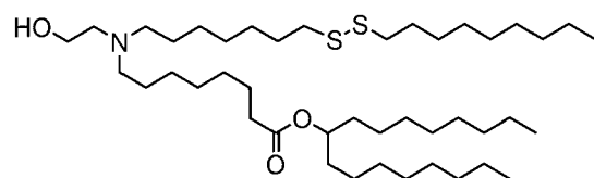
(Compound 215),
