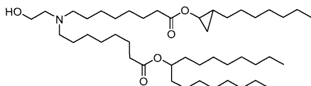
(Compound 93),
