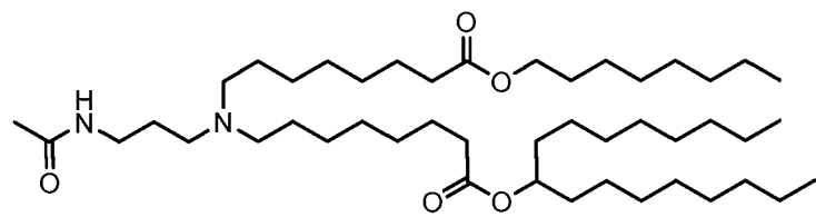
(Compound 36),
