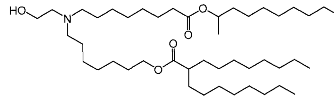
(Compound 135),
