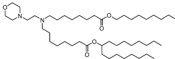
(Compound 103),
