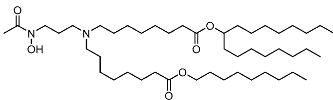
(Compound 204),
