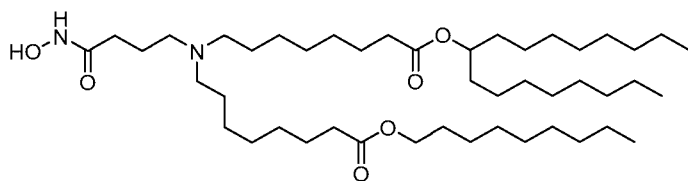
(Compound 225),
