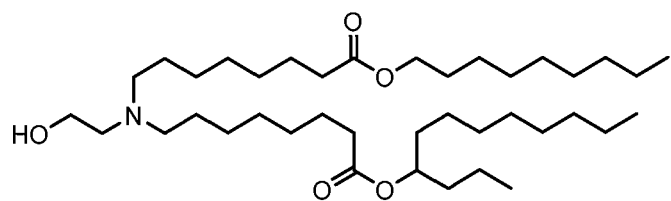
(Compound 34),
