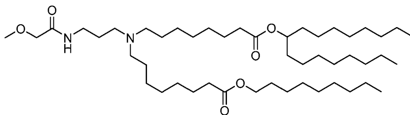
(Compound 178),
