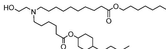
(Compound 191),
