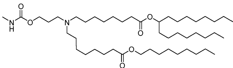
(Compound 175),
