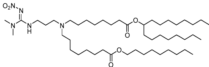
(Compound 209),
