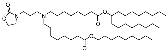
(Compound 199),
