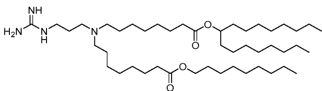
(Compound 207),
