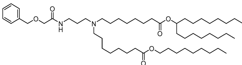
(Compound 196),
