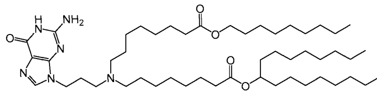
(Compound 117),
