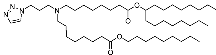
(Compound 179),
