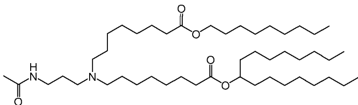
(Compound 108),
