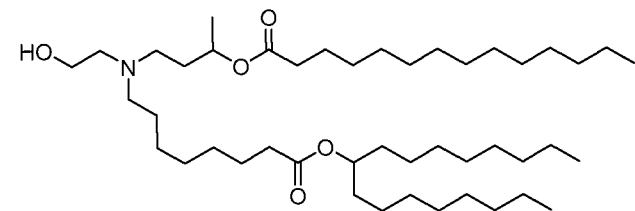
(Compound 99),
