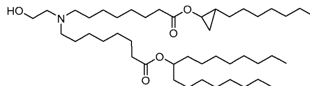
(Compound 88),
