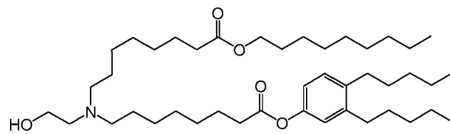
(Compound 118),
