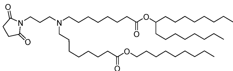
(Compound 176),
