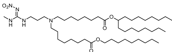
(Compound 200),
