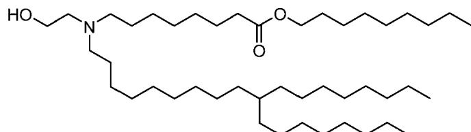
(Compound 153),
