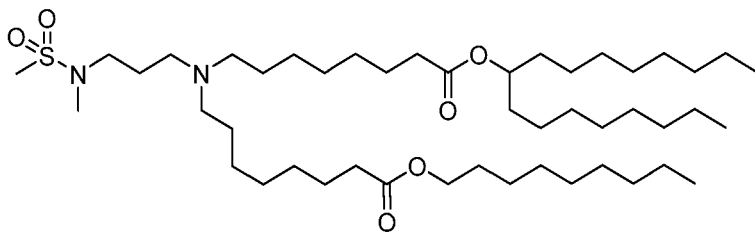
(Compound 173),
