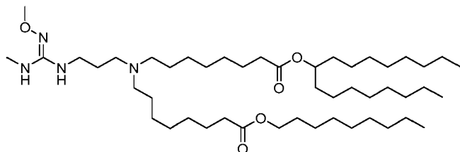
(Compound 210),
