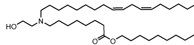
(Compound 136),
