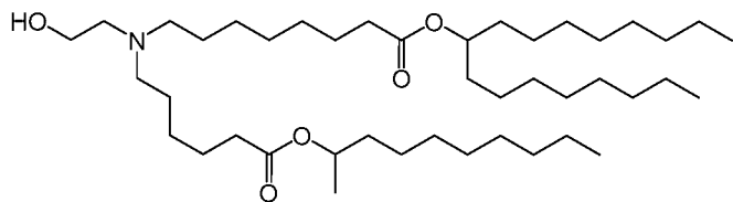
(Compound 122),
