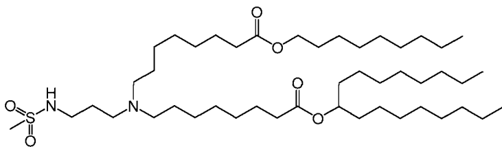
(Compound 109),
