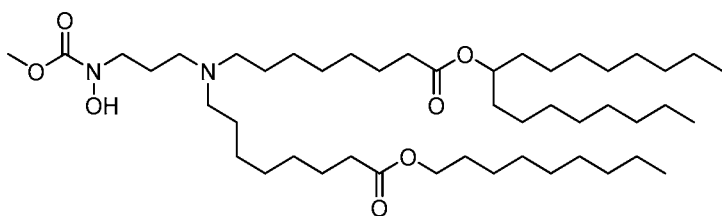
(Compound 205),
