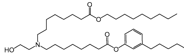
(Compound 120),
