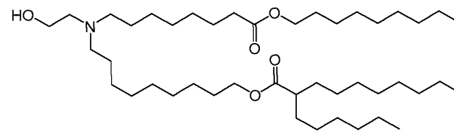
(Compound 134),
