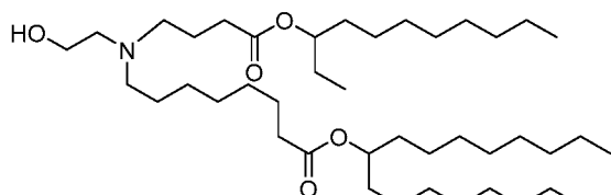
(Compound 72),
