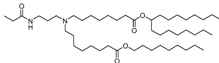
(Compound 192),
