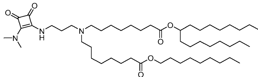
(Compound 169),
