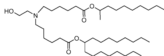
(Compound 89),
