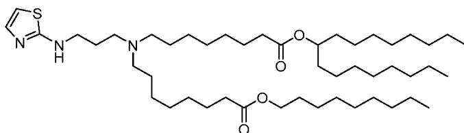
(Compound 208),
