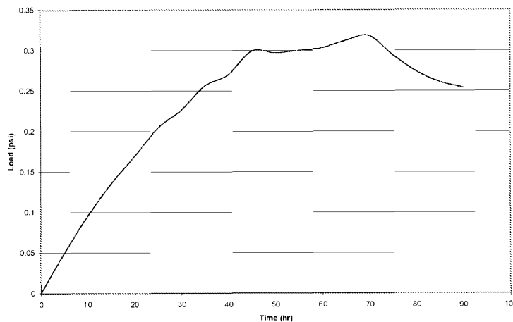
Swell Force of 5% 4armPEG-SH and 4armPEG-SC
