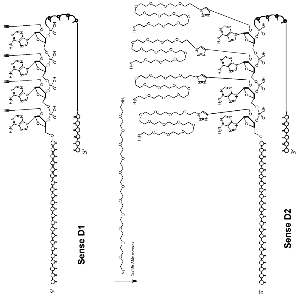
SCHEME D: Synthesis of GalNAc Nicked Tetraloop dsNA Conjugate with Multiple GalNAc on the Stem Post Synthetic Conjugation Using "Click" Chemistry
