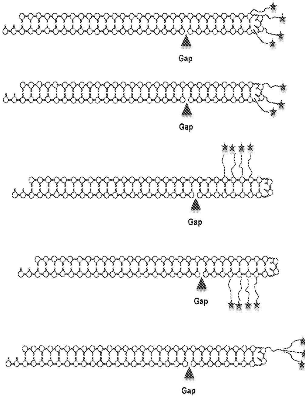
Fig 42 dsNA Conjugates with Nicked Tetraloop
