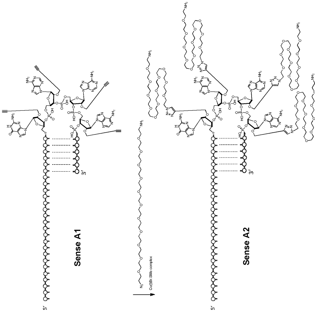
SCHEME A: Synthesis of GalNAc Nicked Tetraloop dsDNA Conjugate with Multiple GalNAc on the loop Post Synthetic Conjugation Using "Click" Chemistry
