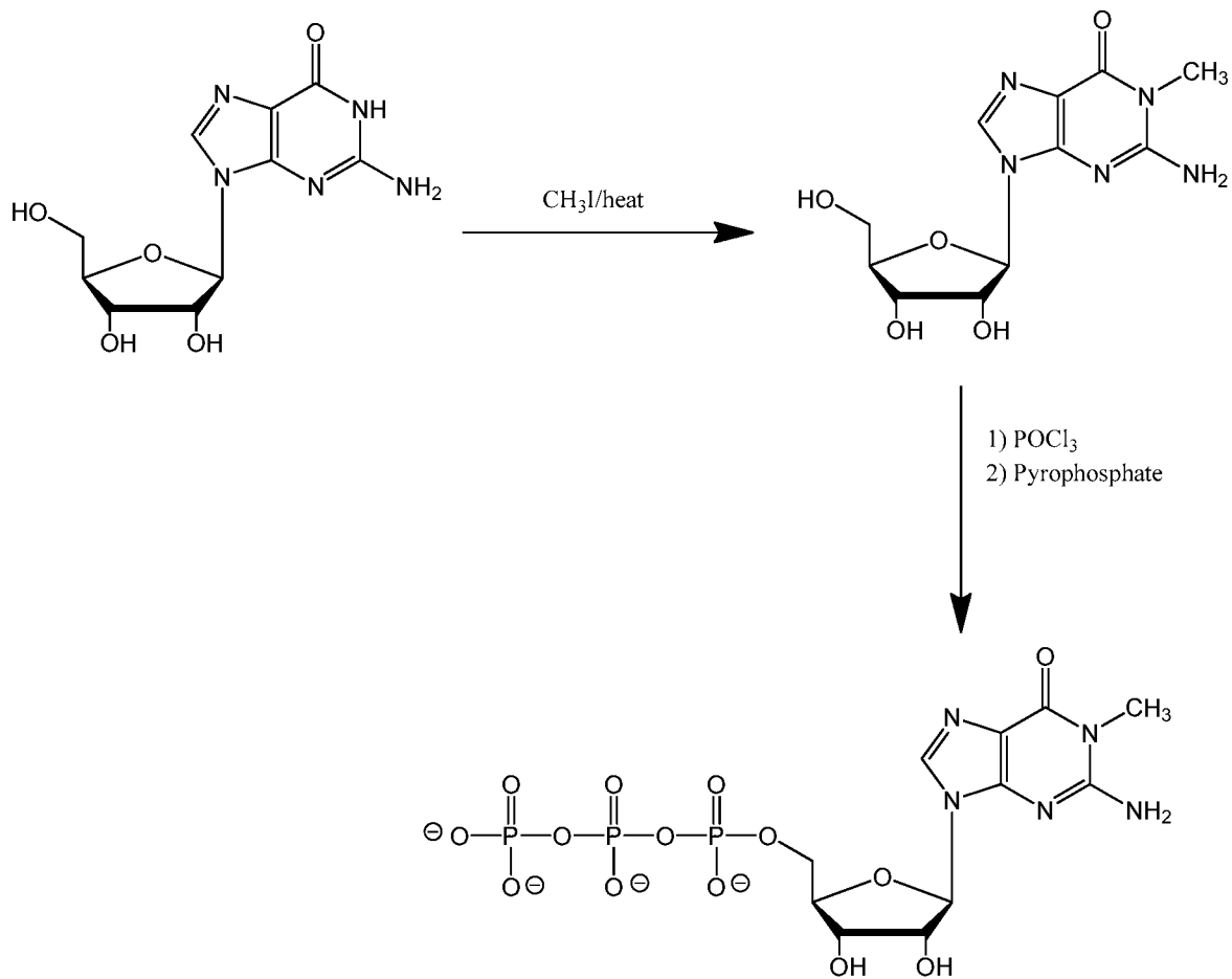
Scheme 3
