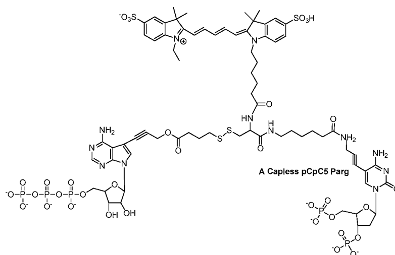
Scheme 12
