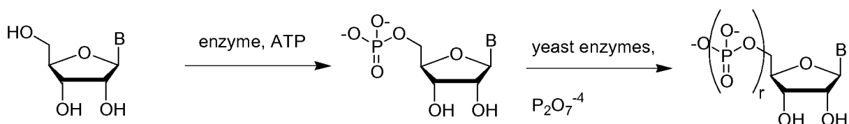
Scheme 10
