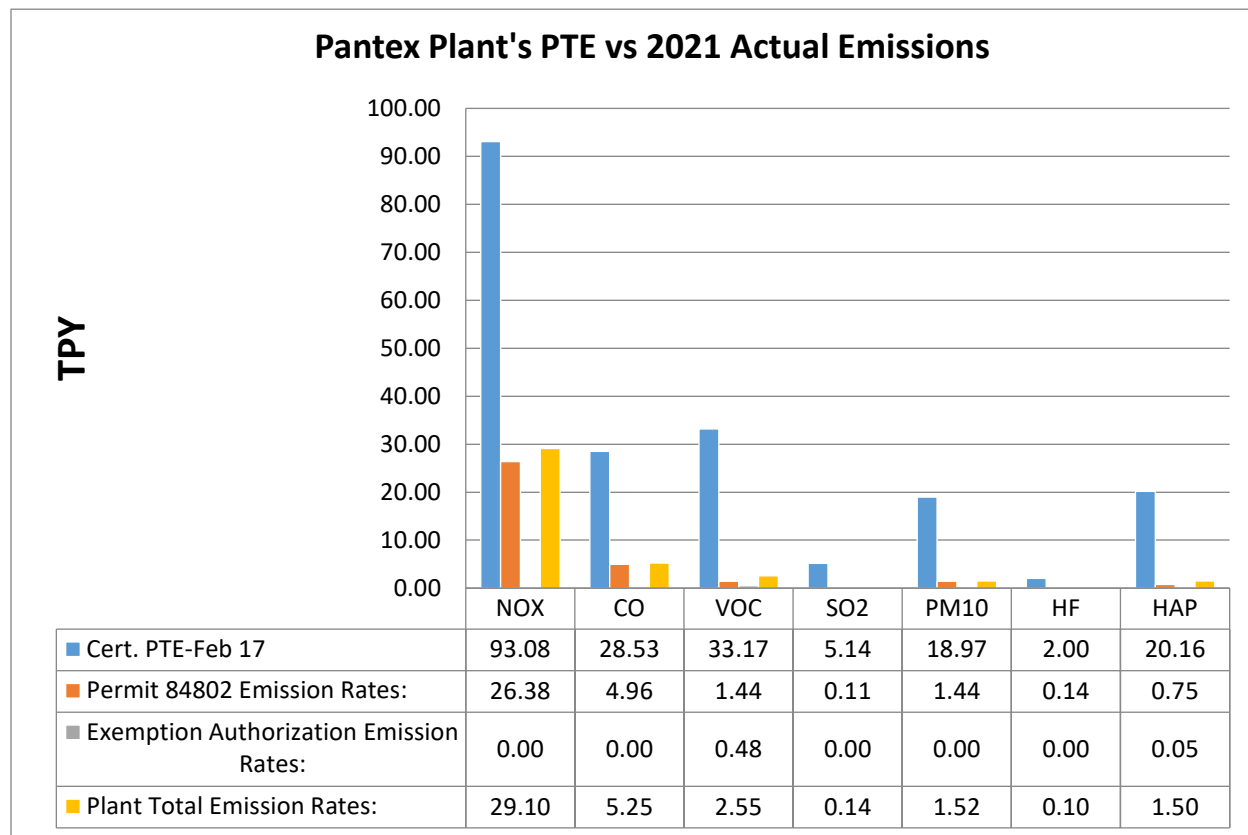
Figure 2.1 – Pantex Plant’s PTE vs January – December 2021 Actual Emissions
