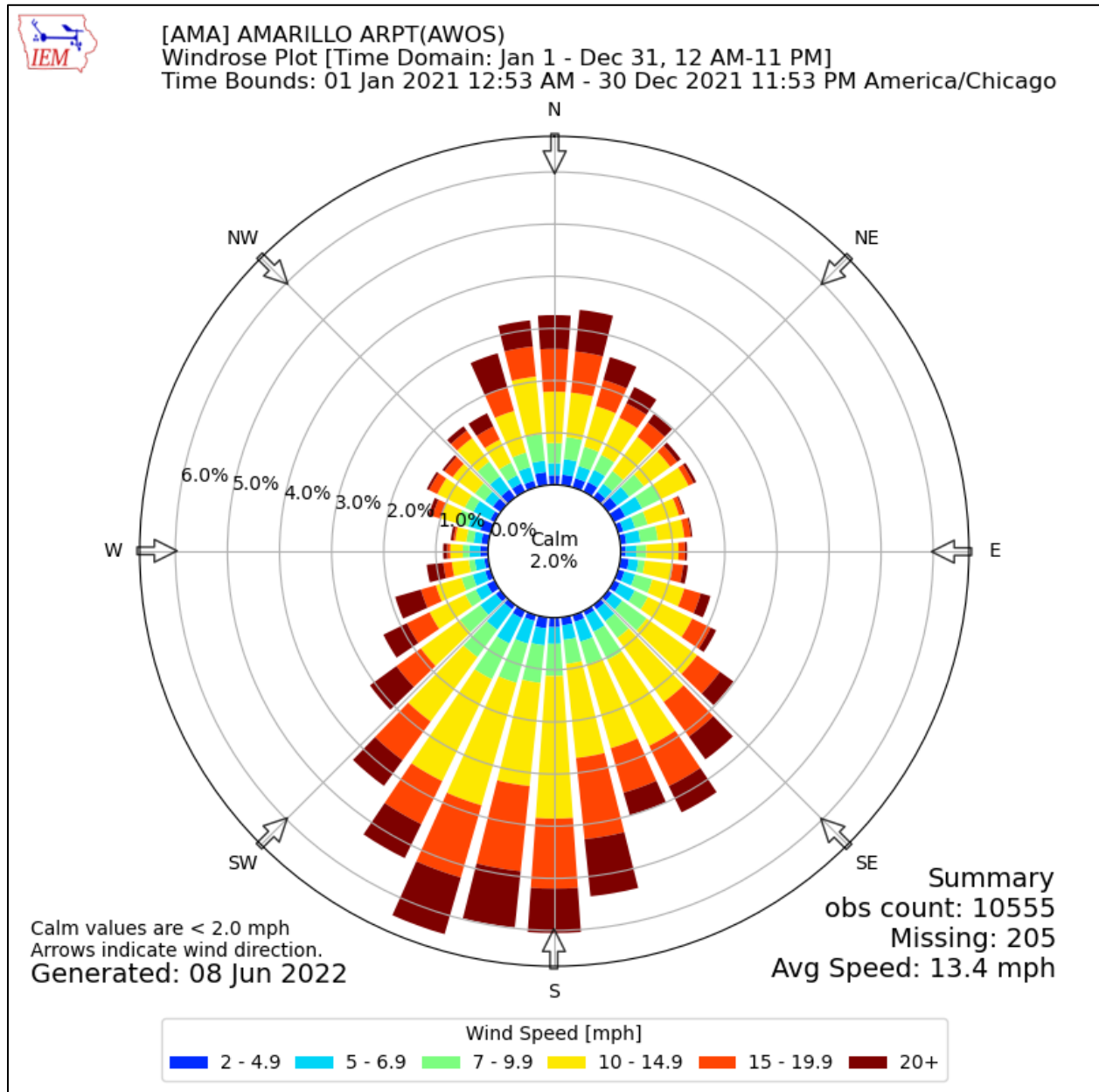
Figure 1.2 – Pantex Plant Annual Wind Rose for 2021 (Iowa Environmental Mesonet)
