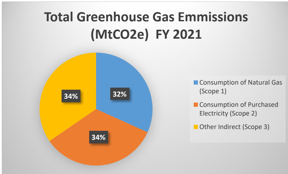
Figure 3.2 – Total 2021 GHG Emissions
