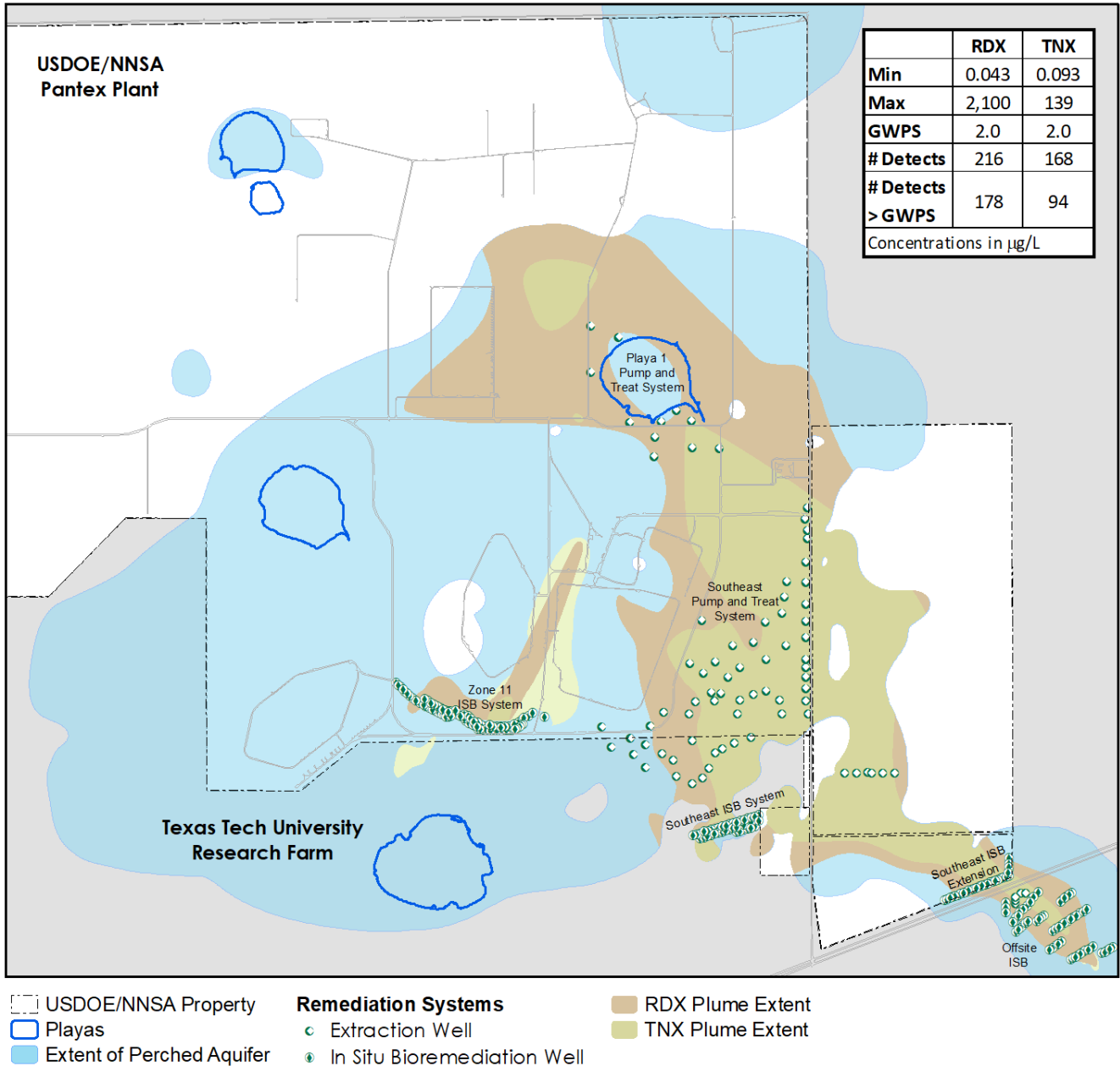
Figure 6.10 – RDX and Degradation Product Plume
