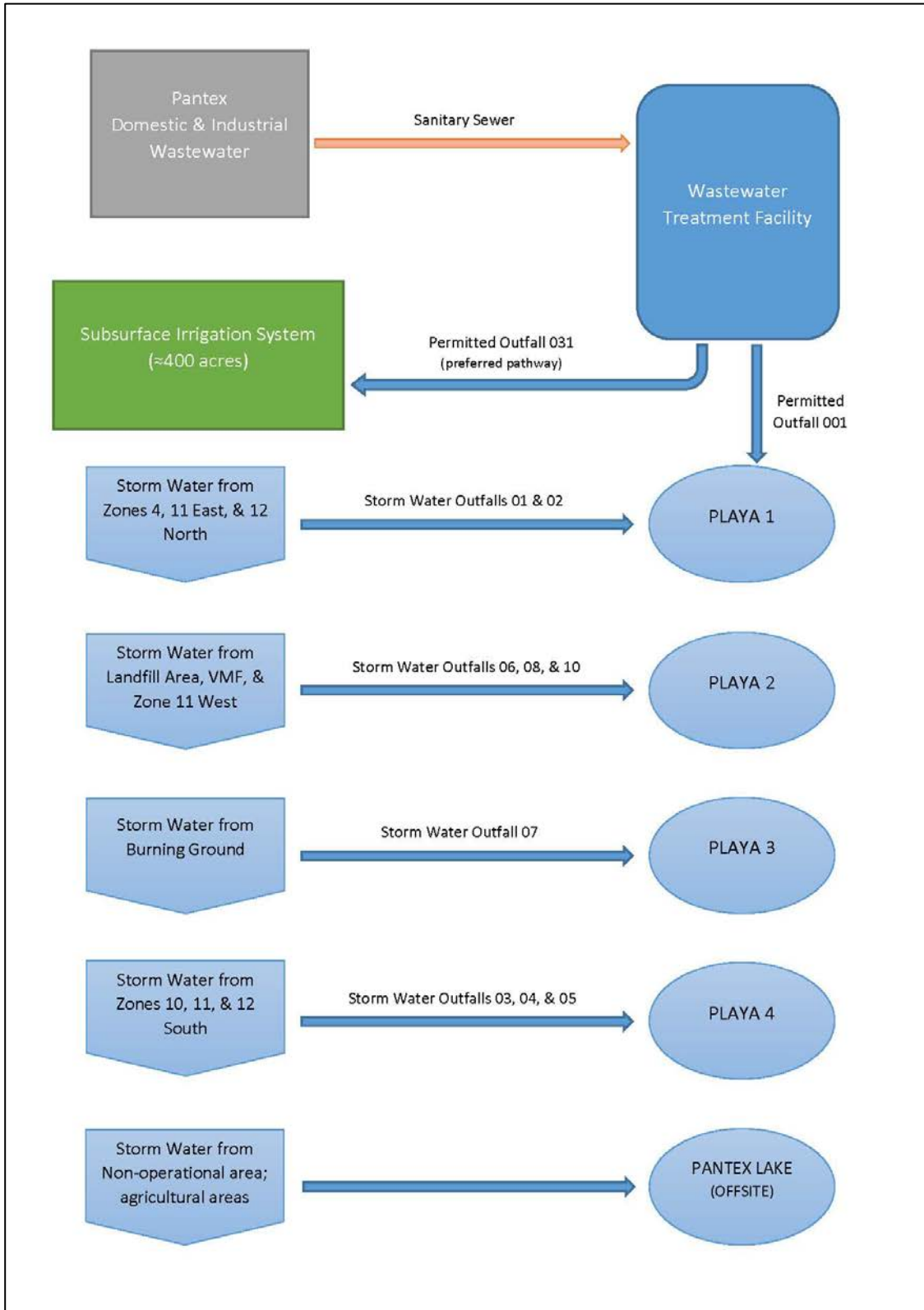
Figure 9.2 – Pantex Plant Surface Water Schematic
