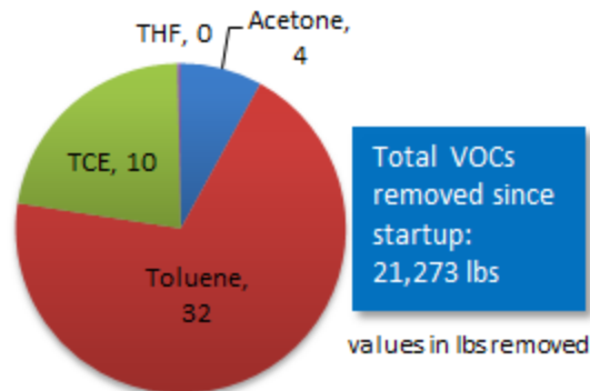
Figure 3.10 – 2021 SVE Mass Removal
