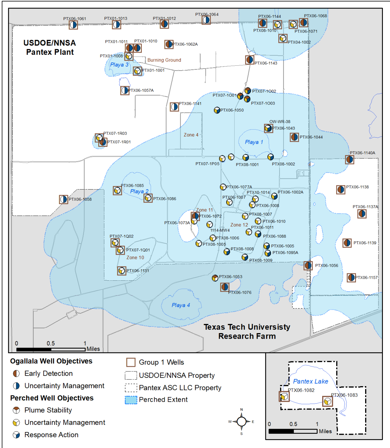
Figure 6.7 – Uncertainty Management and Early Detection Wells
