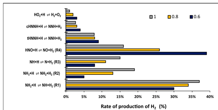
Figure 4. Rate of production analysis of \text{H}_2 in 70/30 vol% \text{NH}_3/\text{H}_2 premixed flame at lean conditions estimated by the Glarborg, [90] kinetic model.
