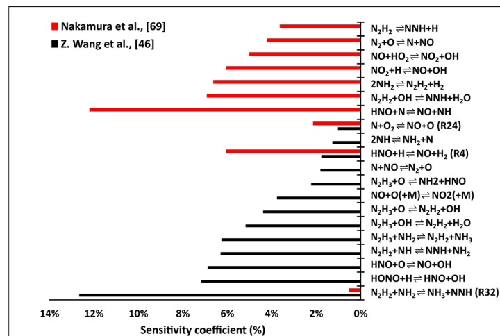
Figure 20. Reactions with the largest negative sensitivity coefficients for NO in 70/30 (vol%) NH 3 /H 2 premixed flame at \phi = 1.2 estimated by the Nakamura et al., [69] and Z. Wang et al., [46] kinetic models.
