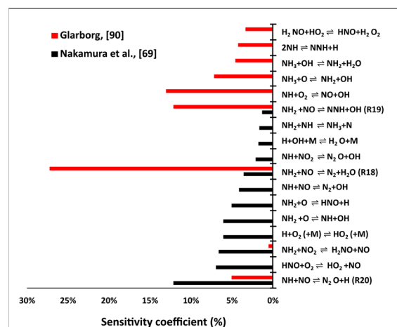
Figure 6. Reactions with the largest negative sensitivity coefficients for NO in 70/30 vol% NH 3 /H 2 premixed flame at \phi = 0.8 estimated by the Glarborg, [90] and Nakamura et al., [69] kinetic models.
