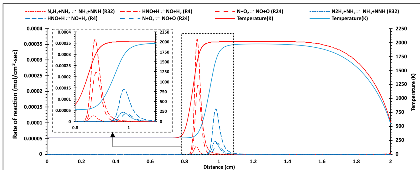
Figure 21. The reaction rate profiles of reactions most influential to the formation/reduction of NO mole fractions for 70/30 vol% \text{NH}_3/\text{H}_2 mixture at \phi = 1.2 ; The result for the Nakamura et al., [69] and Z. Wang et al., [46] models are shown with red and blue lines, respectively.
