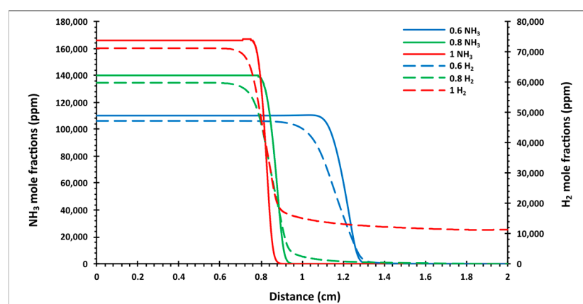
Figure 3. Variation of \text{NH}_3 and \text{H}_2 mole fractions as a function of axial distance at lean flame conditions ( \phi = 0.6, 0.8, 1 ) estimated by the Glarborg,[90] kinetic model.
