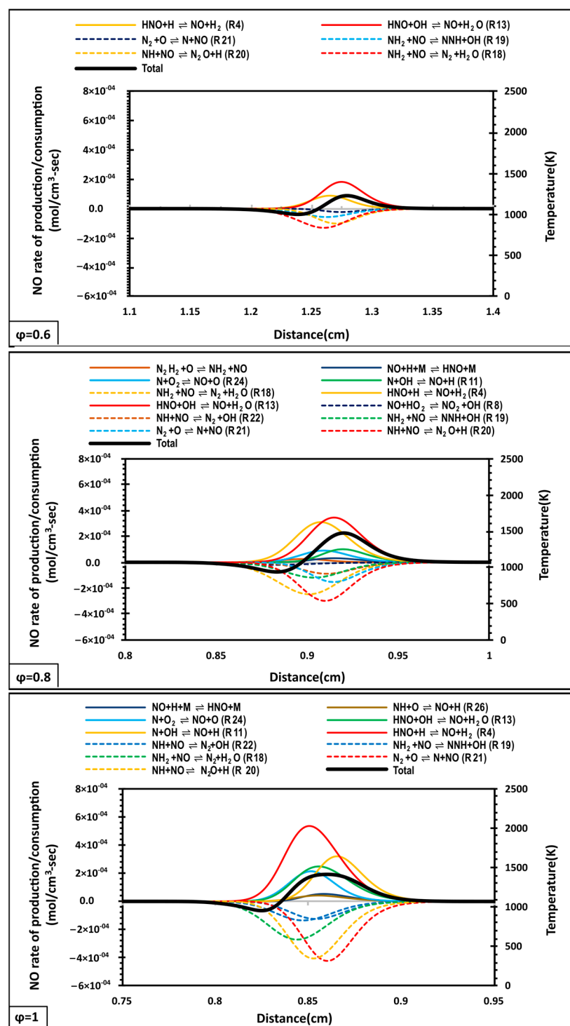
Figure 7. The rate of production/consumption of NO in 70/30 (vol%) \text{NH}_3/\text{H}_2 mixture at lean conditions estimated by the Nakamura et al., [69] kinetic model.
