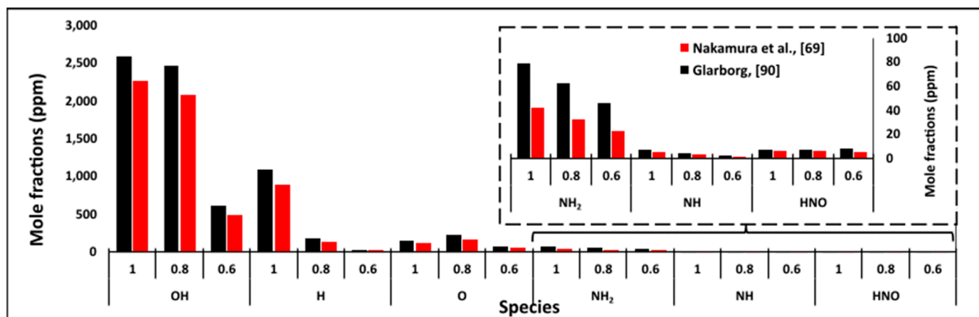
Figure 10. Varieties of mole fractions of OH, H, O, \text{NH}_2 , NH, HNO as a function of equivalence ratio estimated by two selected kinetic models.
