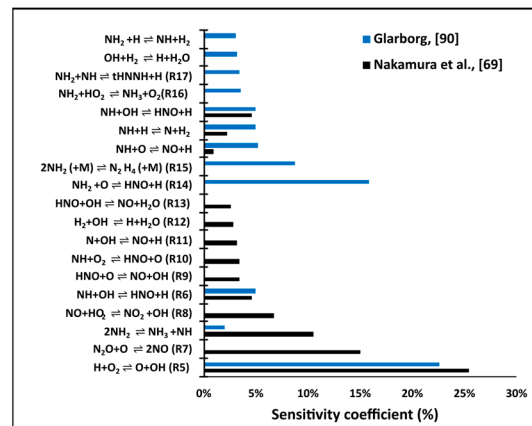
Figure 5. Reactions with the largest positive local sensitivity coefficient for NO in 70/30 vol% NH 3 /H 2 premixed flame at \phi = 0.8 estimated by the Glarborg, [90] and Nakamura et al., [69] kinetic models.
