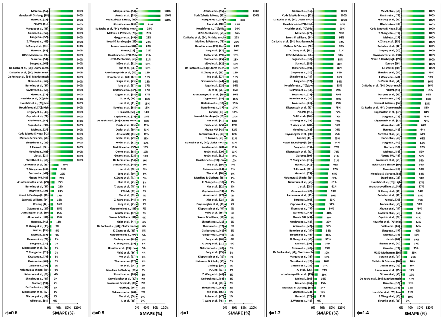
Figure 1. NO mole fractions for 67 reaction mechanisms calculated by symmetric mean absolute percentage error (SMAPE) formula at various equivalence ratios ( \phi ).
