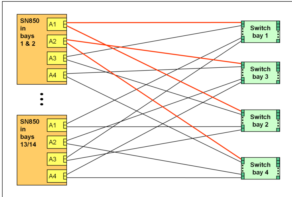
Figure 10. Logical layout of the interconnects between I/O adapters and I/O modules
