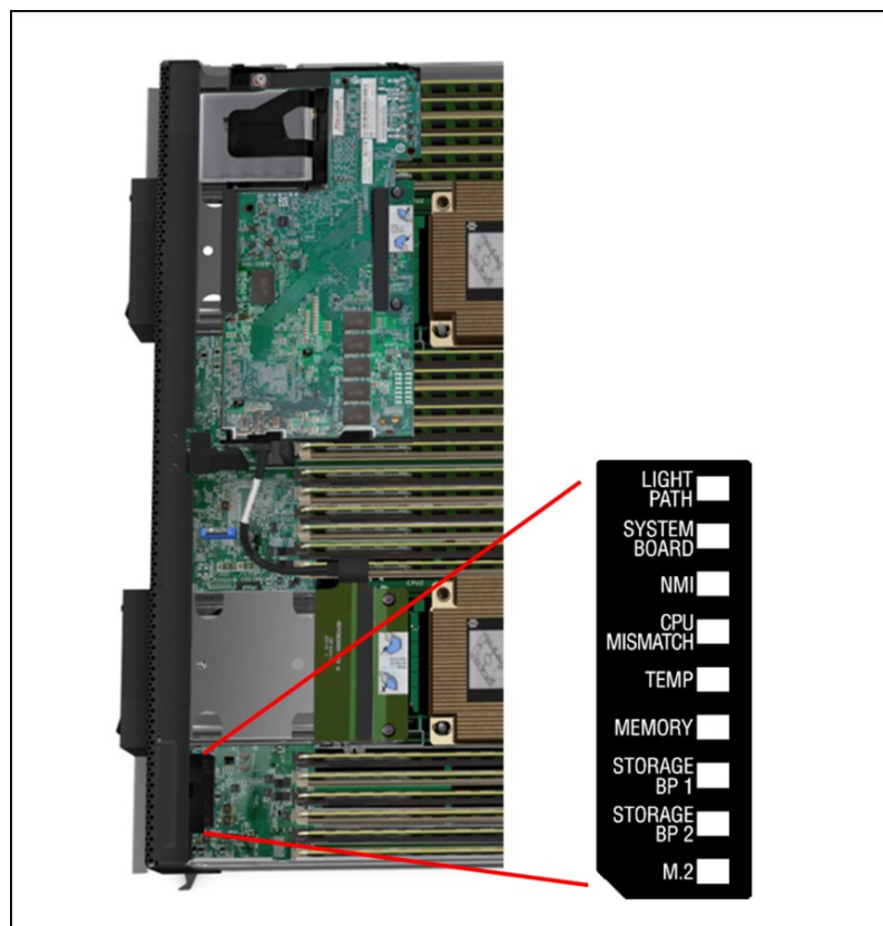
Figure 11. Location of SN850 light path diagnostics panel
