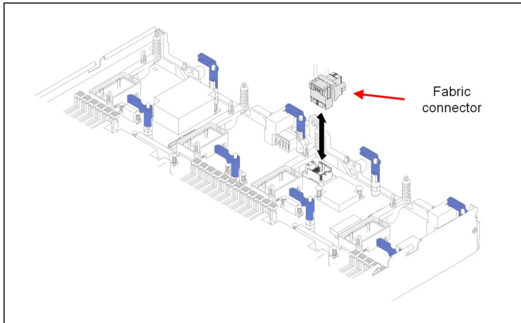
Figure 7. Location of fabric connector in SN850 server
