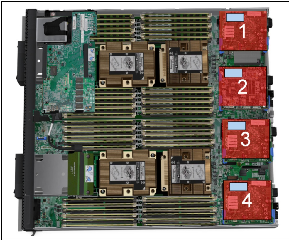
Figure 8. Location of the I/O adapter slots in the SN850 server
