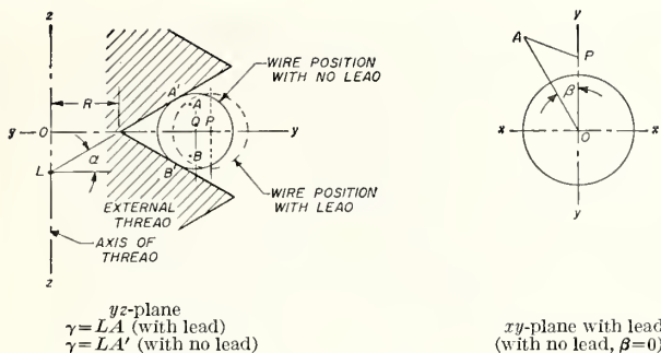
FIGURE 13.1.—Basis of lead angle correction for external thread.
