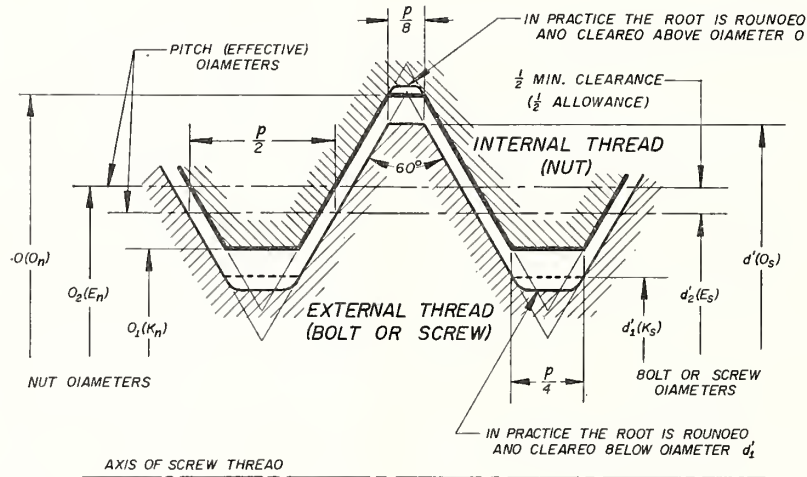
FIGURE 14.2.—ISO design profile of external and internal threads with an allowance for inch and metric screw threads.
