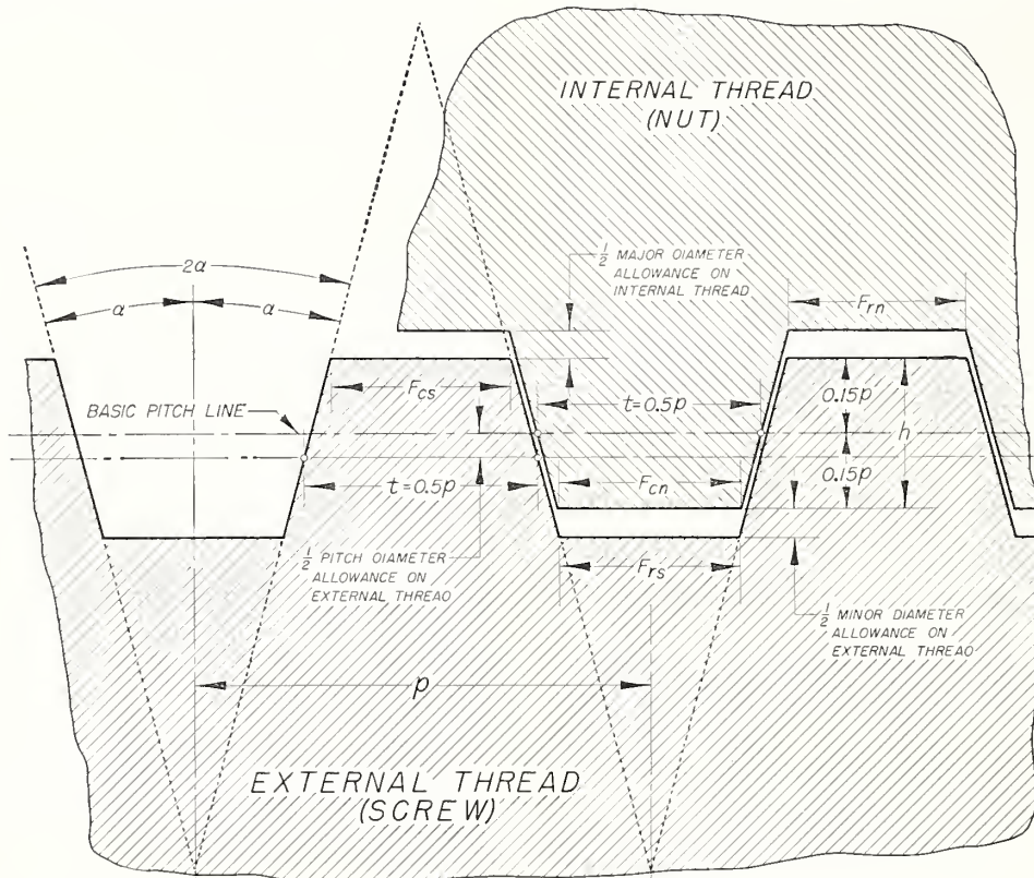
FIGURE XIII.1.—Standard Stub Acme form of thread.
