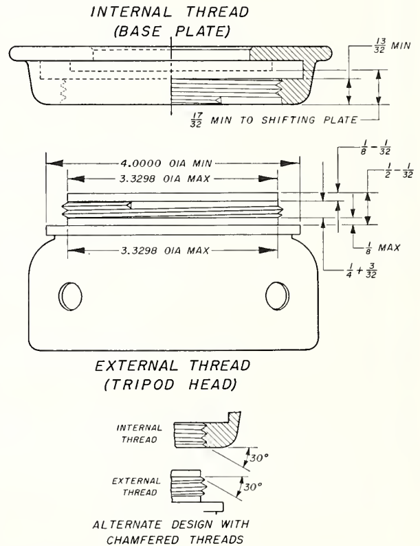
FIGURE XVII.1.—Surveying instrument tripod head and base plate.
