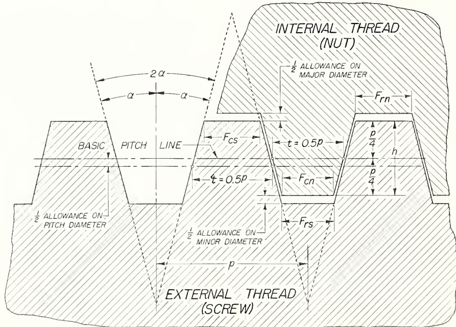
FIGURE XII.1.—General purpose Acme thread form.
