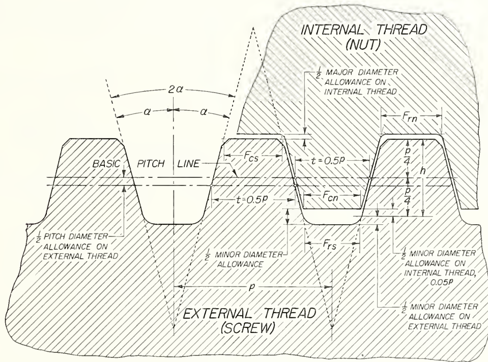
FIGURE XII.2.—Centralizing Acme thread form.
