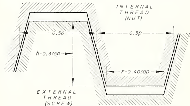
FIGURE XIII.3.—Modified Form 1 Stub Acme thread with basic height of 0.375 pitch.
