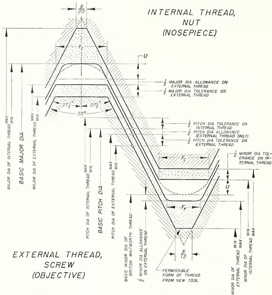
FIGURE XVI.2.—Disposition of tolerances, allowances, and crest clearances for 0.800—36 AMO thread.
