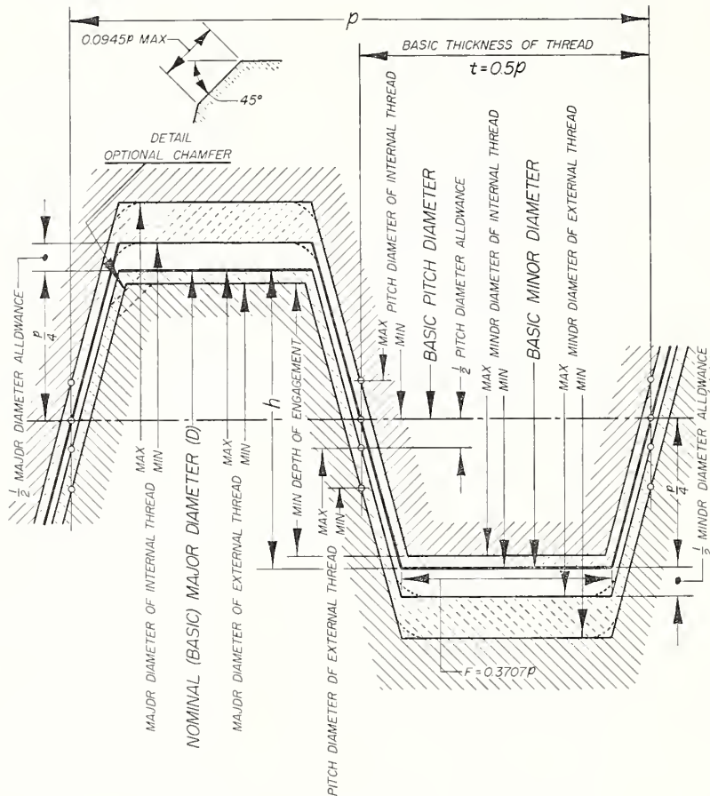
FIGURE XII.3.—Illustration of allowances, tolerances, and crest clearances, general purpose Acme threads, classes 2G, 3G, and 4G.
