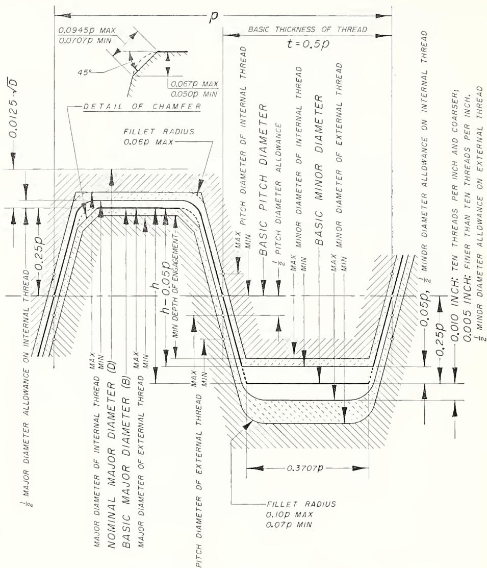
FIGURE XII.5.—Illustration of allowances, tolerances, and crest clearances, centralizing Acme threads, classes 5C and 6C.
