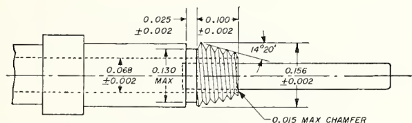
FIGURE XVIII.8.—Shutter cable release tip with taper (European) thread (50 tpi).
