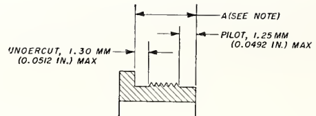
FIGURE XVIII.7.—Length, pilot, and undercut of attachment threads for lens accessories.
