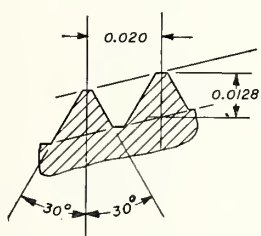
FIGURE XVIII.9.—Thread details for shutter cable release tip and socket with taper (European) thread (50 tpi).
