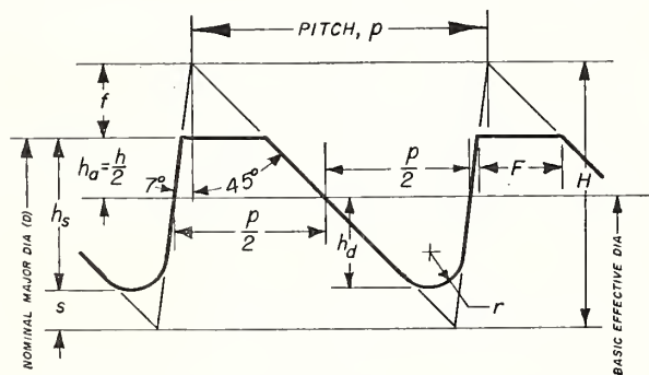
FIGURE XIV.3.—British Standard form of Buttress thread.
