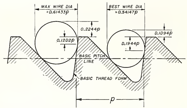
FIGURE 13.2.—Diameters of “best” and “maximum” thread wires for Buttress threads.
