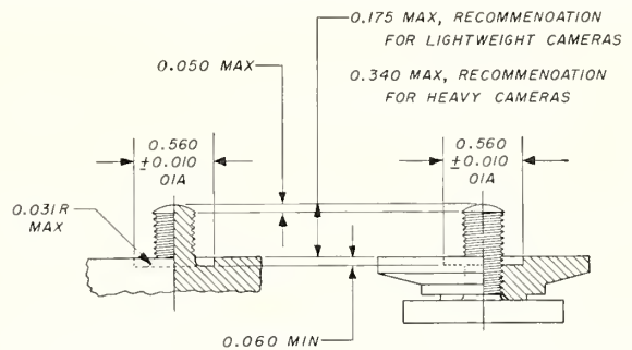
FIGURE XVIII.1.—Tripod screw, \frac{1}{4} -20 UNC-1A.
