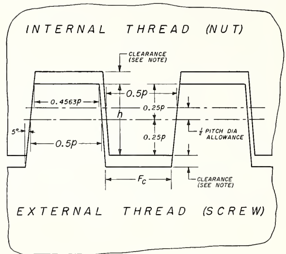
FIGURE XIX.1.—Modified square thread (10° included angle), basic proportions.
