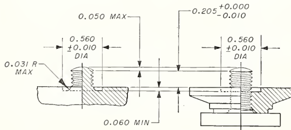
FIGURE XVIII.4.—Tripod screw, 3/8—16 UNC—1A
