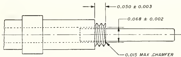
FIGURE XVIII.10.—Shutter cable release tip with straight (American) thread.
