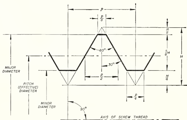
FIGURE 14.1.—ISO basic profile for inch and metric screw threads.
