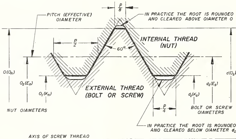
FIGURE 14.3.—ISO design profile of external and internal threads without an allowance for inch and metric screw threads.
