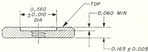
FIGURE XVIII.3.—Spacer for use on tripod with 0.340-in. length screw, 1/4—20 UNC—1B.
