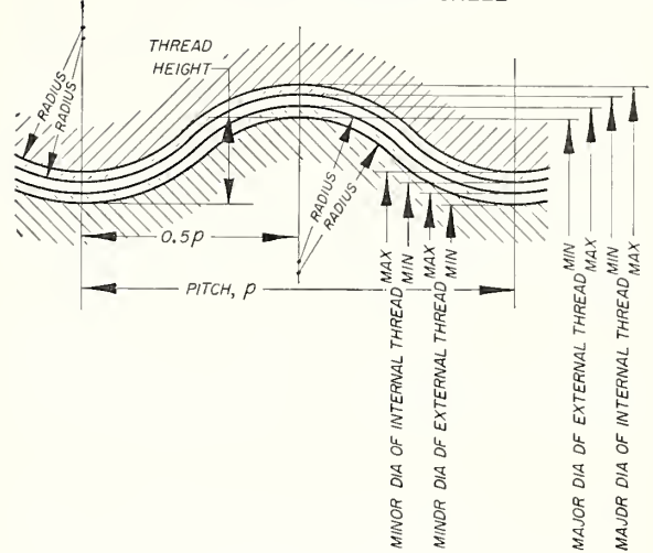
FIGURE XV.1.—Illustration of thread form, allowance, and tolerances, American Standard rolled threads for screw shells of electric lamp holders and lamp bases.
