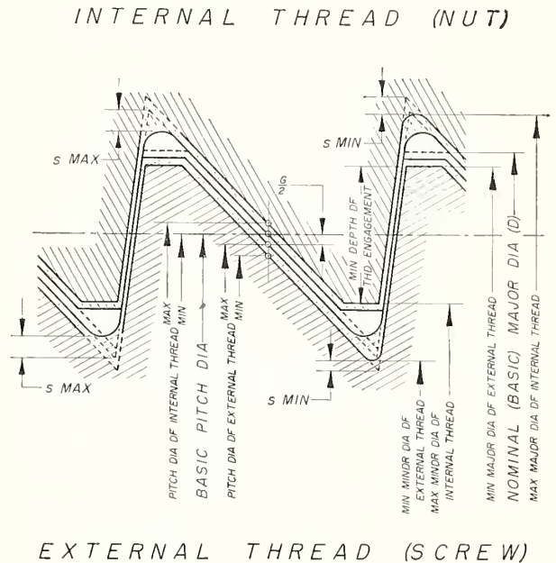
FIGURE XIV.2.—Illustration of tolerances, allowances, and root truncations, Buttress threads.
