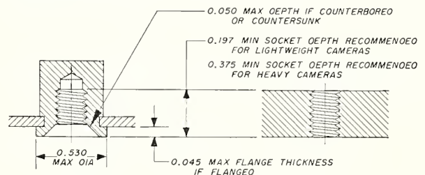
FIGURE XVIII.2.—Tripod socket in camera, \frac{1}{4} -20 UNC-1B.
