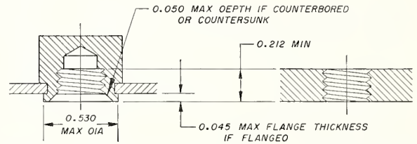
FIGURE XVIII.5.—Tripod socket in camera, 3/8—16 UNC—1B.
