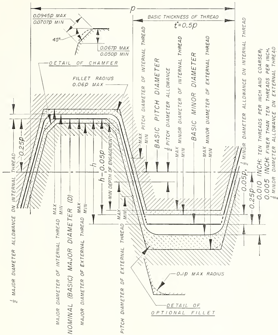
FIGURE XII.4.—Illustration of allowances, tolerances, and crest clearances, centralizing Acme threads, classes 2C, 3C, and 4C.
