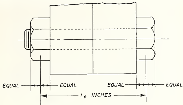
FIGURE 12.1.—Effective length applicable in elongation formula.
