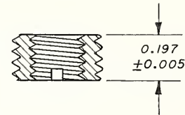
FIGURE XVIII.6.—Adapter; 3/8—16 UNC—1A external thread, 1/4—20 UNC—1B internal thread.
