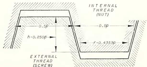
FIGURE XIII.4.—Modified Form 2 Stub Acme thread with basic height of 0.25 pitch.
