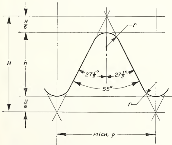
FIGURE XVI.3.—Basic form of Whitworth thread.
