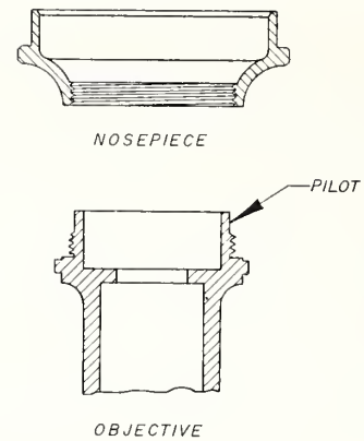
FIGURE XVI.1.—Typical arrangement of microscope objective and nosepiece.
