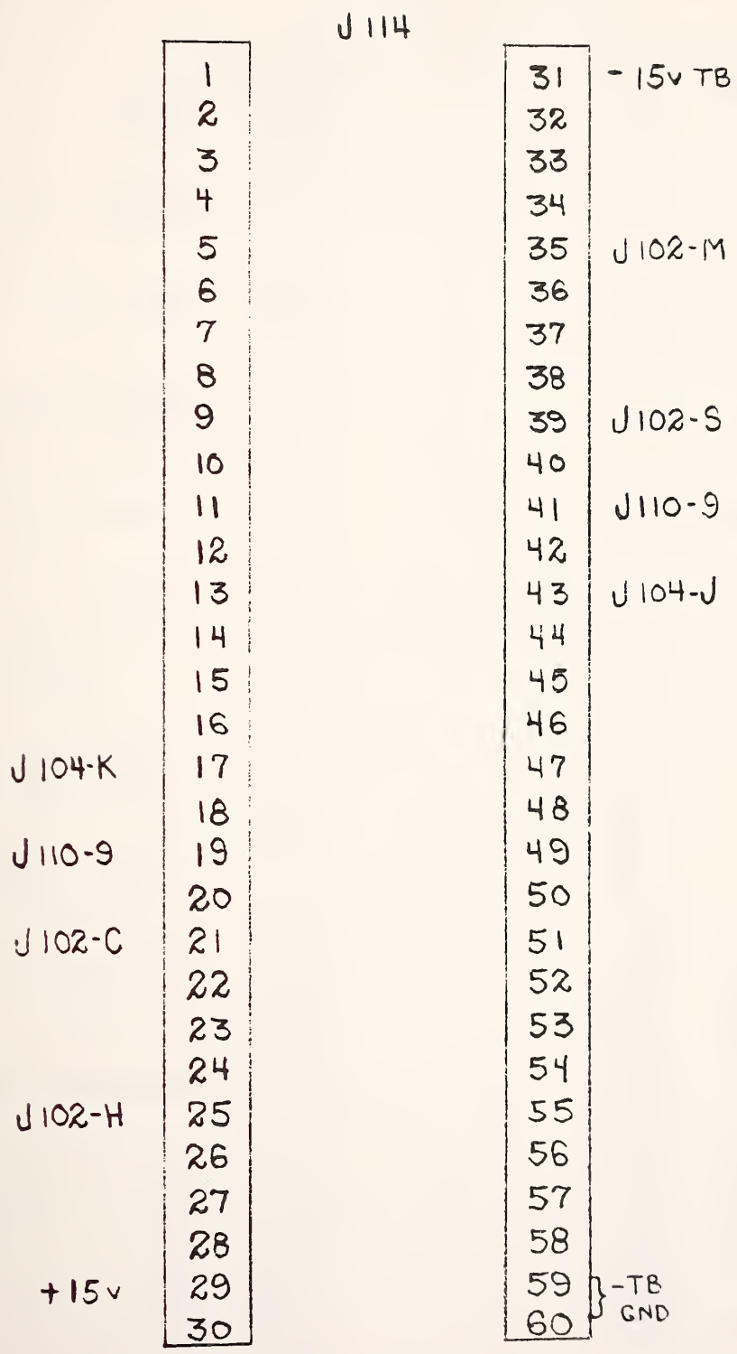
J114, SWITCH DRIVER CARD INPUT AND OUTPUT CONNECTOR
