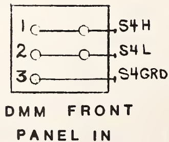
NOISE STANDARDS WIRING DIAGRAM AND SCANNER CONNECTIONS
