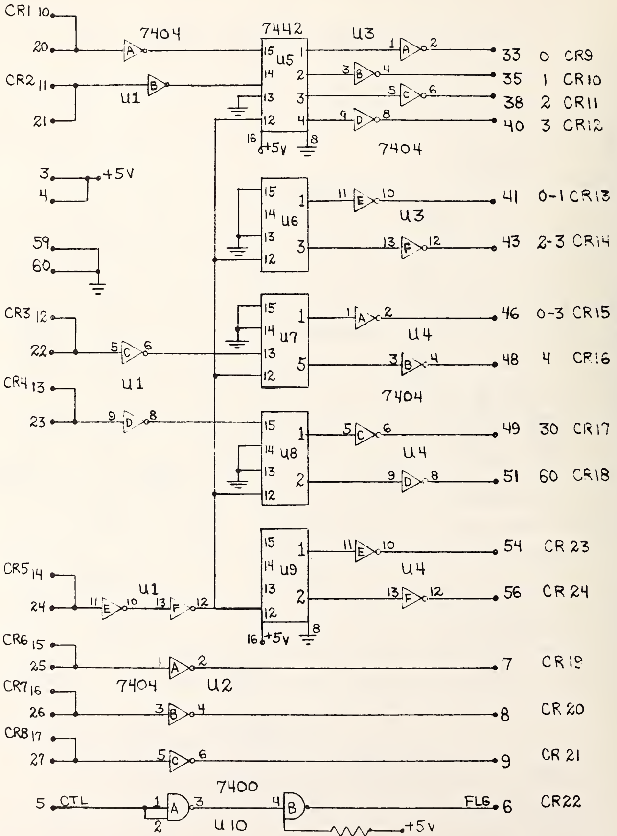
110 DECODER CARD SCHEMATIC DIAGRAM
