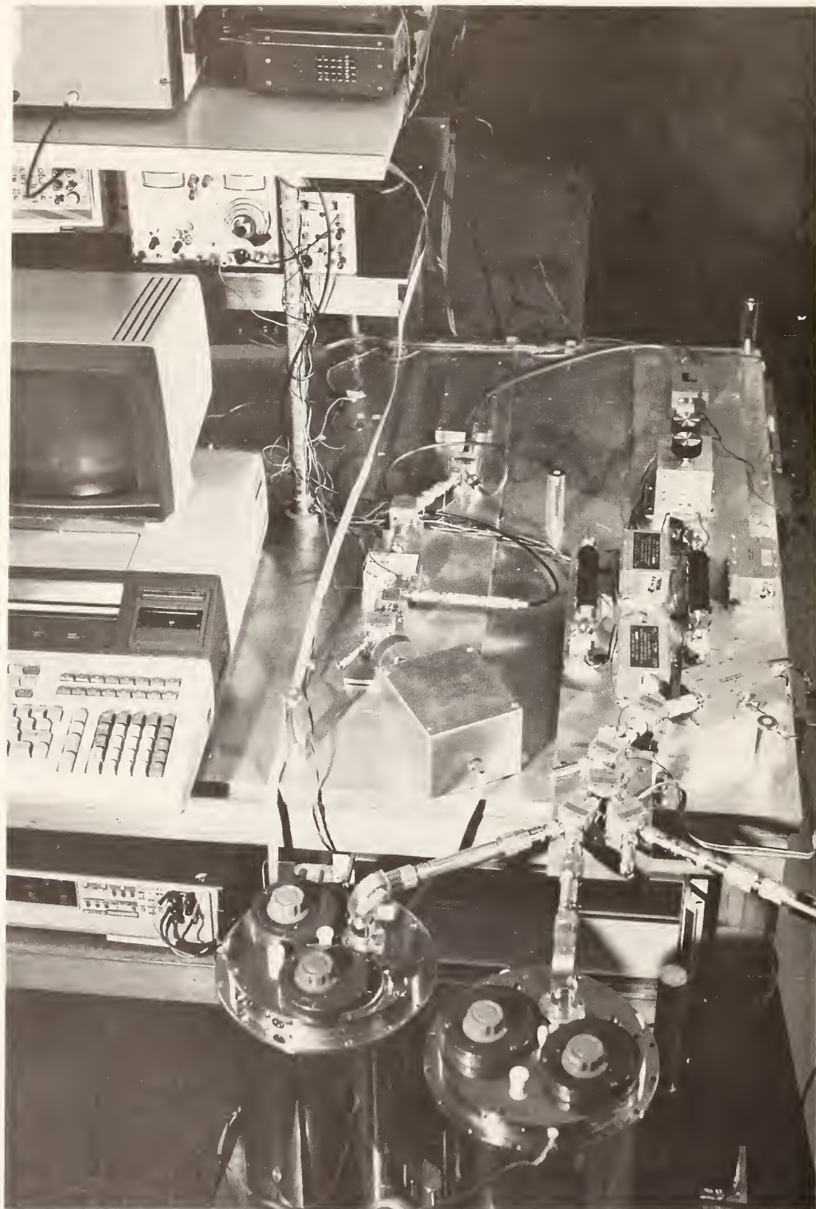
30/60 MHz RADIOMETER
