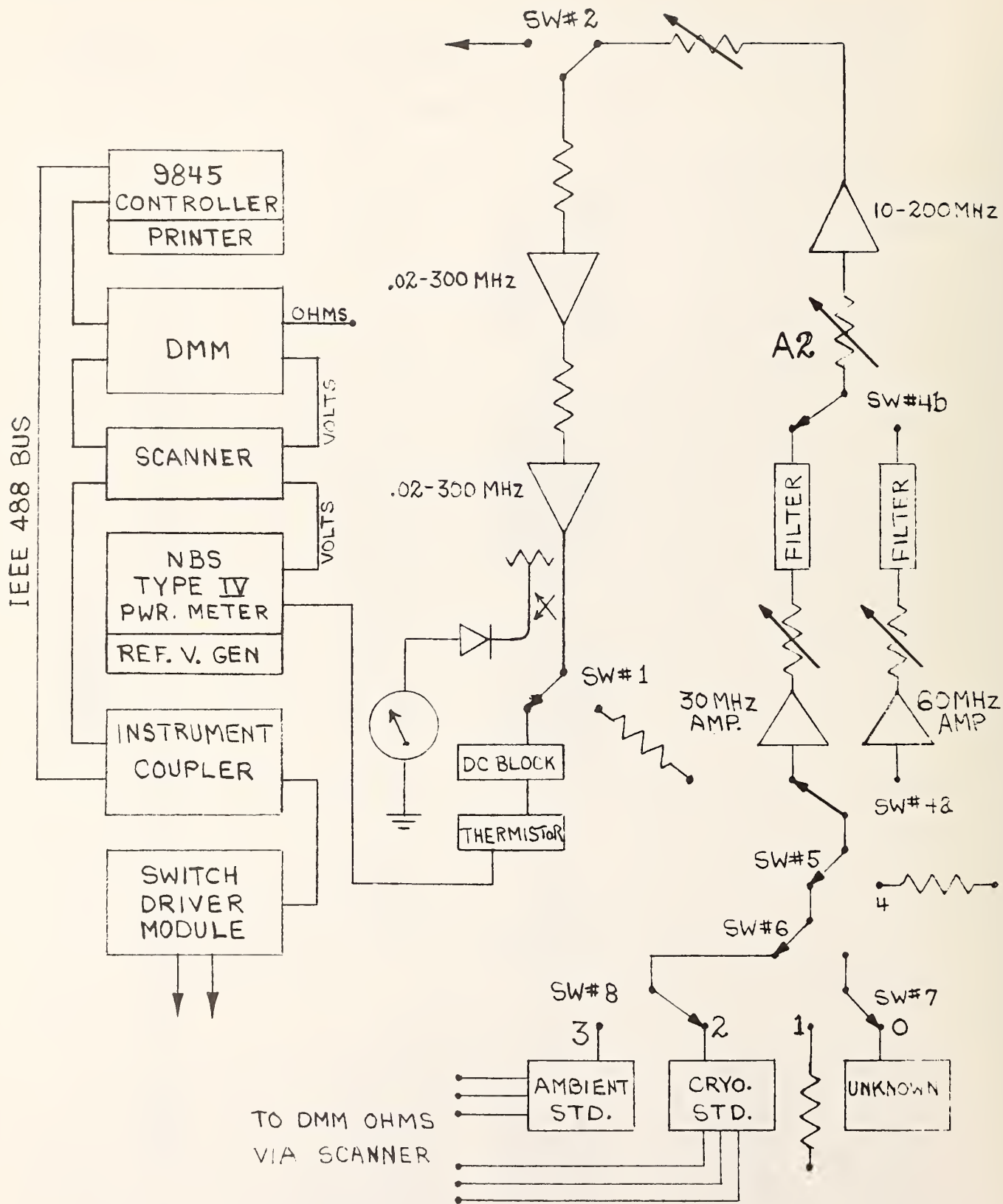
30/60 MHz RADIOMETER BLOCK DIAGRAM
