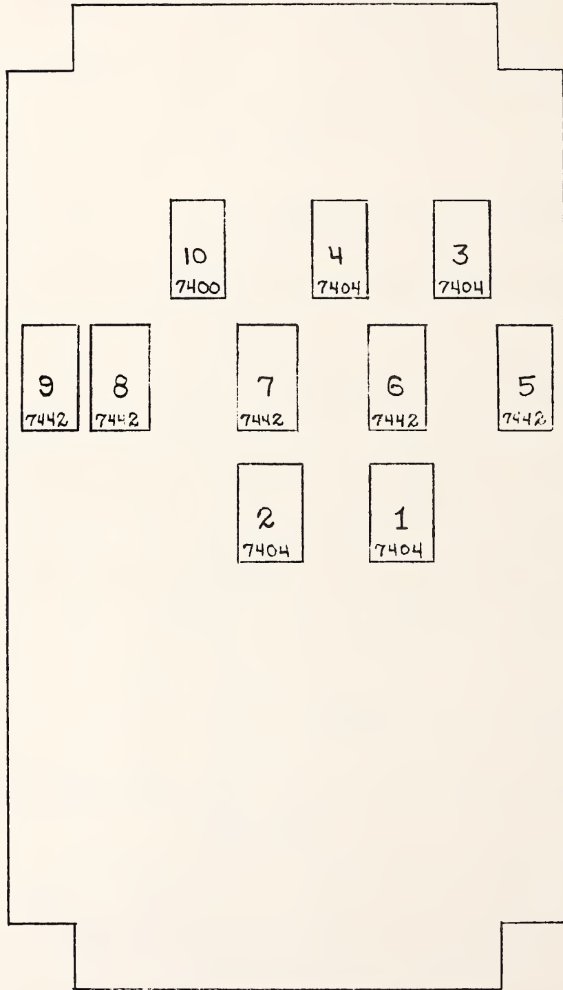
110 DECODER CARD PARTS PLACEMENT
