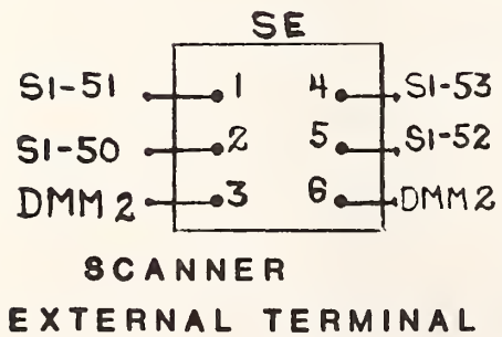
NOISE STANDARDS WIRING DIAGRAM AND SCANNER CONNECTIONS
