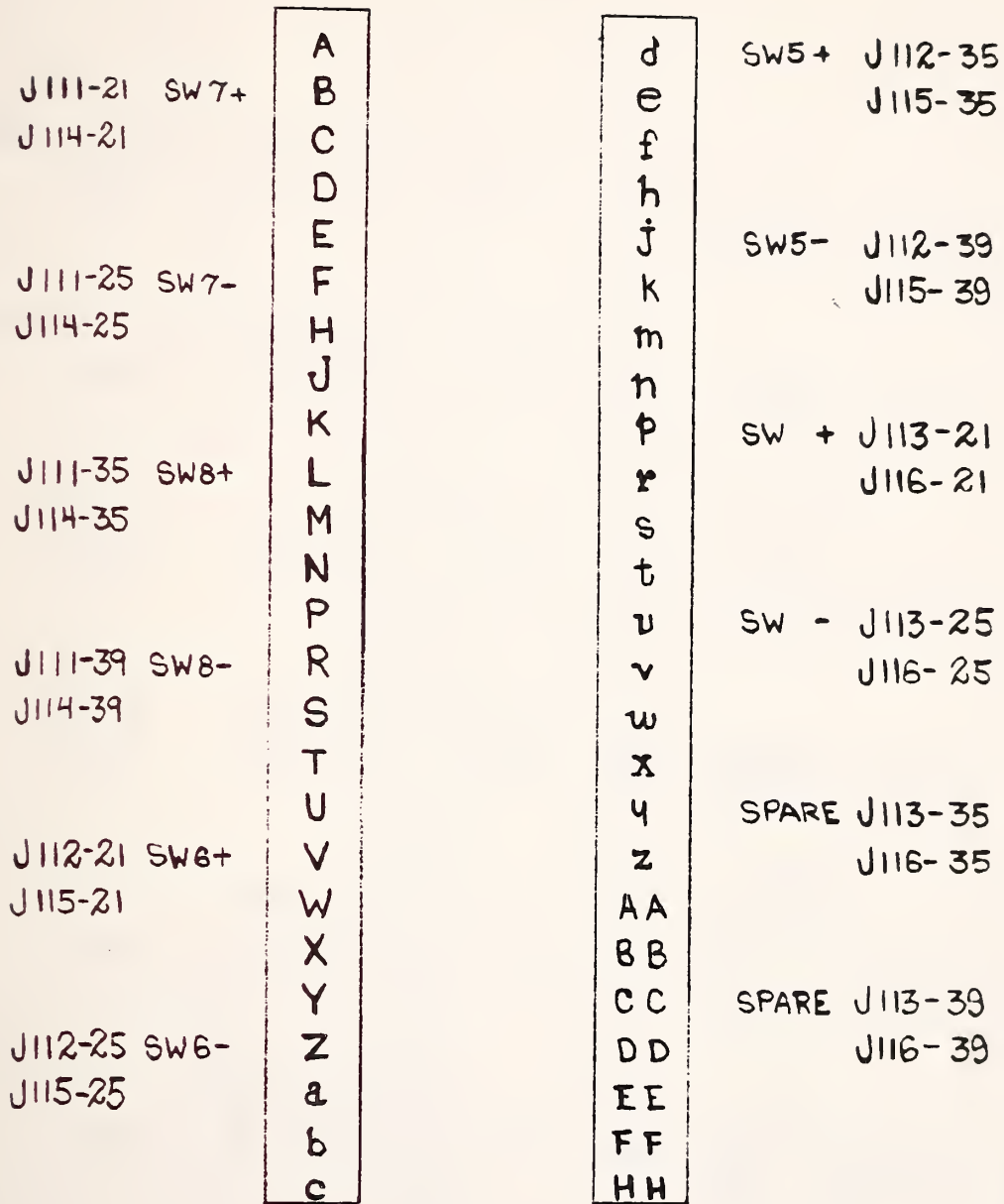
PIN CONNECTIONS FOR J102, SWITCH DRIVER MODULE OUTPUT
