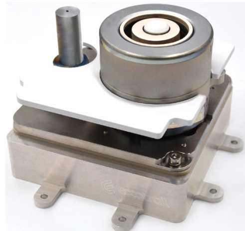
Figure 4.36: spaceware-micro thruster. Credit: Exotrail.
