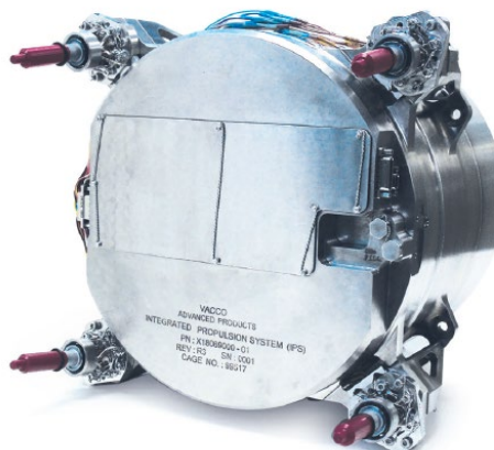
Figure 4.12: VACCO Industries IPS. Credit: VACCO Industries.
