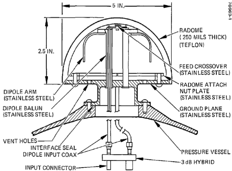
Figure 5.2—Illustration of Venus Probe LGA
