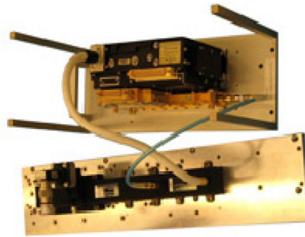
Figure 5.5—Image of Representative TWTA and EPC.
