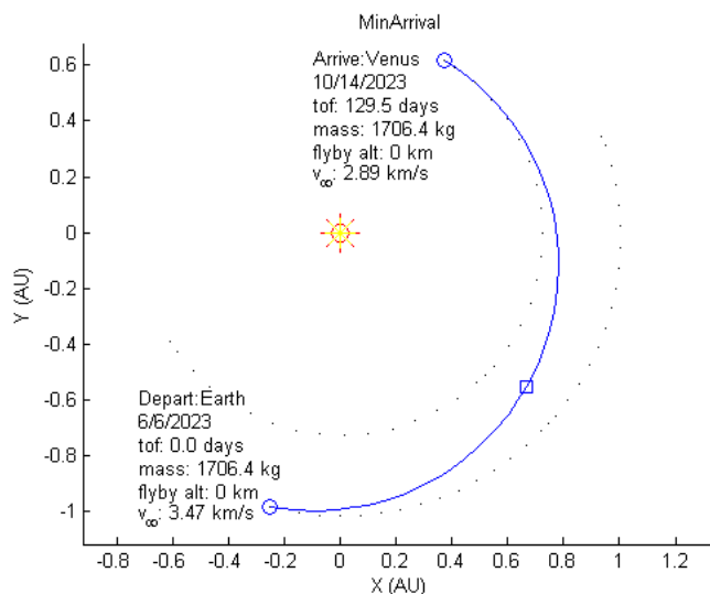
Figure 2.7—Minimum arrival energy solution.
