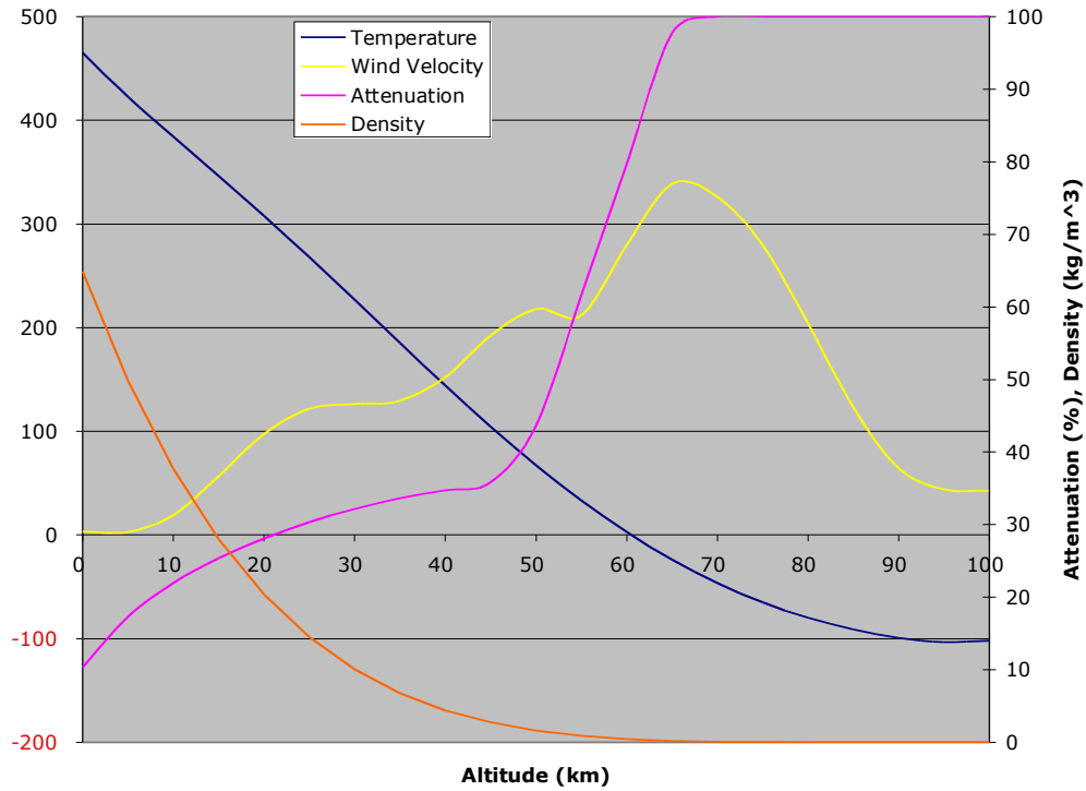
Figure 5.20—Venus atmospheric properties.
