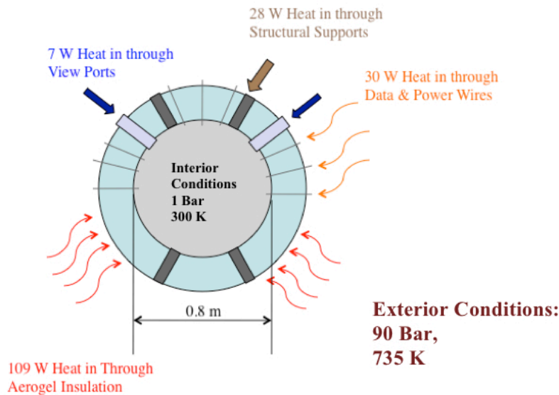
Figure 5.25—Heat leak into the Lander electronics enclosure pressure vessel.
