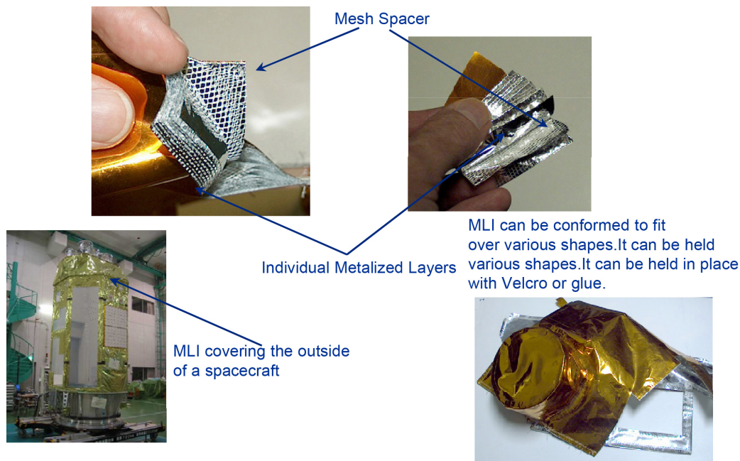
Figure 5.17—Example of MLI blanket design and application.
