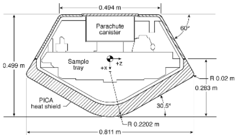
Figure 5.23—Stardust Aeroshell Geometry
