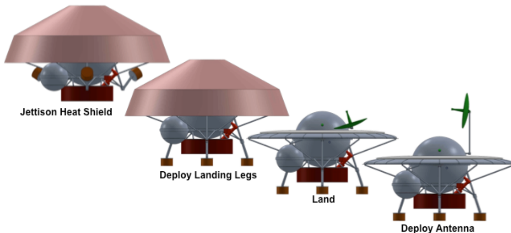
Figure 2.19—Landing legs and X-band antenna deployment sequence.
