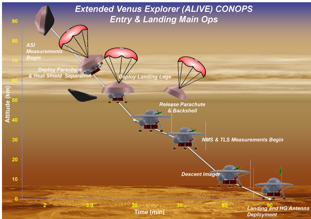
Figure 2.9—ALIVE EDL operations.
