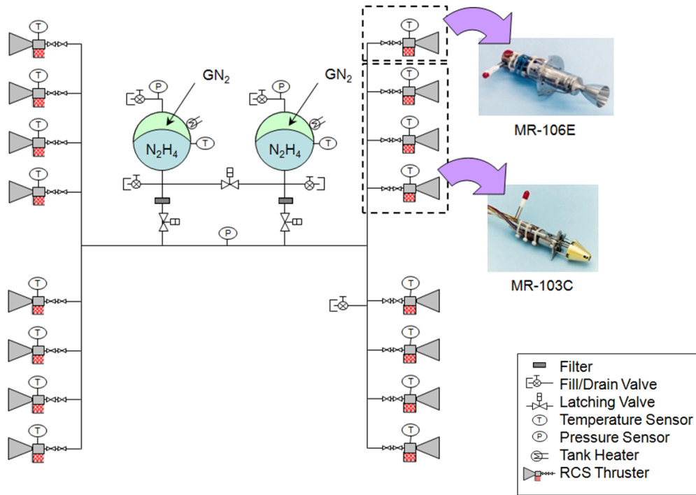
Figure 5.14—Preliminary Cruise Deck Propulsion P&ID
