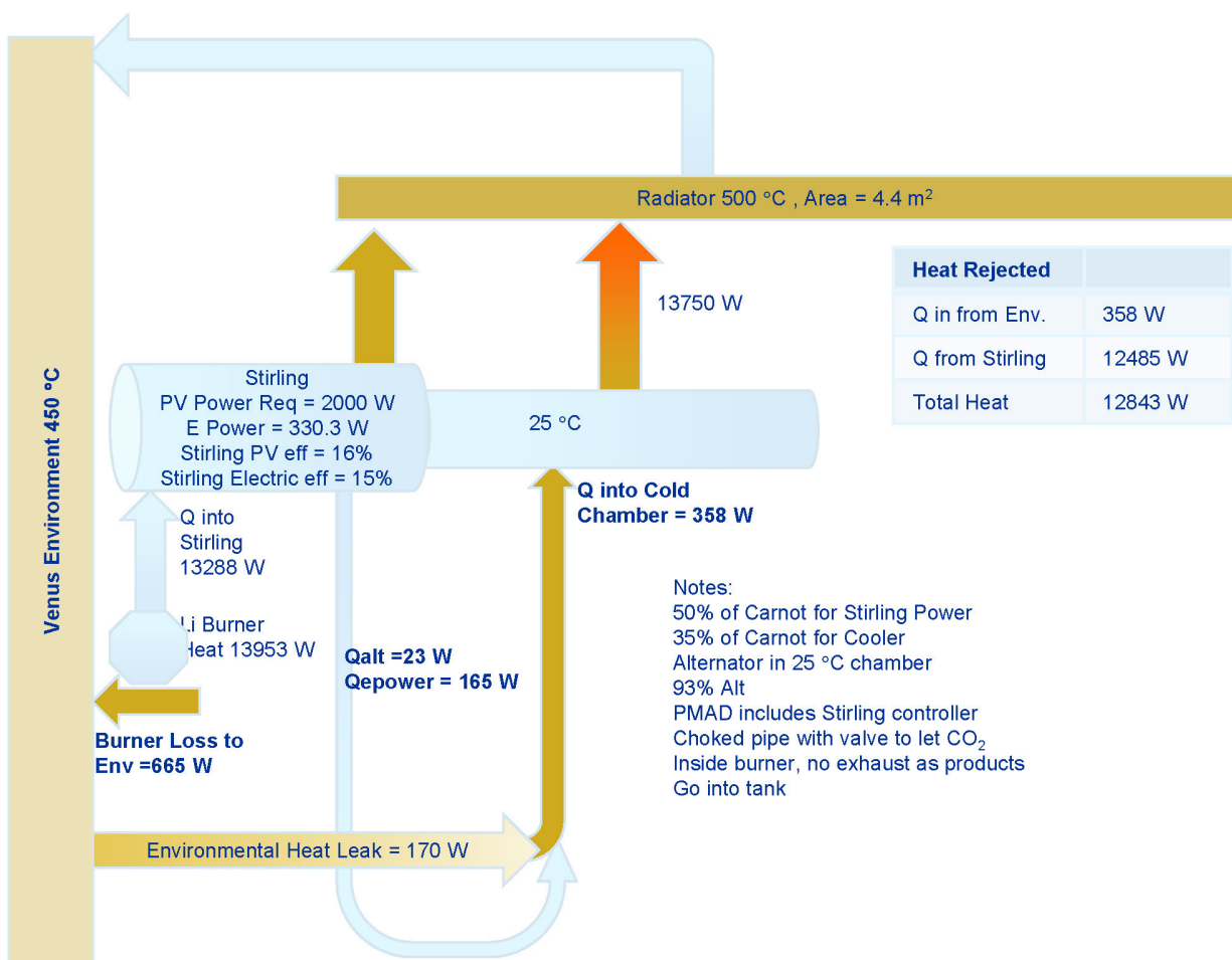
Figure 5.11—Heat and power flows for ALIVE Power and Cooling System.
