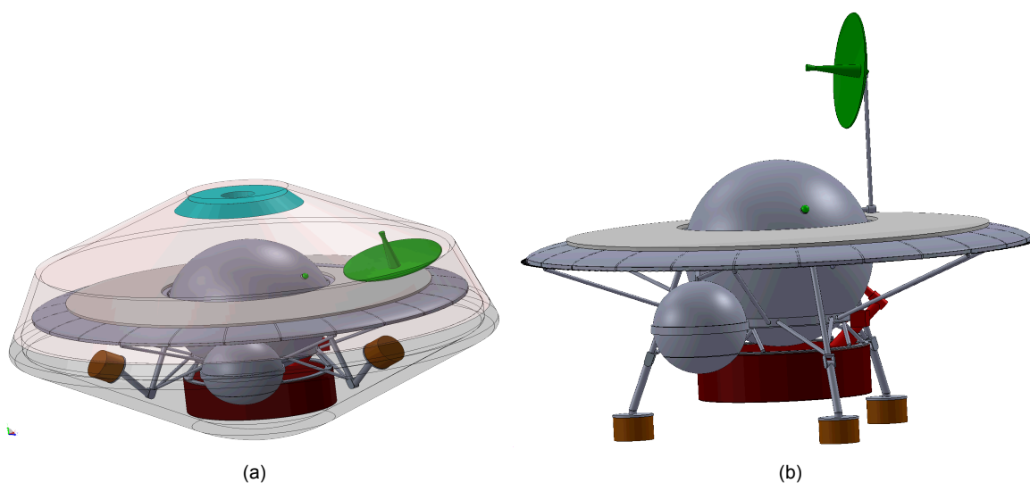
Figure 5.15—(a) The Lander stowed within the heat shield/backshell assembly and (b) the Lander fully deployed.
