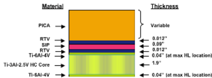
Figure 5.22—Orion heat shield structural makeup.
