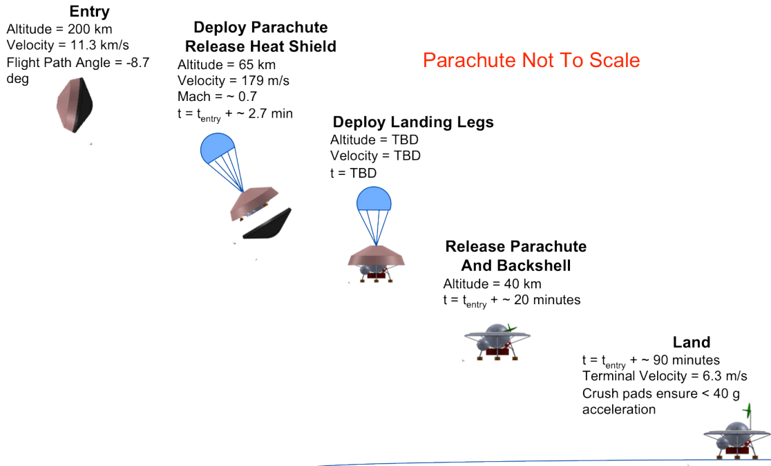
Figure 5.6—Summary of nominal EDL profile.
