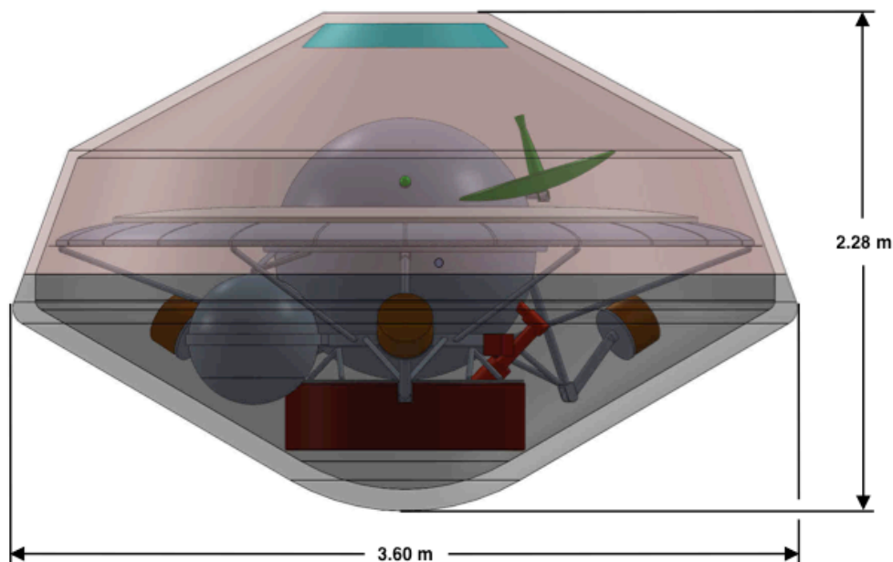
Figure 2.17—ALIVE Lander aeroshell dimensions.
