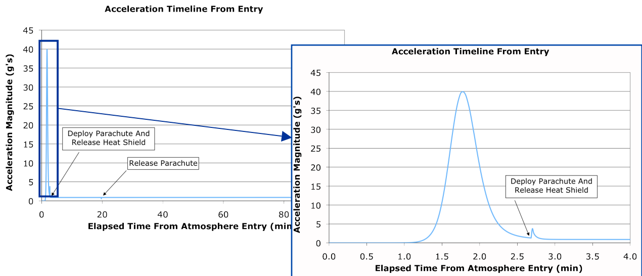
Figure 5.7—Acceleration timeline from atmospheric entry.
