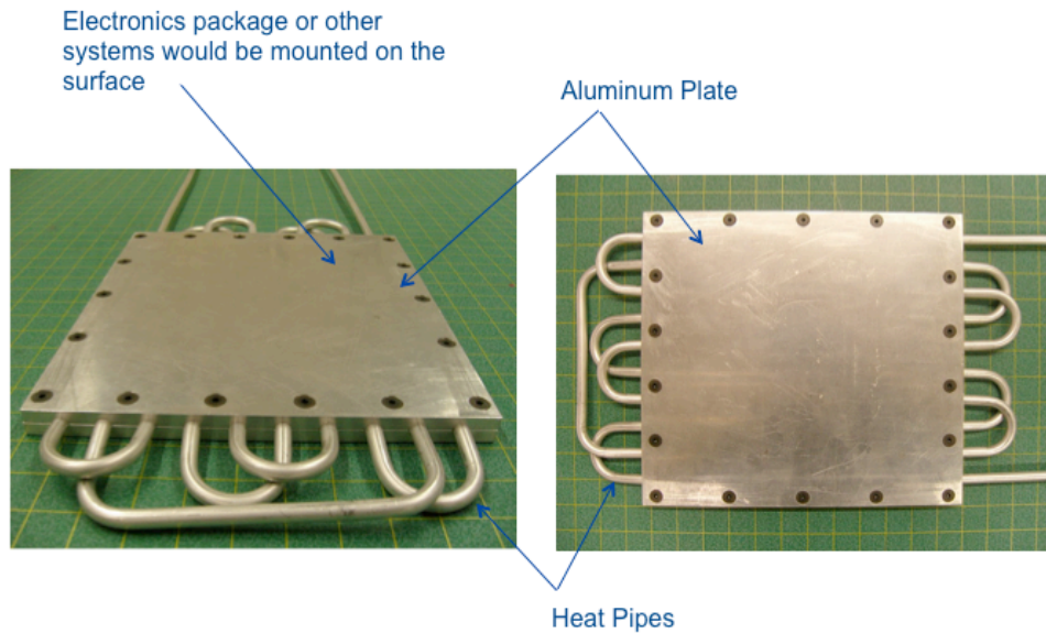
Figure 5.18—Example of a cold plate with integrated heat pipes.
