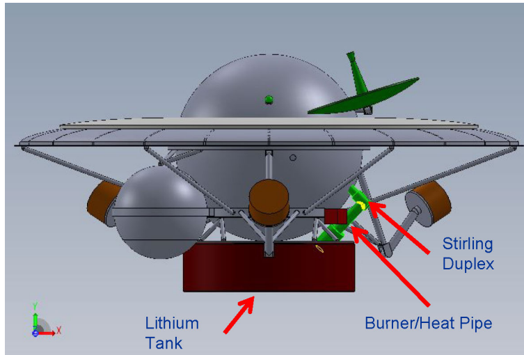
Figure 5.12—ALIVE Power/Cooling System highlights.
