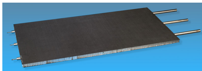
Figure 5.19—Radiator with integral heat pipes (ACT, inc).
