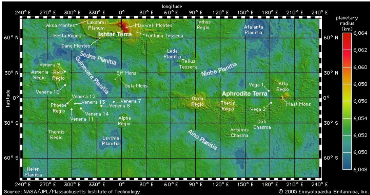
Figure 2.3—Cartesian Map of Ovda Regio.
