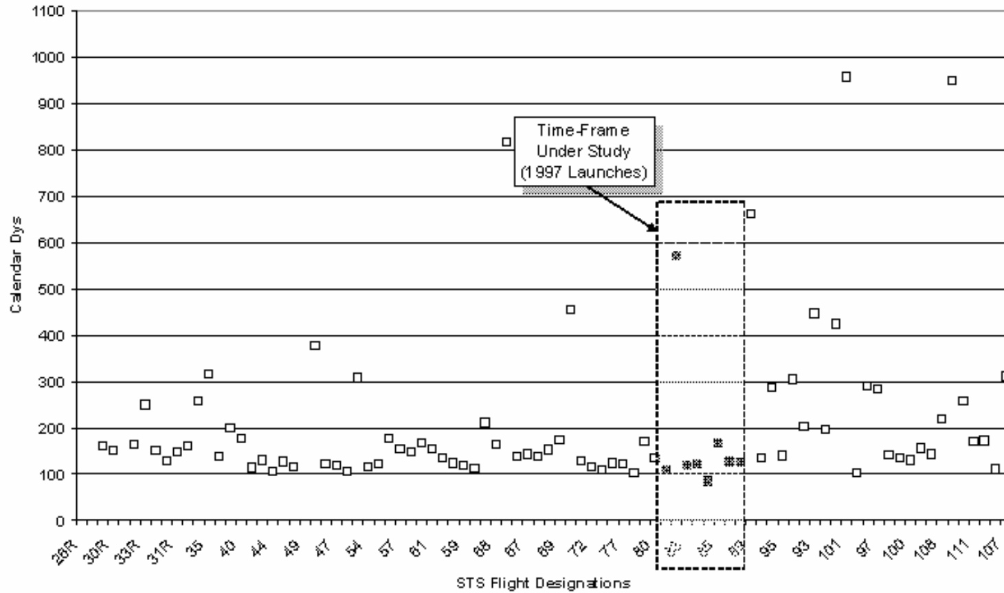
Figure 18. Shuttle Processing Intervals—From Orbiter Landing to Next Launch
