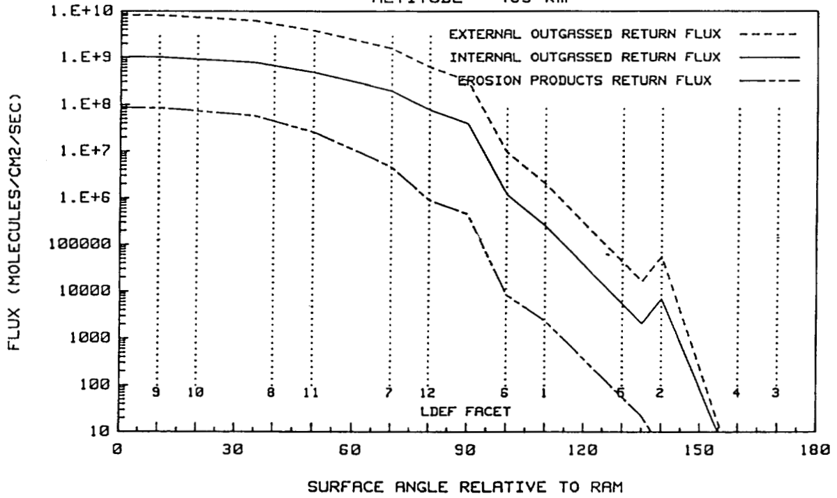
OUTGAS AND EROSION PRODUCT FLUX ON LDEF SURFACES AS A FUNCTION OF ANGLE ALTITUDE = 463 km
