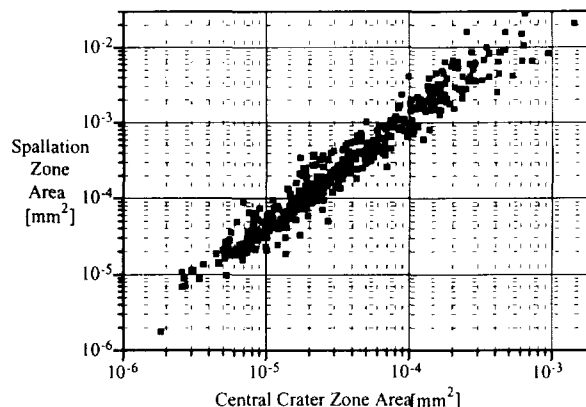
Figure 13. Relationship between central crater and damaged (spalled) area
