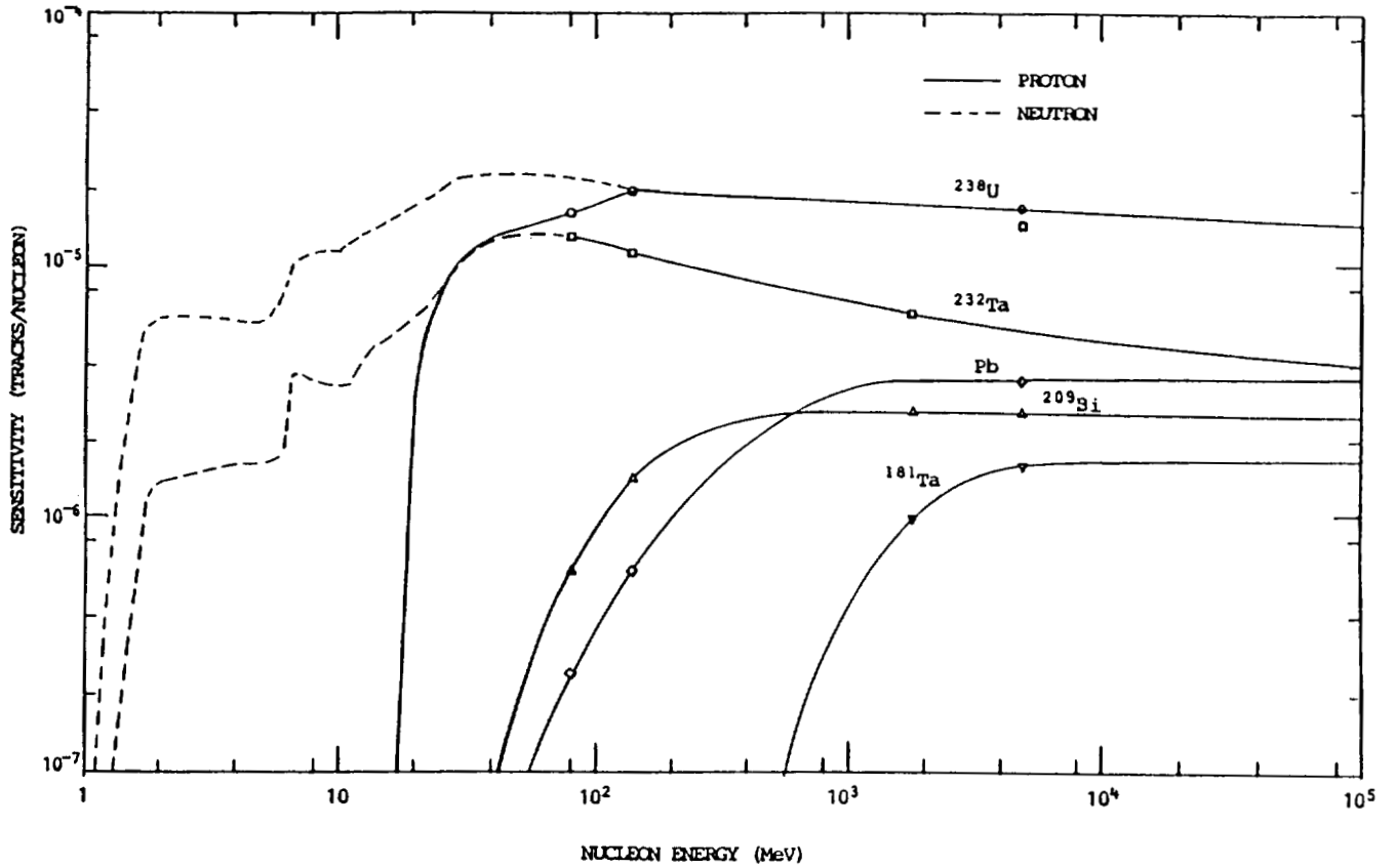
Figure 2: Sensitivities of fission foil detectors to neutrons and protons.
