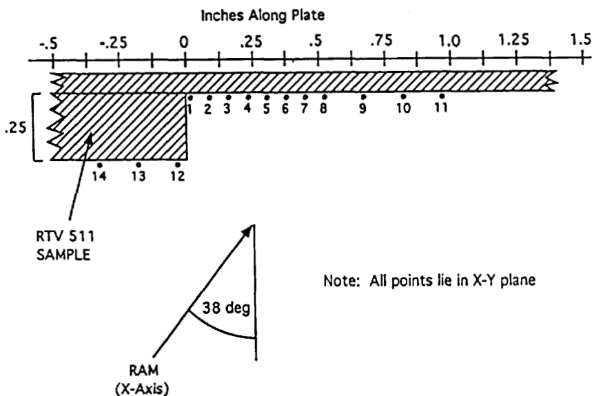
Figure 9. Micro Model Flux Computation Points
