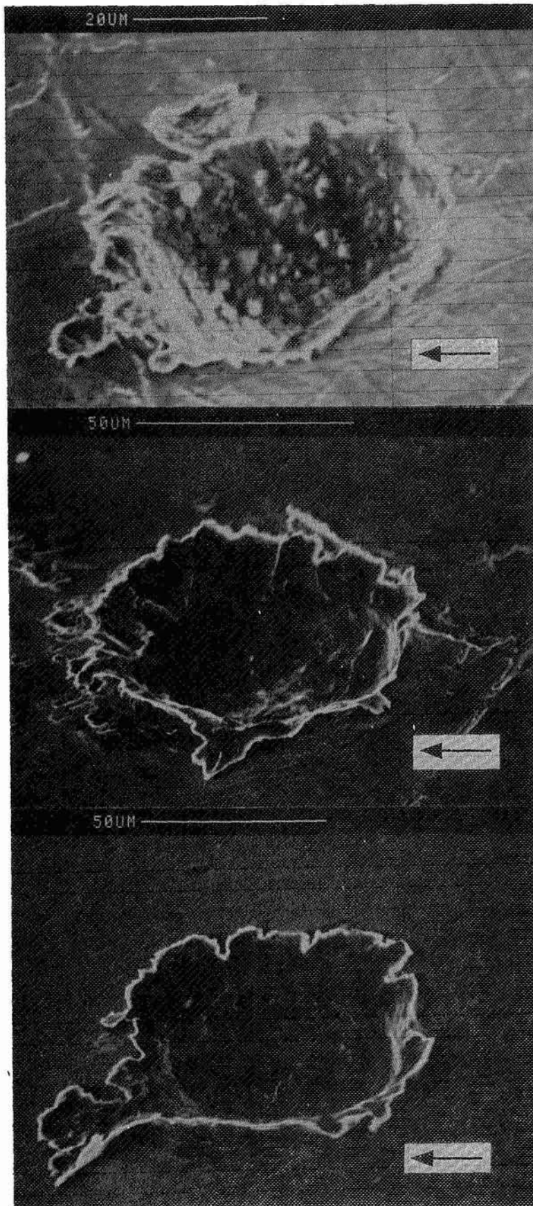
Figure 8. Photomicrograph of impact site D78-03-17. Impact velocity was 10.5 \text{ km}\cdot\text{s}^{-1} and angle of incidence is 60^\circ (w.r.t. surface normal). Impact direction is indicated by the arrow. Note the granular residue and pronounced trailing edge lips. p/D ratio is 0.40.
