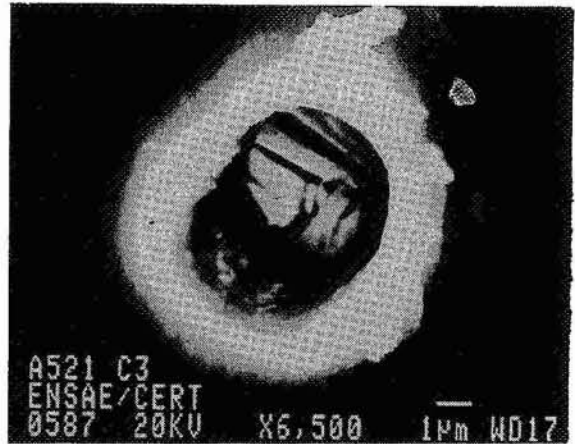
Figure a: Oblique impact (6.6 x 5.4 μm) on 99% pure Al experiment surface.
