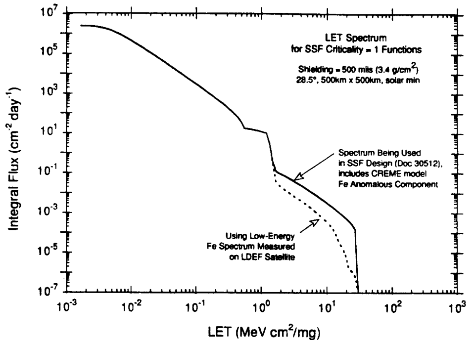
Figure 10. Comparison of Space Station Freedom Requirement document SSP 30512 (ref. 19) spectra vs. LET and measured results from the HIIS experiment on LDEF from (ref. 16).
