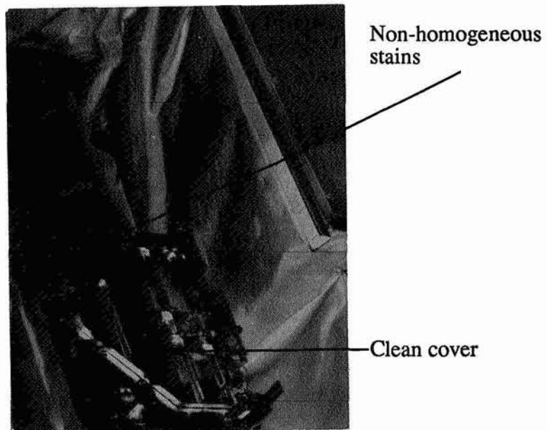
PHOTOGRAPH N° 6. View of SOVA experiment. Notice the non-homogeneous stains on the aluminised FEP tape due to temperature gradients on the surface at perforations and tape joints. (NASA photo)
