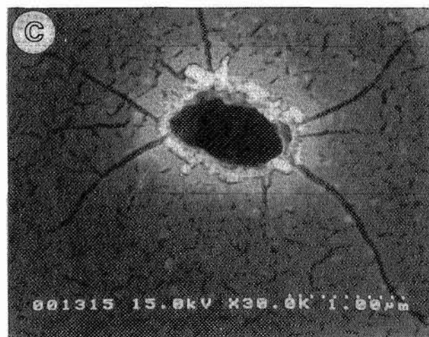
Fig. 10. SEM images of ZnS formed craters in glass: (a) 4.6 km sec -1 crater. Impactor apparently separated into 3 fragments at impact. Impactor size was 0.0089 mm. (b) 6.4 km sec -1 crater. Cracked surface is due to breakup of Au coating with time. Impactor dia. was 0.001 mm. (c) 10.1 km sec -1 crater. Impactor dia. was 0.00066 mm. All crater outlines depart from circularity. All launches were 90° to the target and all rims contain detectable Zn.
