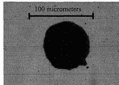
Figure 11. Perforation of witness foil used in the impact detector (revealing a particle diameter 74 \mu\text{m} )
