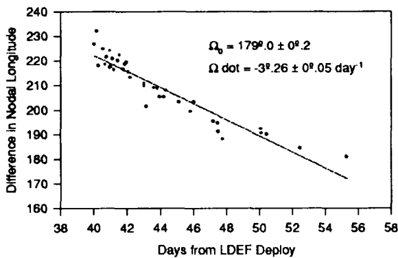
Figure 4: Linear fit to determine nodal line properties
