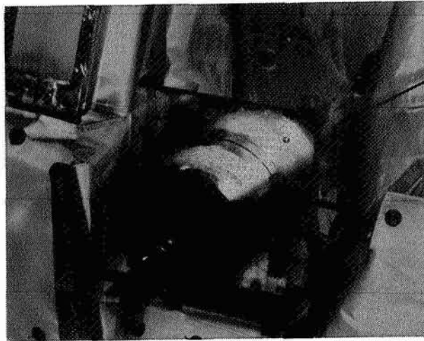
PHOTOGRAPH N° 9. View of RITA. Notice gap behind back plate which provides a chimney for outgassed materials to vent from within the spacecraft. (NASA photo)
