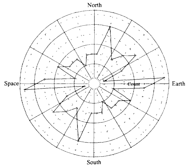
Figure 15. Distribution of direction of major axis ellipse fits for craters with a b/a ratio smaller than 0.7. Coordinate system as if looking from ram direction on bay E08.
