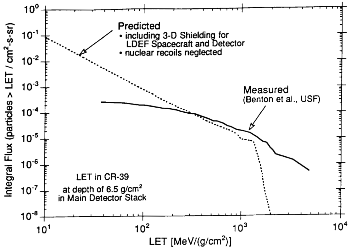
Fig. 4. Predicted LET using 3-D shielding model.
