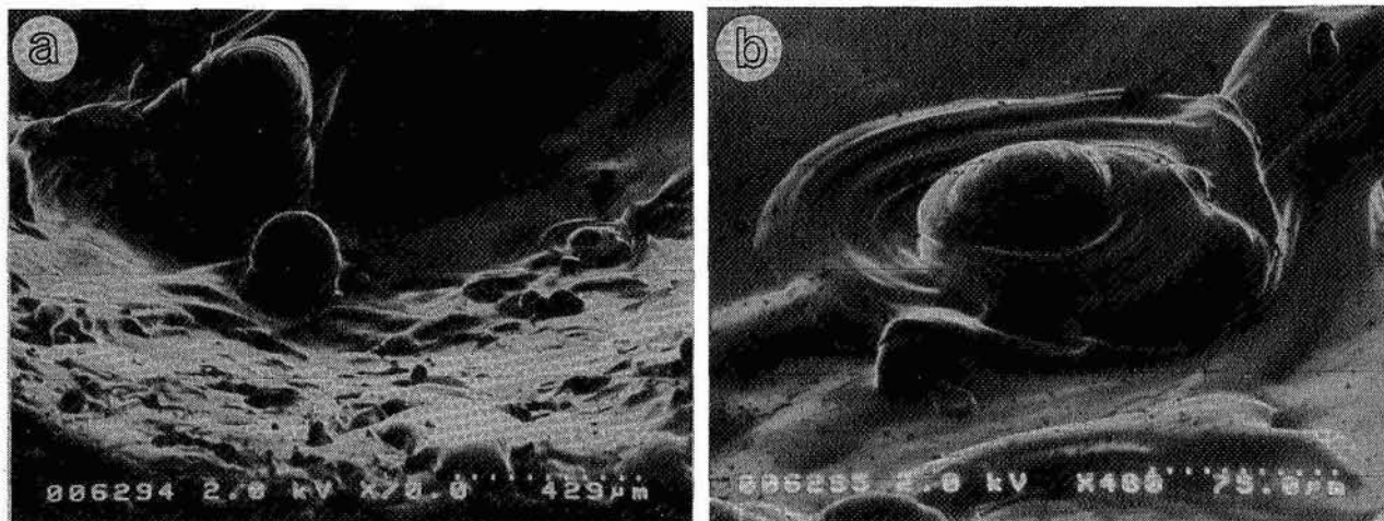
Figure 3. FESEM images. (a) Open arrow points to domed object with prominent rings/layers. Solid arrow indicates a melt droplet that collapsed into a "puddle" before solidifying. (b) Enlarged view of collapsed droplet.
