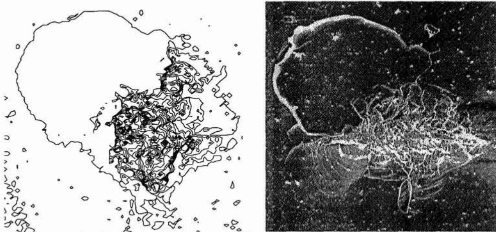
Figures 19 and 20. Hypervelocity impact into germanium at an impact angle of 70^\circ . Velocity and particle size for this particular impact were not measured. Note the ejecta spray on the right side
