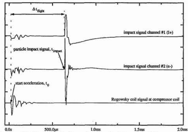
Figure 10. Impact signal of a 7.4 km/s, 54 \mu\text{m} diameter particle
