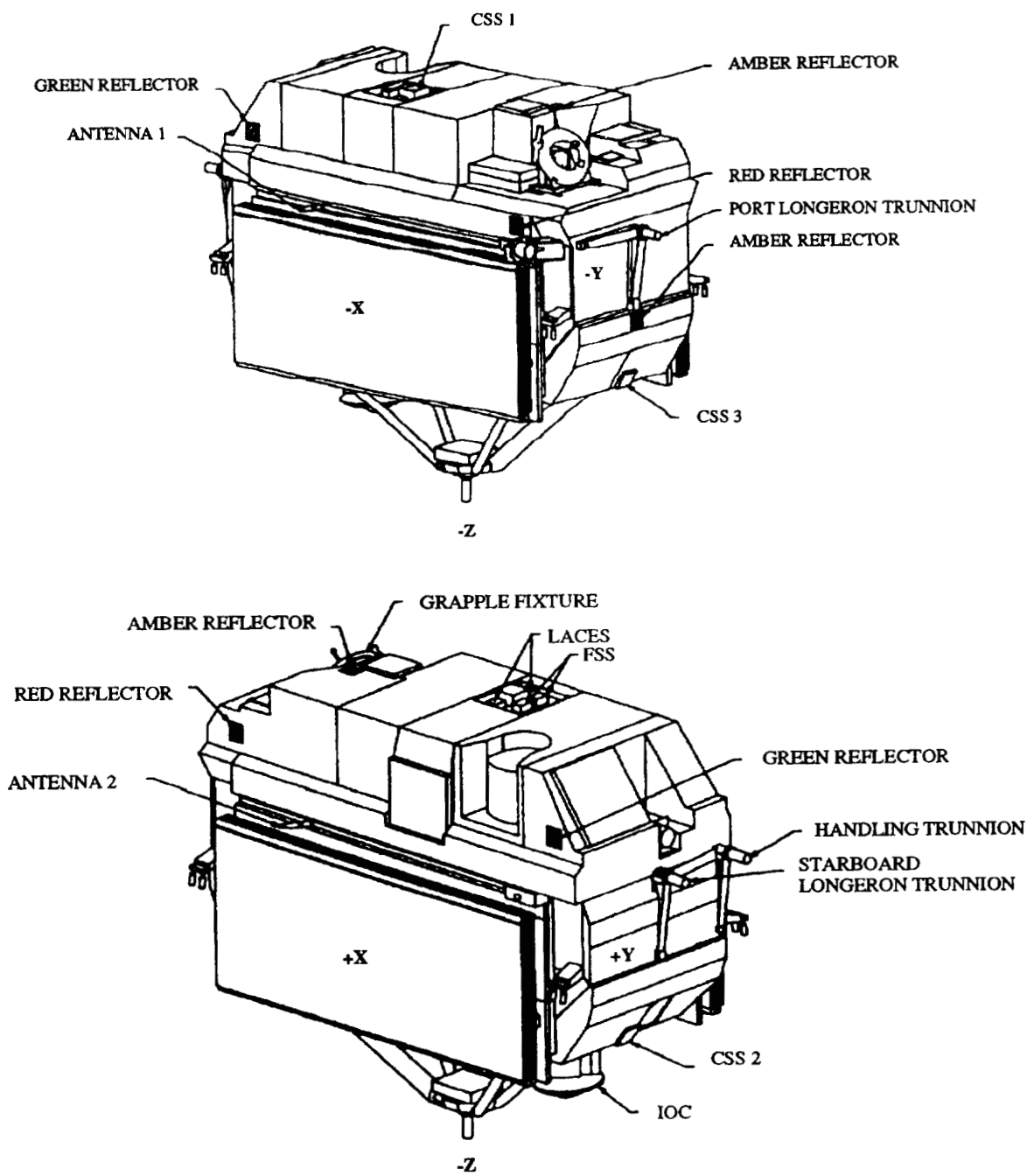
Fig. 1. Schematic view of EURECA
