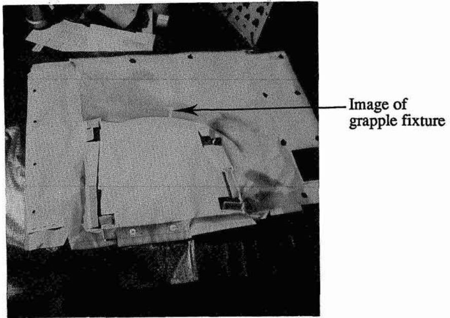
PHOTOGRAPH N° 5. View of UV degradation and outgassed material deposited and polymerised on the MLI surrounding the grapple fixture. Notice the image caused by the shadow of the grapple on the MLI. (DASA ERNO photo)
