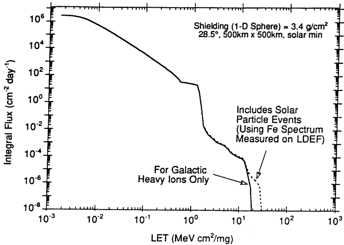
Fig. 6. Influence of SEP iron ions on LET.
