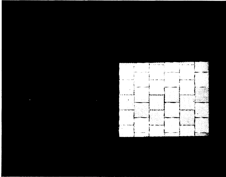
Figure 5. Photograph of uncoated (dark image on the left) and approximately 1000Å thick 8% fluoropolymer-filled SiO x coated (bright image on the right) EURECA retroreflector samples after exposure to a Kapton effective atomic oxygen fluence of 3 \times 10^{20} atoms/cm 2 .
