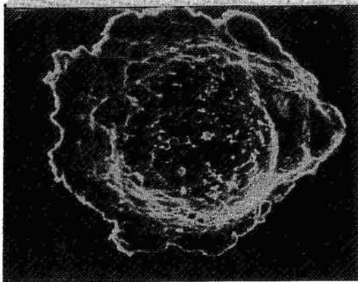
Figure a: Oblique impact (235 x 176 μm) on Al alloy experiment support surface.
