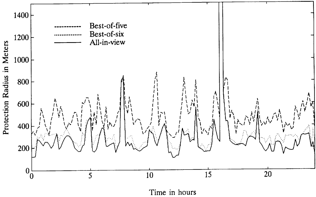
Figure 4. Worst Case Protection Radius (36N 140E)
