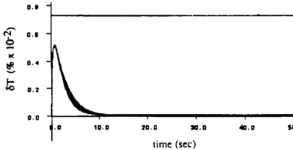
b) 15 fps velocity command: thrust response
