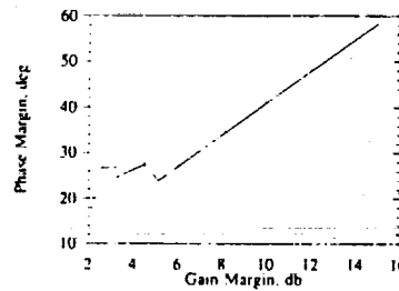
Fig. 1 Nominal gain and phase relationships of the 10 controllers.
