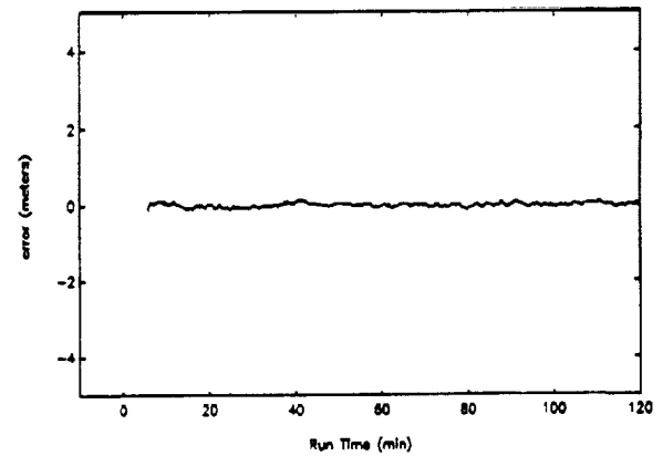
Figure 19. SV23: P-code
