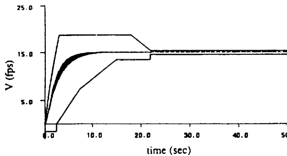
a) 15 fps velocity command: velocity response
