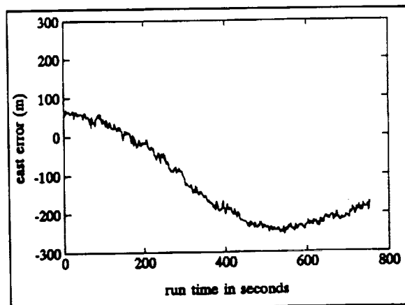
Figure 9. Loran-C position error.
