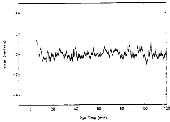
Figure 14. SV17: C/A-code
