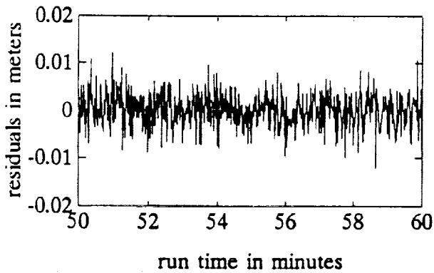
Figure 17. SV 28 residuals
