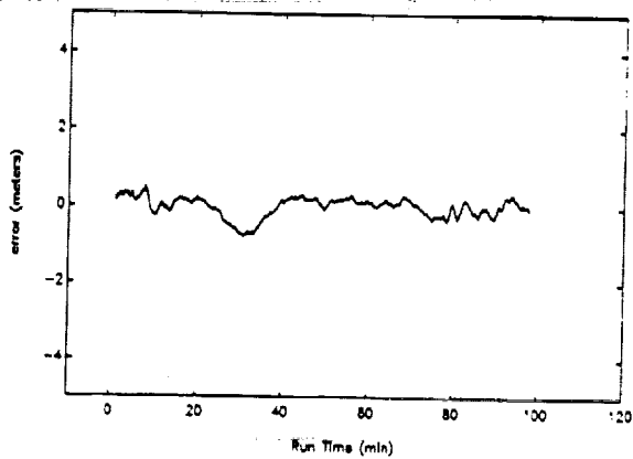
Figure 10. SV23: P-code
