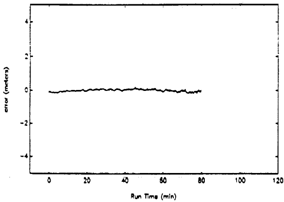
Figure 21. SV3:P-code
