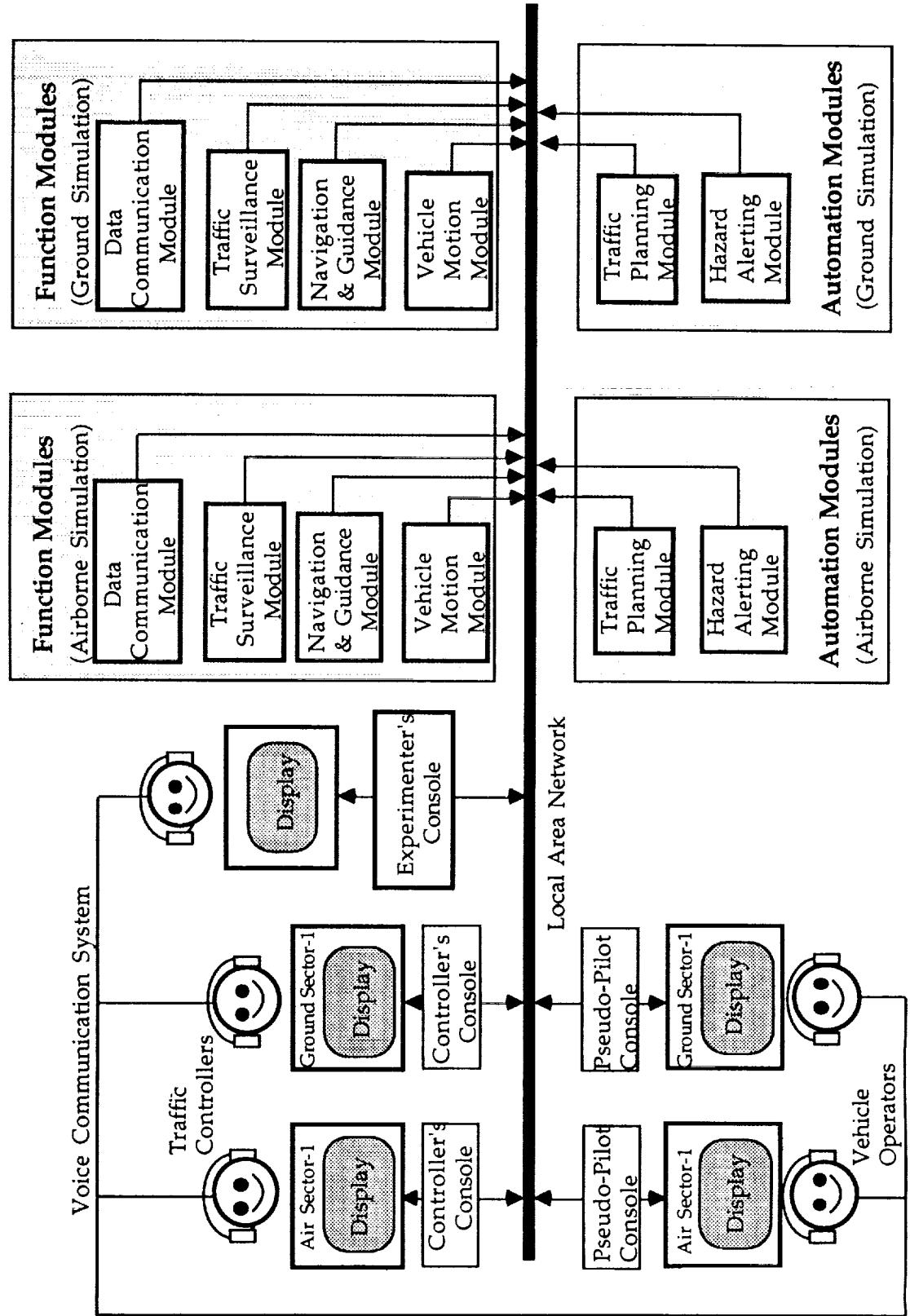
Figure 1 - ATCSIM FUNCTIONALITIES
