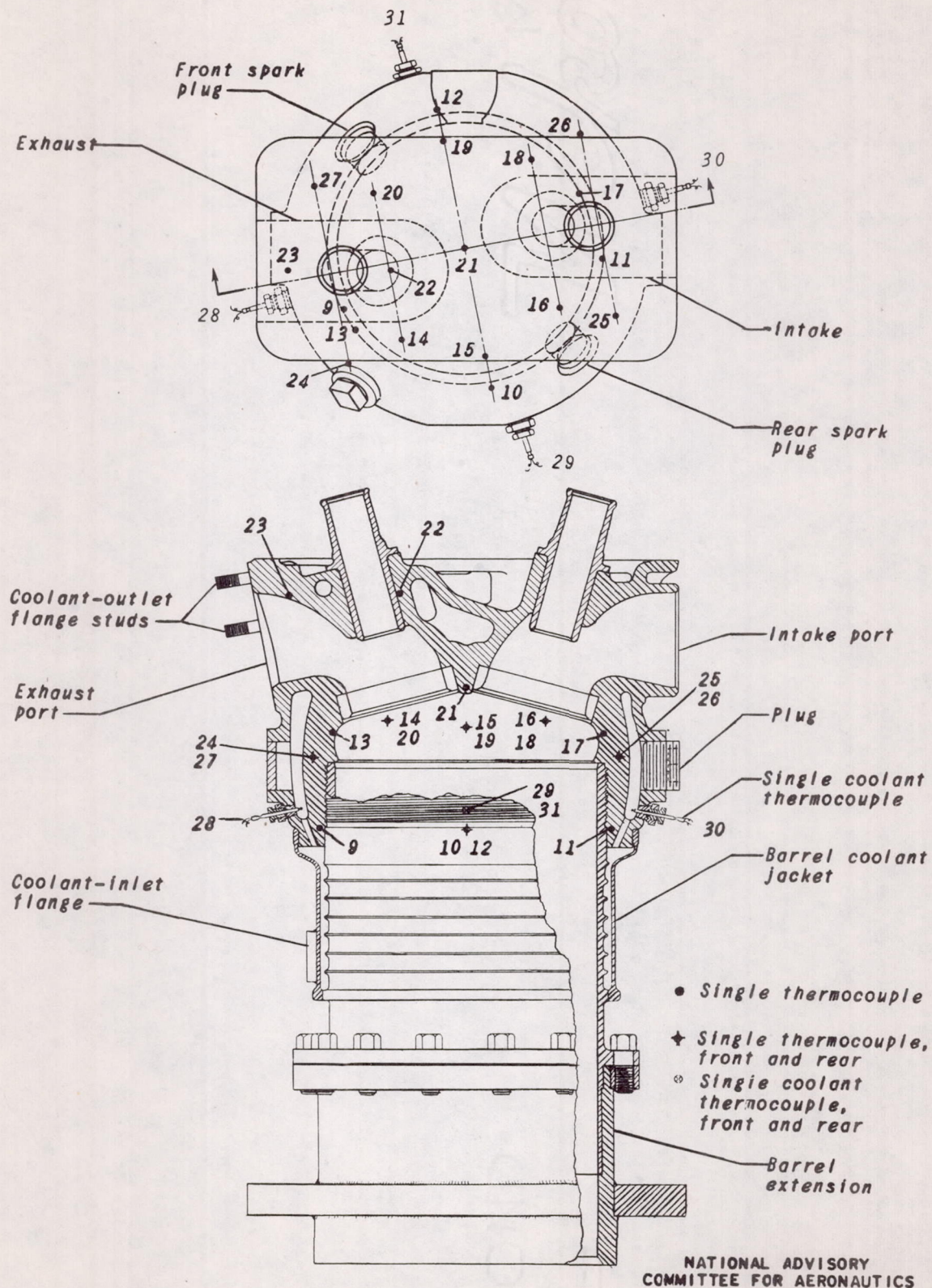
Figure 4. - Thermocouple installation of cylinder B.
