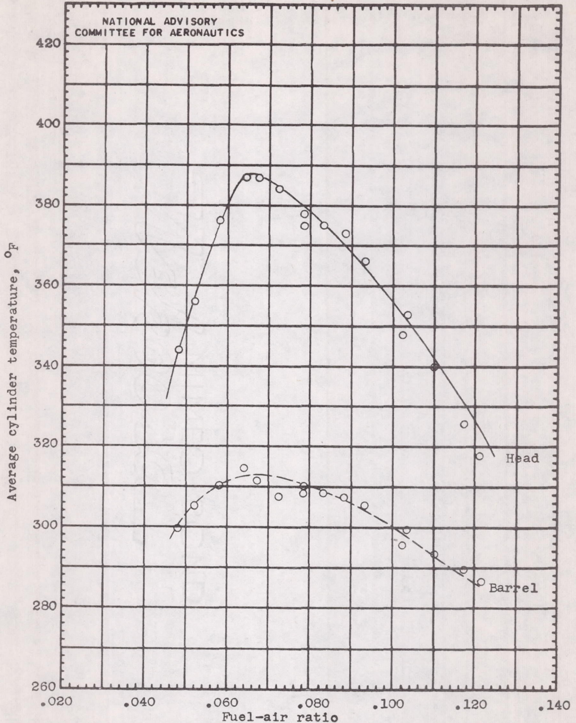
Figure 13.- Effect of fuel-air ratio on average head and barrel temperatures. Cylinder A; coolant, AN-E-2 ethylene glycol; average coolant temperature: head, 249° F, barrel, 247° F; coolant-flow rate: head, 73 pounds per minute, barrel, 30 pounds per minute; coolant pressure, 19 pounds per square inch absolute; engine speed, 2000 rpm; indicated horsepower, 43 to 54; charge-flow rate, 5.3 to 5.5 pounds per minute; spark advance, 28° B.T.C.; carburetor-air temperature, 80° F; runs, 95 to 110.
