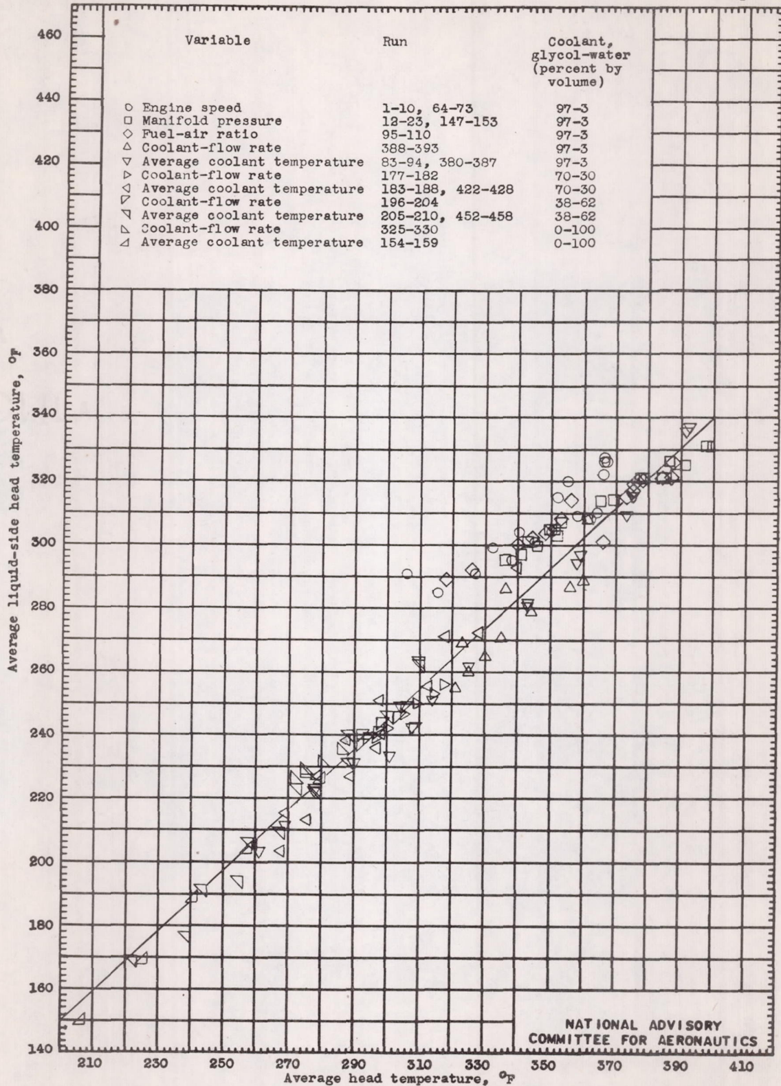
Figure 27.- Relation between average liquid-side head and average head temperatures under various operating conditions, cylinder A.
