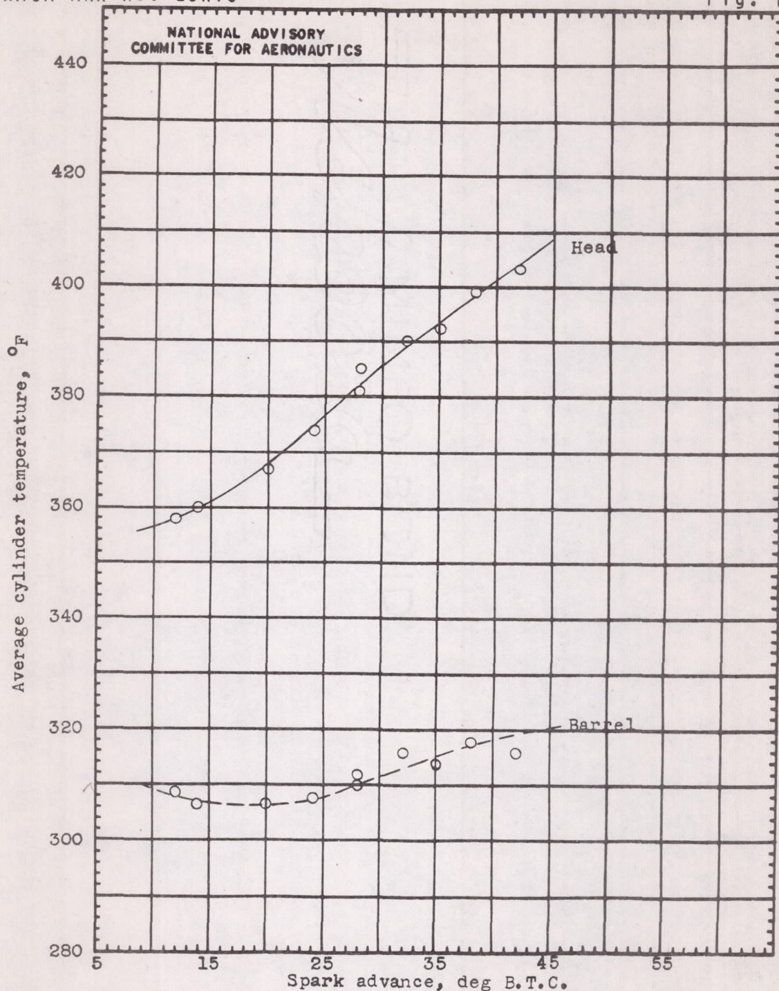
Figure 15. - Effect of spark advance on average head and barrel temperatures. Cylinder A; coolant, AN-E-2 ethylene glycol; average coolant temperature: head, 249° F, barrel, 247° F; coolant-flow rate: head, 72 pounds per minute, barrel, 30 pounds per minute; coolant pressure, 19 pounds per square inch absolute; engine speed, 2000 rpm; indicated horsepower, 48 to 55; charge-flow rate, 5.4 pounds per minute; fuel-air ratio, 0.077; carburetor-air temperature, 83° F; runs, 118 to 127.
