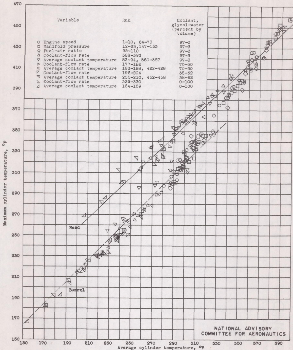
Figure 23.- Relation between maximum and average cylinder temperatures under various operating conditions, cylinder A.
