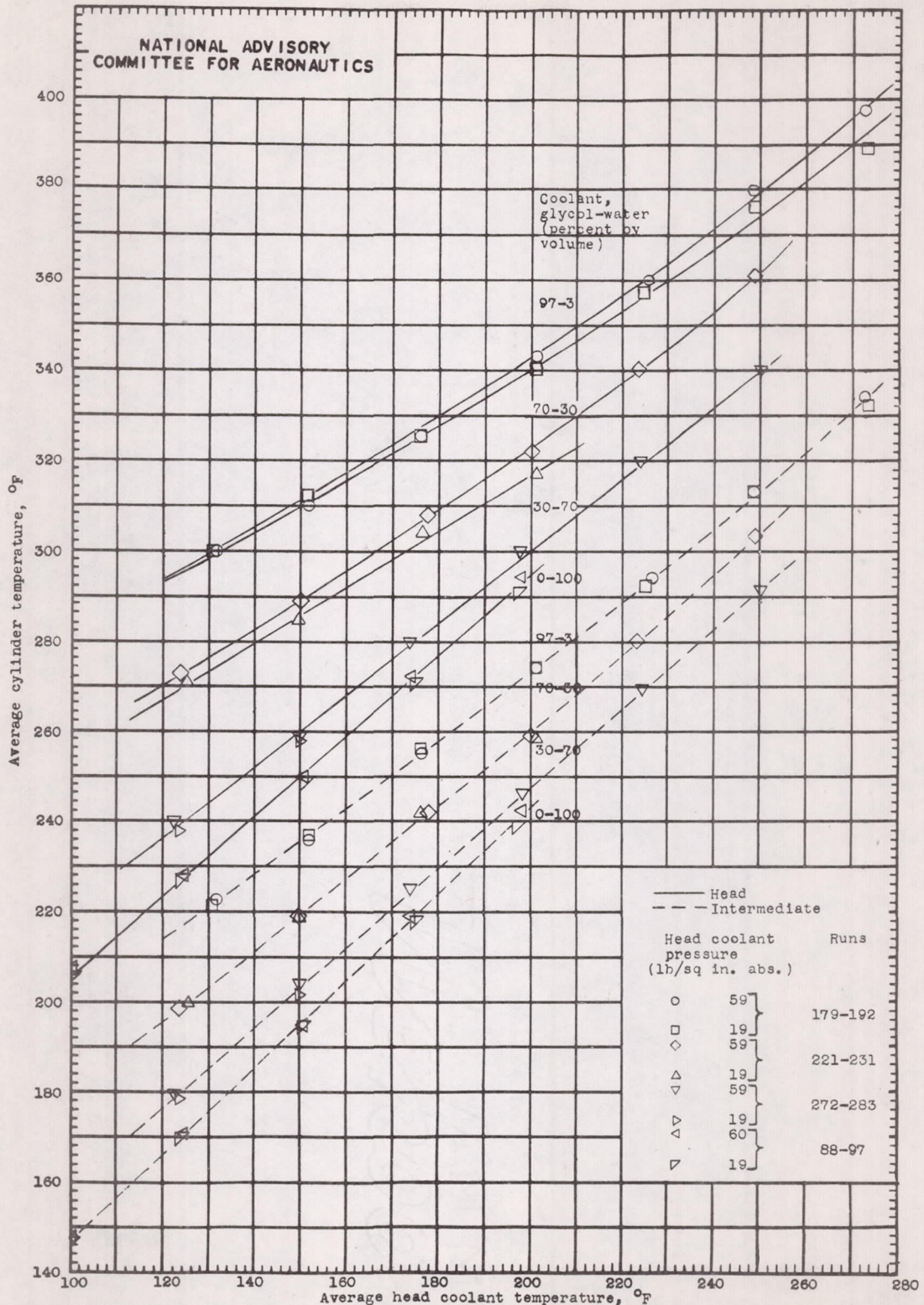
Figure 19.- Effect of average coolant temperature on average head and intermediate temperatures using various glycol-water solutions at a coolant-flow rate of approximately 70 pounds per minute. Cylinder B; engine speed, 2000 rpm; indicated horsepower, 56; charge-flow rate, 5.6 pounds per minute; fuel-air ratio, 0.079; spark advance, 28° B.T.C.; carburetor-air temperature, 75° F.
