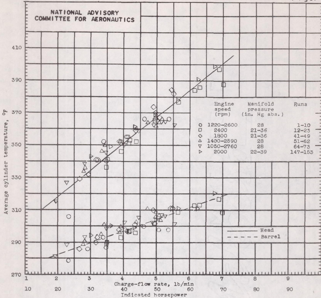
Figure 8.- Effect of charge-flow rate and indicated horsepower on average head and barrel temperatures. Cylinder A; coolant, AN-E-2 ethylene glycol; average coolant temperature, 247° F; coolant-flow rate; head, 73 pounds per minute; barrel, 30 pounds per minute; barrel pressure, 19 pounds per square inch absolute; fuel-air ratio, 0.075; spark advance, 28° B.T.C.; carburetor-air temperature, 80° F.
