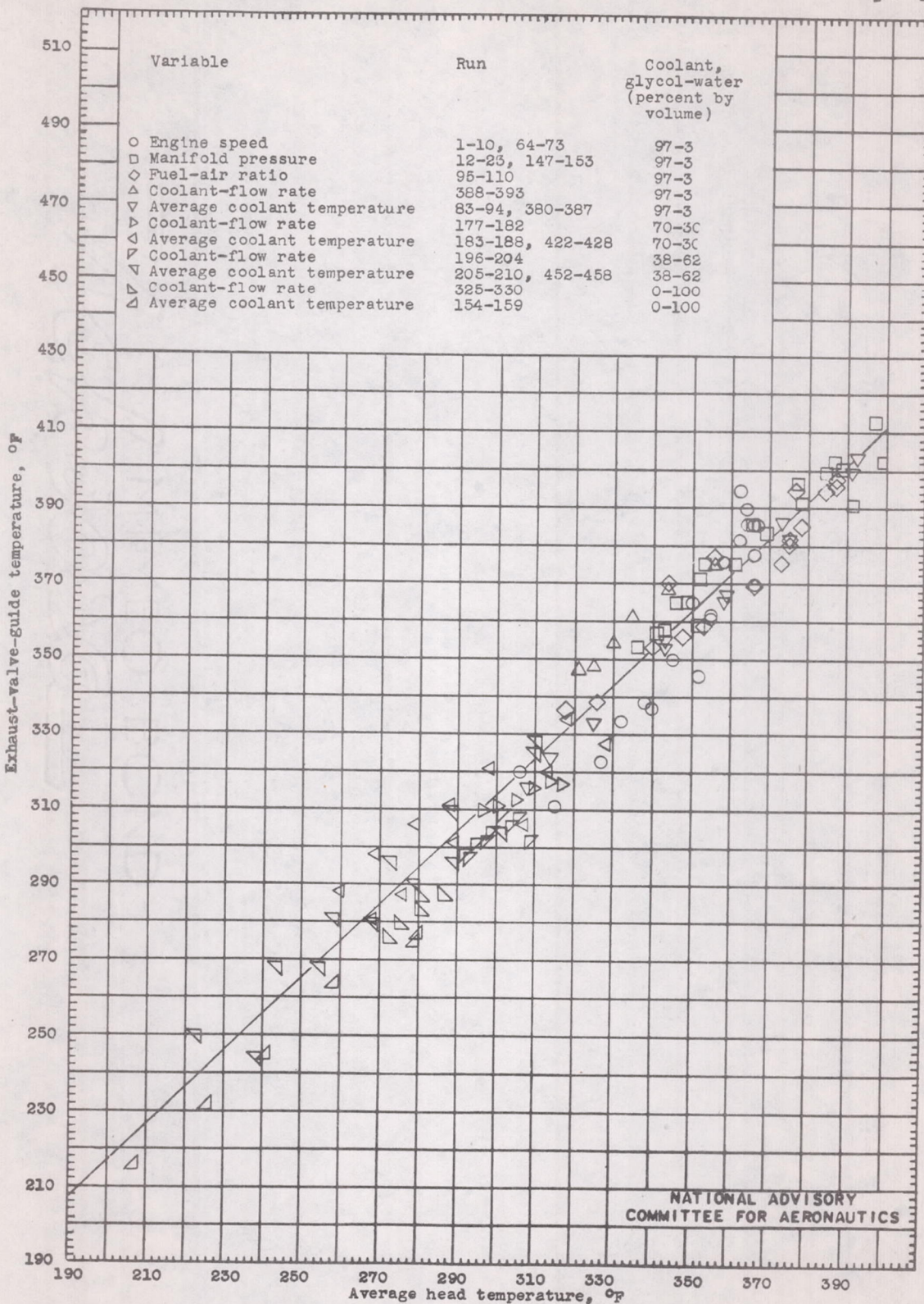
Figure 25.- Relation between exhaust-valve-guide and average head temperatures under various operating conditions, cylinder A.
