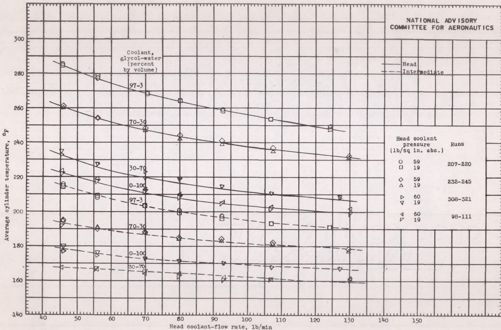
Figure 17.- Effect of coolant-flow rate on average head and intermediate temperatures using various glycol-water solutions. Cylinder B; average coolant temperature, 125° F; engine speed, 1800 rpm; indicated horsepower, 47; charge-flow rate, 4.6 pounds per minute; fuel-air ratio, 0.079; spark advance, 28° B.T.C.; carburetor-air temperature, 75° F.
