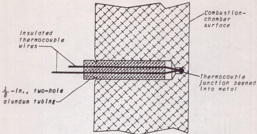
(a) Gas-side head thermocouple in solid portions of cylinder head.
