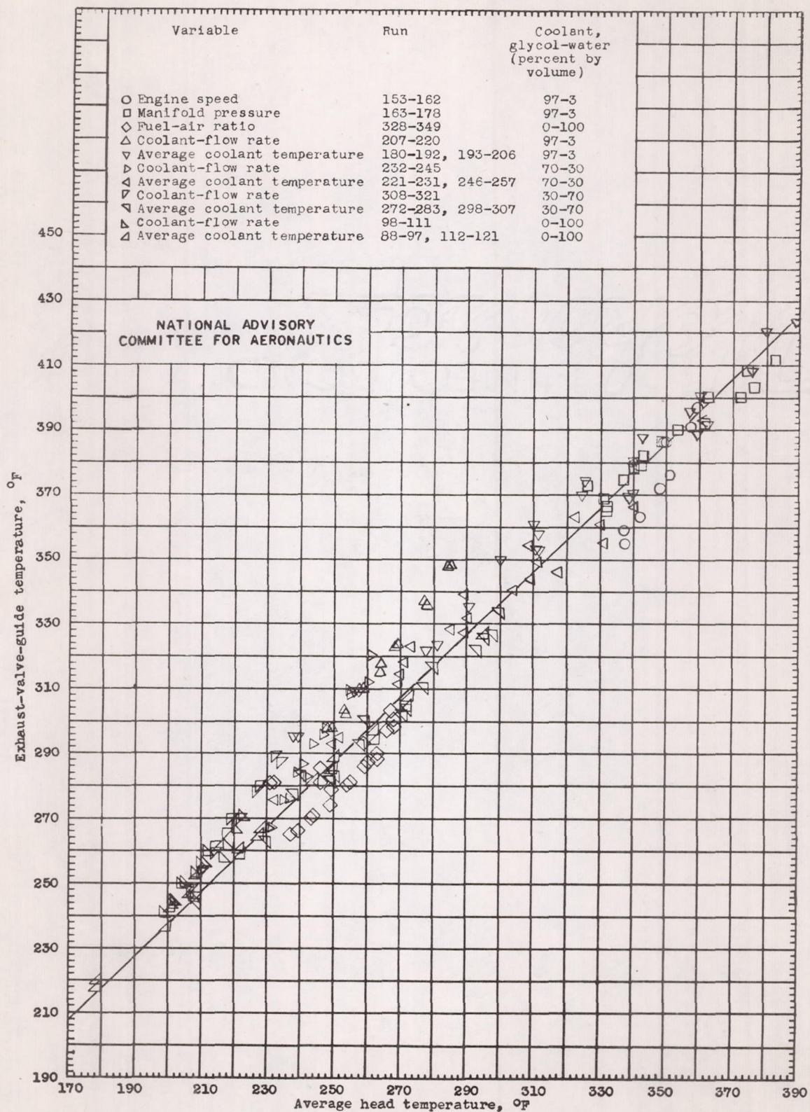
Figure 26.- Relation between exhaust-valve-guide and average head temperatures under various operating conditions, cylinder B.
