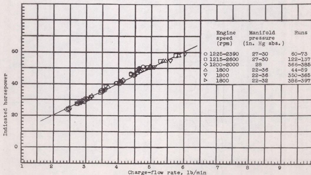
Figure 11.- Relation of indicated horsepower to charge-flow rate, cylinder B.
