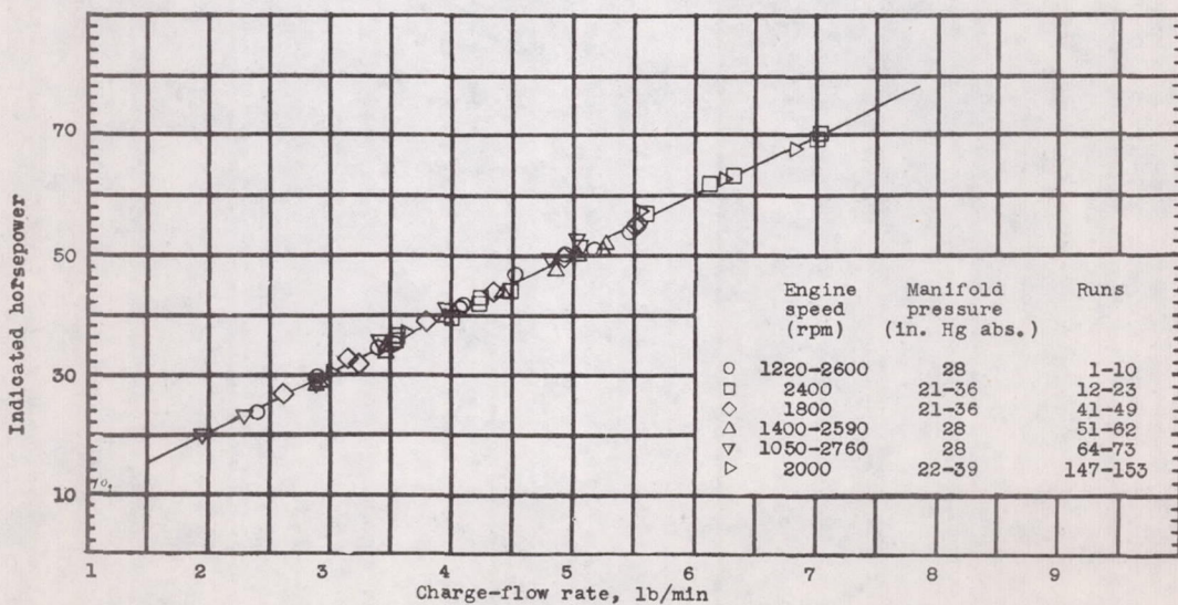
Figure 9.- Relation of indicated horsepower to charge-flow rate, cylinder A.
