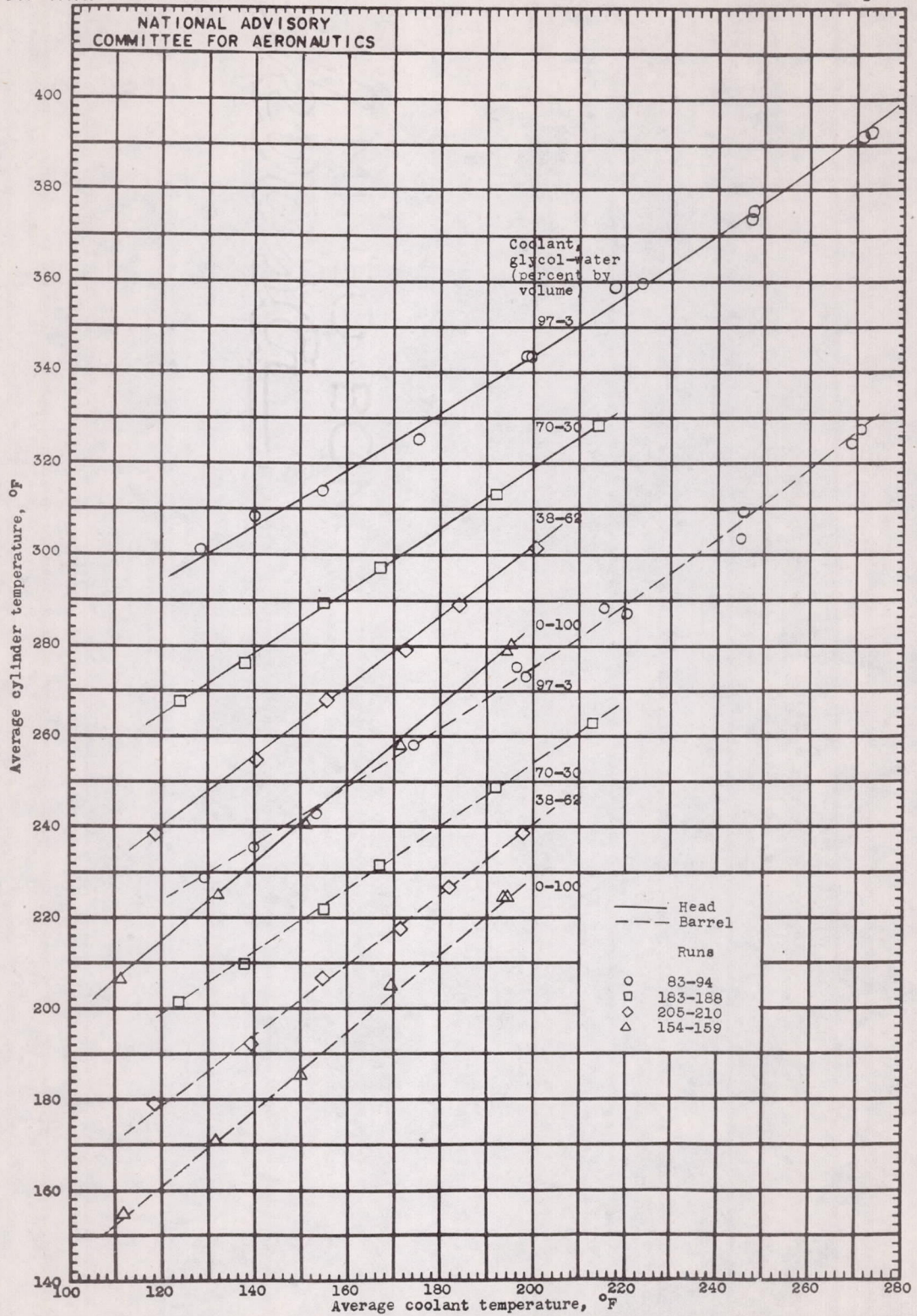
Figure 18.- Effect of average coolant temperature on average head and barrel temperatures using various glycol-water solutions at a head coolant-flow rate of approximately 70 pounds per minute and a barrel coolant-flow rate of 30 pounds per minute. Cylinder A; coolant pressure, 19 pounds per square inch absolute; engine speed, 2000 rpm; indicated horsepower, 55; charge-flow rate, 5.4 pounds per minute; fuel-air ratio, 0.078; spark advance, 28° B.T.C.; carburetor-air temperature, 81° F.
