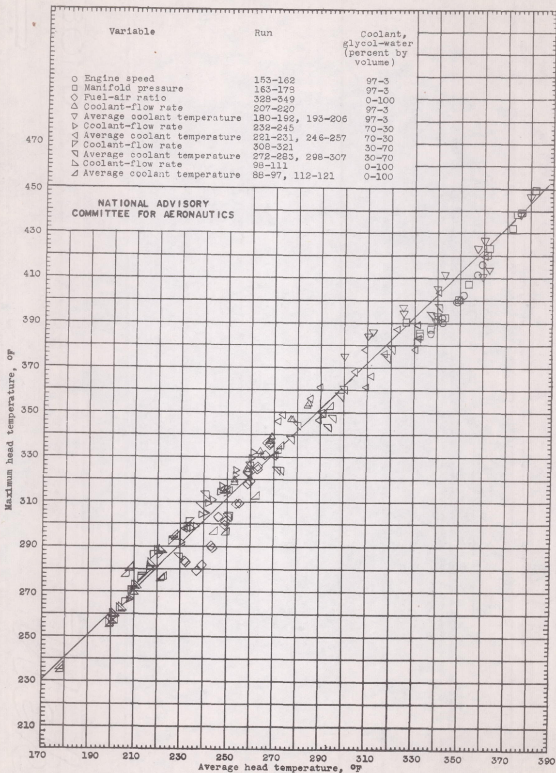
Figure 24.- Relation between maximum and average head temperatures under various operating conditions, cylinder B.
