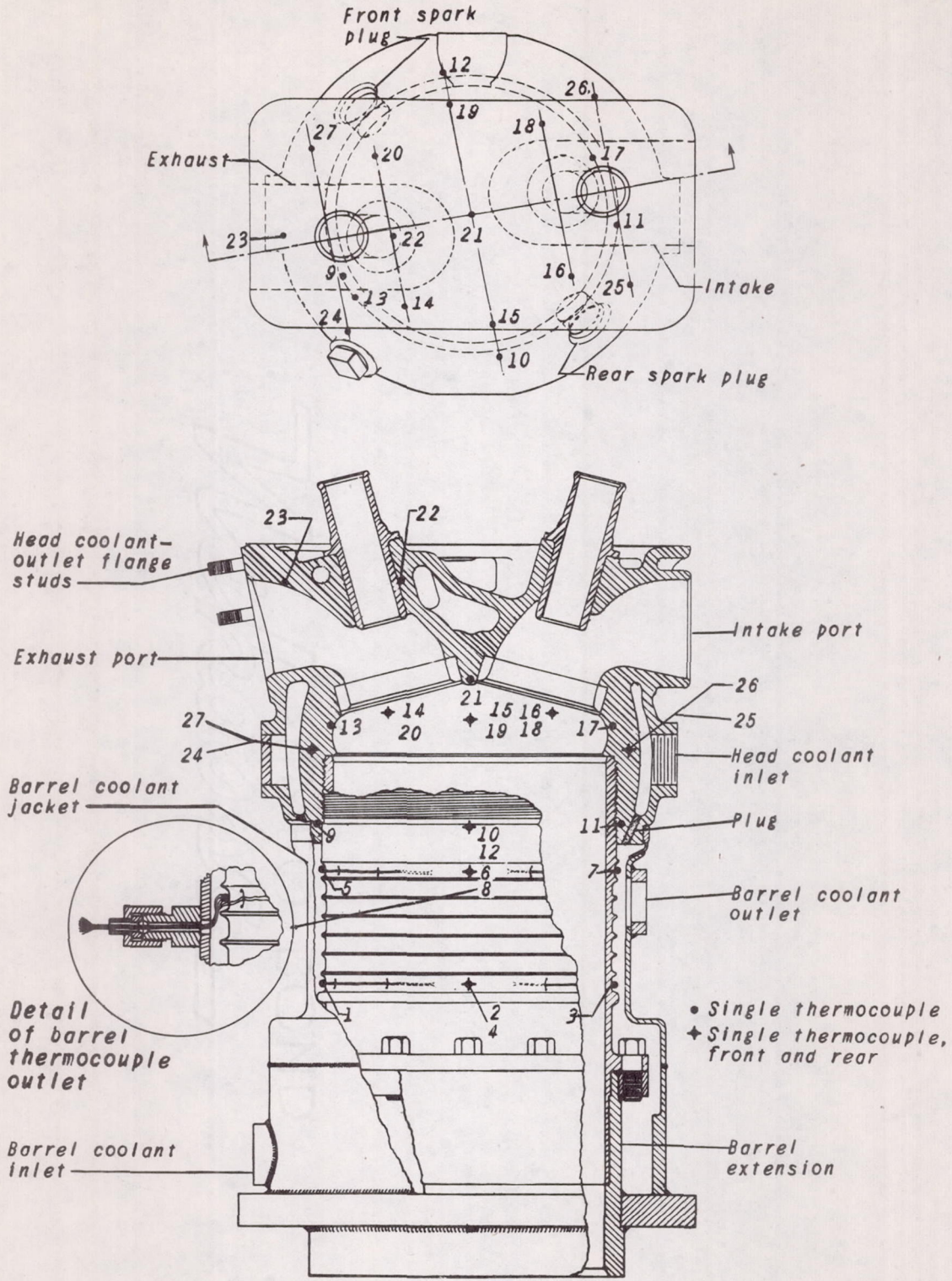
Figure 2. - Thermocouple installation and modifications of cylinder A.
