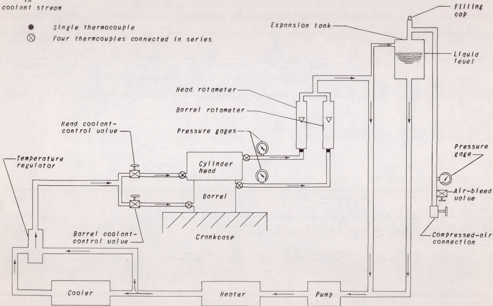
Figure 5. - Schematic diagram of cooling system, cylinder A.
