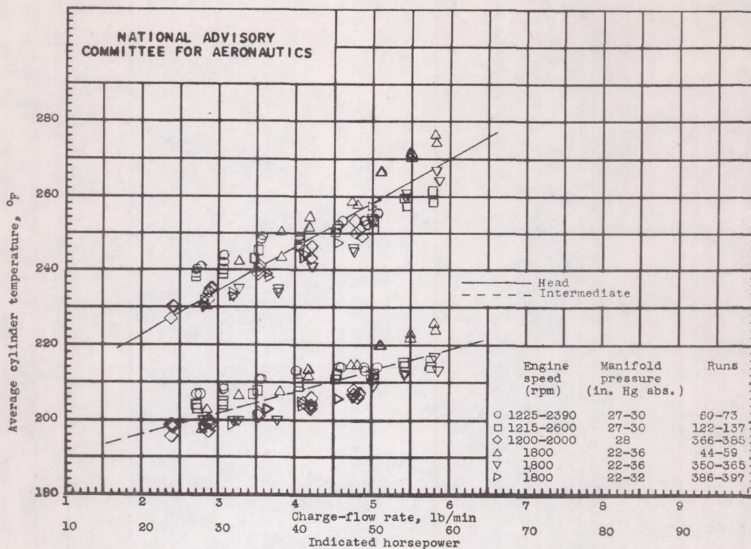
Figure 10.- Effect of charge-flow rate and indicated horsepower on average head and intermediate temperatures. Cylinder B; coolant, water; average coolant temperature, 173° F; coolant-flow rate, 70 pounds per minute; coolant pressure, 15 and 59 pounds per square inch absolute; fuel-air ratio, 0.079; spark advance, 28° B.T.C.; carburetor-air temperature, 76° F.
