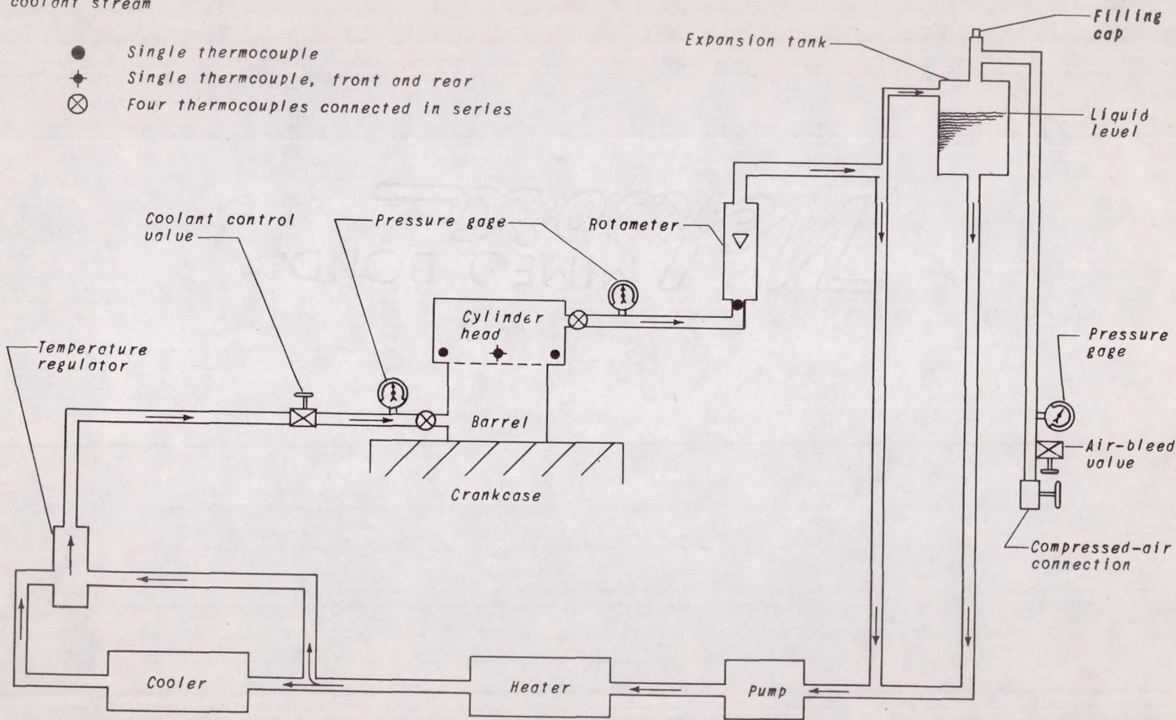
Figure 6. - Schematic diagram of cooling system, cylinder B.
