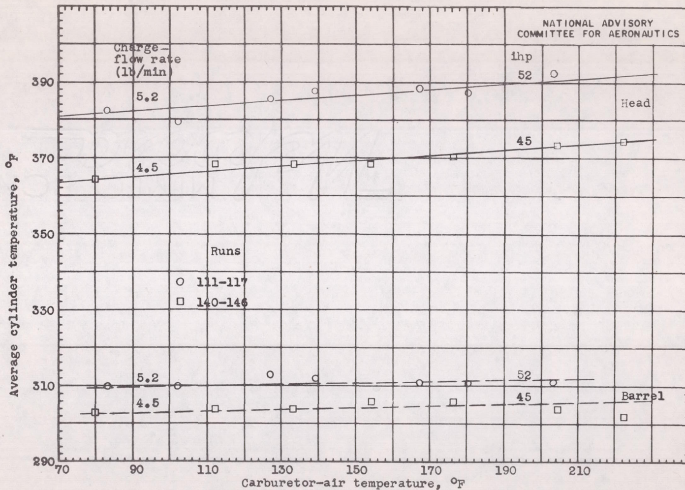
Figure 12.- Effect of carburetor-air temperature on average head and barrel temperatures. Cylinder A; coolant, AN-E-2 ethylene glycol; average coolant temperature: head, 249° F, barrel, 247° F; coolant-flow rate: head, 72 pounds per minute, barrel, 30 pounds per minute; coolant pressure, 19 pounds per square inch absolute; engine speed, 2000 rpm; fuel-air ratio, 0.077; spark advance, 28° B.T.C.
