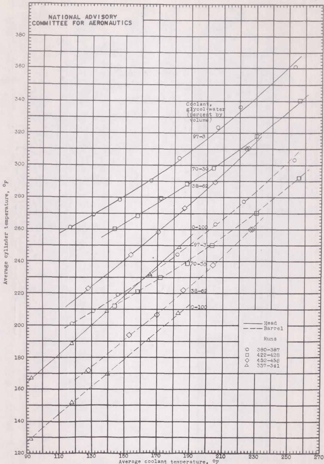
Figure 20.- Effect of average coolant temperature on average head and barrel temperatures using various glycol-water solutions at a head coolant-flow rate of approximately 125 pounds per minute and a barrel coolant-flow rate of 46 pounds per minute. Cylinder A; coolant pressure; head, 50 pounds per square inch absolute, barrel, 42 pounds per square inch absolute; engine speed, 1800 rpm; indicated horsepower, 48; charge-flow rate, 4.6 pounds per minute; fuel-air ratio, 0.078; spark advance, 28° B.T.C.; carburetor-air temperature, 86° F.
