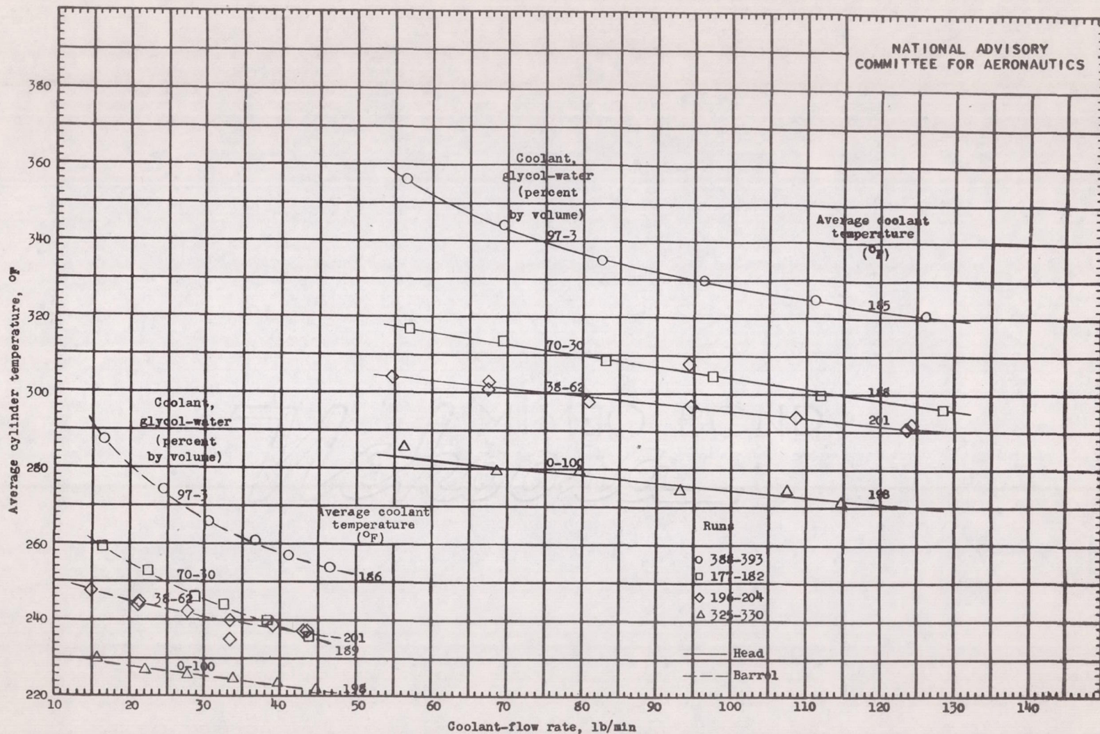
Figure 16.- Effect of coolant-flow rate on average head and barrel temperatures using various glycol-water solutions. Cylinder A; coolant pressure, 19 pounds per square inch absolute; engine speed, 2000 rpm; indicated horsepower, 55; charge-flow rate, 5.5 pounds per minute; fuel-air ratio, 0.078; spark advance, 28° B.T.C.; carburetor-air temperature, 84° F.
