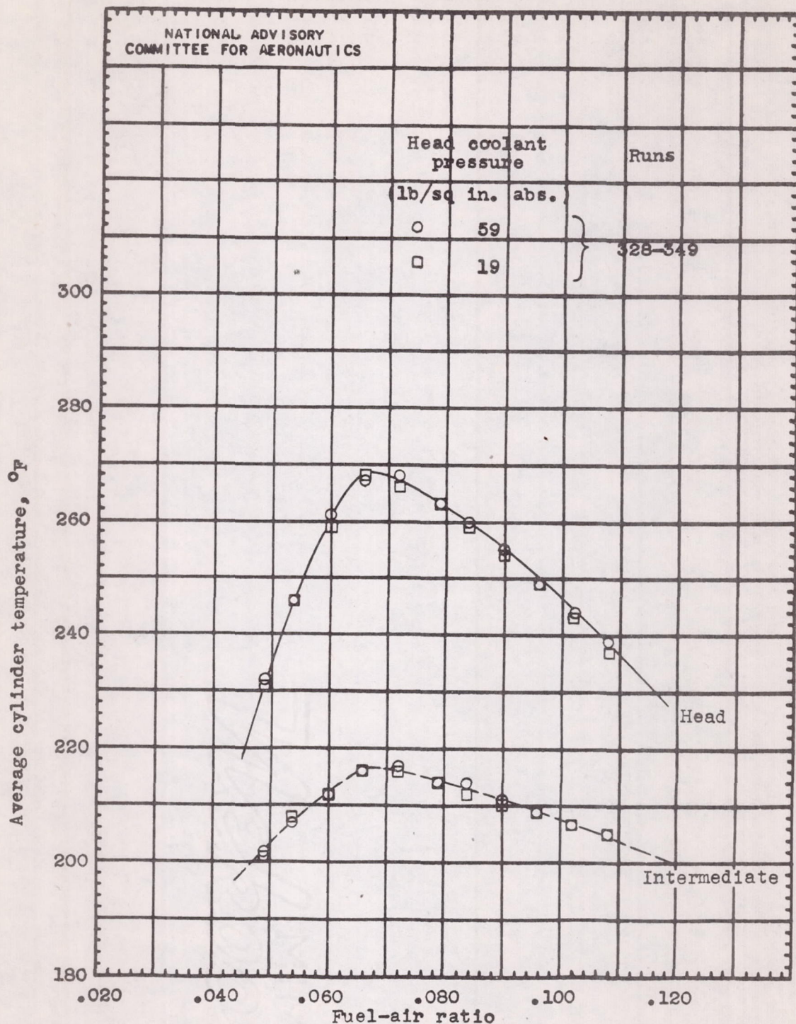
Figure 14.- Effect of fuel-air ratio on average head and intermediate temperatures. Cylinder B; coolant, water; average coolant temperature, 173° F; coolant-flow rate, 70 pounds per minute; engine speed, 2000 rpm; indicated horsepower, 40 to 62; charge-flow rate, 5.6 to 5.9 pounds per minute; spark advance, 28° B.T.C.; carburetor-air temperature, 74° F.
