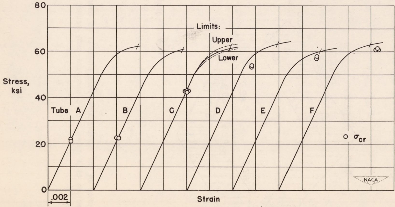
Figure 6.— Correlation of test results for the critical compressive stress for long, simply supported, flat plates with the compressive stress-strain curves for 14S-T6 aluminum alloy. (Calculated elastic critical compressive strain used for plate tests.)
