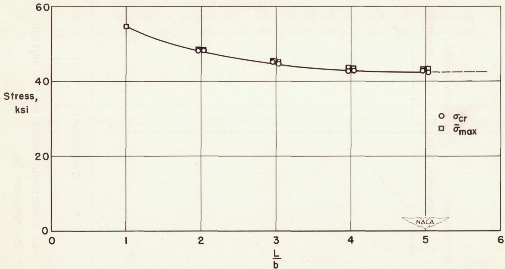
Figure 5.— Variation of critical compressive stress \sigma_{cr} and average stress at maximum load \bar{\sigma}_{max} with the length-width ratio L/b for square tubes of 14S-T6 aluminum alloy (tube C).
