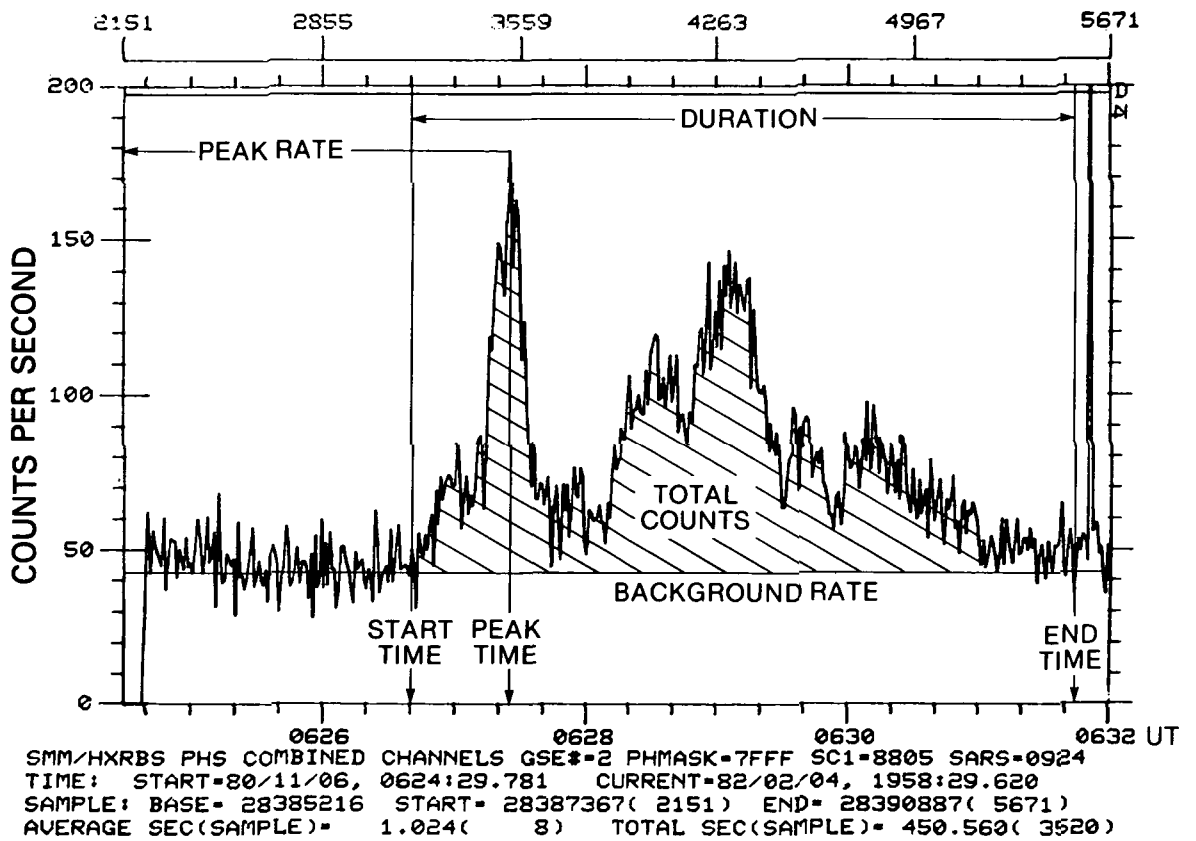
FIGURE 3. A standard plot of a hard X-ray burst (HXRB event #1544) showing the rate of counts in channels 1 through 15 versus Universal Time. The time resolution is 1.024 s, the time scale is 1 inch per minute, and the counting rate is corrected for instrumental dead time. The start time, peak time, duration, peak rate and total number of counts are indicated as they are determined for inclusion in the event listing.
