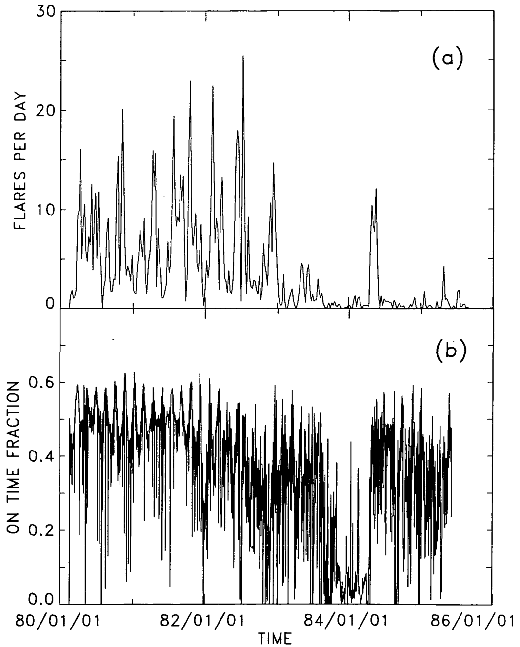
FIGURE 1. (a) The weekly average number of flares observed with HXRBS per day plotted as a function of time from 1980 through June 1985. (b) The fraction of time each day that HXRBS was operating with the sun in the field of view and for which data were recorded on the data retrieval computers within 24 hours of the observation.
