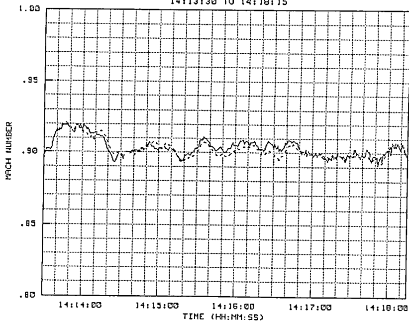
Figure 3-15(b). TP #5 radar-derived and on-board Mach number.
