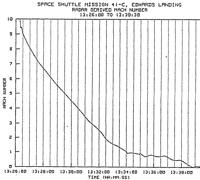
Figure 7-5(b). STS-41C radar-derived Mach number.
