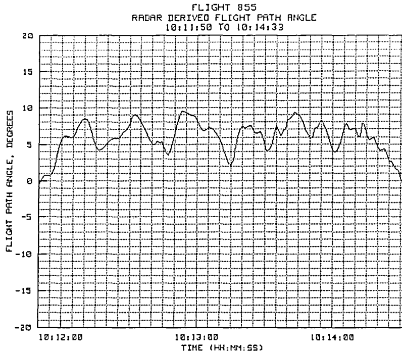
Figure 5-11(d). TP #2 radar-derived flight path angle.
