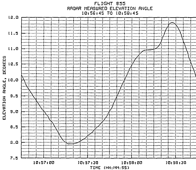
Figure 5-21(f). TP #12 radar-derived elevation angle.
