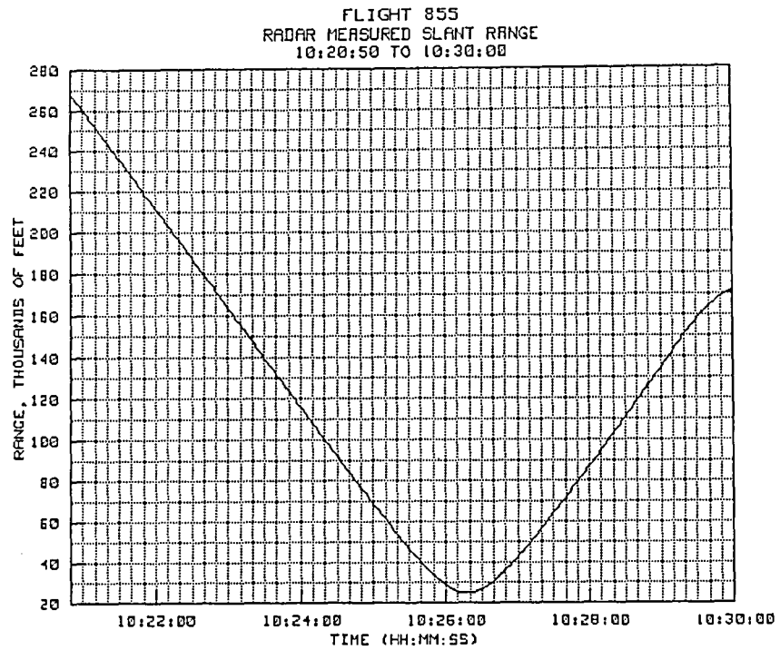
Figure 5-13(e). TP #4 radar-derived slant range.
