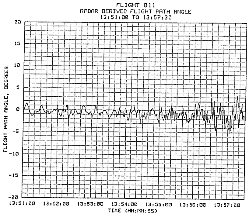
Figure 3-12(d). TP #3 radar-derived flight path angle.
