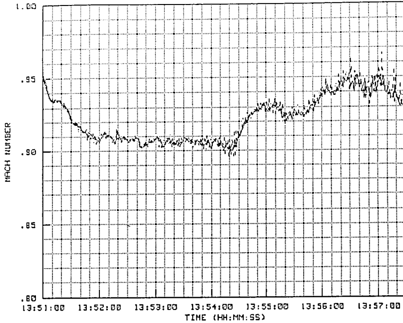
Figure 9-5. Cyber software analysis Mach number comparison plot.
