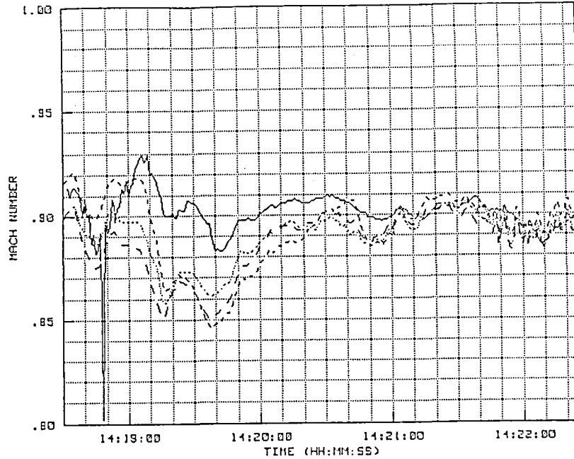
Figure 4-16. Mach comparison using three wind sources.
