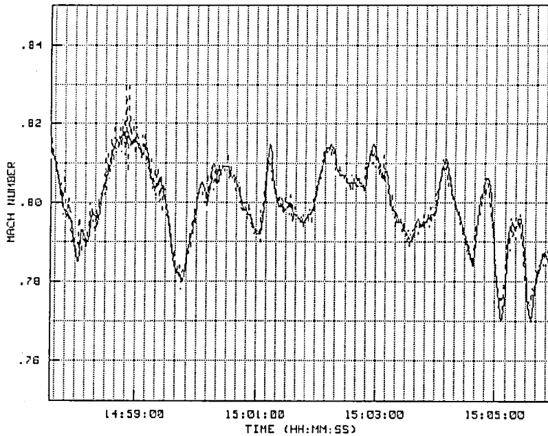
Figure 9-6. Cyber software analysis Mach number comparison plot.
