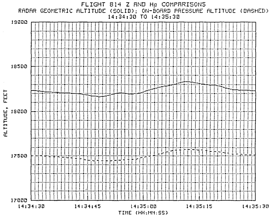
Figure 4-6. Flight 814 Z and H p comparison at 18,000 feet.
