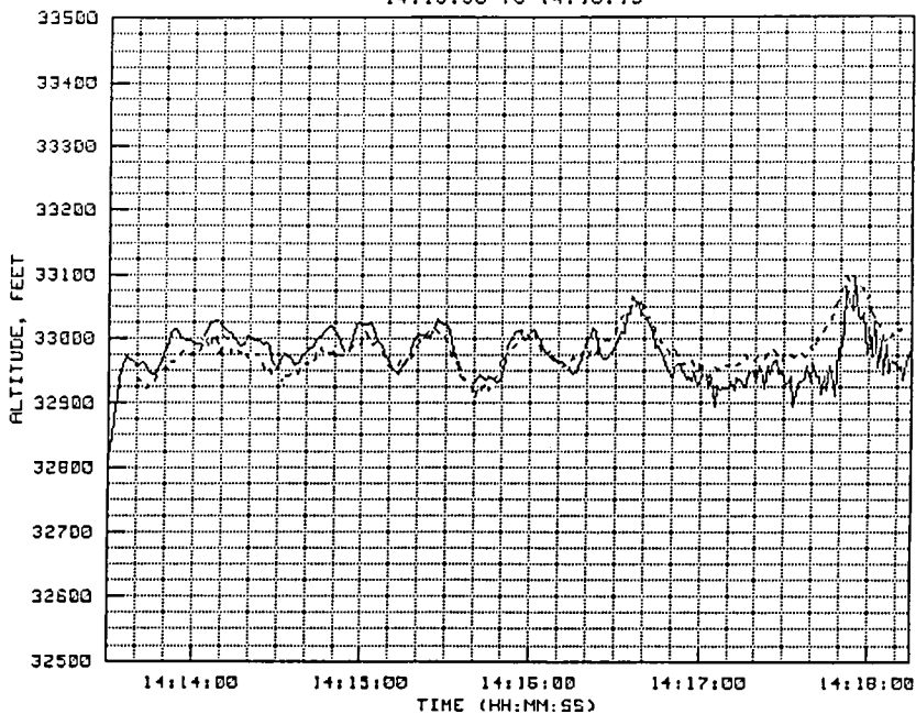
Figure 3-15(a). TP #5 radar-derived and on-board altitude.
