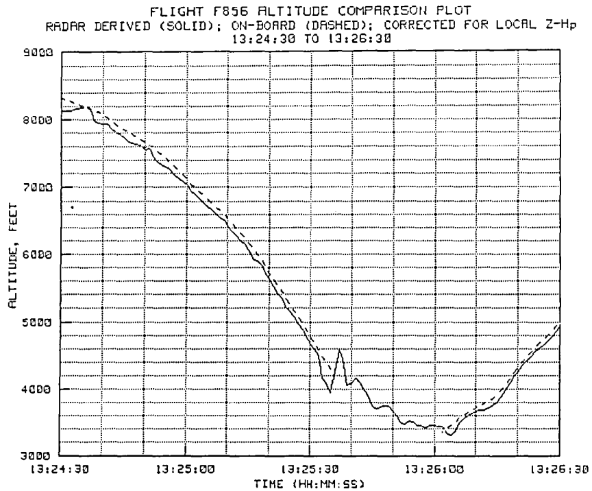
Figure 6-22(a). TP #13 radar-derived and on-board altitude.
