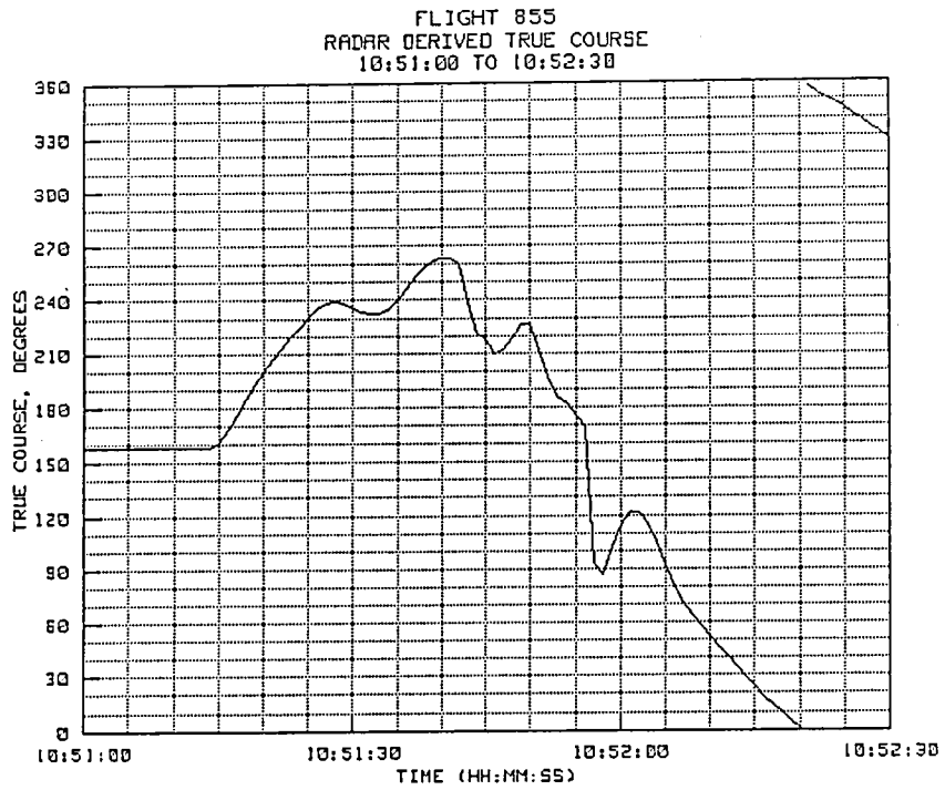
Figure 5-19(c). TP #10 radar-derived true course.
