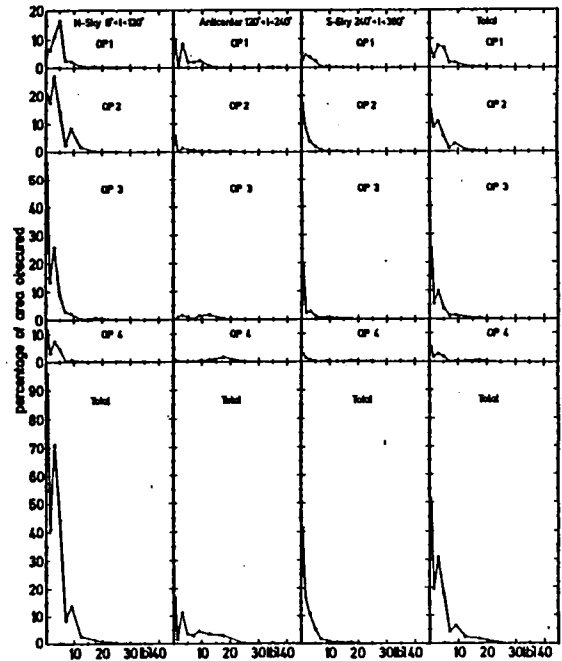
Fig.4 Percentage of obscured area as function of the galactic latitude |b| and the opacity classes
