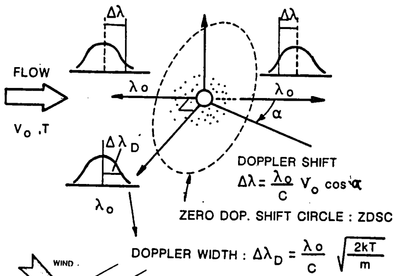
Figure 1. The Doppler width of the backscattered line profile is connected to the temperature ; the wavelength shift \Delta\lambda depends on angle \alpha between the line of sight and the flow direction.
