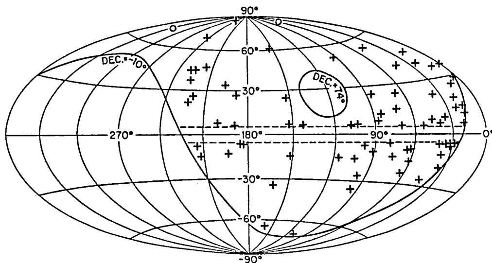
Fig. 1 - Directions of the high galactic latitude H\alpha scans. The map is in galactic coordinates centered on l = 180^\circ , b = 0^\circ . The crosses represent directions toward pulsars and the two open circles represent additional very high latitude H\alpha observations which are not part of the pulsar survey.
