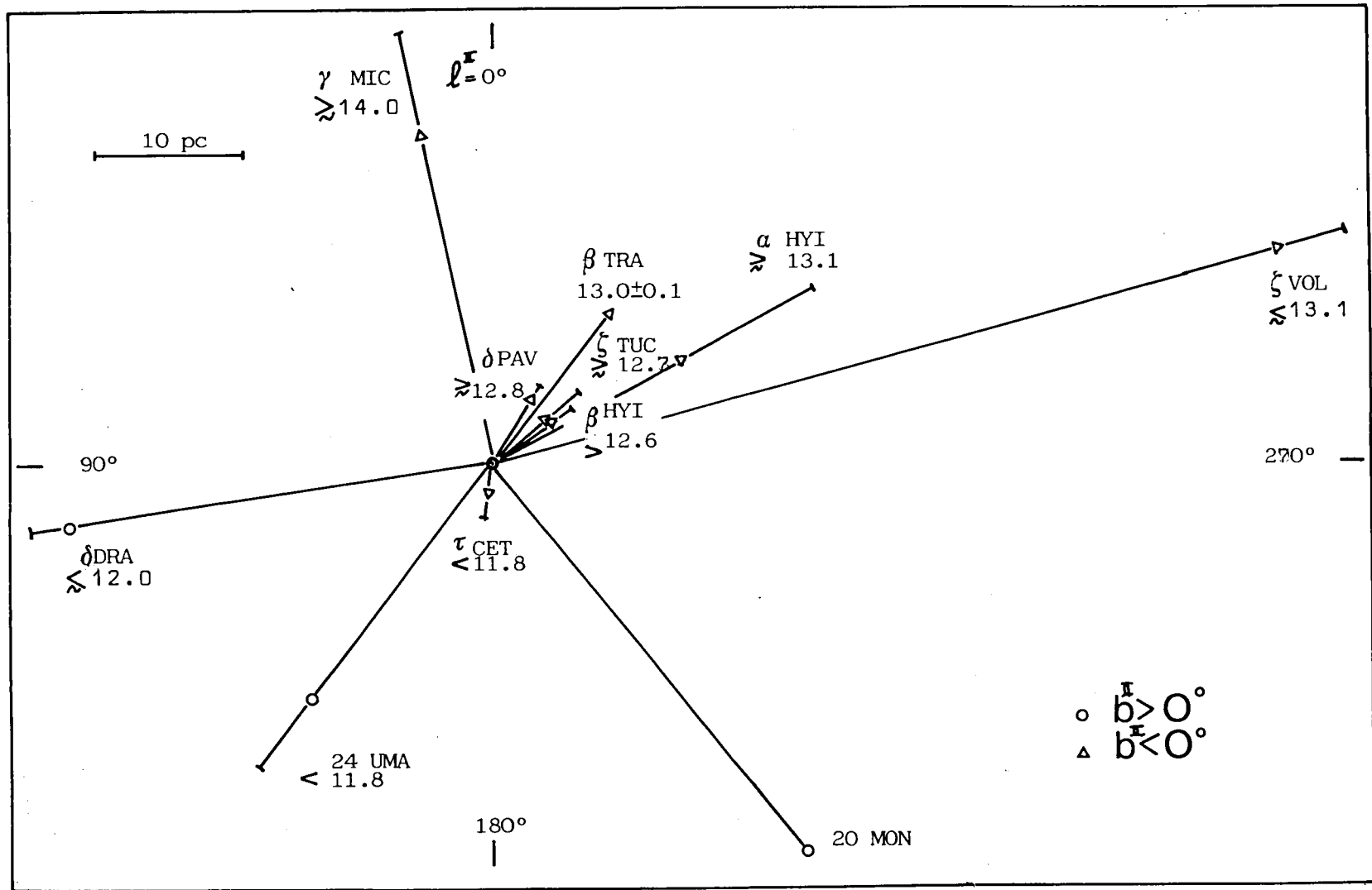
Figure 2. Log column densities of MgII towards late-type stars within 60 pc of the sun. Linear distances d to stars are solid lines. Projected distances d \cos b in the galactic plane are indicated by triangles and circles.
