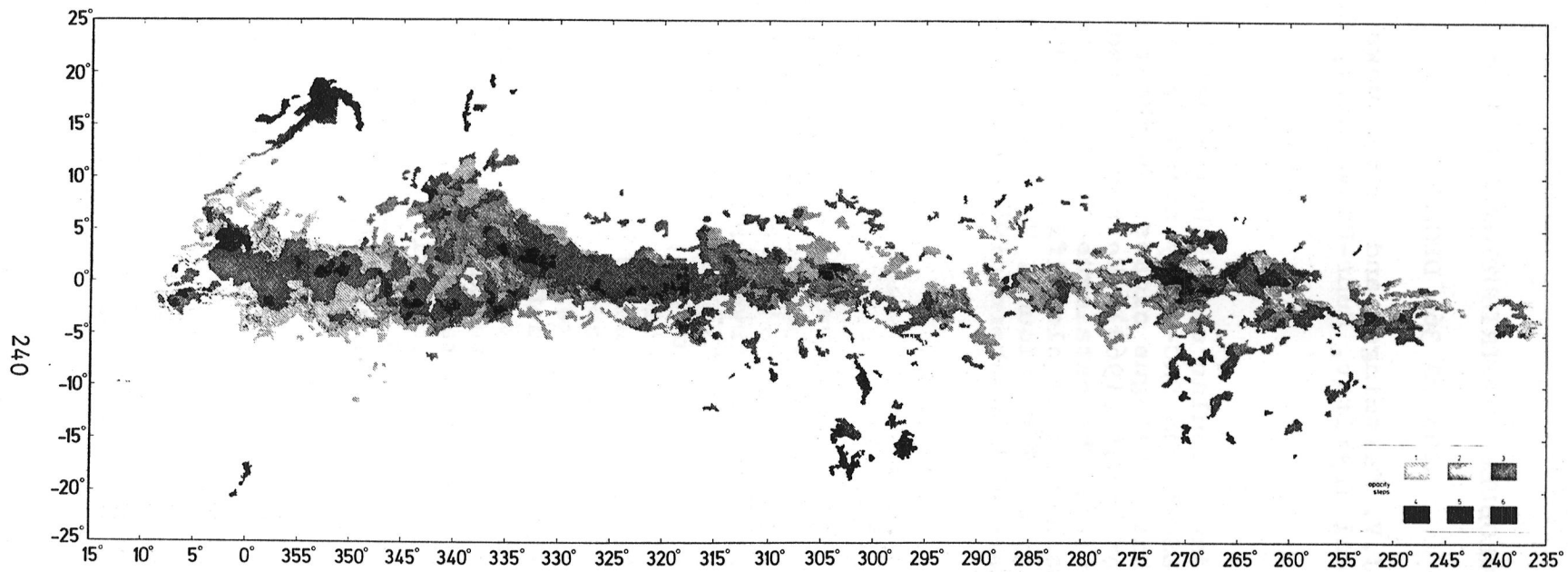
Fig.1 Distribution of dark clouds ( > 0.01 sqdeg)
