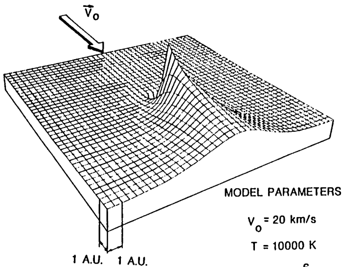
Figure 3. 3D representation of the density distribution in a plane containing the flow vector \vec{V}_0 . The vertical coordinate is proportional to the He density in the horizontal plane (after Dalaudier et al., 1984).
