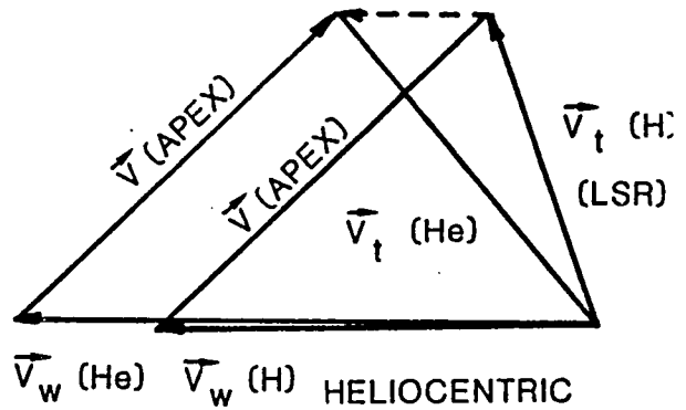
Fig.9 In the solar system, the vectors V_w(H) and V_w(He) have the same direction, but seems to have different modulus. Therefore, the difference V_w(H) - V_w(He) , which is independent of the coordinates system, is parallel to V_w(H) , which includes the particular motion of the Sun. This suggests an artefact in the determination of the modulus of V_w(He) .
