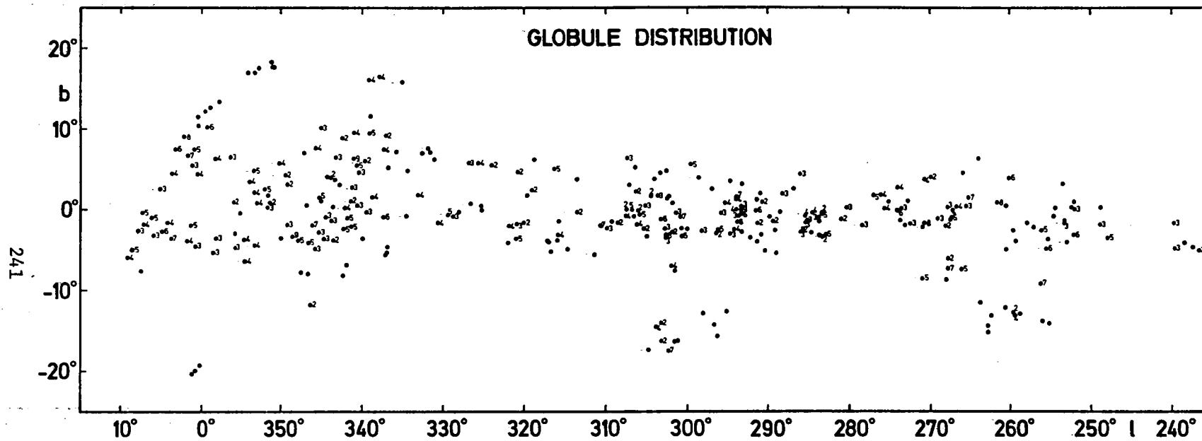
Fig.2 Distribution of globules ( 0.01 sqdeg). The numbers count globules almost at the same position.
