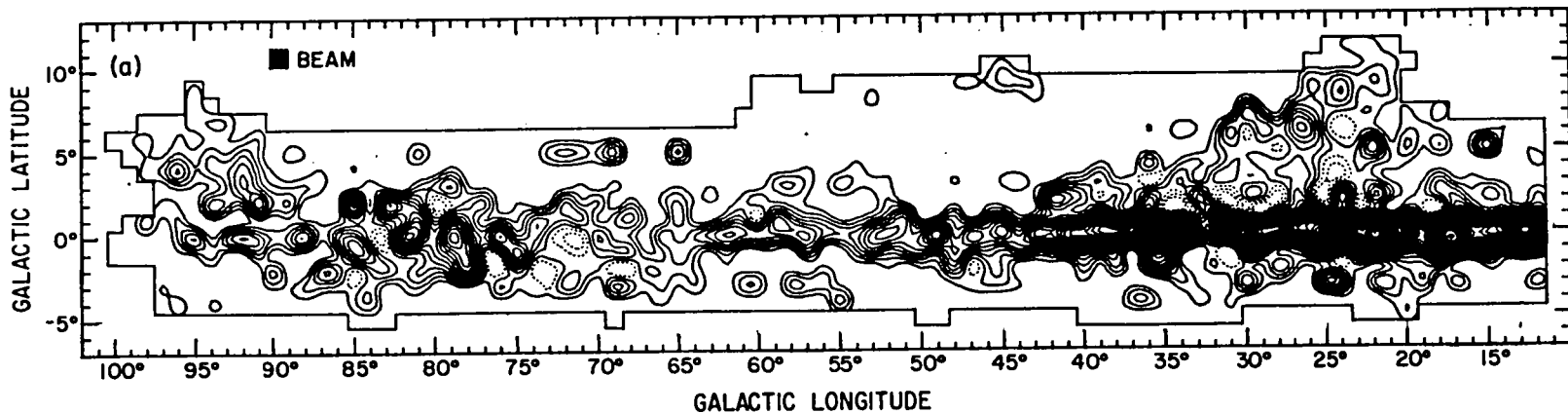
Figure 1. Contour map of the survey integrated over the full velocity range observed. For |b| \geq 3^\circ the velocity range is -83 to 83 \text{ km s}^{-1} , while for |b| < 3^\circ the range is -13 to 153 \text{ km s}^{-1} at l \leq 60^\circ , and -113 to 53 \text{ km s}^{-1} at l > 60^\circ . The contour interval is 4 \text{ K km s}^{-1} .
