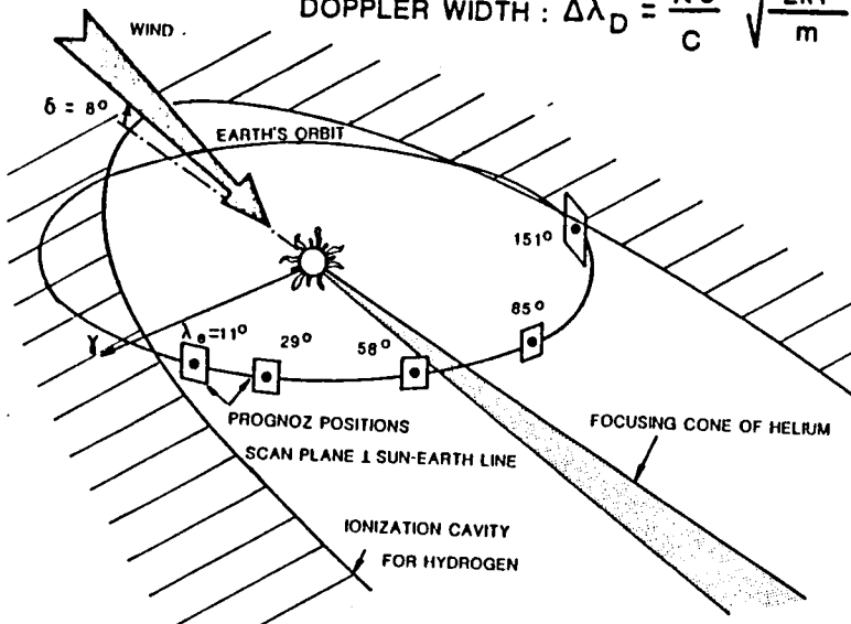
Figure 2. The main features of interstellar gas distribution in the solar system are i) a focusing cone of helium in the downwind direction ; ii) a cavity of ionization, void of atoms, elongated toward the downwind direction.
