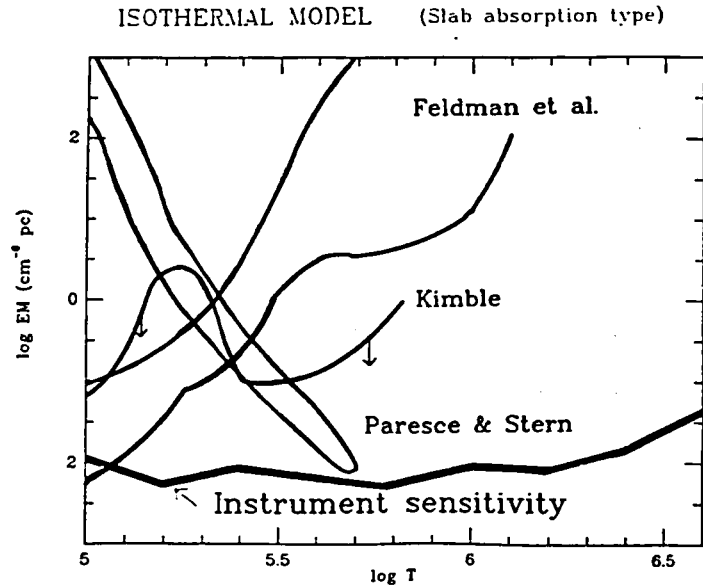
Figure 3. The constraints imposed on an isothermal model by previous observations is shown with the minimum emission measure necessary to detect two emission lines.
