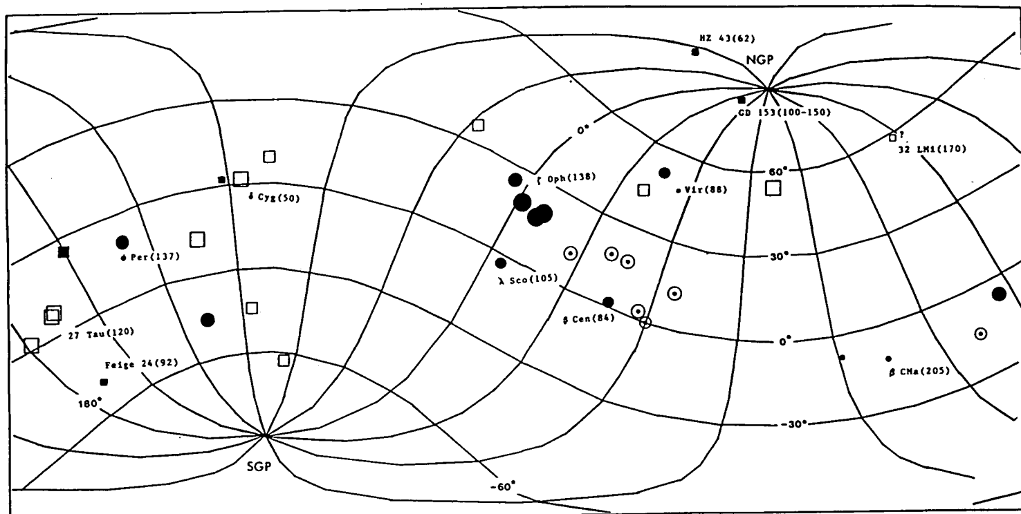
Figure 2. H I Column Densities Toward Stars with 50 < d < 150 pc. (See caption for Fig.1) Most directions exhibit N(\text{H I}) > 10^{19} \text{ cm}^{-2} . Two regions, with N(\text{H I}) on the order of 10^{18} \text{ cm}^{-2} ( \beta CMa) or less (GD 153 and HZ 43 toward the NGP), are indicated. Stars at greater distances toward the NGP reveal significant amounts, N(\text{H I}) > 10^{19} \text{ cm}^{-2} (See text.). A low column density measurement for the white dwarf, 2111+49, seems in conflict with that of \delta Cyg, a few degrees away in the sky. Yet, uncertainties in distances may make 2111+49 like W1346 (Fig. 1), a foreground object to \delta Cyg. The column density measured for \lambda Sco is probably mostly due to the local cloud, which extends no further than 20 pc from the Sun. (Again, see Fig.1.)
