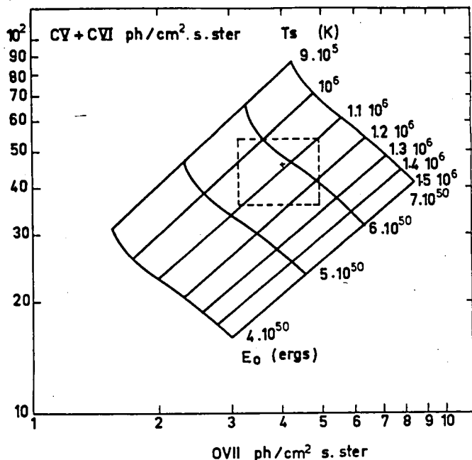
Fig.2 : Full lines: (CV + CVI) and OVII line intensities computed in our model for different values of E_0 and T_s . Dashed line : intensity range allowed by observations. Fig.3 : 99% confidence contour on the parameters.
