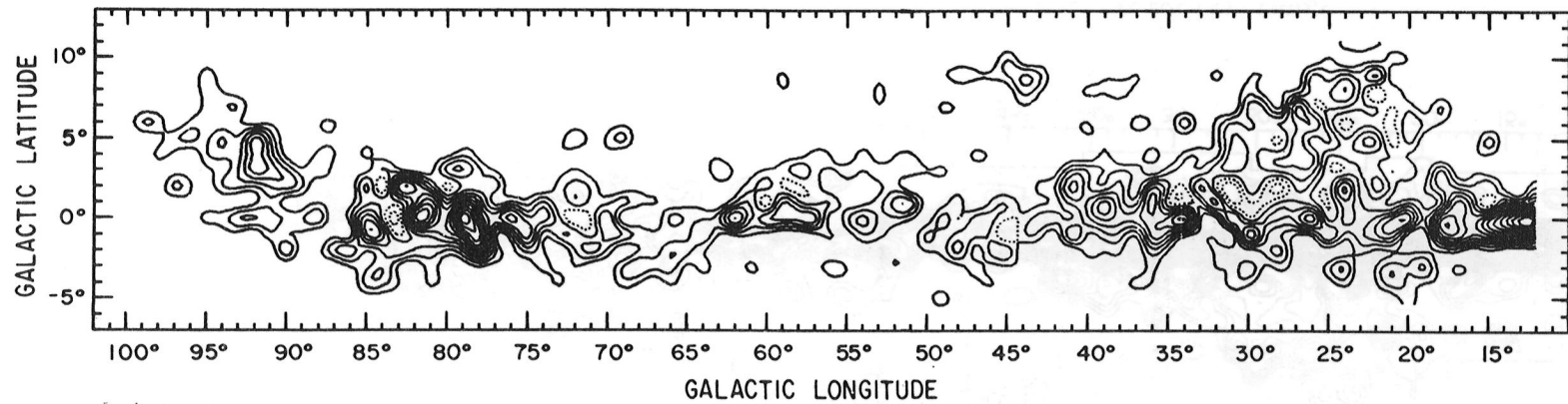
Figure 2. Mt. Wilson mosaic of the Milky Way, with a contour map on the same scale of the CO emission integrated between -10 and 34 \text{ km s}^{-1} . The contour interval is 4 \text{ K km s}^{-1} ; the lowest contour is overlaid on the photo.
