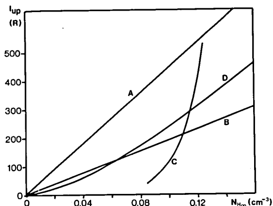
Figure 2: Upwind Ly-alpha resonance luminescence intensities versus asymptotic hydrogen density N_{H\infty} . Curve A: "Classical" dependence without interface extinction; curve B: with interface extinction, and constant N_{p\infty} ; curve C: with interface extinction, using (N_{H\infty} + N_{p\infty}) = \text{const} ; curve D: self-consistent p\infty interface of Baranov (1981), using only loss processes. Curves A, B, and C use as a reference point the interplanetary Ly-alpha observations of Bertaux et al. (1976).
