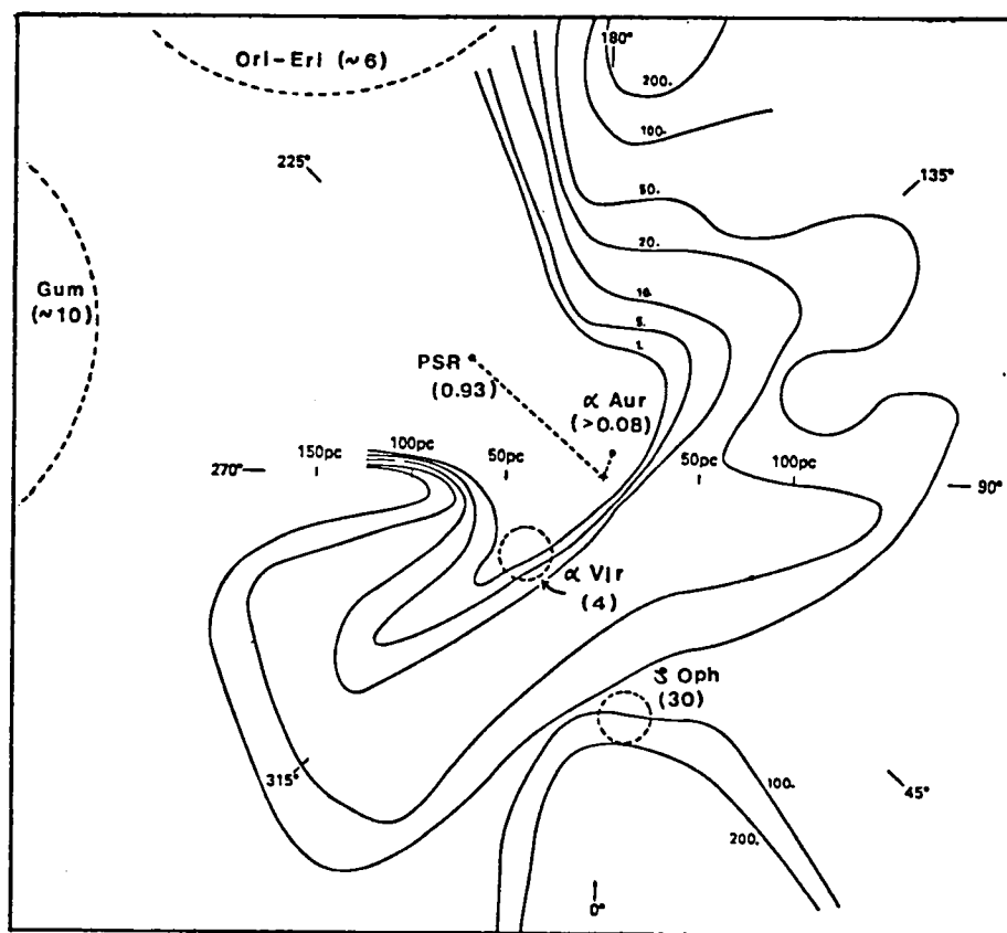
Fig. 4 - Observed regions of ionized gas in the local interstellar medium projected onto the galactic plane and superposed on a contour map of H ^{\circ} column densities by Paresce (1984). The lines of sight to PSR0950+08 and Capella ( \alpha Aur) are indicated by straight dotted lines. The size and location of HII regions are indicated by dotted circles. The number in parentheses denotes the H ^+ column density in units of 10^{19} \text{ cm}^{-2} along the line of sight to the star or pulsar or through the center of the HII region. The contours of H ^{\circ} column density (solid curves) are labeled from 1 to 200 units of 10^{19} \text{ cm}^{-2} .
