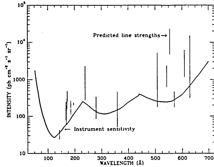
Figure 4. The minimum detectable line flux and a range of predicted line strengths.
