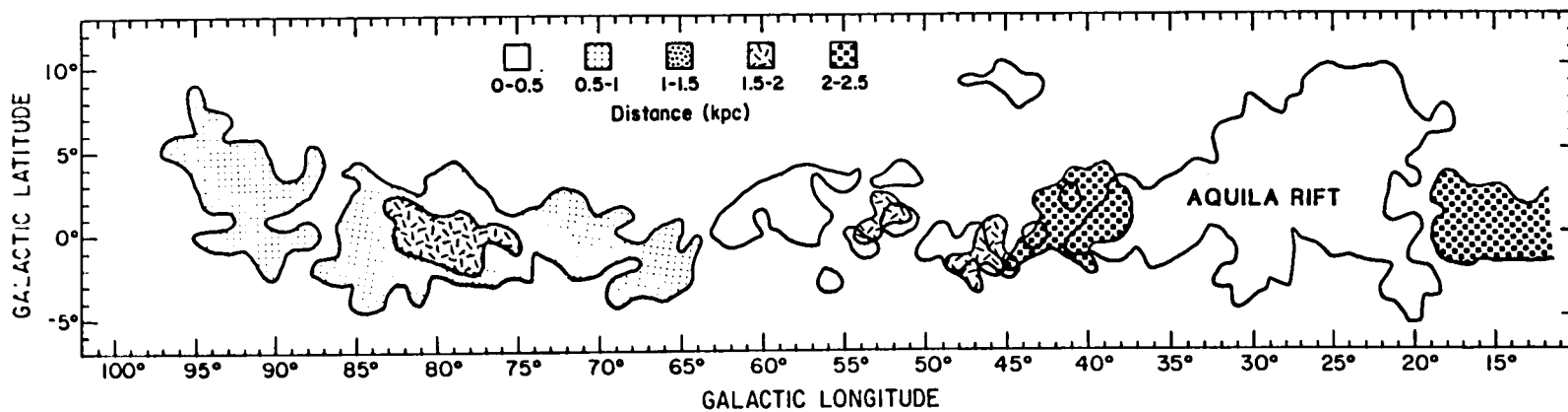
Figure 3. Schematic map of the individual molecular clouds which comprise the Great Rift. The clouds are outlined by their 4 \text{ K km s}^{-1} CO emission contours. Distances are indicated by the shading.
