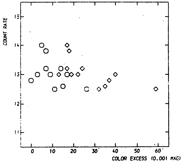
Fig.2. 0.5 0.5 sq.deg counts versus upper and lower excess limit. Only pixels with more than two extinctions observations.
