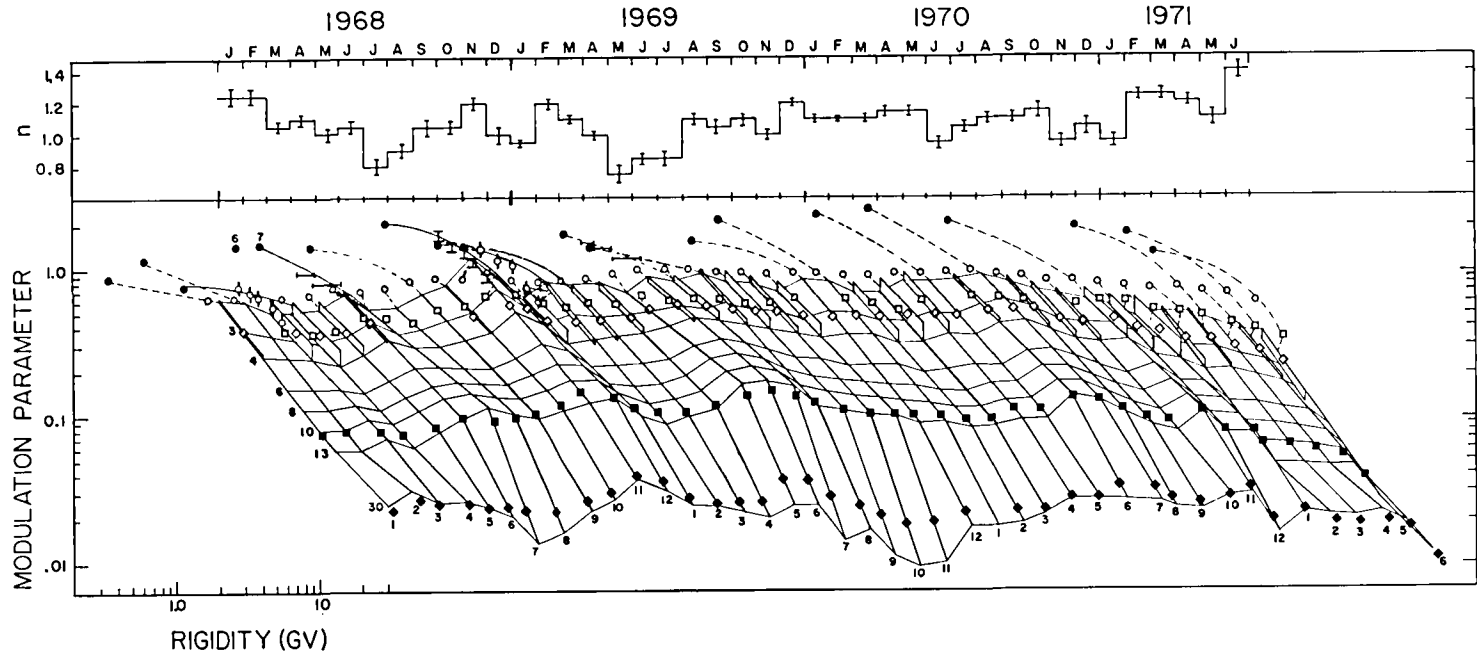
Figure 46. - Spectrum of the modulation parameter, M , monthly averages, between 1/68 and 6/71. M = \ln(J_{1965}/J_t) .
