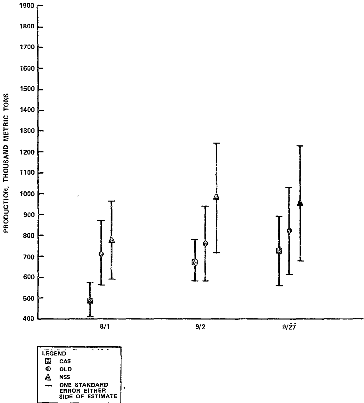
(b) Production. Figure 5.— Concluded.
