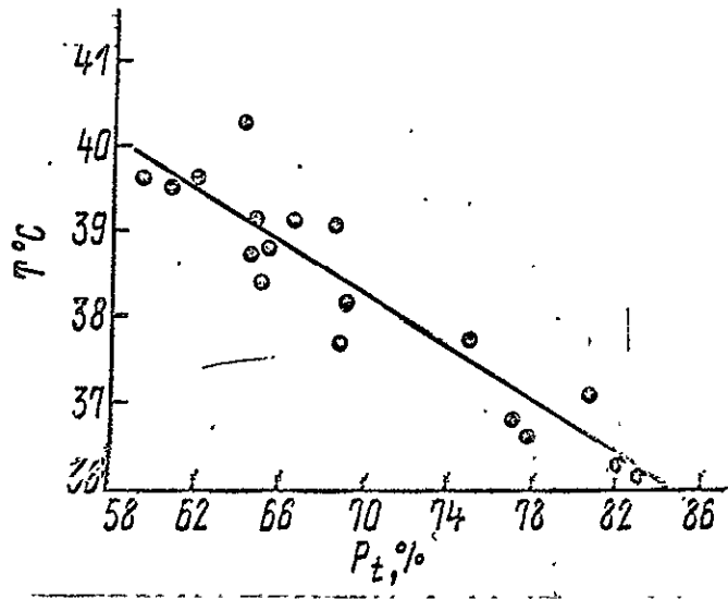
Figure 12. Dependence of thermodynamic temperature of the cotton leaf ( T^{\circ}C ) on relative turgor (%) (Holter, 1970).
