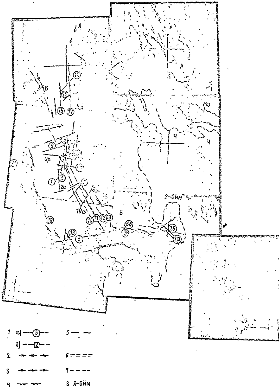
Fig. 2. Scheme of structural-geomorphological interpretation of montage of telephoto images of Verkhoyan ridge (4th AES "Meteor" 6/7/1970), on section of telephoto image of central portion of Verkhoyan: ridge-basin of Lynyshka River (4th AES "Meteor") (6/17/1970) (see similar images fig. 2, II, III, IV).
