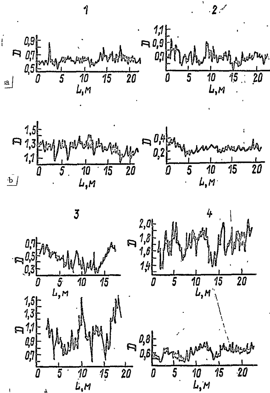
Figure 11. Comparison of densitometric registrograms of identical profiles by multi-band photographs (Vinogradov, 1966): a — in orange-red part of the spectrum \lambda 0.58–0.69 micron and b — in green-yellow part of the spectrum \lambda 0.52–0.62 micron, where: 1 — mesophyt-mixed grass-couch grass meadows, 2 — hygromesophyte-mixed grass-sedge swamp, 3 — shoots of willow on alluvium, 4 — fields with sprouting crops.
