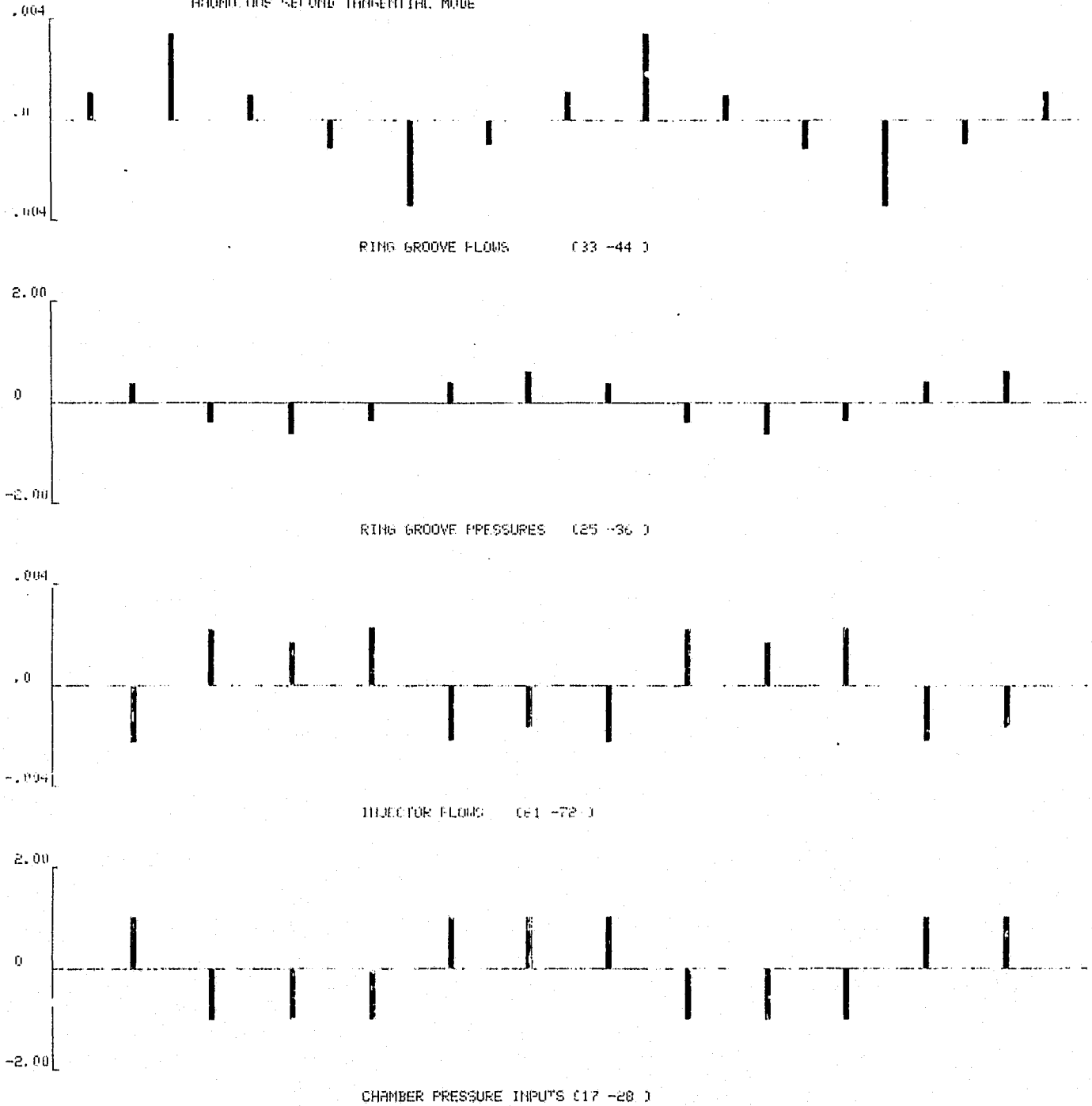
Figure 51. Results for Fuel Ring of XRL Injector - No Dams
