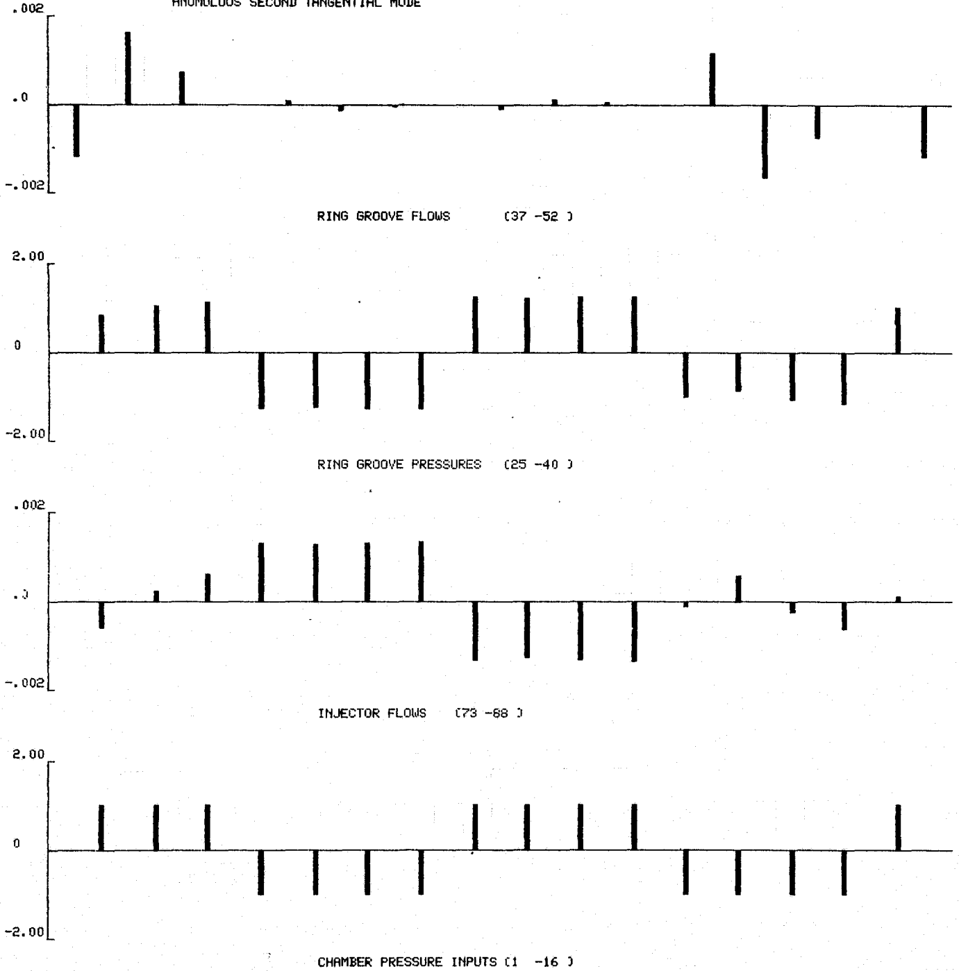
Figure 54. Results for Ox Ring of XRL Injector - Dams
