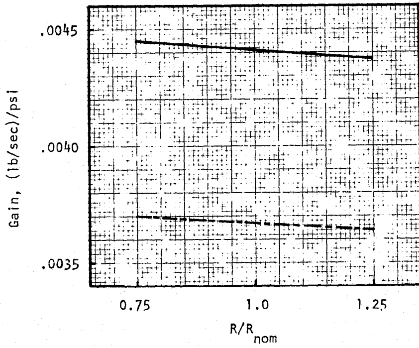
Figure 64. Effect of Frequency and Resistance on Gain for Fuel Side of Rocketdyne OME Technology Injector
