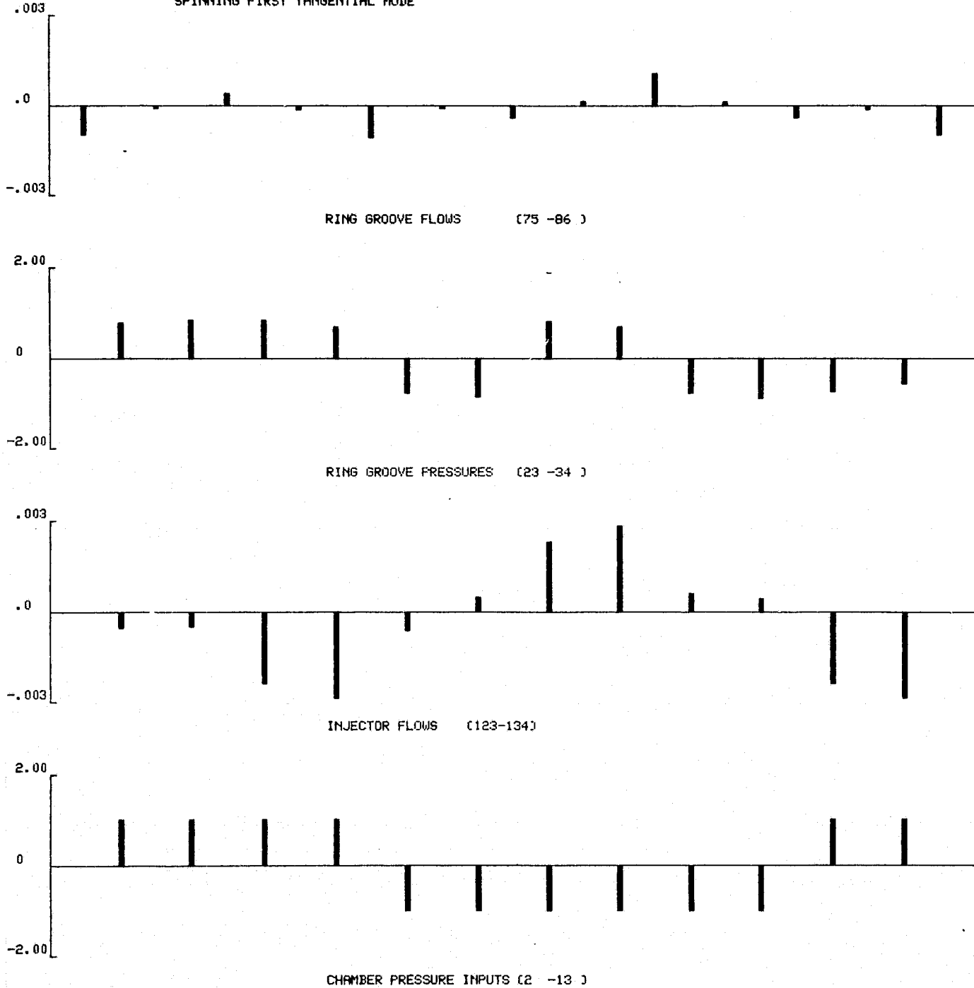
Figure 57. Results for Outer Ox Ring Groove of Aerojet Injector - No Dams
