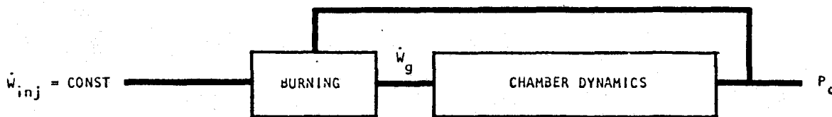
Figure 1. Acoustic Instability - Variations in Burning Rate
