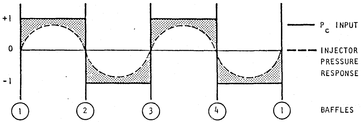
Figure 29. Pressure Response Characteristics
