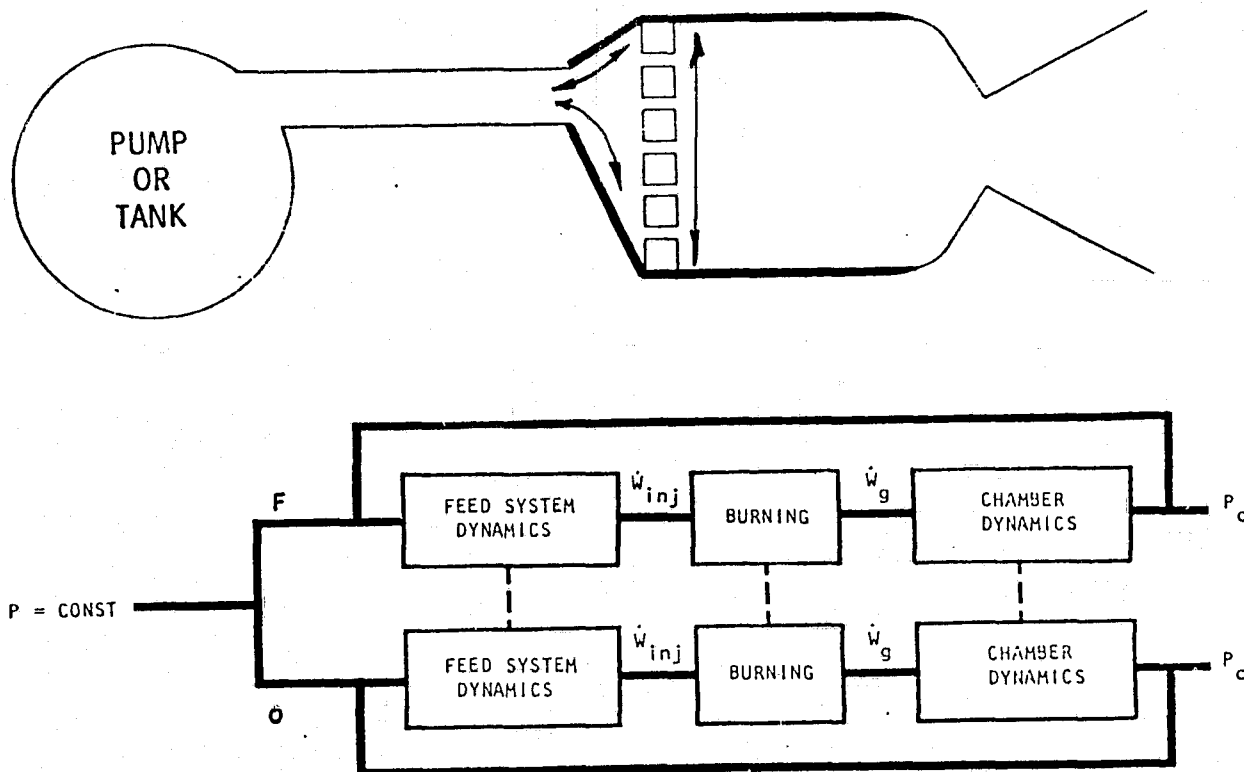
Figure 4. Hybrid Instability
