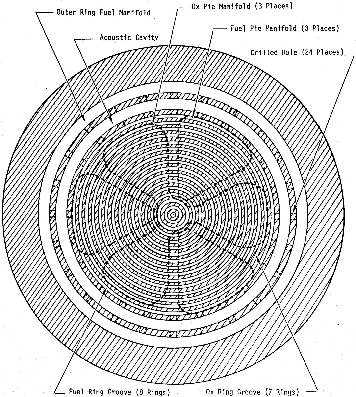
Figure 16. Bottom View of Aerojet OMF Technology Injector
