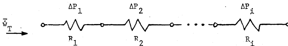
Figure 22. Series Flow
