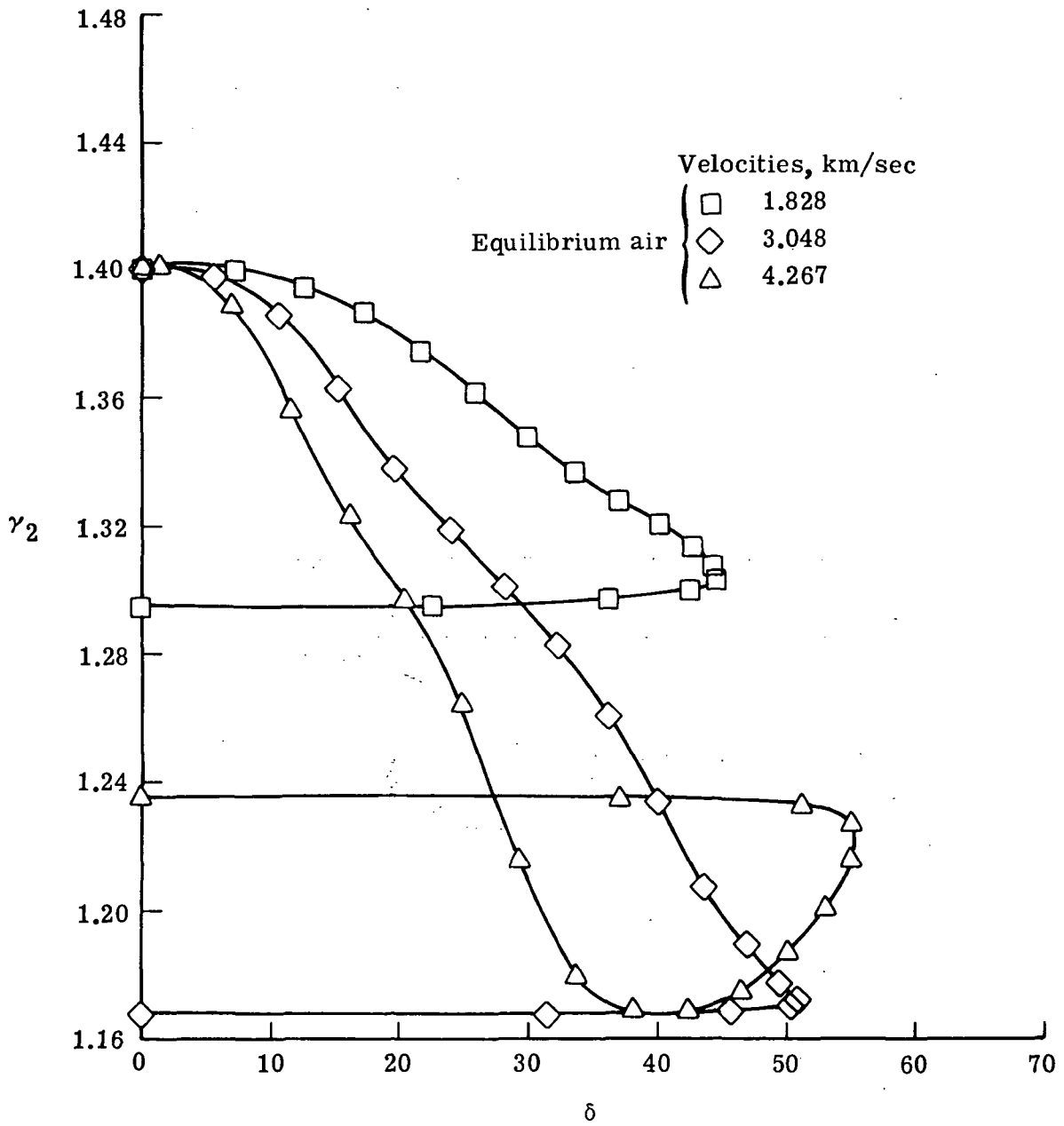
(e) \gamma_2 .
