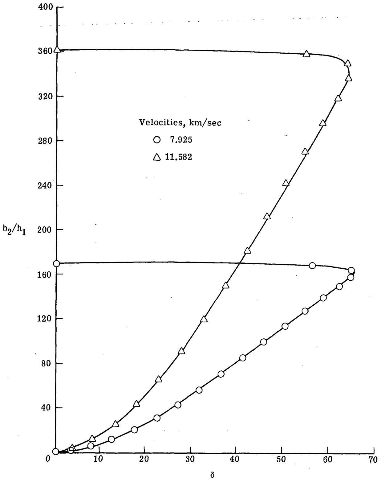
(i) h_2/h_1 .
