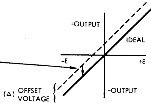
Figure AD-15. Buffer; V_{out} vs V_{in}
