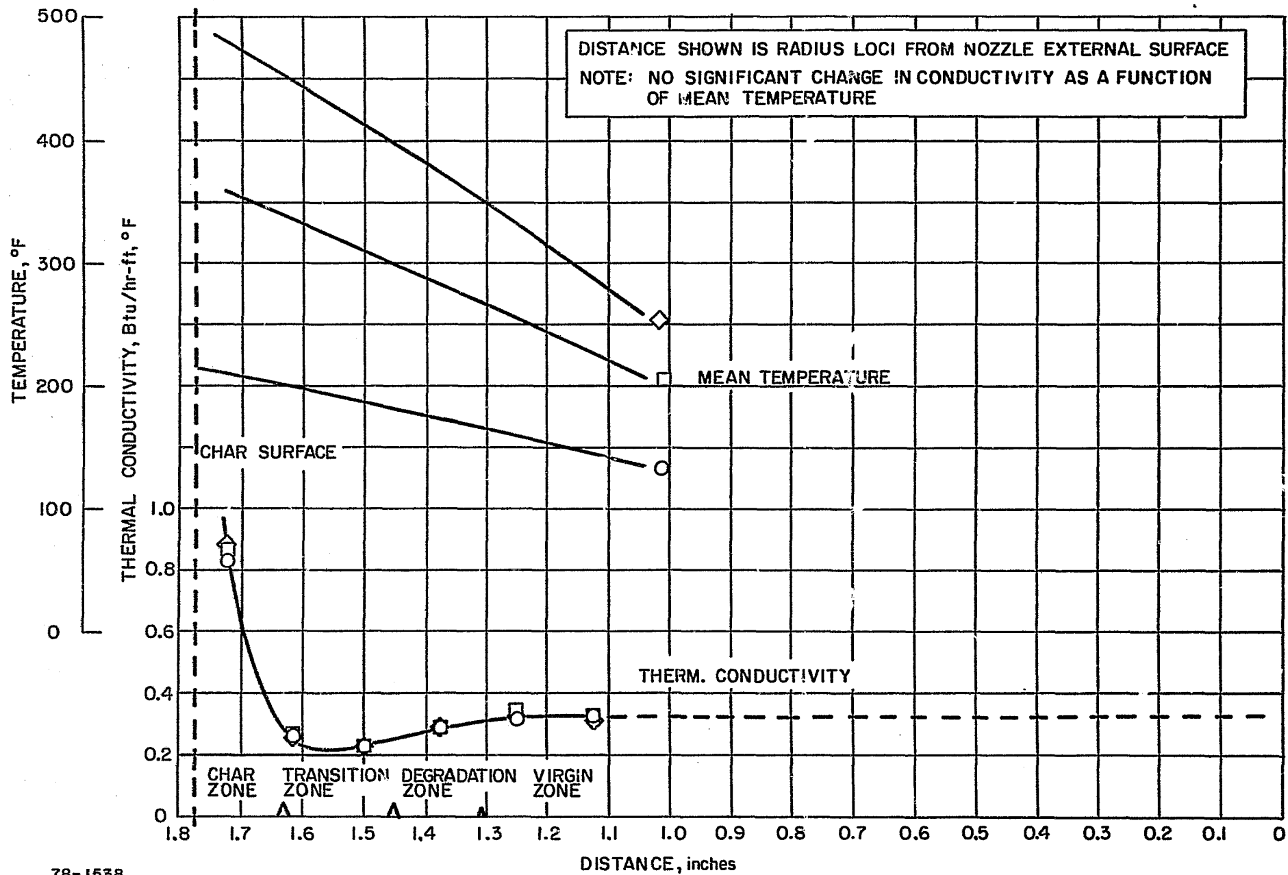
Figure 95 SILICA-PHENOLIC NOZZLE EXIT, THERMAL CONDUCTIVITY VERSUS CHAR DEPTH
