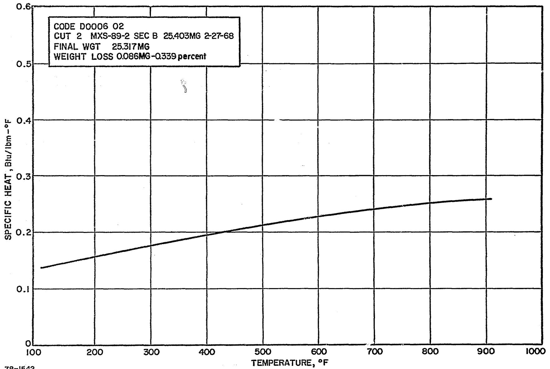
Figure 99 SILICA-PHENOLIC NOZZLE THROAT, 1.707-INCH CHAR LAYER, SPECIFIC HEAT VERSUS TEMPERATURE
