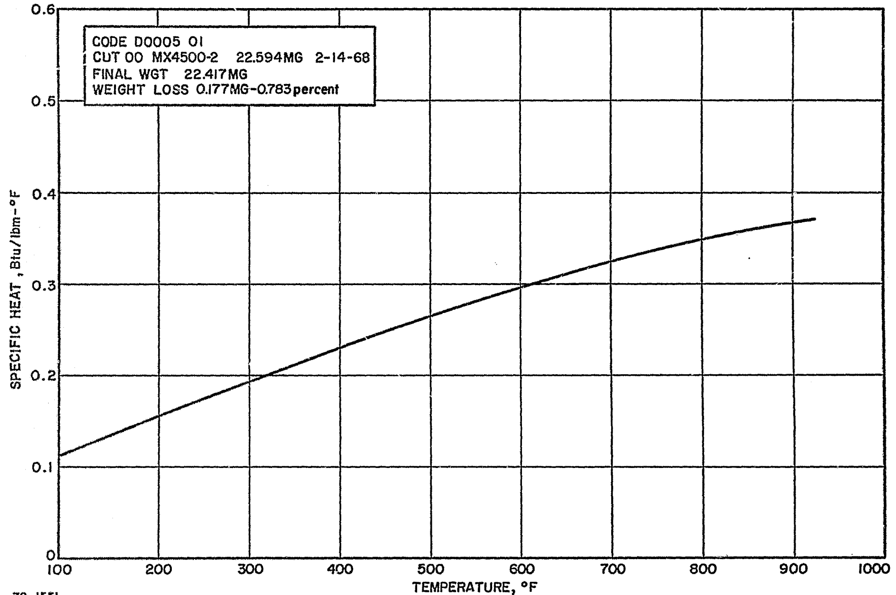
Figure 108 GRAPHITE-PHENOLIC NOZZLE EXIT, SURFACE CHAR, SPECIFIC HEAT VERSUS TEMPERATURE
