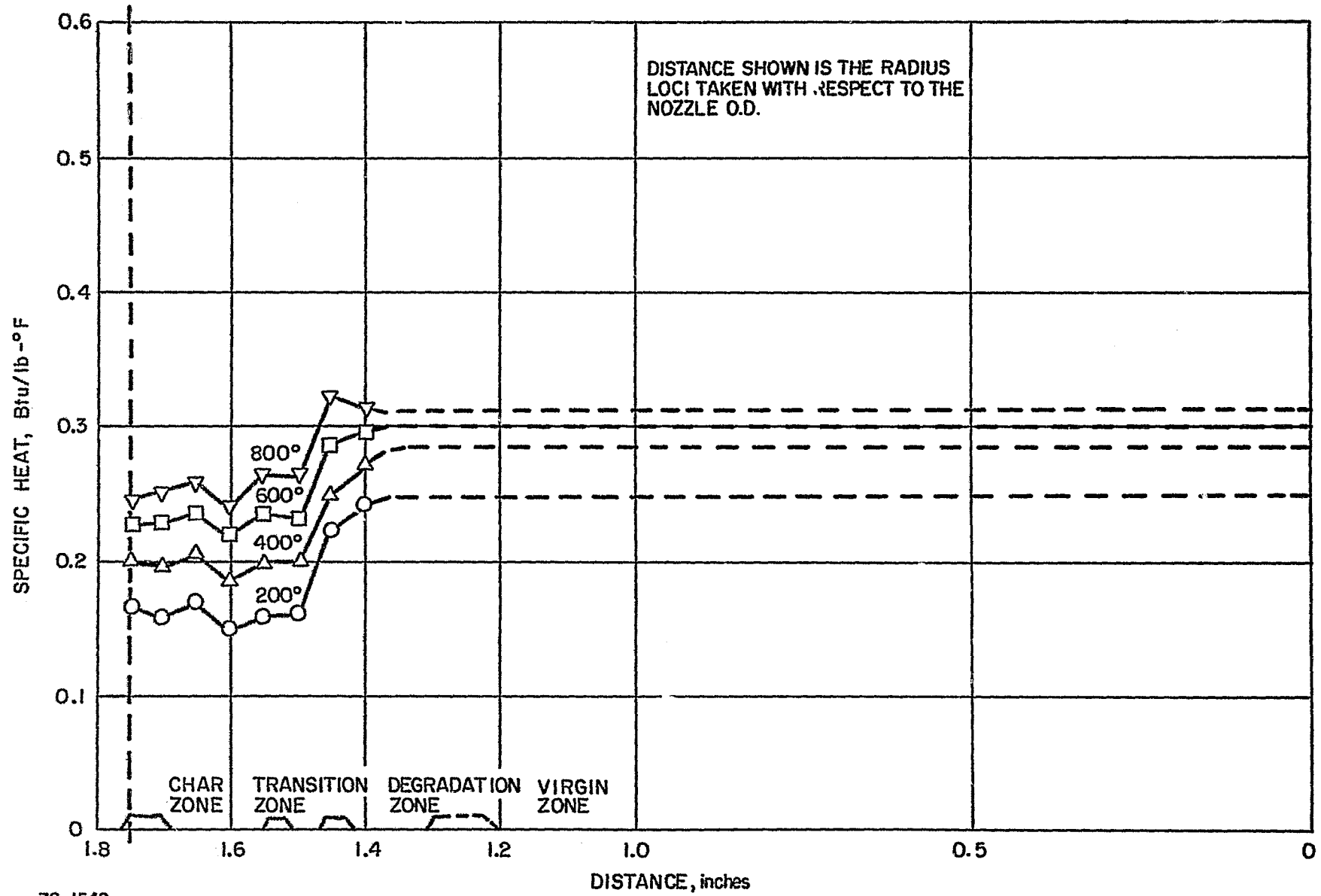
Figure 106 SILICA-PHENOLIC NOZZLE THROAT, SPECIFIC HEAT (AT TEMPERATURE) VERSUS CHAR DEPTH
