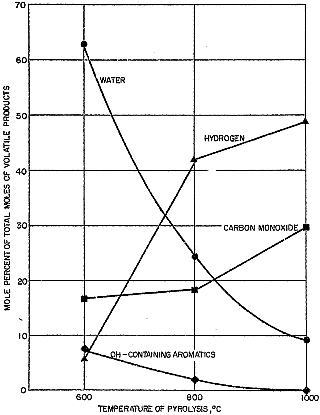
Figure 40 PRODUCT DISTRIBUTION FROM DECOMPOSITION OF SILICA REINFORCED PHENOLIC RESIN
