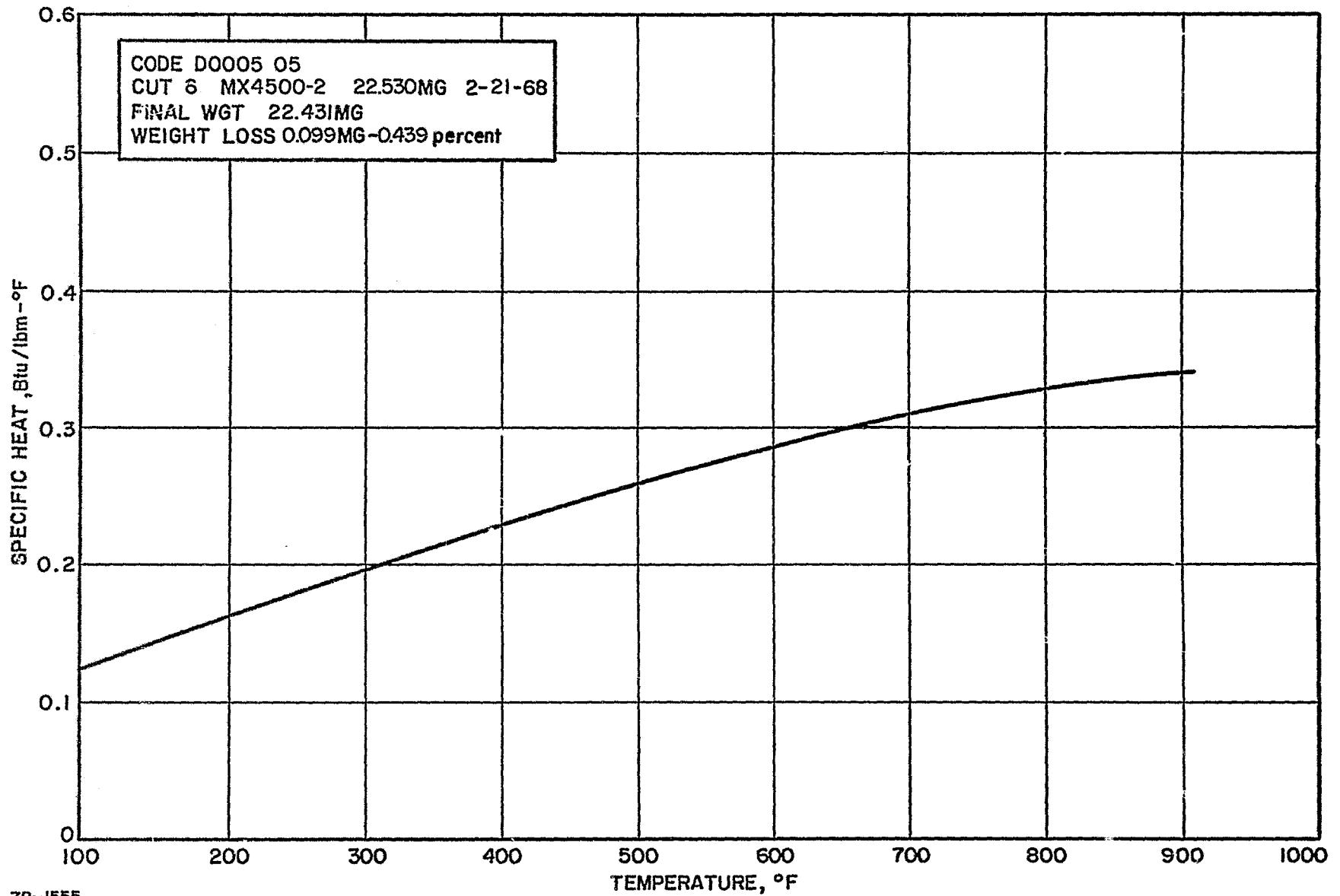
Figure 112 GRAPHITE-PHENOLIC NOZZLE EXIT, 1.553-INCH CHAR LAYER, SPECIFIC HEAT VERSUS TEMPERATURE
