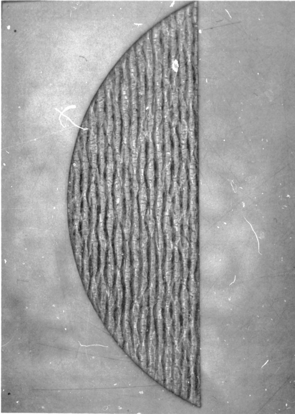
Figure 10 1000°F OVEN-CHARRED SILICA-PHENOLIC MXS-89 CORING (5X MAGNIFICATION)
