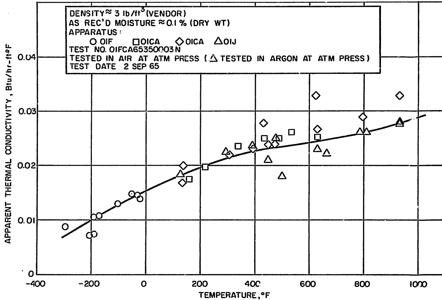
Figure C-3 APPARENT THERMAL CONDUCTIVITY VERSUS TEMPERATURE, TG15000
