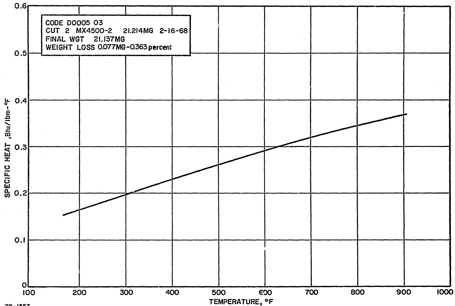
Figure 110 GRAPHITE-PHENOLIC NOZZLE EXIT, 1.653-INCH CHAR LAYER, SPECIFIC HEAT VERSUS TEMPERATURE
