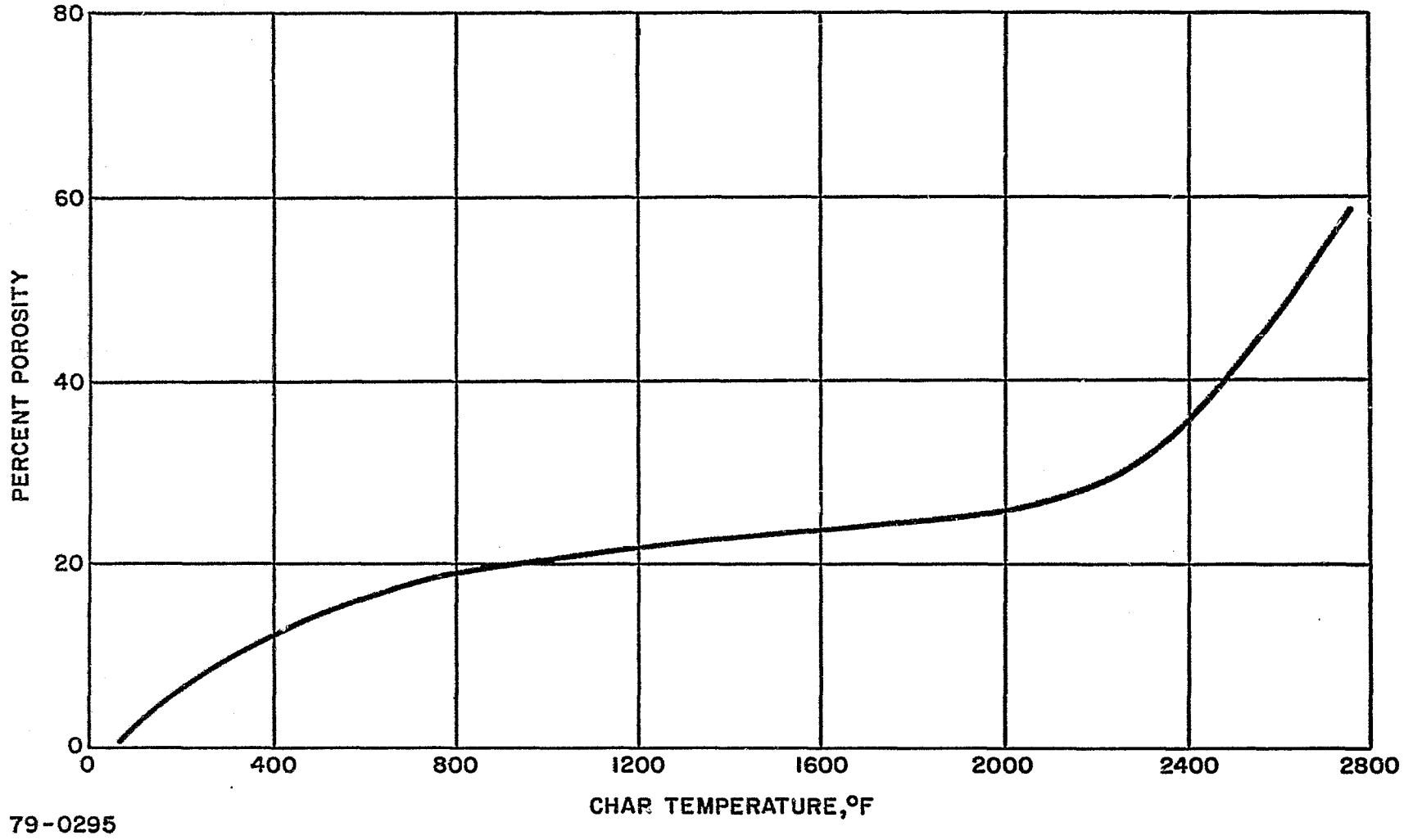
Figure 31 SILICA PHENOLIC MXS-89, PERCENT POROSITY VERSUS CHAR TEMPERATURE
