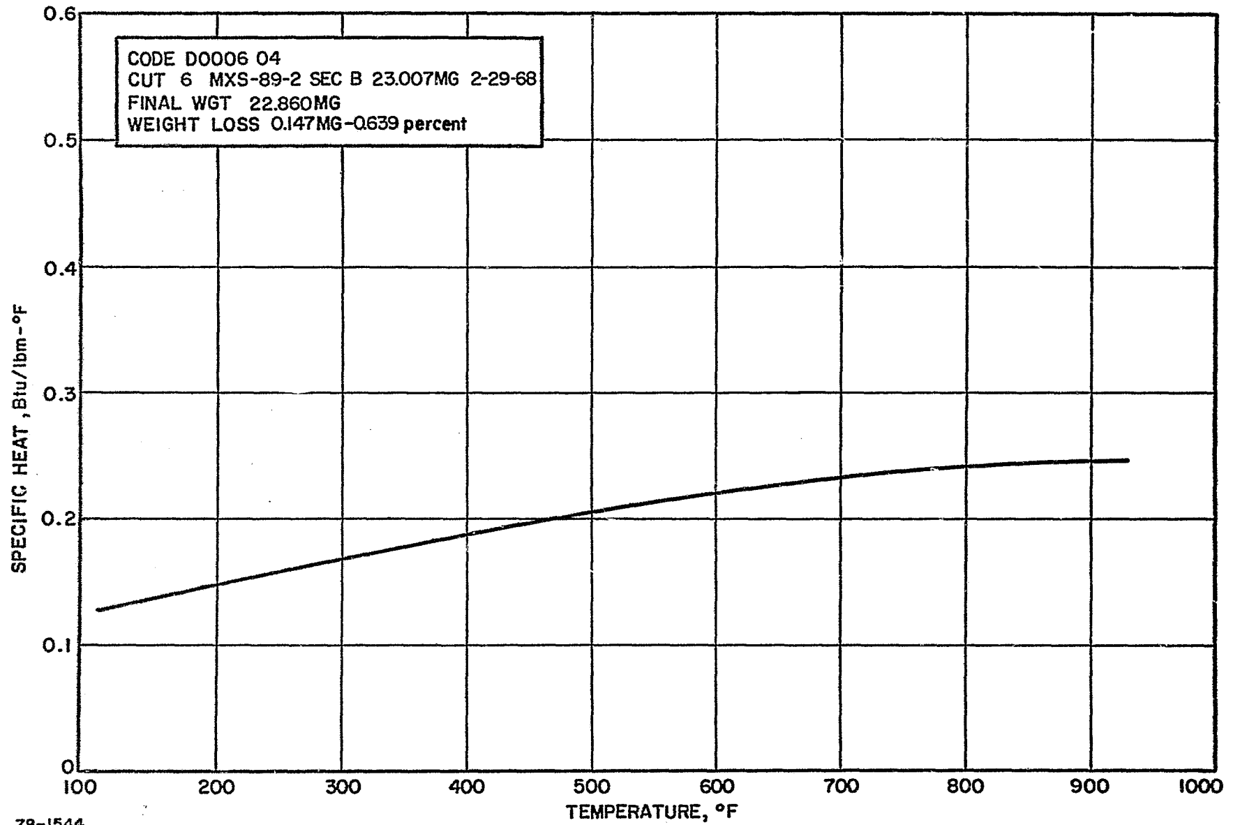
Figure 101 SILICA-PHENOLIC NOZZLE THROAT, 1.604-INCH CHAR LAYER, SPECIFIC HEAT VERSUS TEMPERATURE
