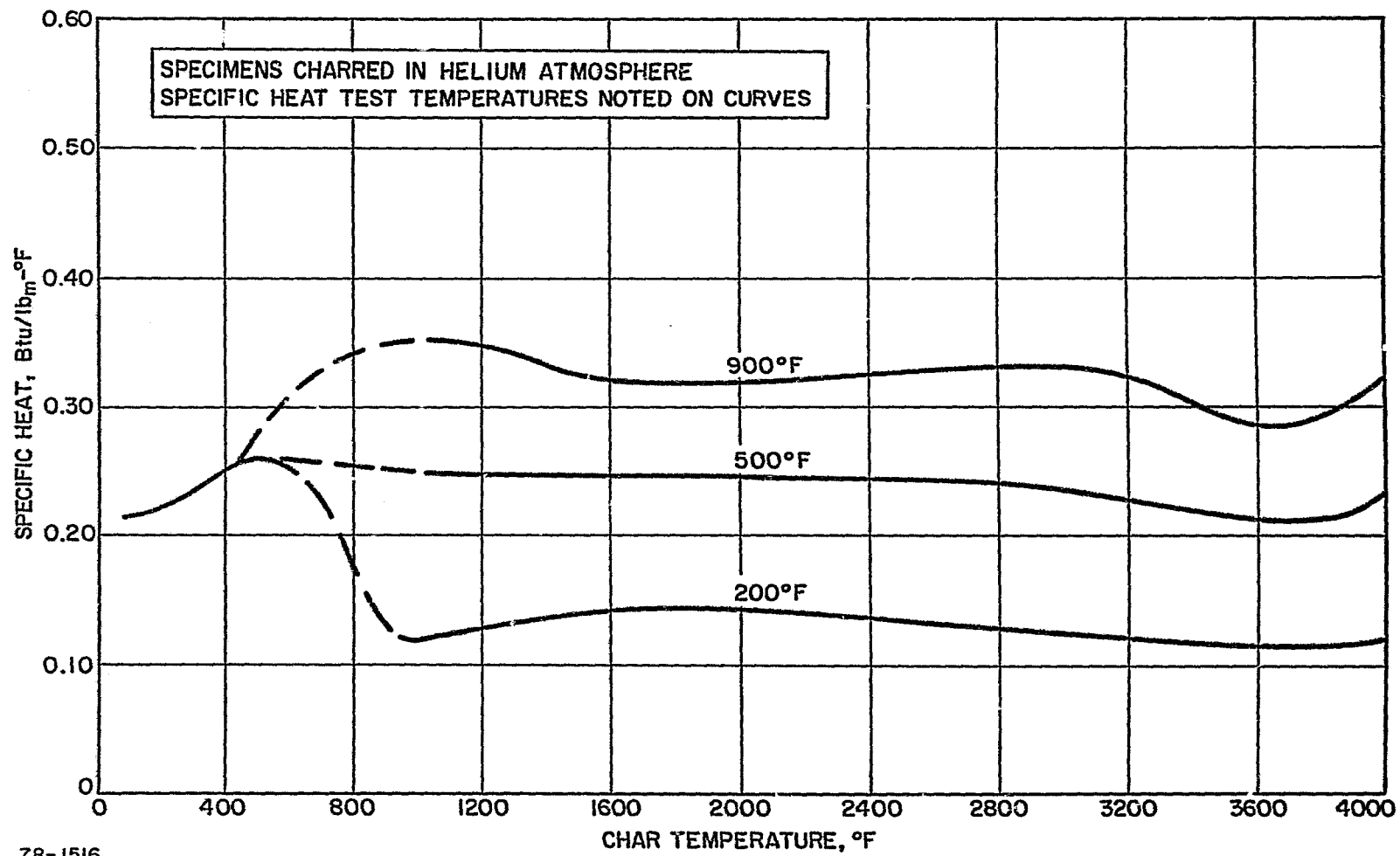
Figure 68 GRAPHITE PHENOLIC MX4501, SPECIFIC HEAT (AT TEMPERATURE) VERSUS CHAR TEMPERATURE
