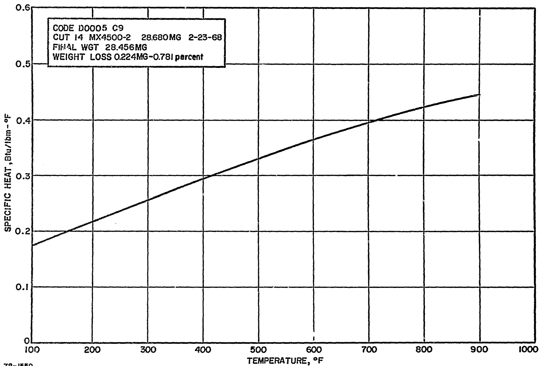
Figure 116 GRAPHITE-PHENOLIC NOZZLE EXIT, 1.326-INCH CHAR LAYER, SPECIFIC HEAT VERSUS TEMPERATURE
