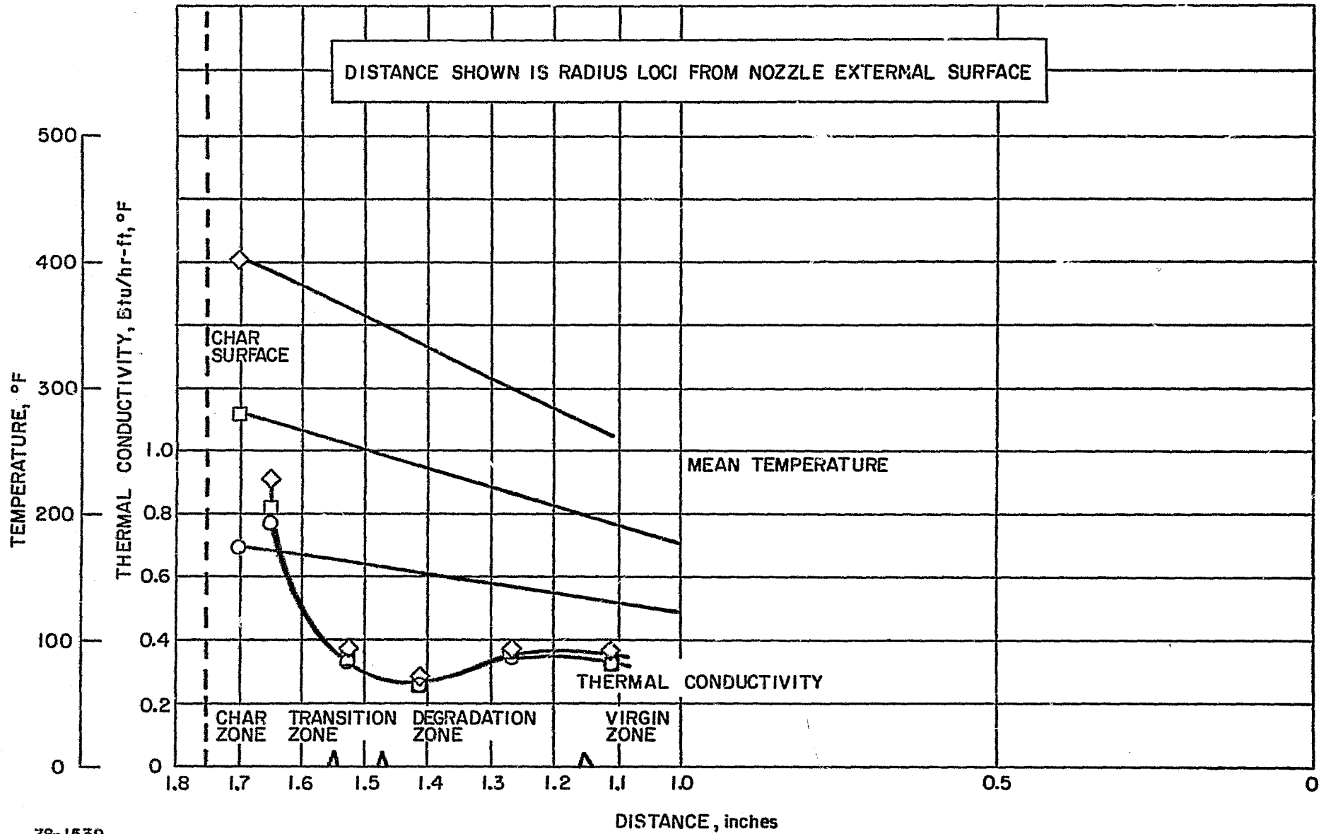
Figure 96 SILICA-PHENOLIC NOZZLE RAMP, THERMAL CONDUCTIVITY VERSUS CHAR DEPTH
