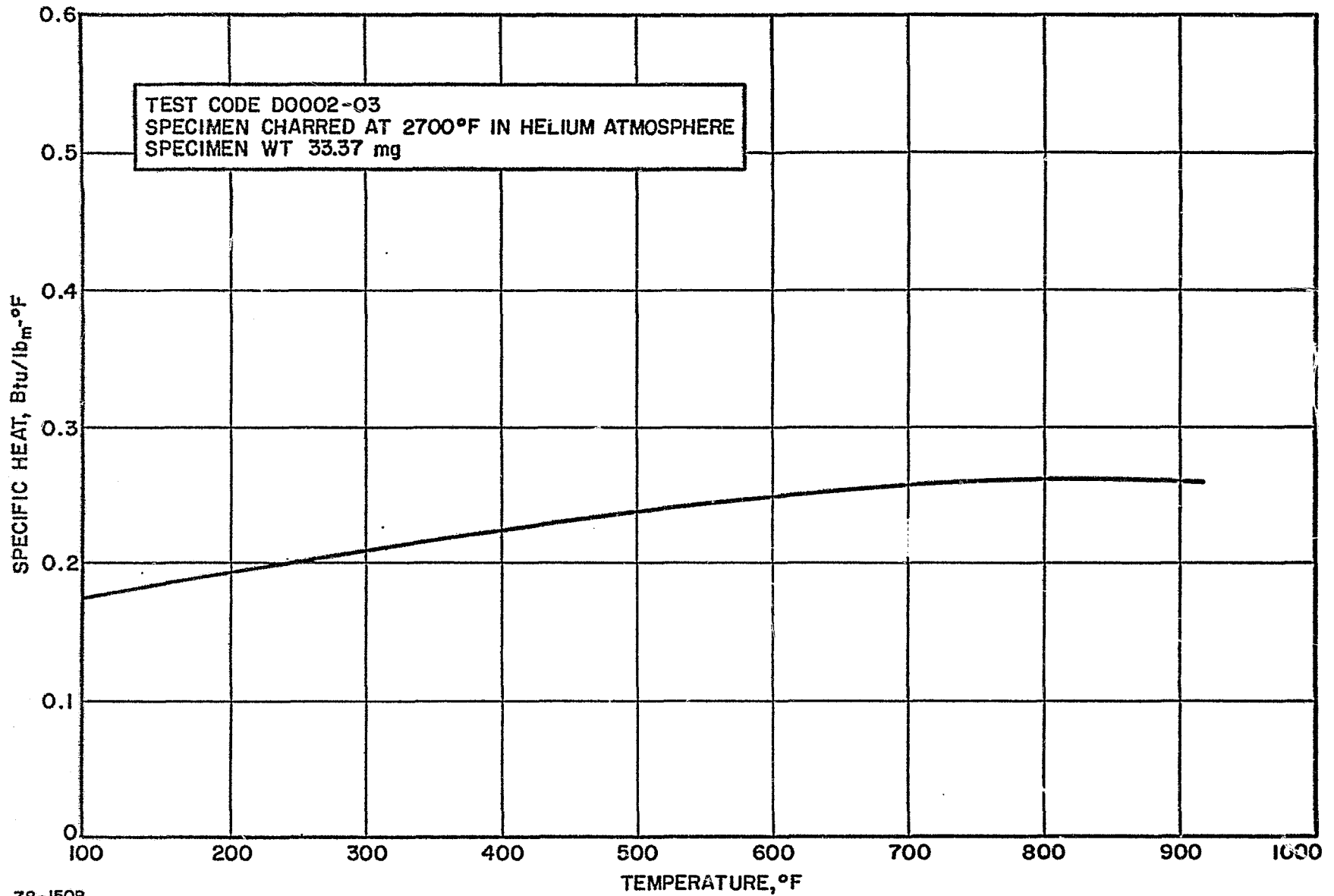
Figure 60 SILICA-PHENOLIC MXS-89, 2700°F PRECHARRED, SPECIFIC HEAT VERSUS TEMPERATURE
