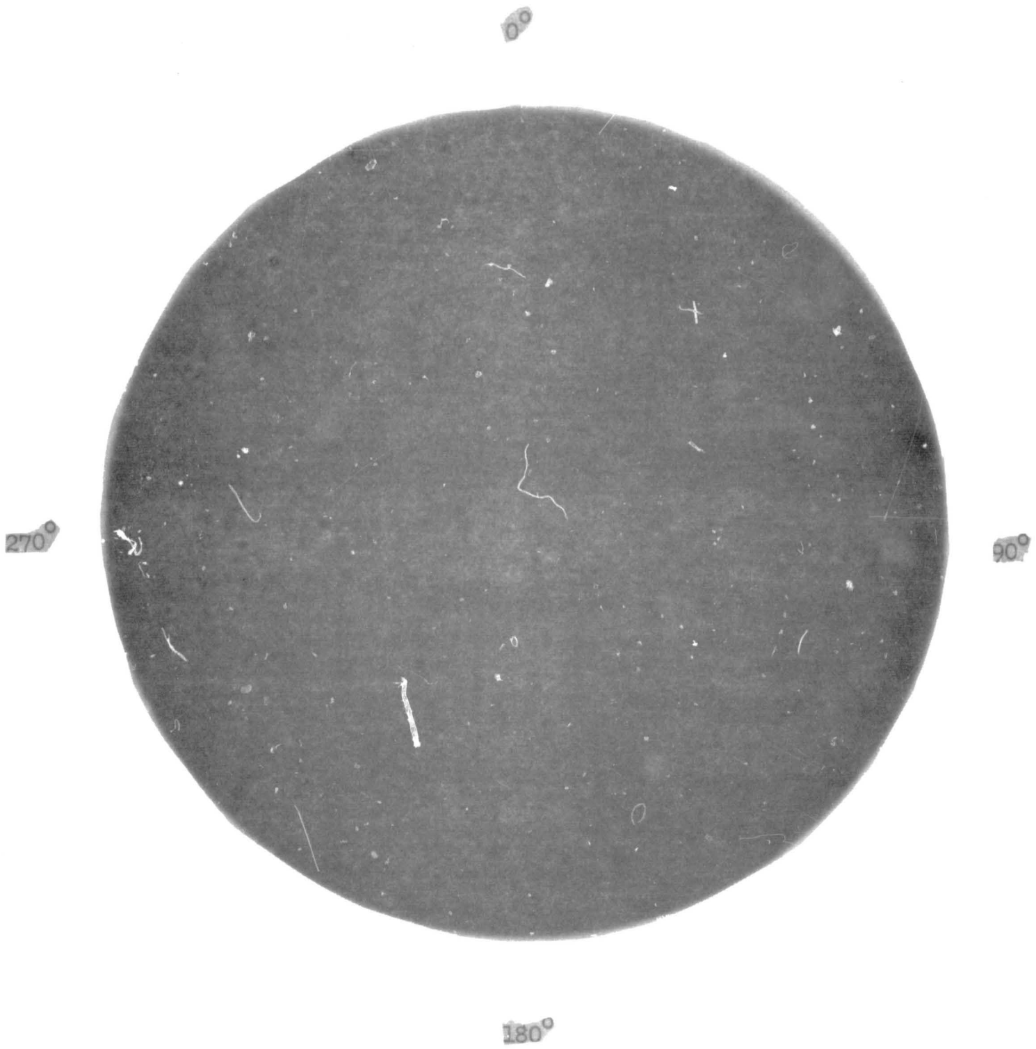
Figure A-1 AXIAL RADIOGRAPH OF SILICA FABRIC/PHENOLIC BILLET
