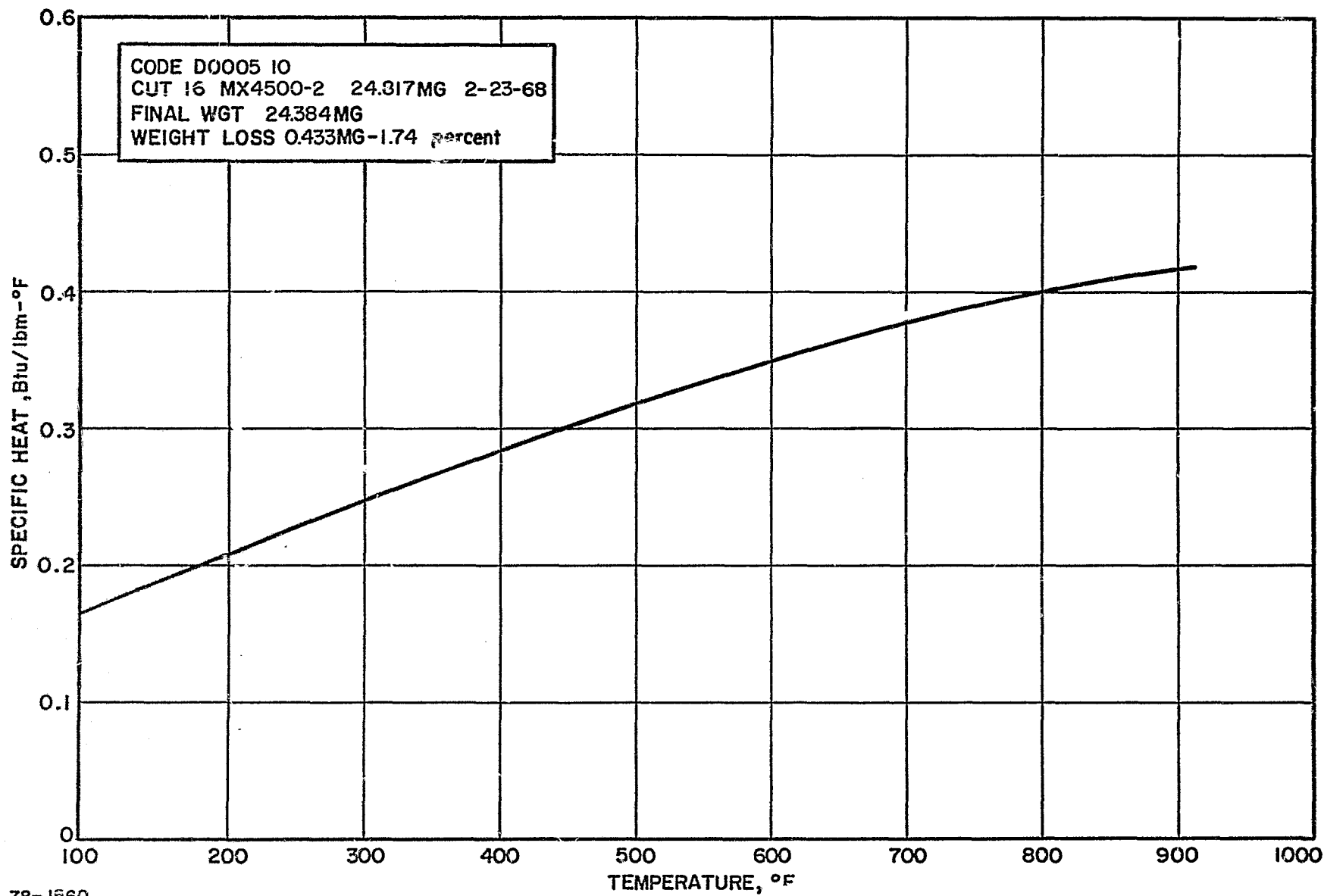
Figure 117 GRAPHITE-PHENOLIC NOZZLE EXIT, 1.276-INCH CHAR LAYER, SPECIFIC HEAT VERSUS TEMPERATURE
