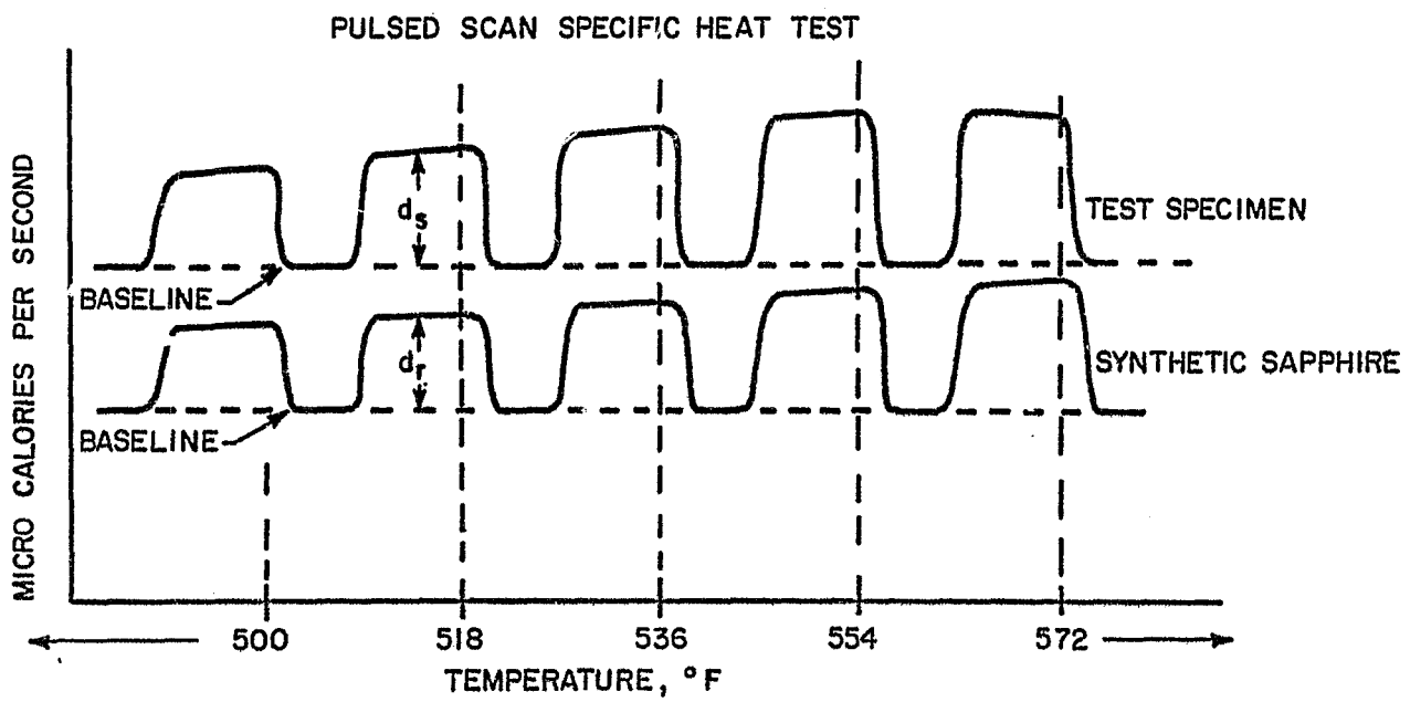
Figure D-6 TYPICAL DIFFERENTIAL SCAN CALORIMETER TRACES
