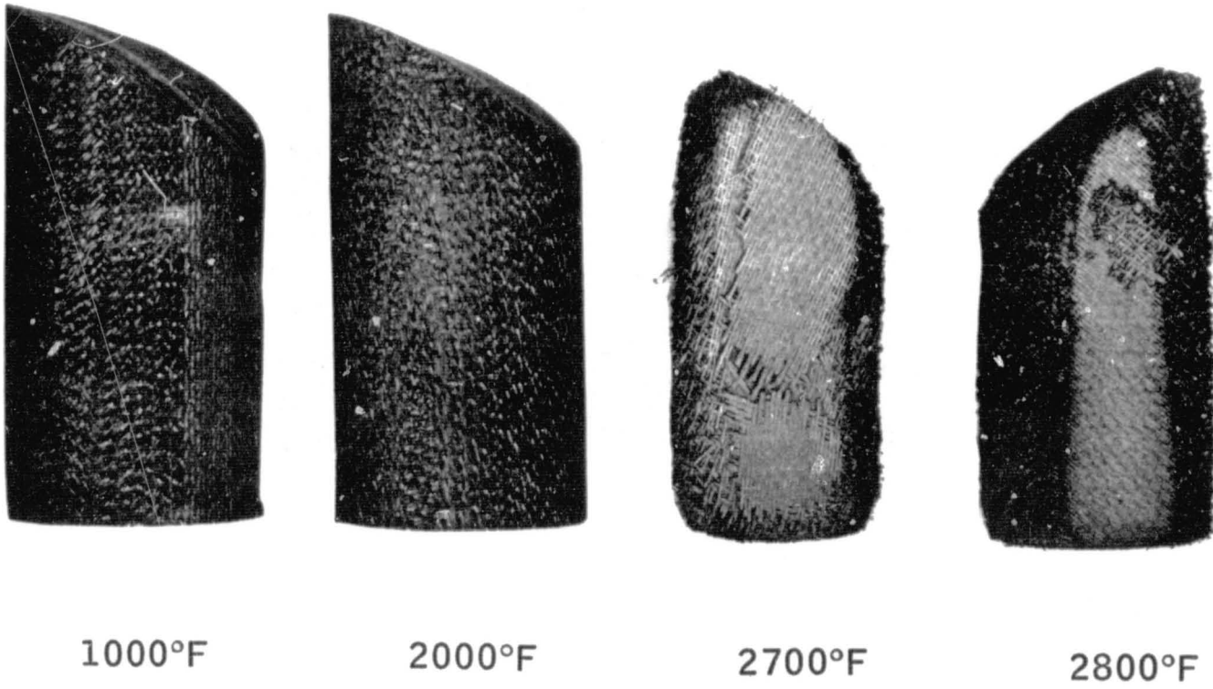
Figure 8 OVEN-CHARRED SILICA-PHENOLIC MXS-89 CORINGS (1X MAGNIFICATION)
