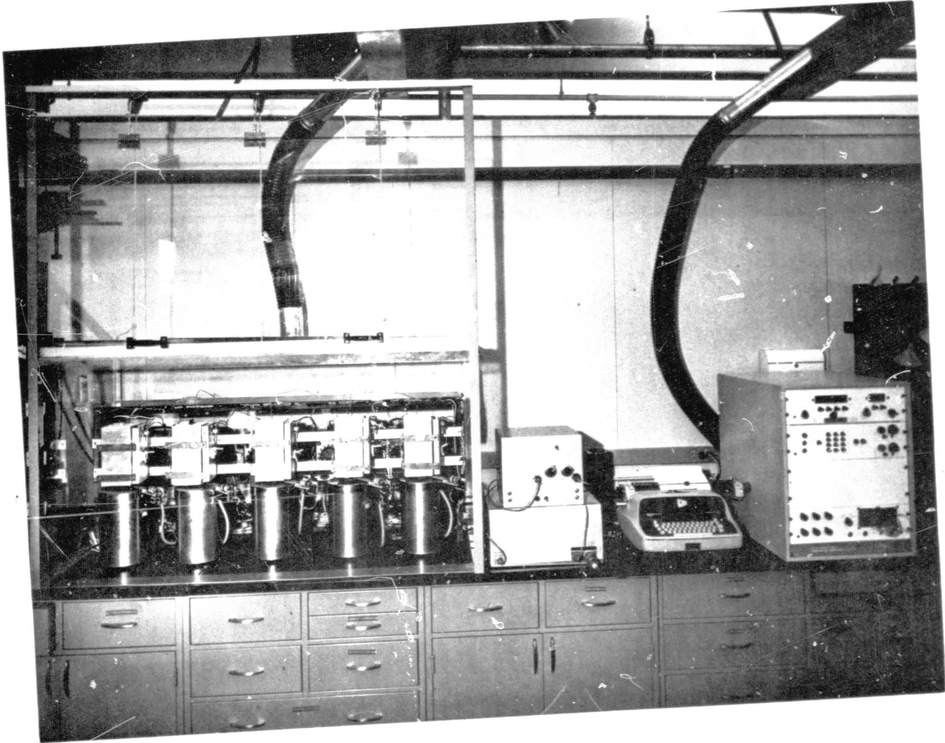
Figure D-1 AUTOMATIC SPECIFIC HEAT APPARATUS
