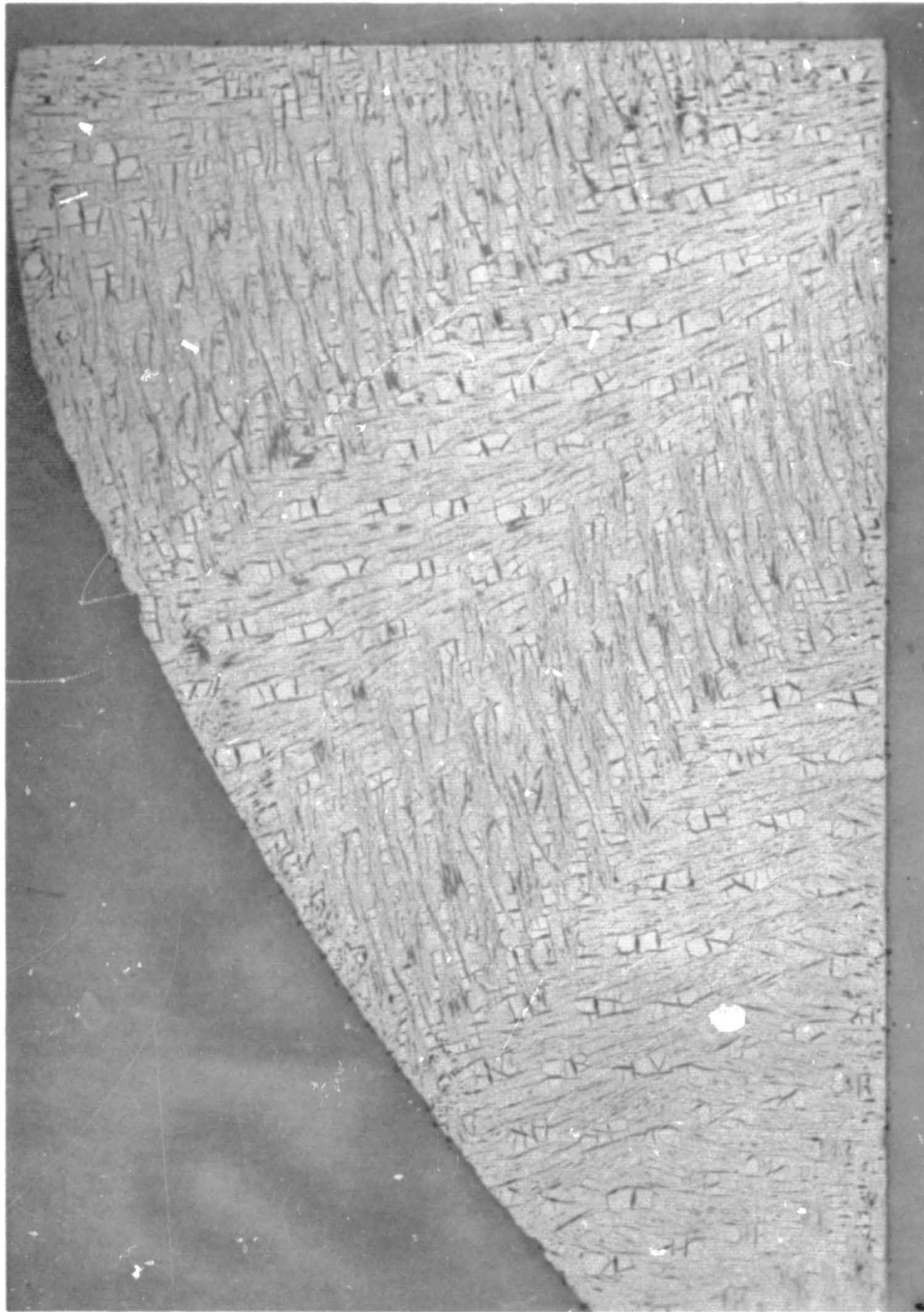
Figure 20 2000°F OVEN-CHARRED GRAPHITE-PHENOLIC MX4501 CORING (5X MAGNIFICATION)
