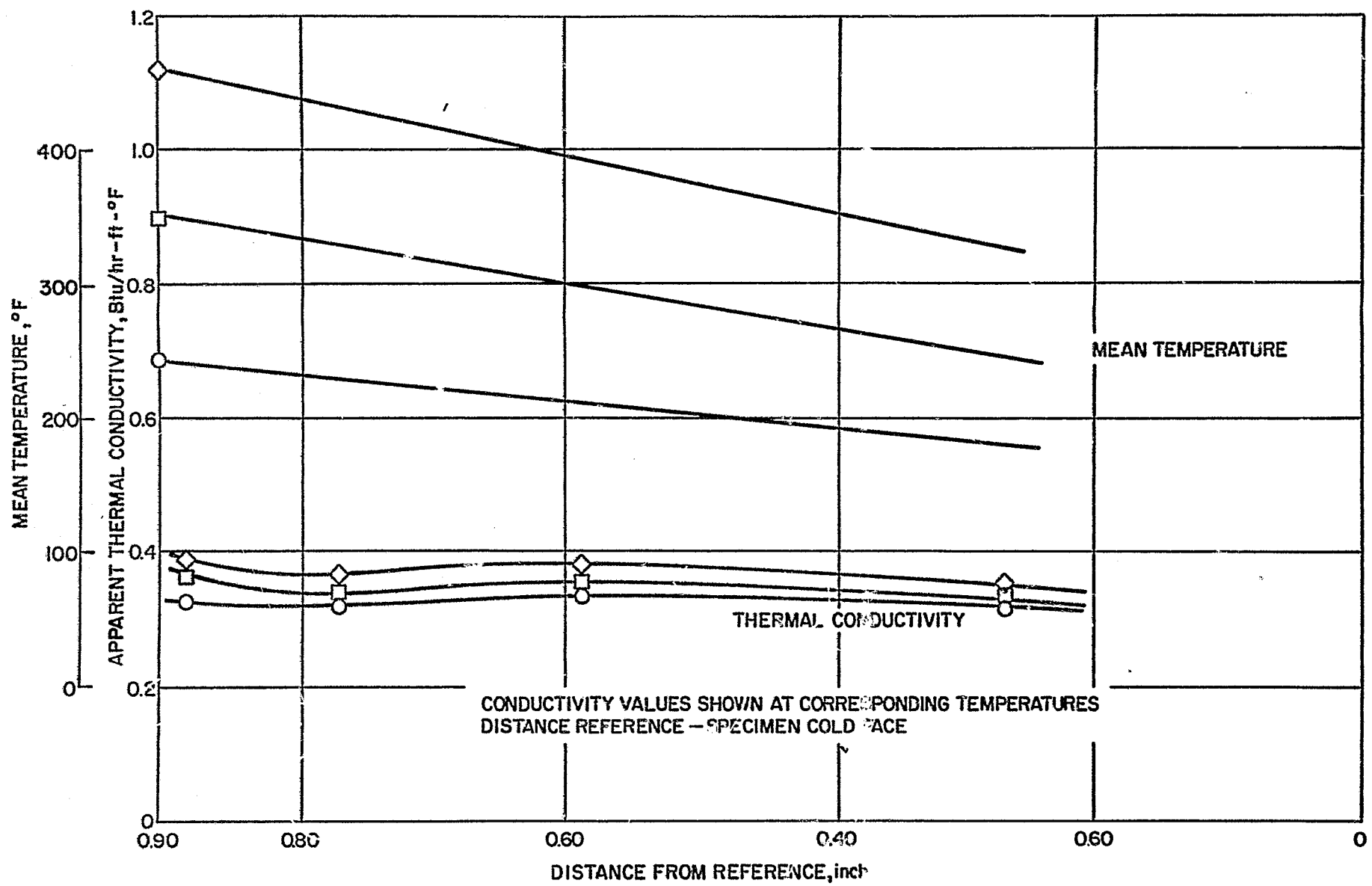
Figure 45 SILICA-PHENOLIC BILLET MXS-89 THERMAL CONDUCTIVITY PROFILE
