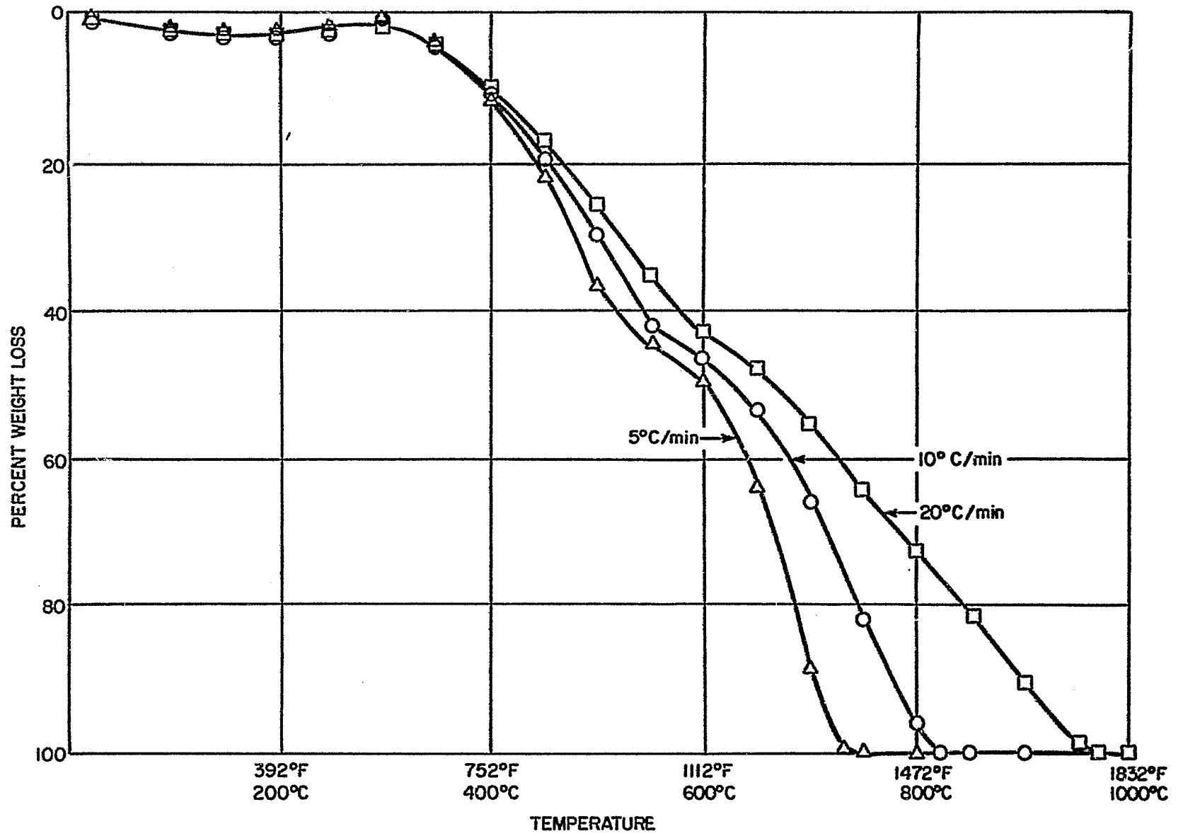
Figure 36 TGA CURVES FOR GRAPHITE-PHENOLIC IN AIR
