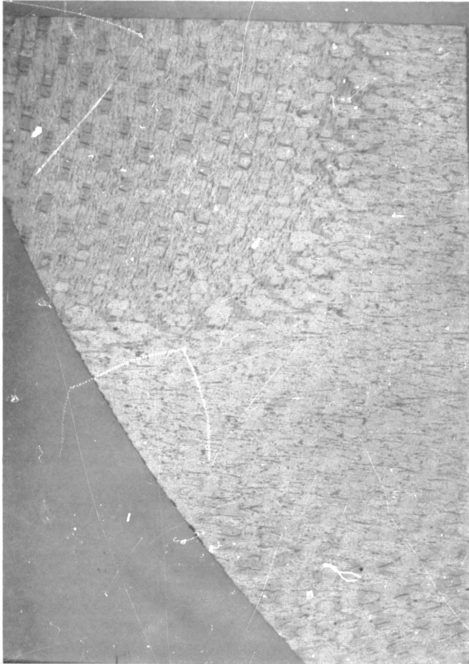
Figure 19 1000°F OVEN-CHARRED GRAPHITE-PHENOLIC MX4501 CORING (5X MAGNIFICATION)
