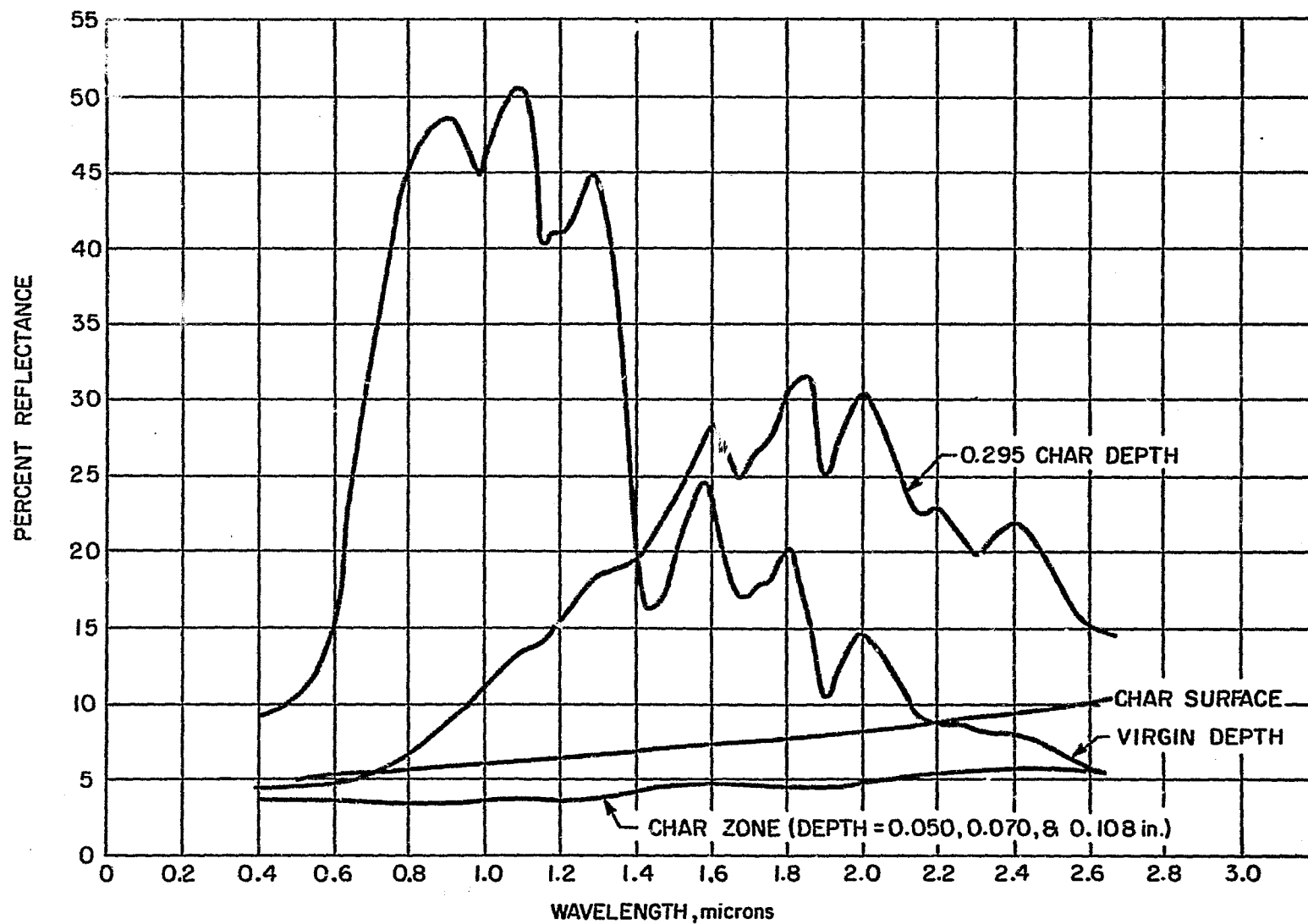
Figure 91 MXS-89 SILICA-PHENOLIC NOZZLE CHAR OPTICAL PROPERTIES
