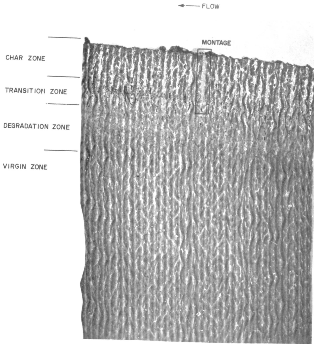
Figure 70 CUTAWAY VIEW OF SILICA-PHENOLIC MXS-89 THROAT SECTION OF POST-FIRED ROCKET NOZZLE (5X MAGNIFICATION)
