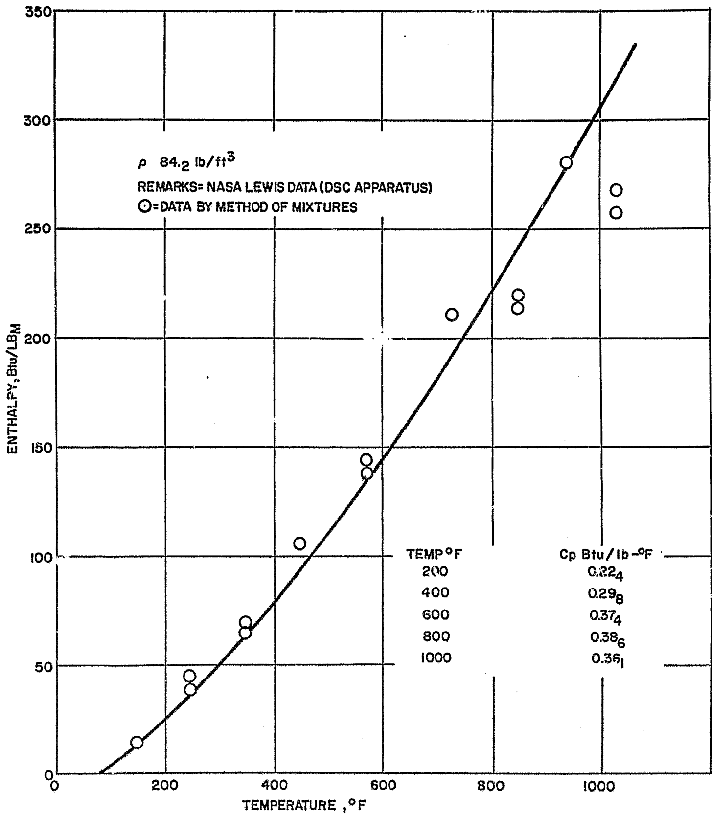
Figure 57 GRAPHITE-PHENOLIC BILLET MX4501, ENTHALPY VERSUS TEMPERATURE
