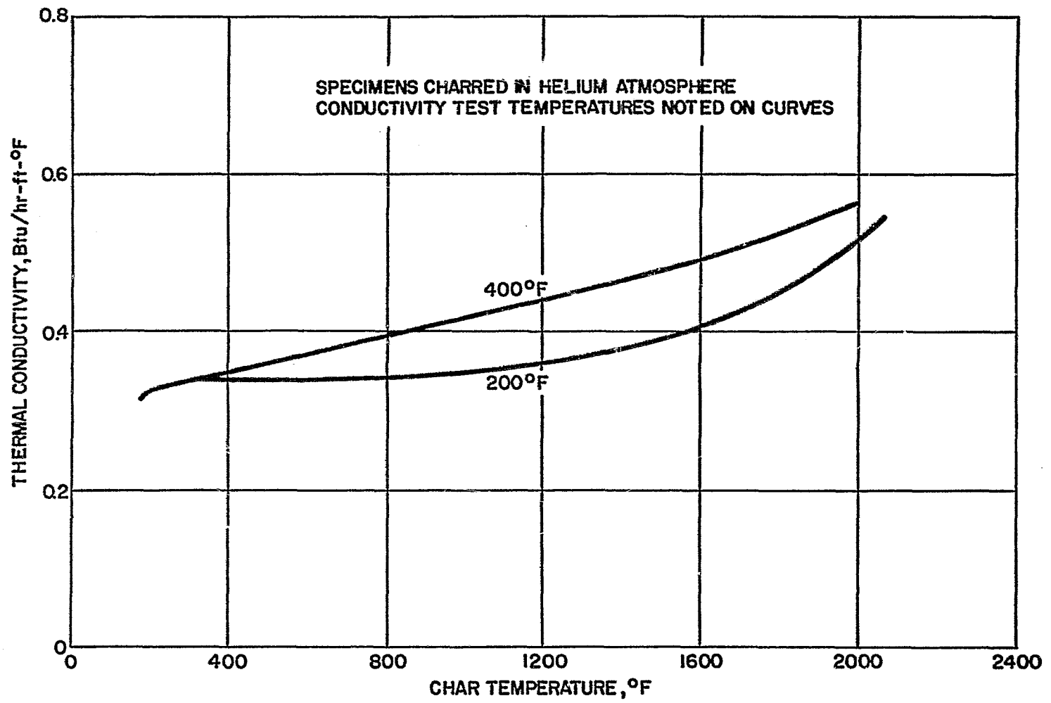
Figure 54 SILICA-PHENOLIC MXS-89, THERMAL CONDUCTIVITY (AT TEMPERATURE) VERSUS CHAR TEMPERATURE
