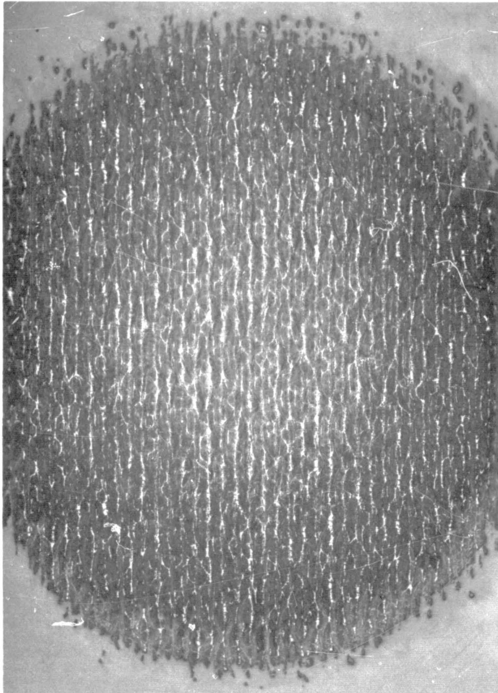
Figure 13 2800°F OVEN-CHARRED SILICA-PHENOLIC MXS-89 CORING (5X MAGNIFICATION)
