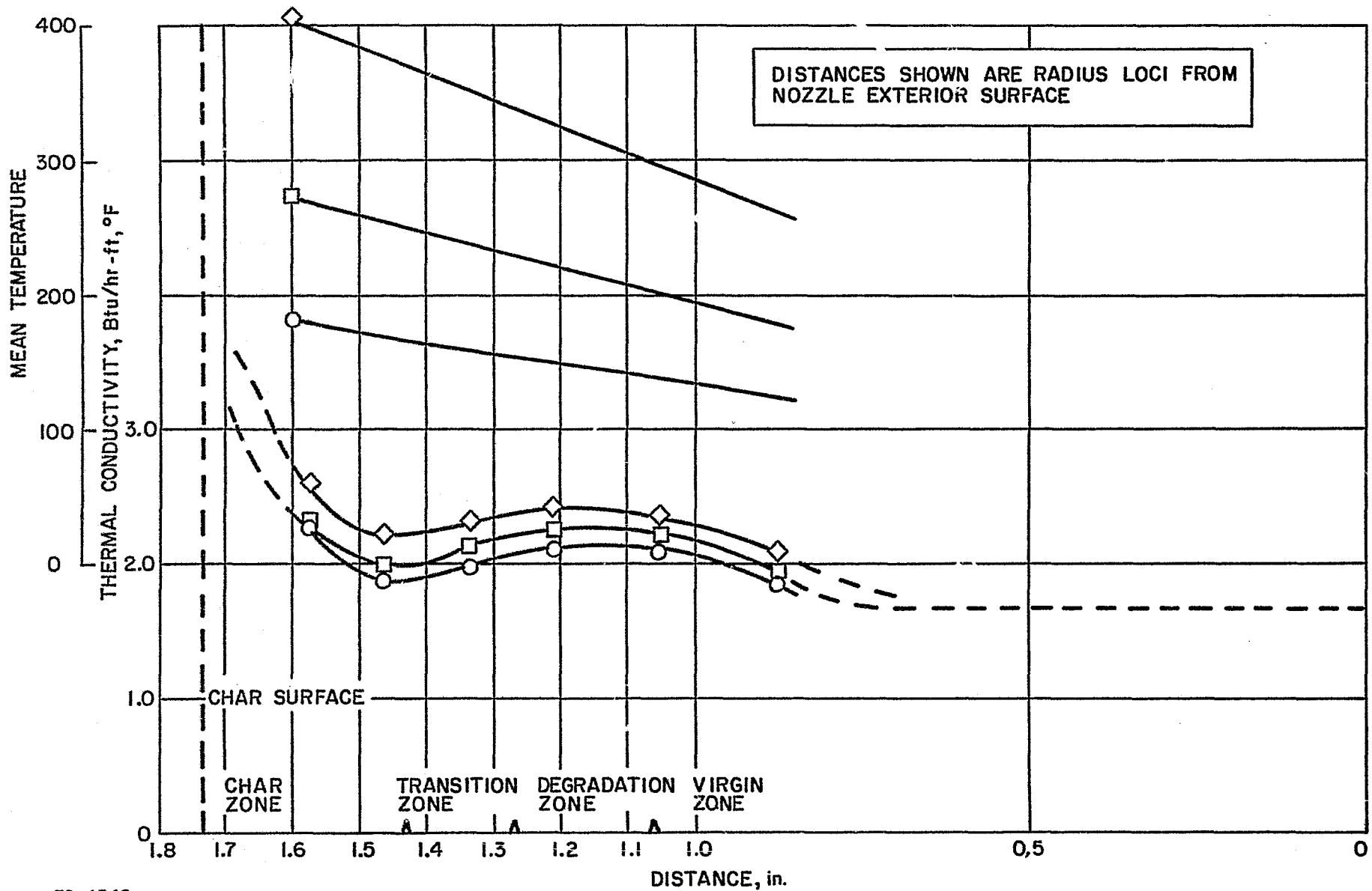
Figure 97 GRAPHITE-PHENOLIC NOZZLE EXIT, THERMAL CONDUCTIVITY VERSUS CHAR DEPTH
