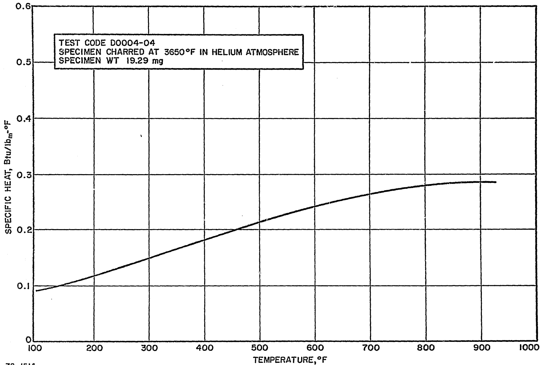
Figure 66 GRAPHITE PHENOLIC MX4501, 3650°F PRECHARRED, SPECIFIC HEAT VERSUS TEMPERATURE
