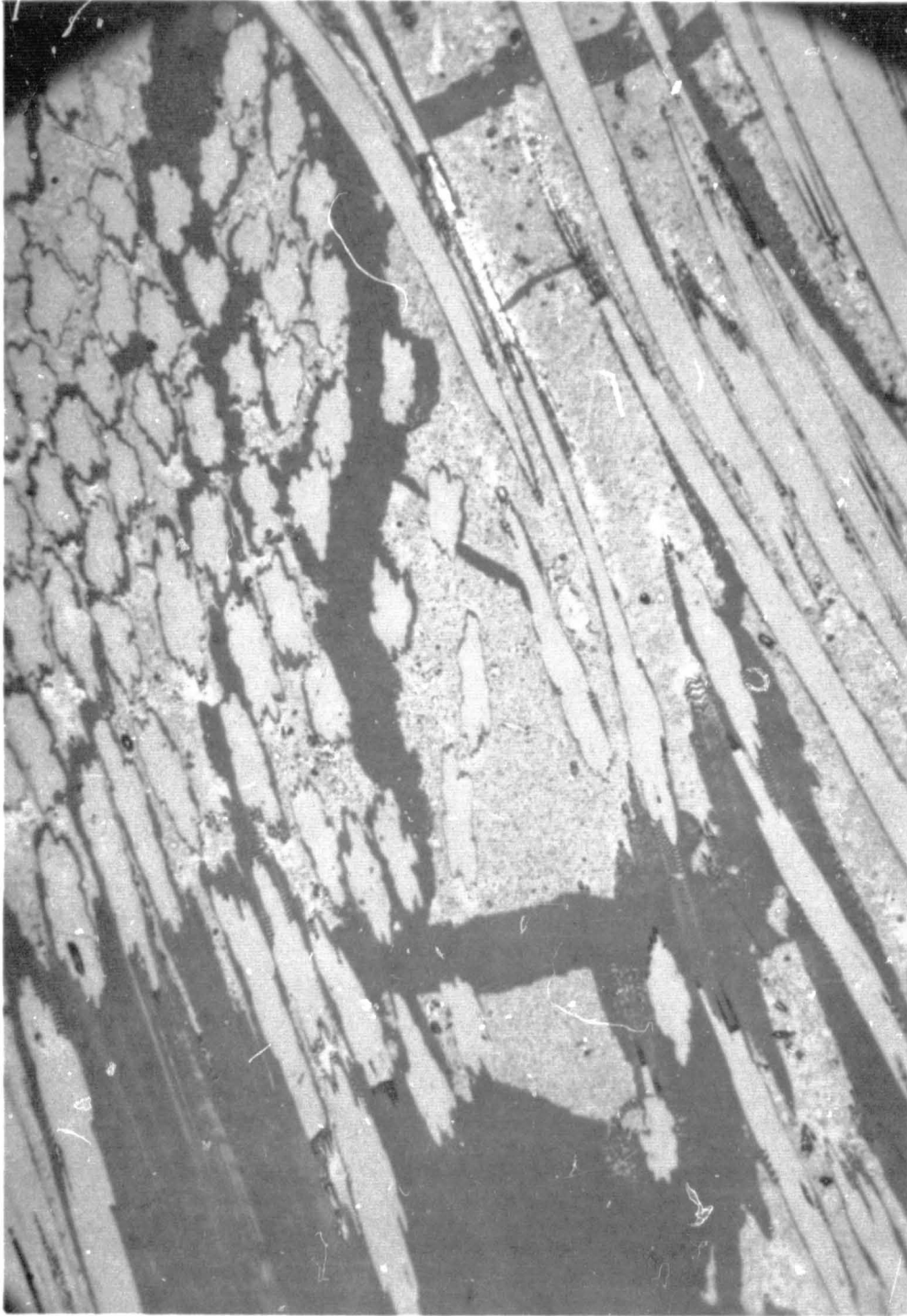
Figure 27 3650°F OVEN-CHARRED GRAPHITE-PHENOLIC MX4501 CORING (500X MAGNIFICATION)
