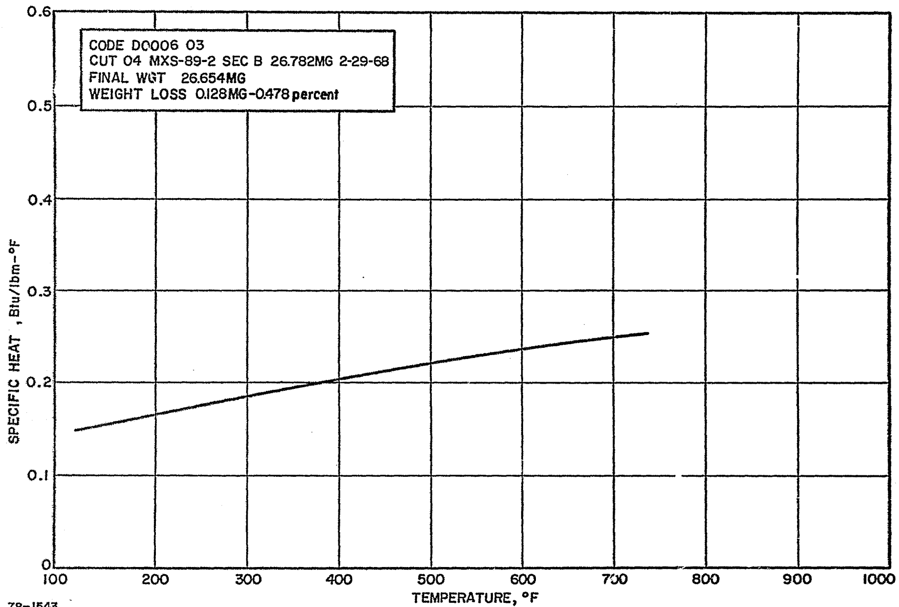
Figure 100 SILICA-PHENOLIC NOZZLE THROAT, 1.656-INCH CHAR LAYER, SPECIFIC HEAT VERSUS TEMPERATURE
