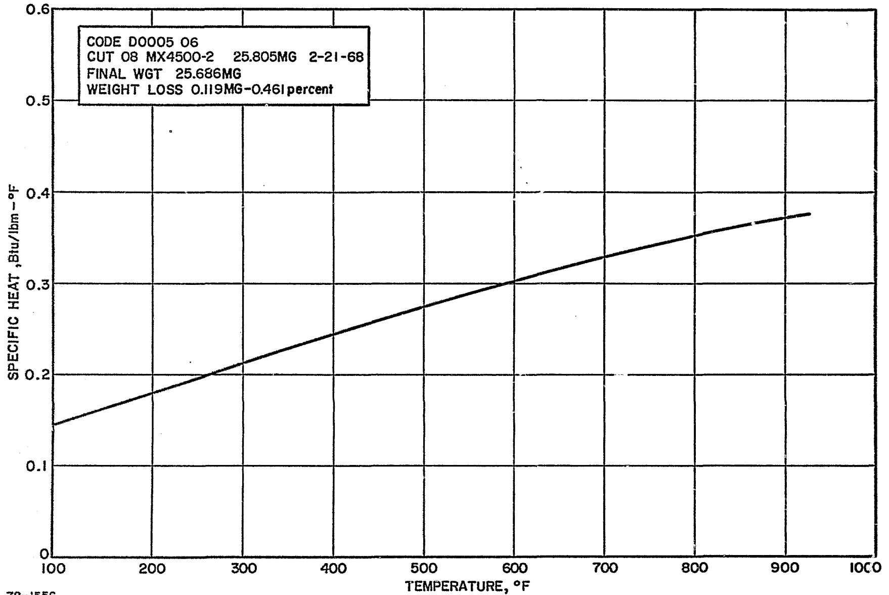
Figure 113 GRAPHITE-PHENOLIC NOZZLE EXIT, 1.483-INCH CHAR LAYER, SPECIFIC HEAT VERSUS TEMPERATURE
