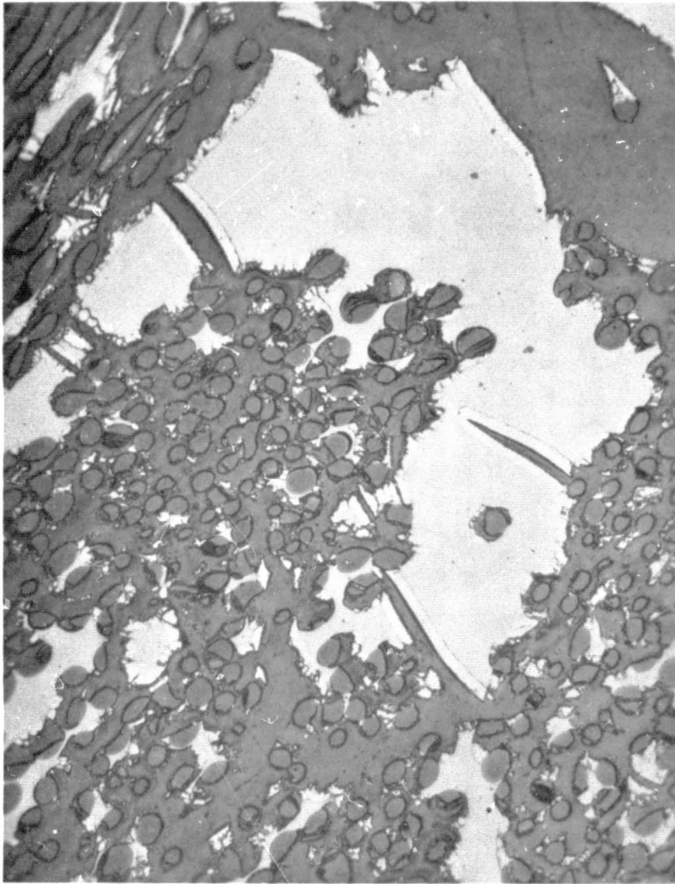
Figure 16 2700°F OVEN-CHARRED SILICA-PHENOLIC MXS-89 CORING (500X MAGNIFICATION)
