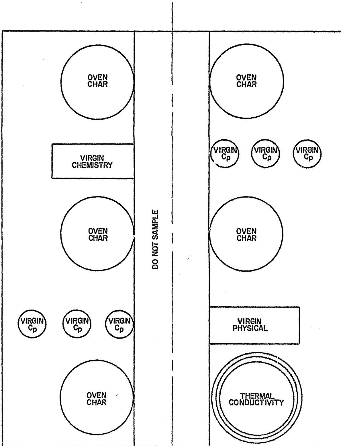
Figure 5 BILLET MATERIAL TEST SPECIMEN LAYOUT
