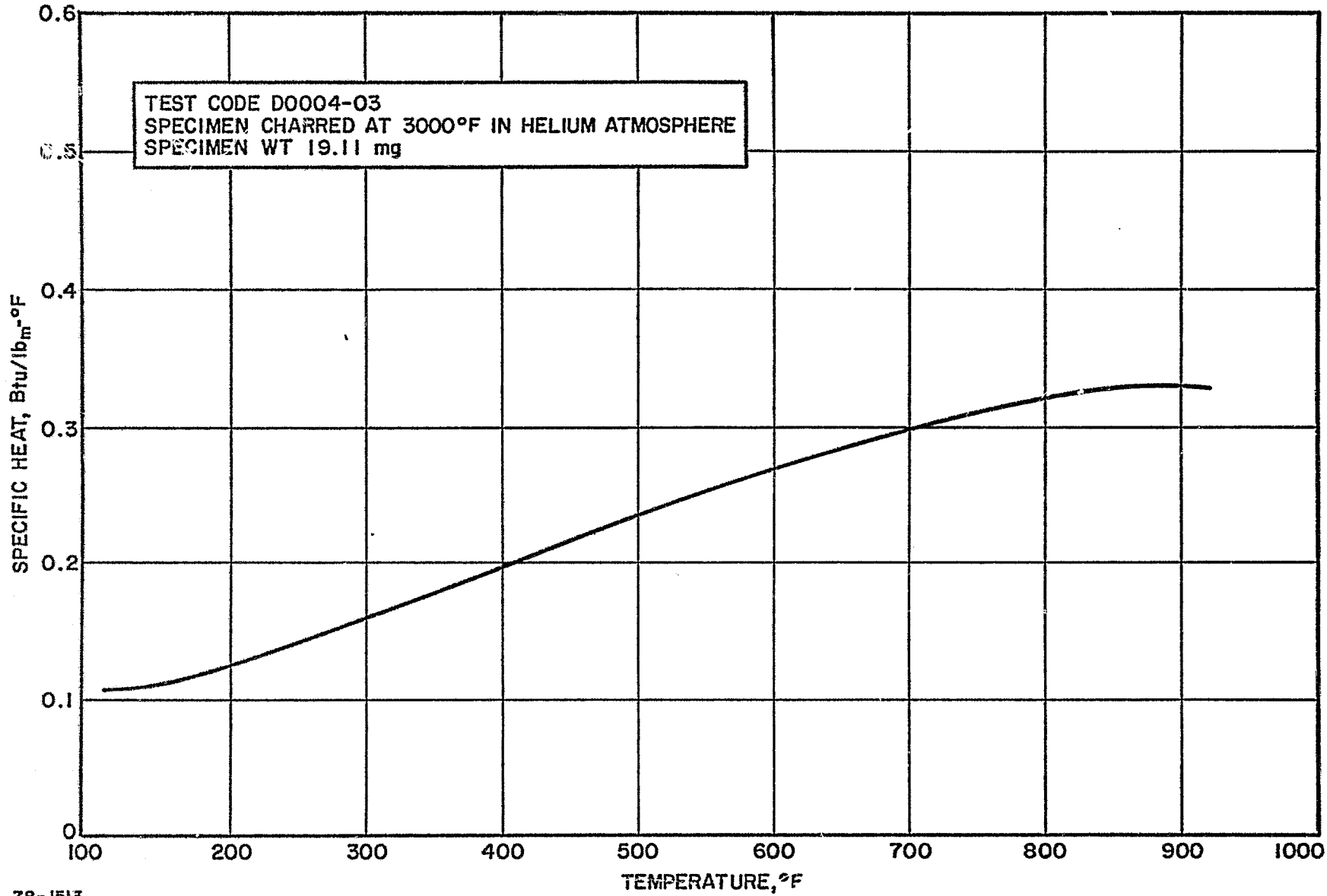
Figure 65 GRAPHITE-PHENOLIC MX4501, 3000°F PRECHARRED, SPECIFIC HEAT VERSUS TEMPERATURE
