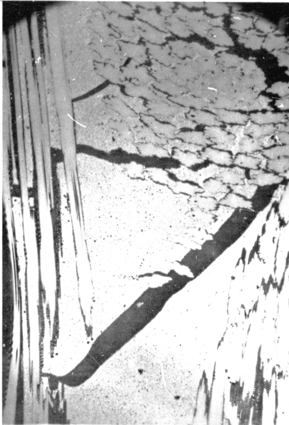
Figure 25 2000°F OVEN-CHARRED GRAPHITE-PHENOLIC MX4501 CORING (500X MAGNIFICATION)
