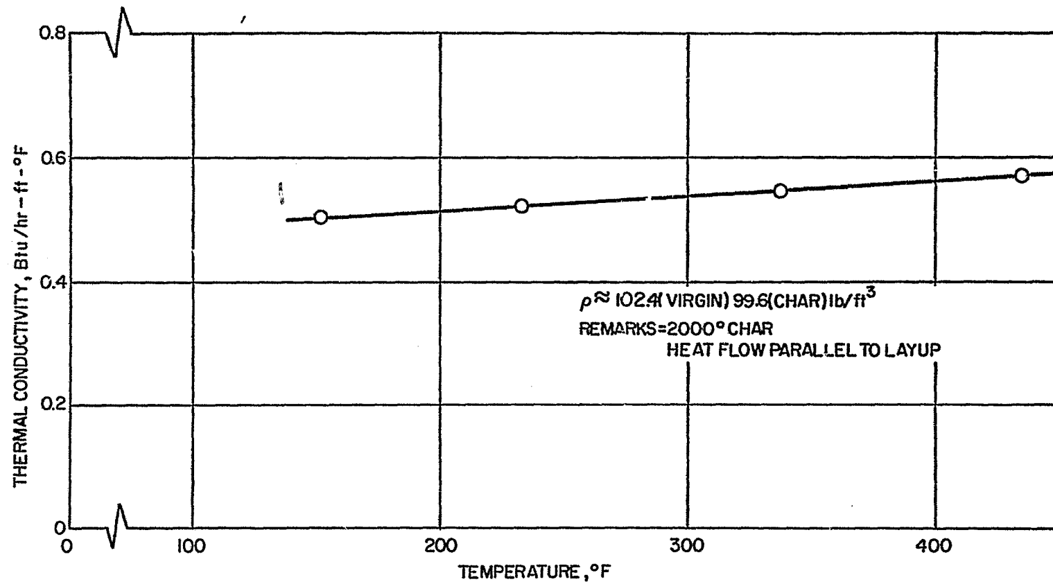
Figure 48 SILICA-PHENOLIC MXS-89, 2000°F PRECHARRED, THERMAL CONDUCTIVITY VERSUS TEMPERATURE
