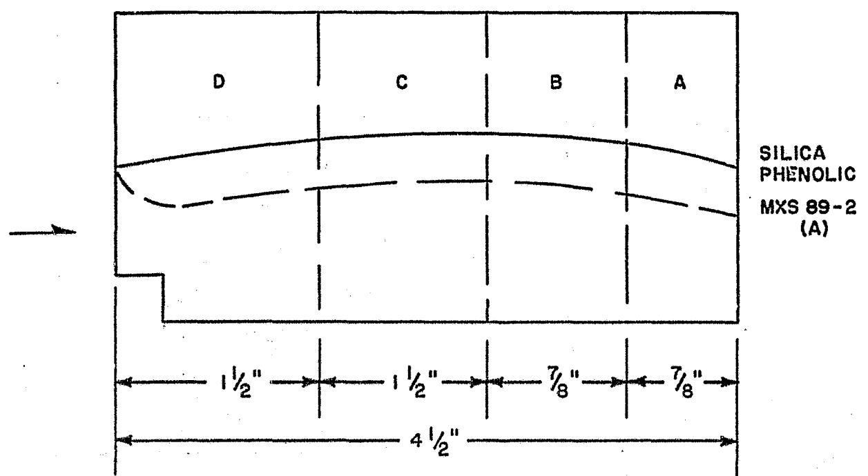
Figure 6 NOZZLE SECTION IDENTIFICATION
