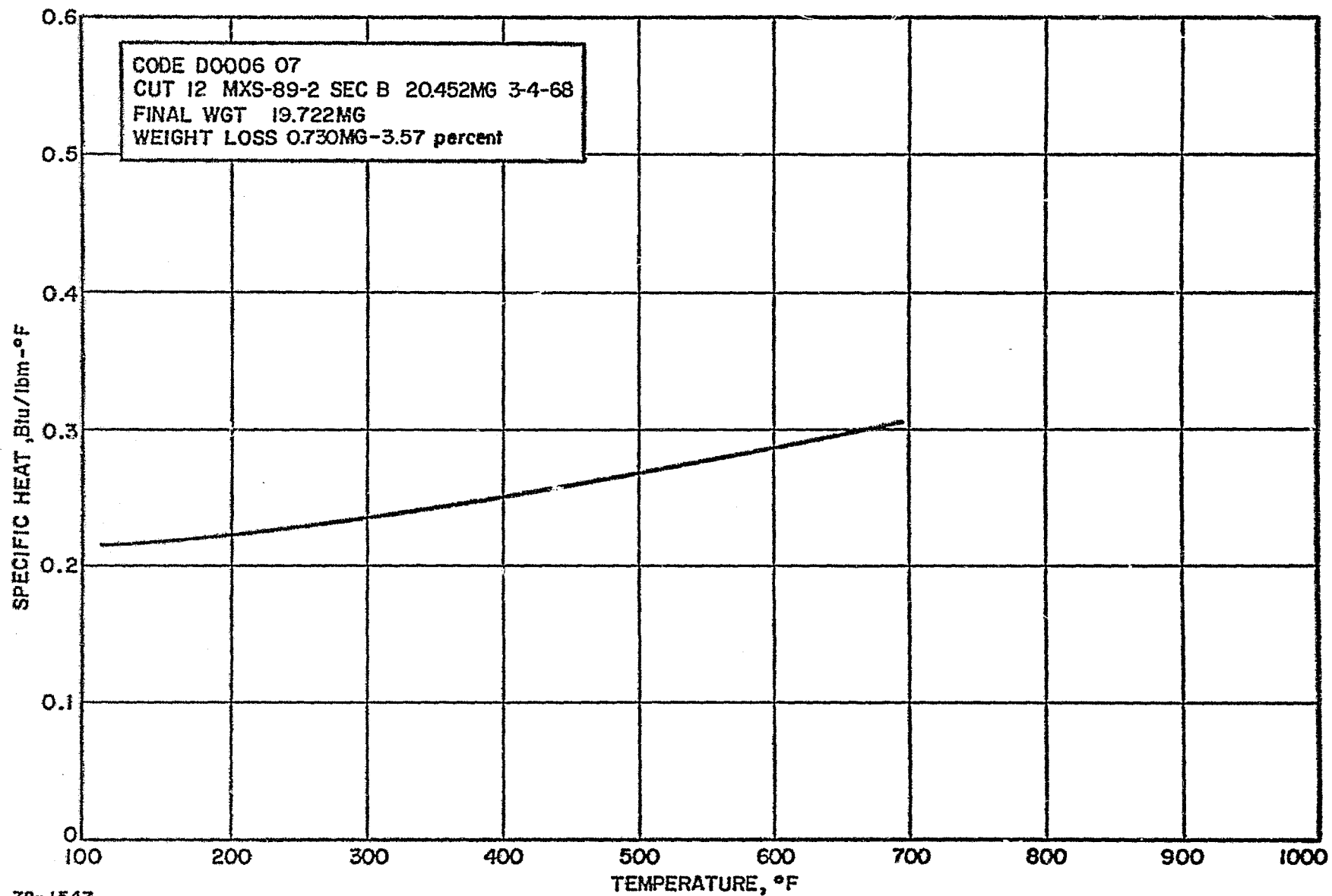
Figure 104 SILICA-PHENOLIC NOZZLE THROAT, 1.451-INCH CHAR LAYER, SPECIFIC HEAT VERSUS TEMPERATURE
