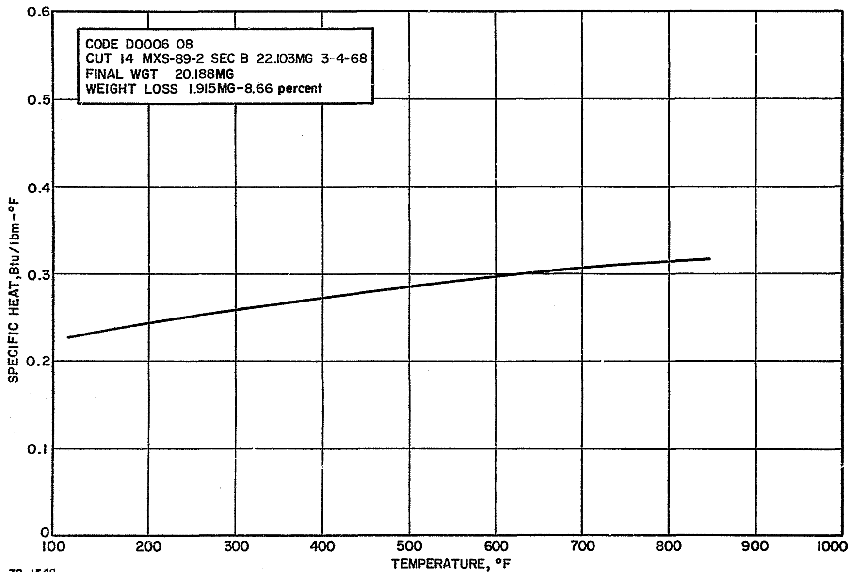
Figure 105 SILICA PHENOLIC NOZZLE THROAT, 1.404-INCH CHAR LAYER, SPECIFIC HEAT VERSUS TEMPERATURE
