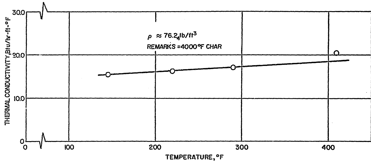
Figure 53 GRAPHITE-PHENOLIC MX4501, 4000°F PRECHARRED, THERMAL CONDUCTIVITY VERSUS TEMPERATURE
