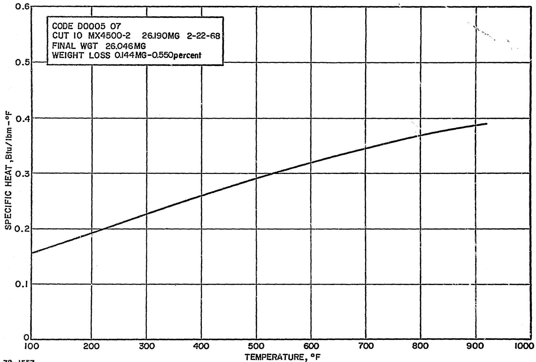
Figure 114 GRAPHITE-PHENOLIC NOZZLE EXIT, 1.433-INC-H CHAR LAYER, SPECIFIC HEAT VERSUS TEMPERATURE
