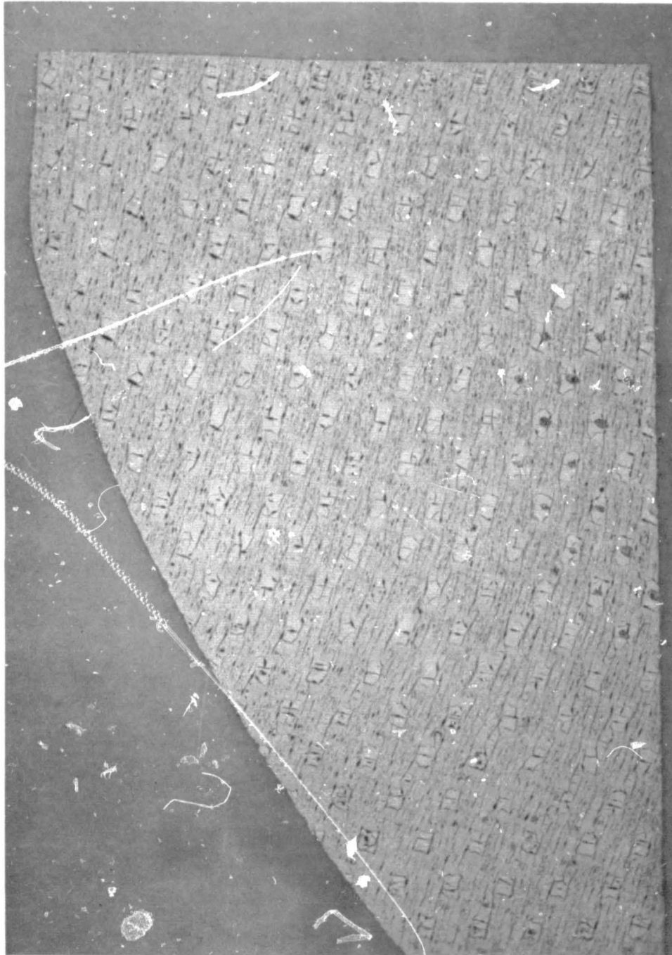
Figure 22 3650°F OVEN-CHARRED GRAPHITE-PHENOLIC MX4501 CORING (5X MAGNIFICATION)
