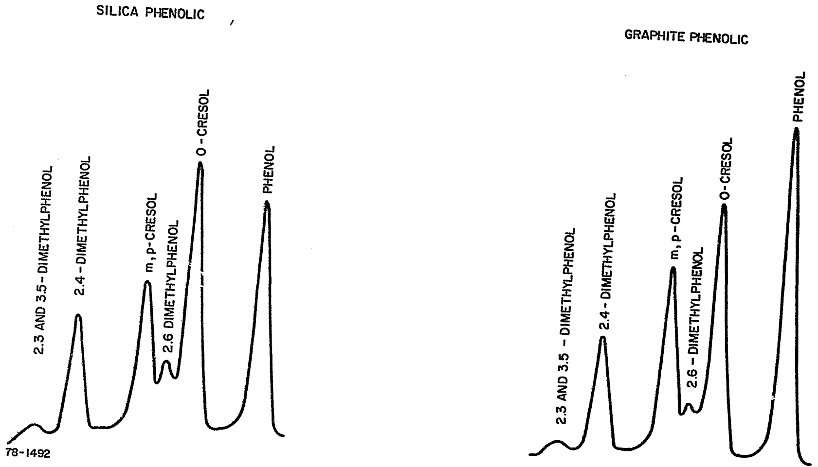
Figure 43 TYPICAL CHROMATOGRAMS OF HYDROXYL-CONTAINING AROMATIC COMPOUNDS YIELDED BY 600°C PYROLYSIS
