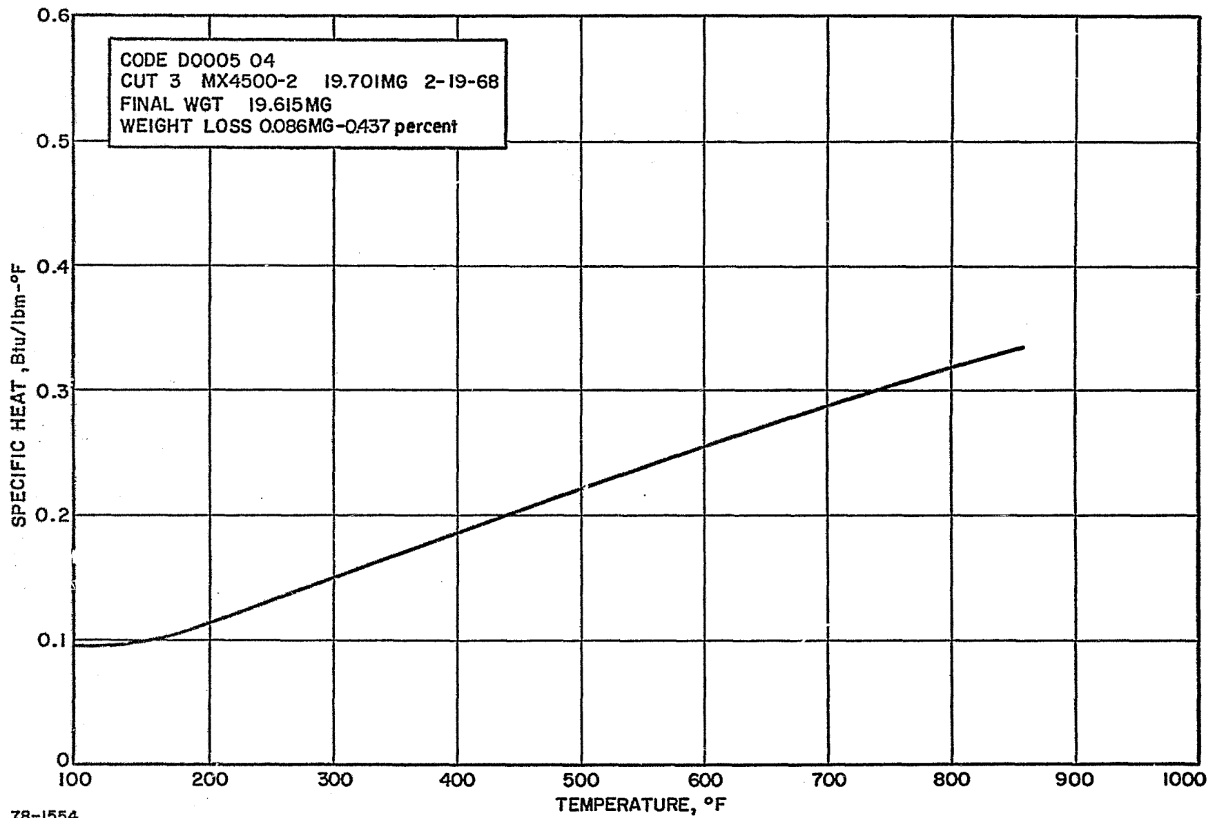
Figure 111 GRAPHITE-PHENOLIC NOZZLE EXIT, 1.627-INCH CHAR LAYER, SPECIFIC HEAT VERSUS TEMPERATURE
