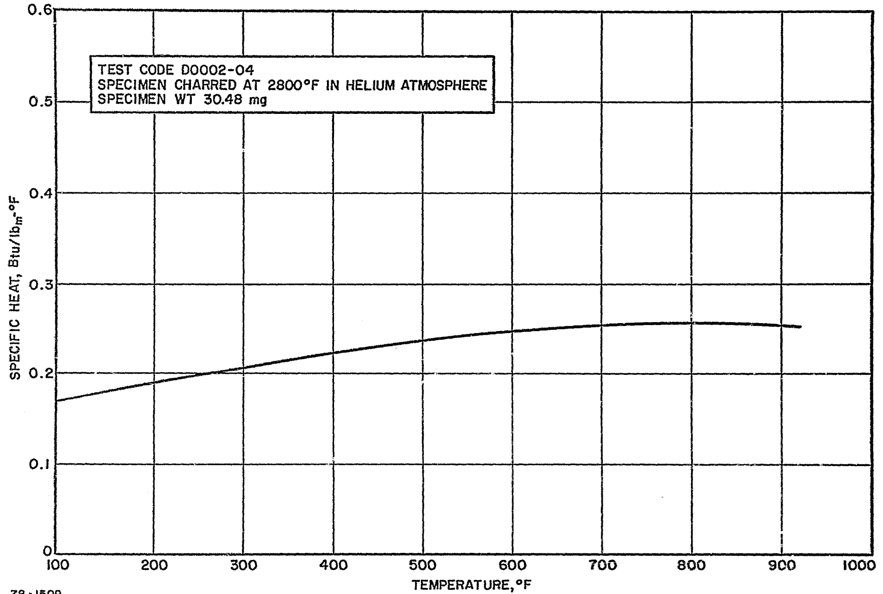
Figure 61 SILICA-PHENOLIC MXS-89, 2800°F PRECHARRED, SPECIFIC HEAT VERSUS TEMPERATURE
