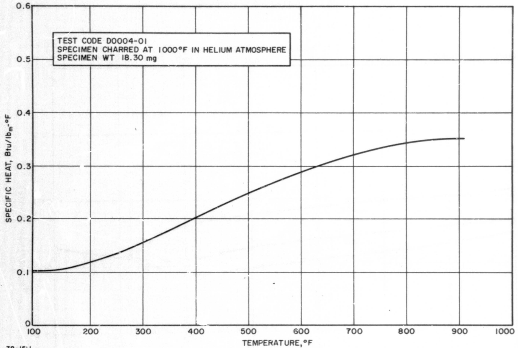
Figure 63 GRAPHITE-PHENOLIC MX4501, 1000°F PRECHARRED, SPECIFIC HEAT VERSUS TEMPERATURE
