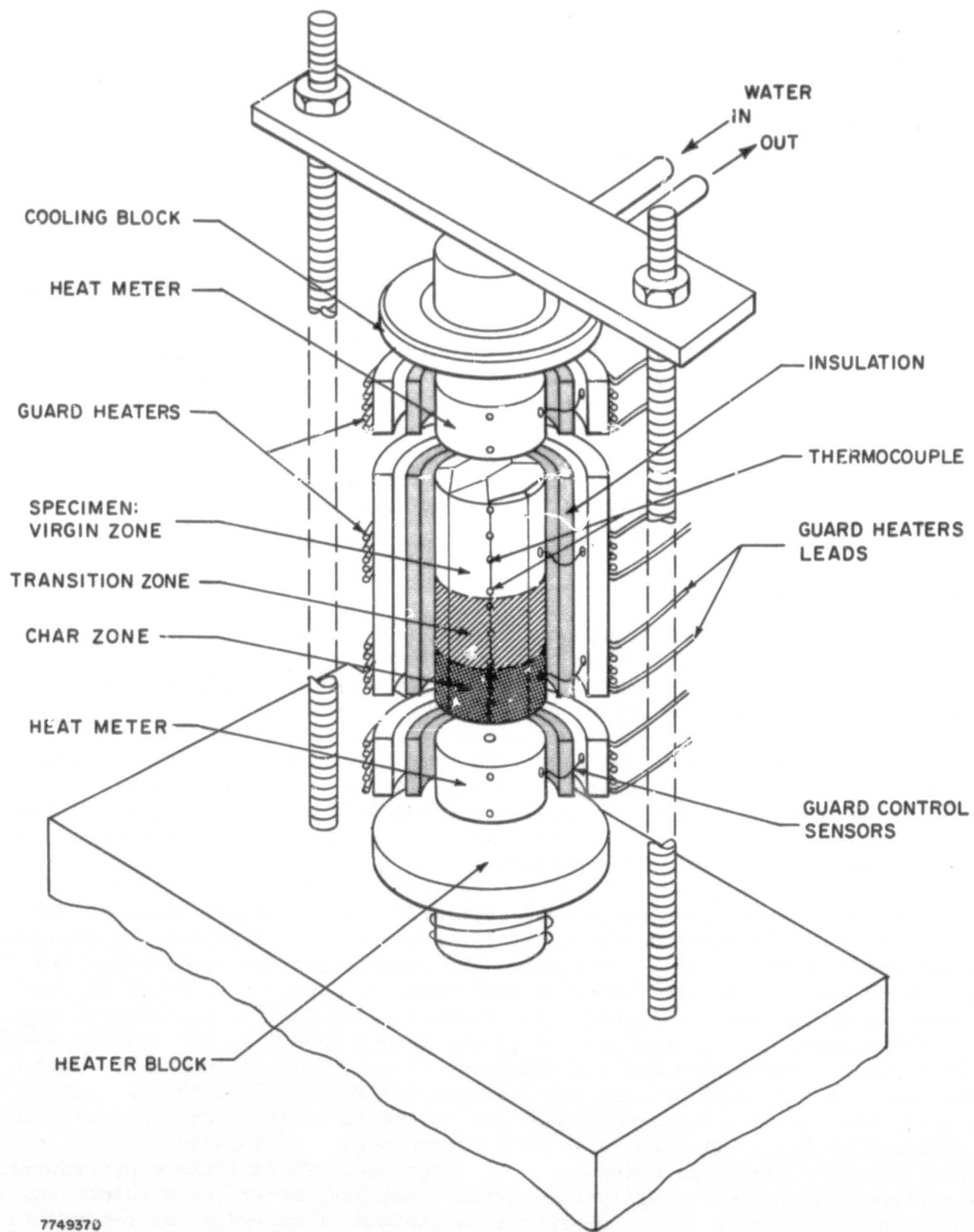
Figure C-5 MODIFIED CUT-BAR SCHEMATIC
