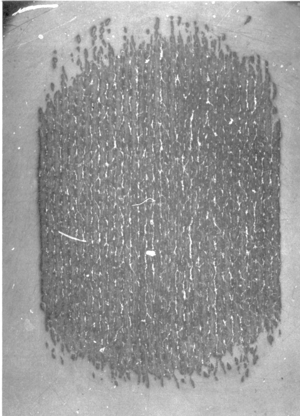
Figure 12 2700°F OVEN-CHARRED SILICA-PHENOLIC MXS-89 CORING (5X MAGNIFICATION)
