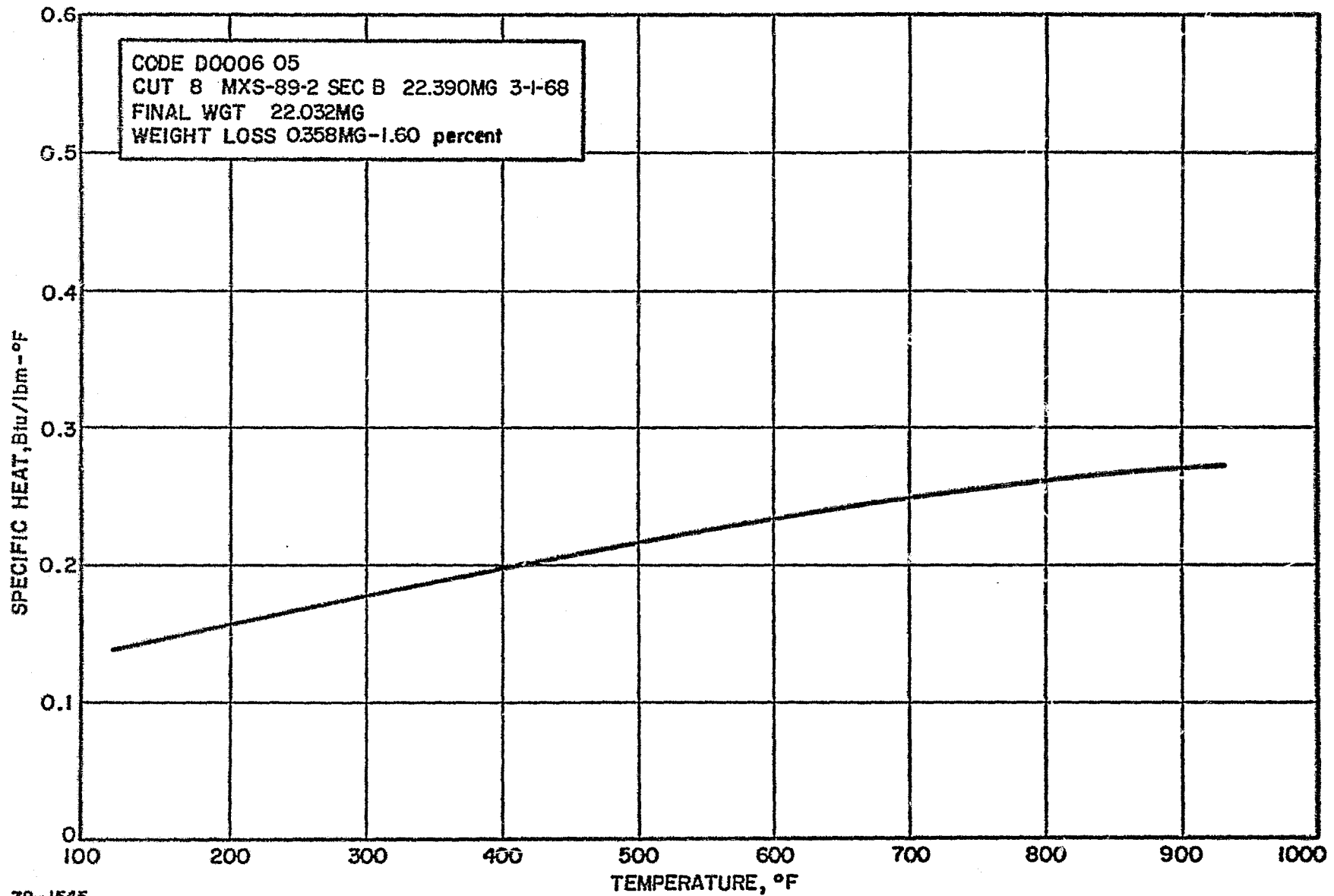
Figure 102 SILICA-PHENOLIC NOZZLE THROAT, 1.552-INCH CHAR LAYER, SPECIFIC HEAT VERSUS TEMPERATURE
