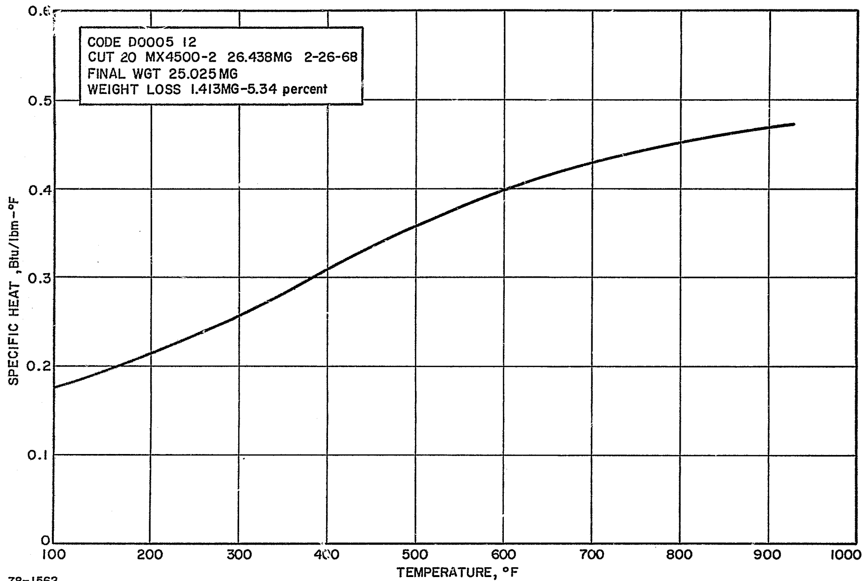
Figure 119 GRAPHITE-PHENOLIC NOZZLE EXIT, 1.178-INCH CHAR LAYER, SPECIFIC HEAT VERSUS TEMPERATURE
