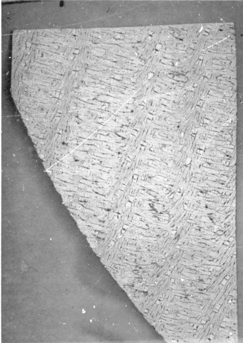
Figure 21 3000°F OVEN-CHARRED GRAPHITE-PHENOLIC MX4501 CORING (5X MAGNIFICATION)
