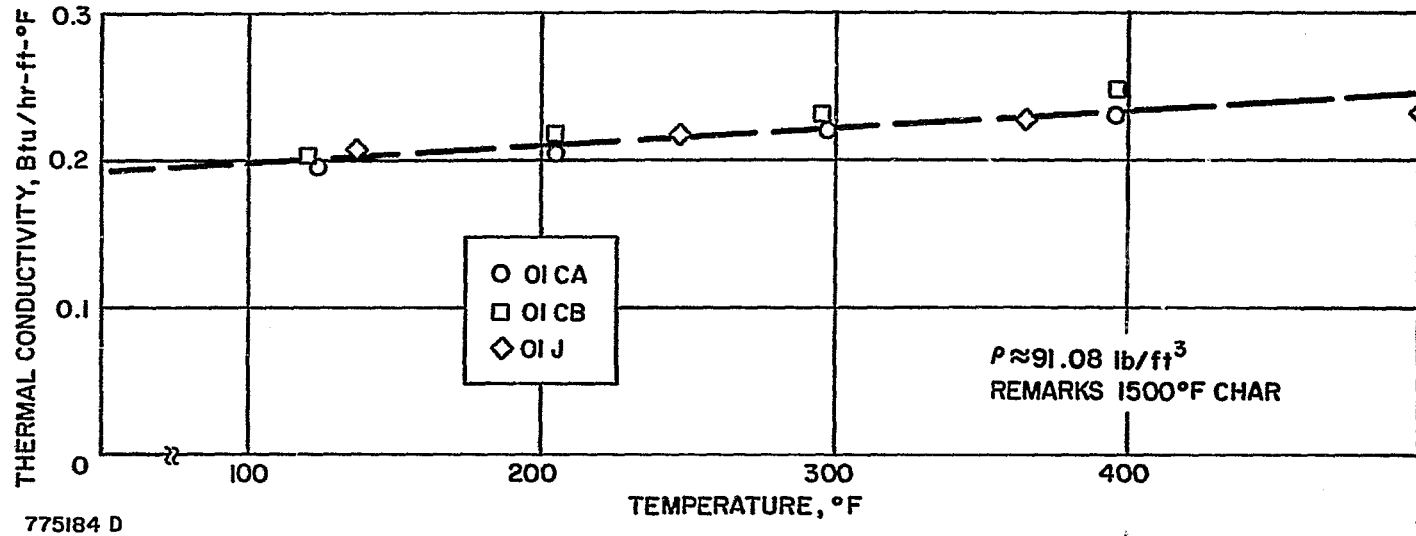
Figure C-2 THERMAL CONDUCTIVITY VERSUS TEMPERATURE FOR OTWR
