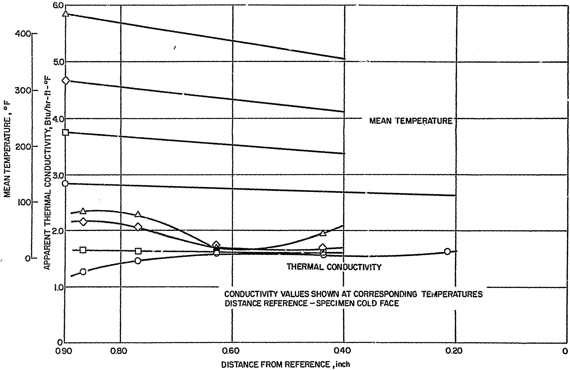
Figure 46 GRAPHITE-PHENOLIC BILLET MX4501 THERMAL CONDUCTIVITY PROFILE
