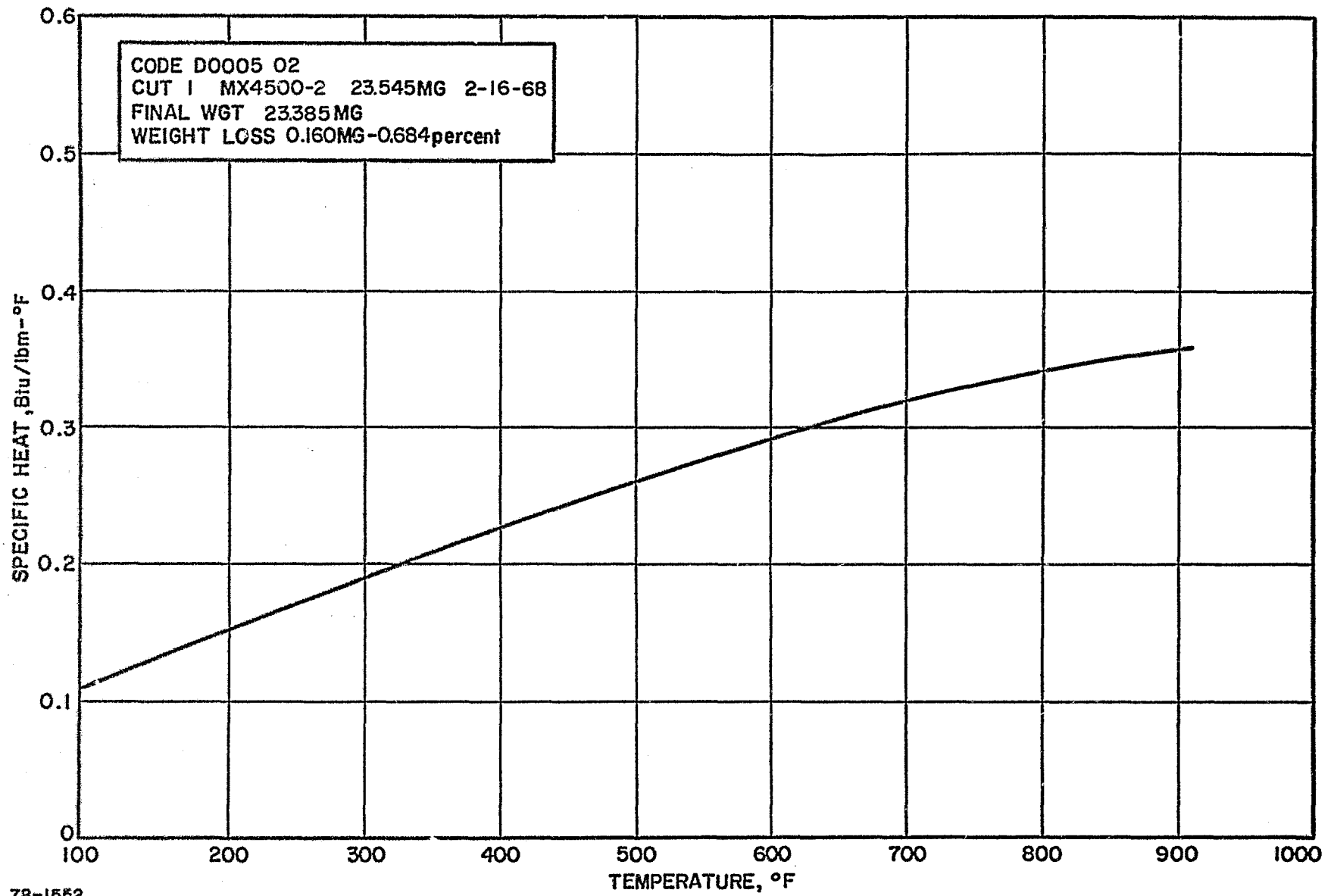
Figure 109 GRAPHITE-PHENOLIC NOZZLE EXIT, 1.678-INCH CHAR LAYER, SPECIFIC HEAT VERSUS TEMPERATURE
