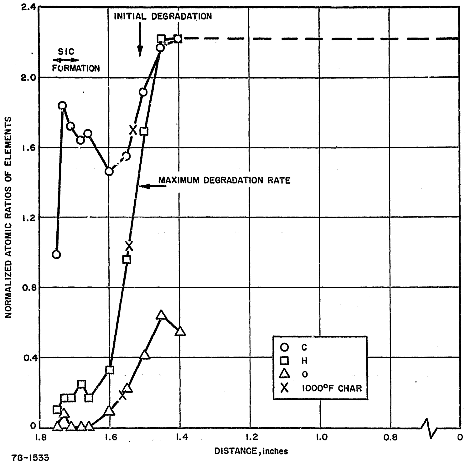
Figure 88 CHEMISTRY PROFILE OF THE SILICA-PHENOLIC NOZZLE MXS-89-2
