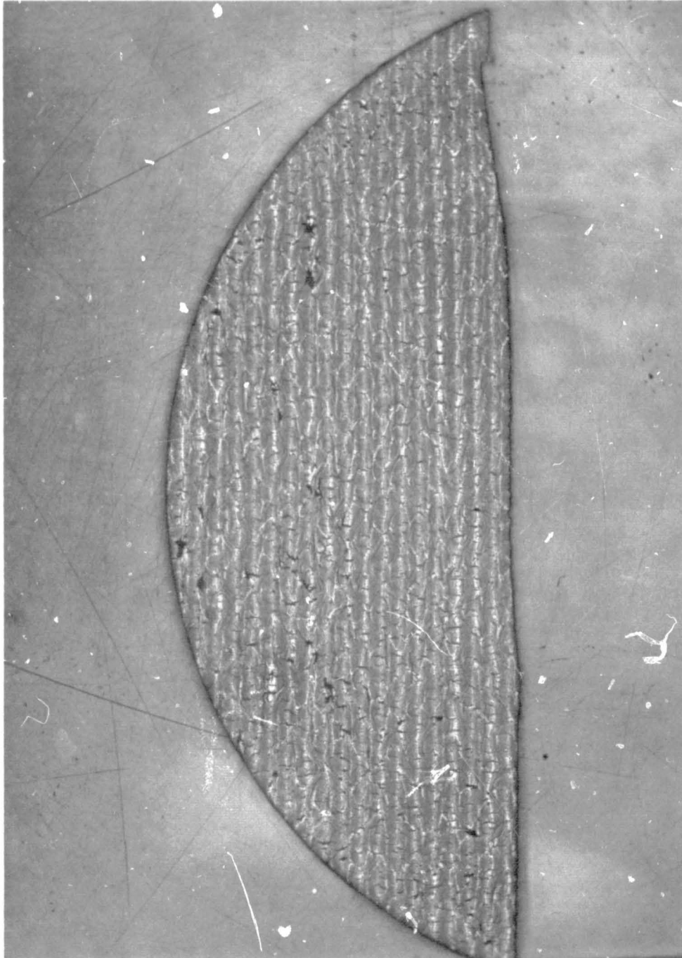
Figure 11 2000°F OVEN-CHARRED SILICA-PHENOLIC MXS-89 CORING (5X MAGNIFICATION)
