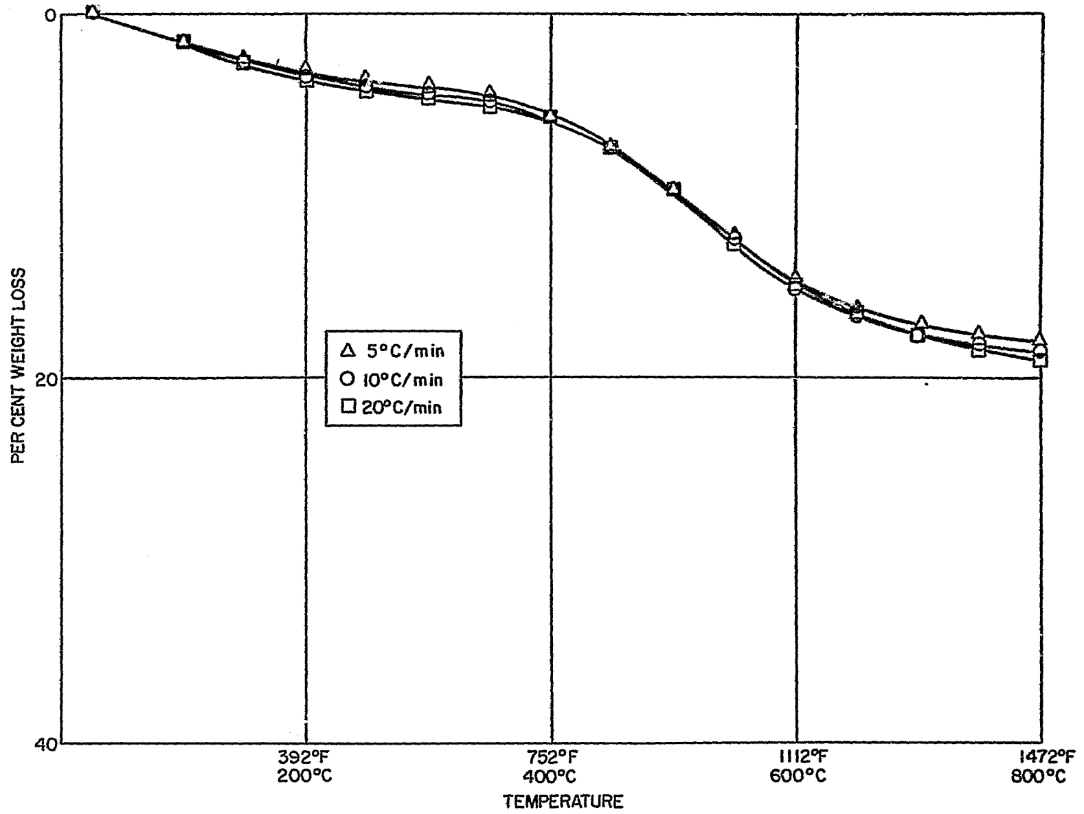
Figure 33 TGA CURVES FOR SILICA-PHENOLIC IN HELIUM
