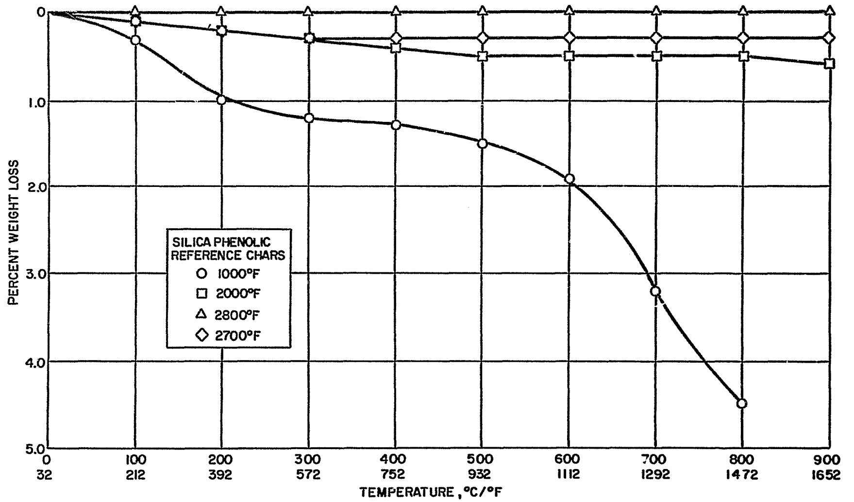
Figure 37 TGA IN HELIUM AT 10° C/MIN -- SILICA-PHENOLIC REFERENCE CHARS
