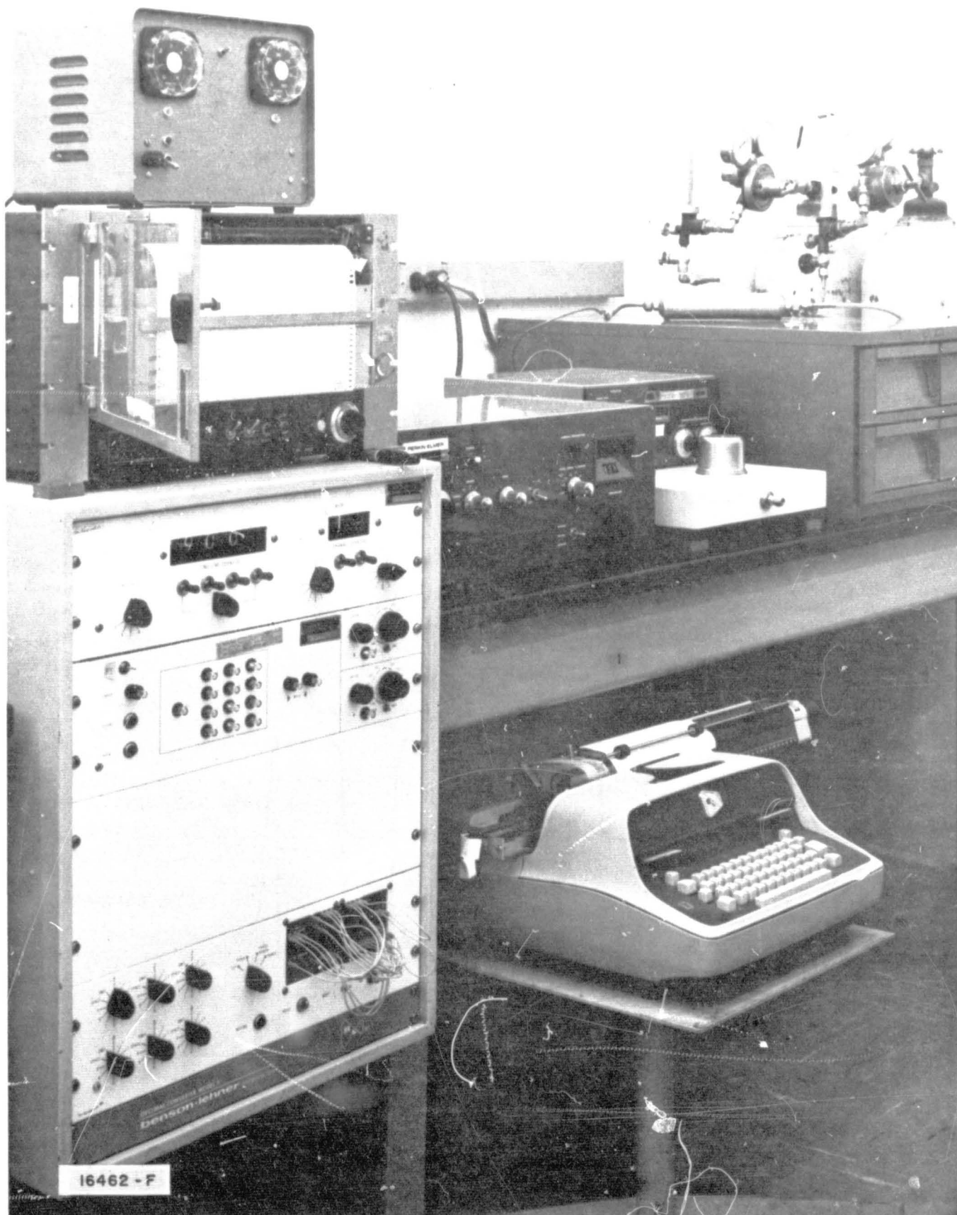
Figure D-5 PERKIN-ELMER DIFFERENTIAL SCANNING CALORIMETER, DSC-1
