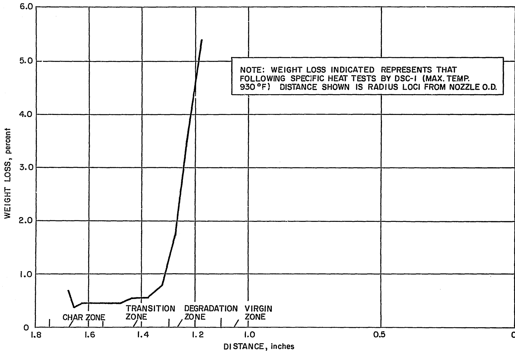
Figure 121 GRAPHITE PHENOLIC NOZZLE EXIT, POST-DSC TEST WEIGHT LOSS VERSUS CHAR DEPTH
