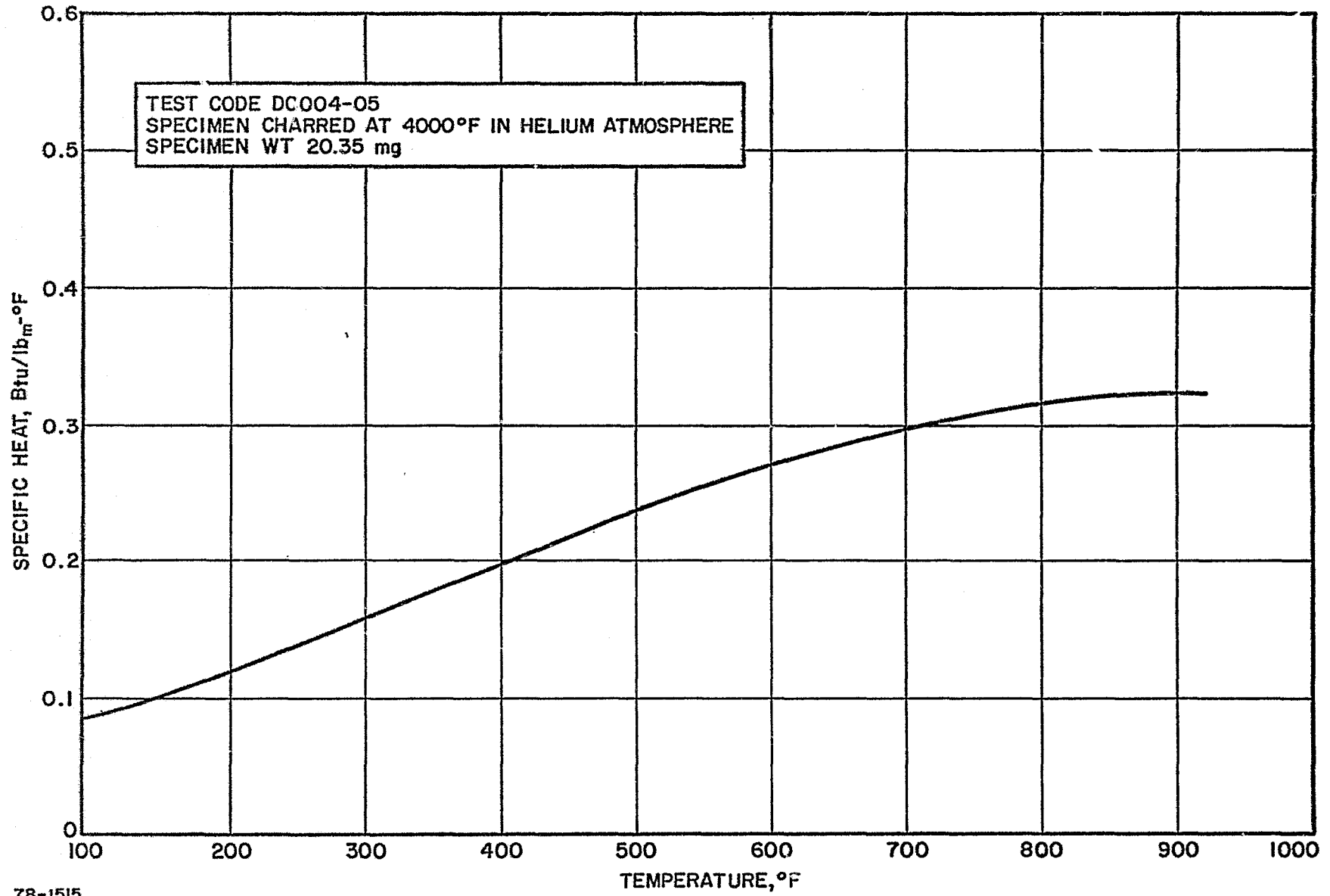
Figure 67 GRAPHITE-PHENOLIC MX4501, 4000°F PRECHARRED, SPECIFIC HEAT VERSUS TEMPERATURE
