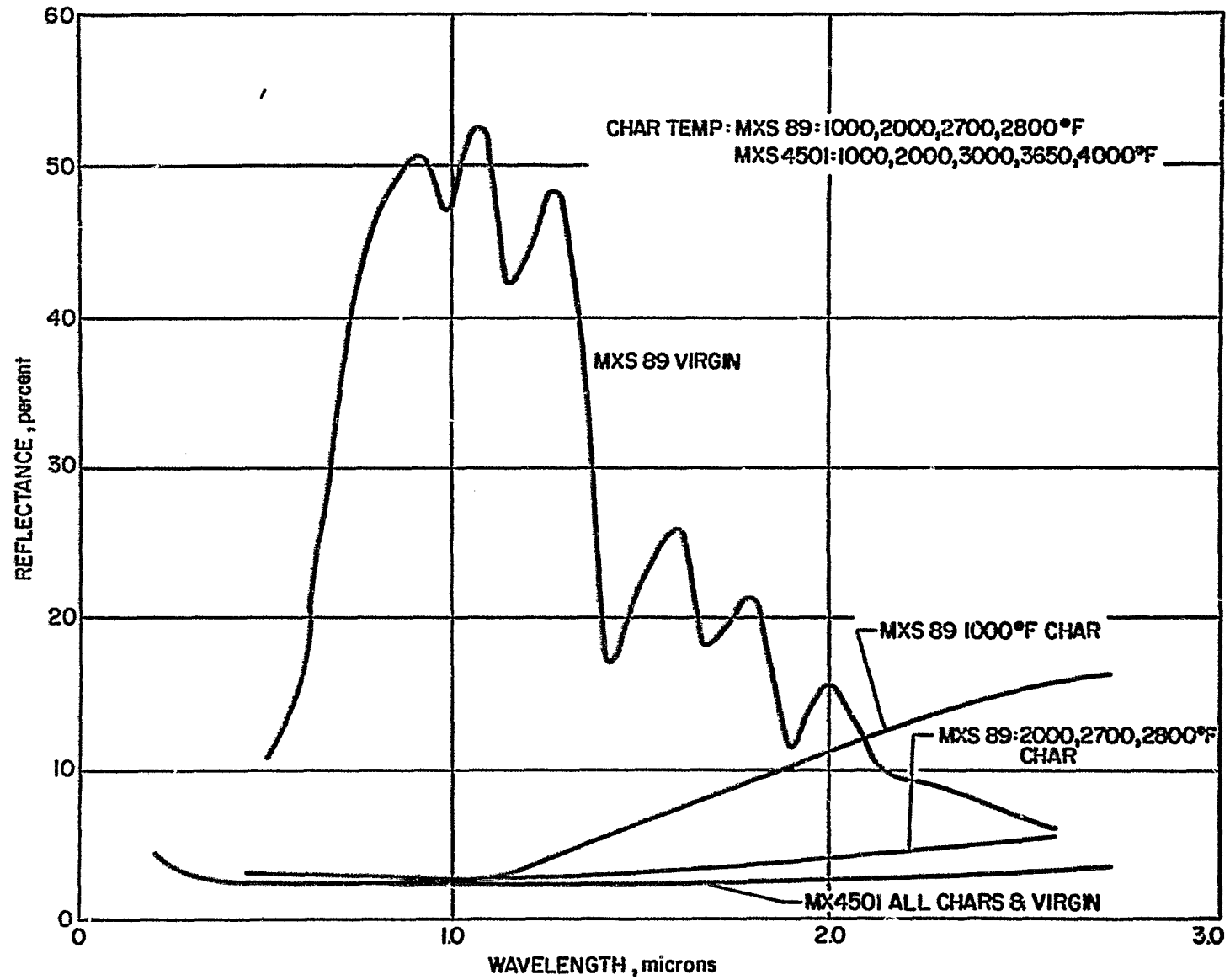
Figure 44 SILICA-PHENOLIC MXS-89 AND GRAPHITE-PHENOLIC MX4501 CHAR OPTICAL PROPERTIES
