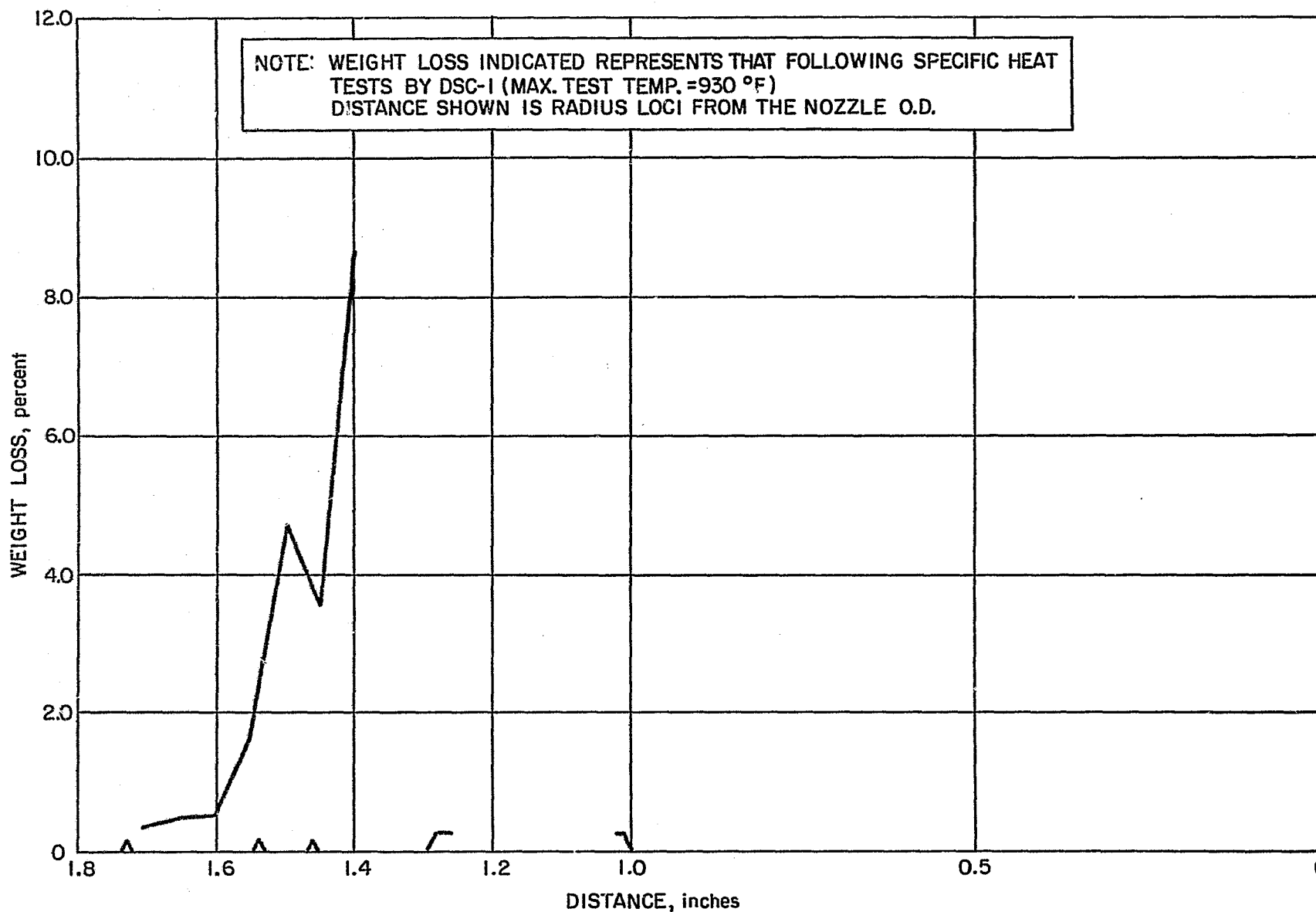
Figure 107 SILICA-PHENOLIC NOZZLE THROAT, POST DSC TEST WEIGHT LOSS VERSUS CHAR DEPTH
