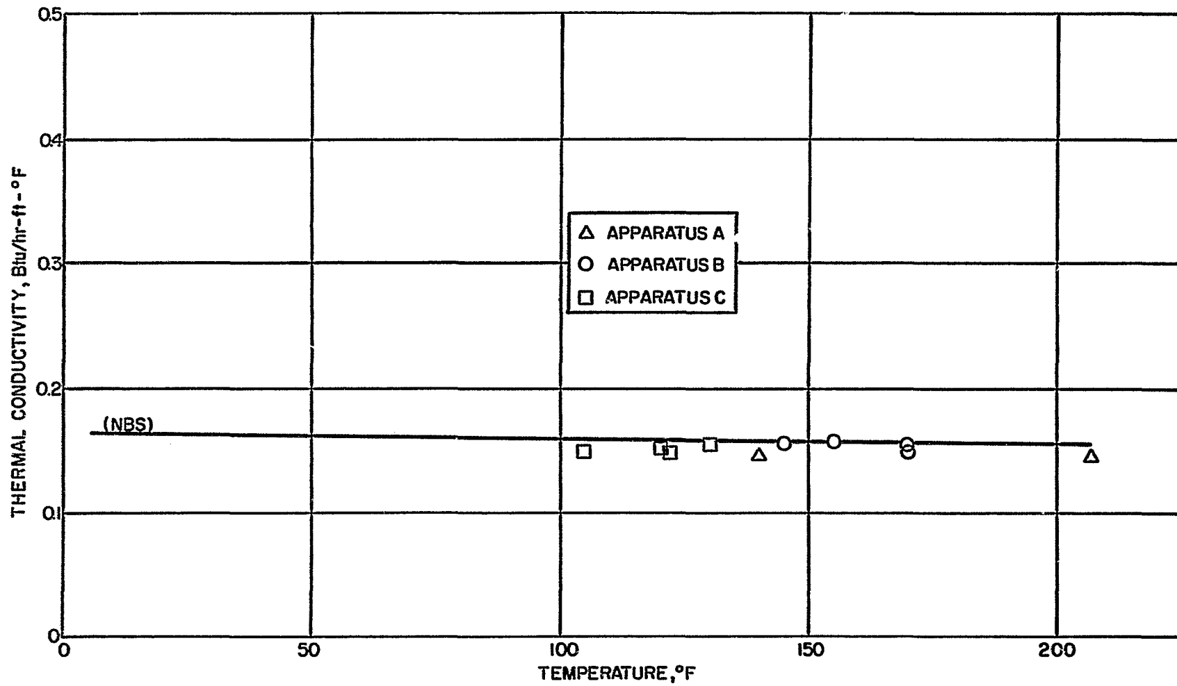
Figure C-4 APPARENT THERMAL CONDUCTIVITY VERIFICATION TEST DATA USING NBS SILICONE RUBBER
