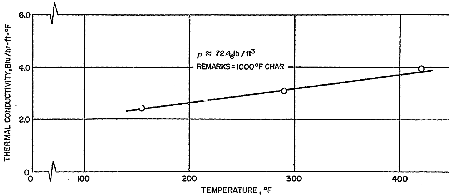
Figure 49 GRAPHITE-PHENOLIC MX4501, 1000°F PRECHARRED, THERMAL CONDUCTIVITY VERSUS TEMPERATURE
