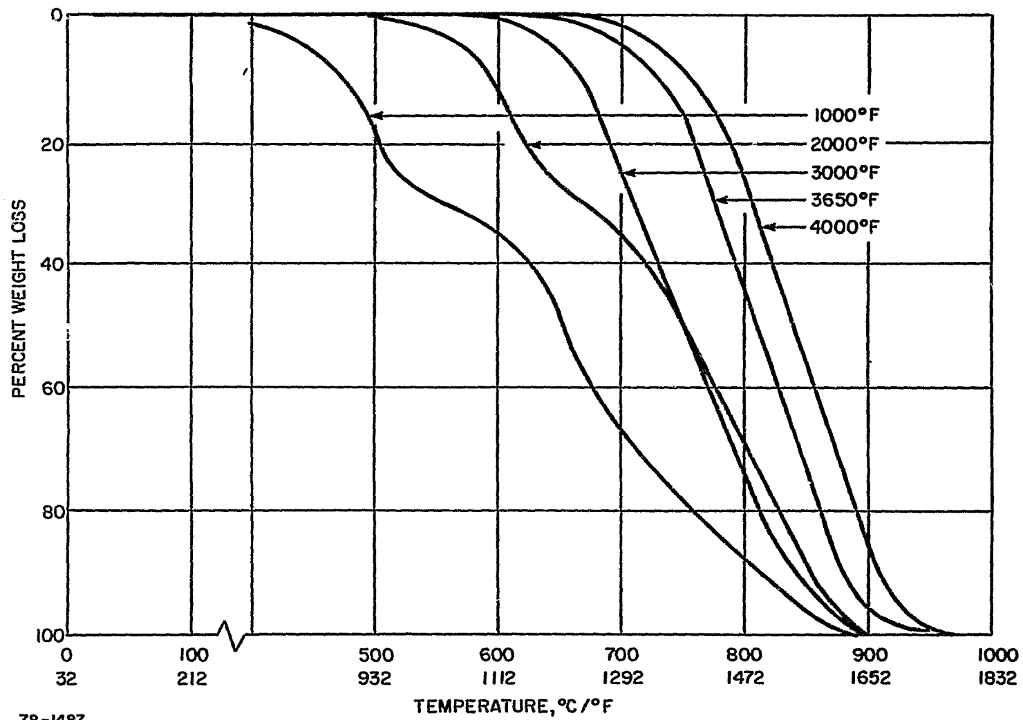
Figure 38 GRAPHITE PHENOLIC THERMOGRAVIMETRIC ANALYSIS IN AIR AT 5° C/MIN
