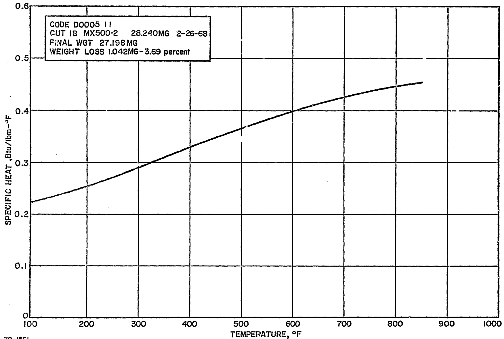
Figure 118 GRAPHITE-PHENOLIC NOZZLE EXIT, 1.228-INCH CHAR LAYER, SPECIFIC HEAT VERSUS TEMPERATURE
