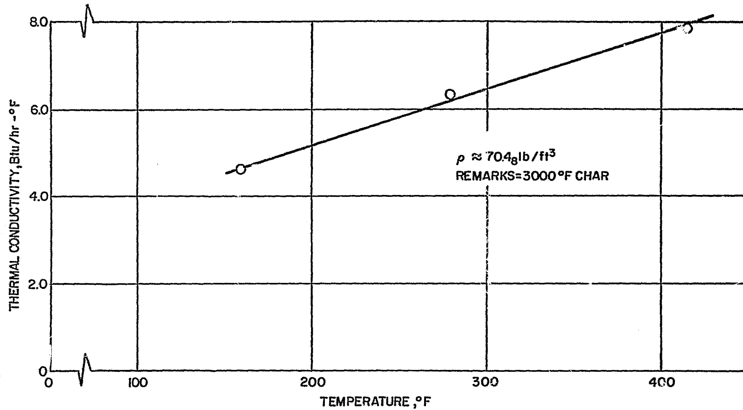
Figure 51 GRAPHITE-PHENOLIC MX4501, 3000°F PRECHARRED, THERMAL CONDUCTIVITY VERSUS TEMPERATURE
