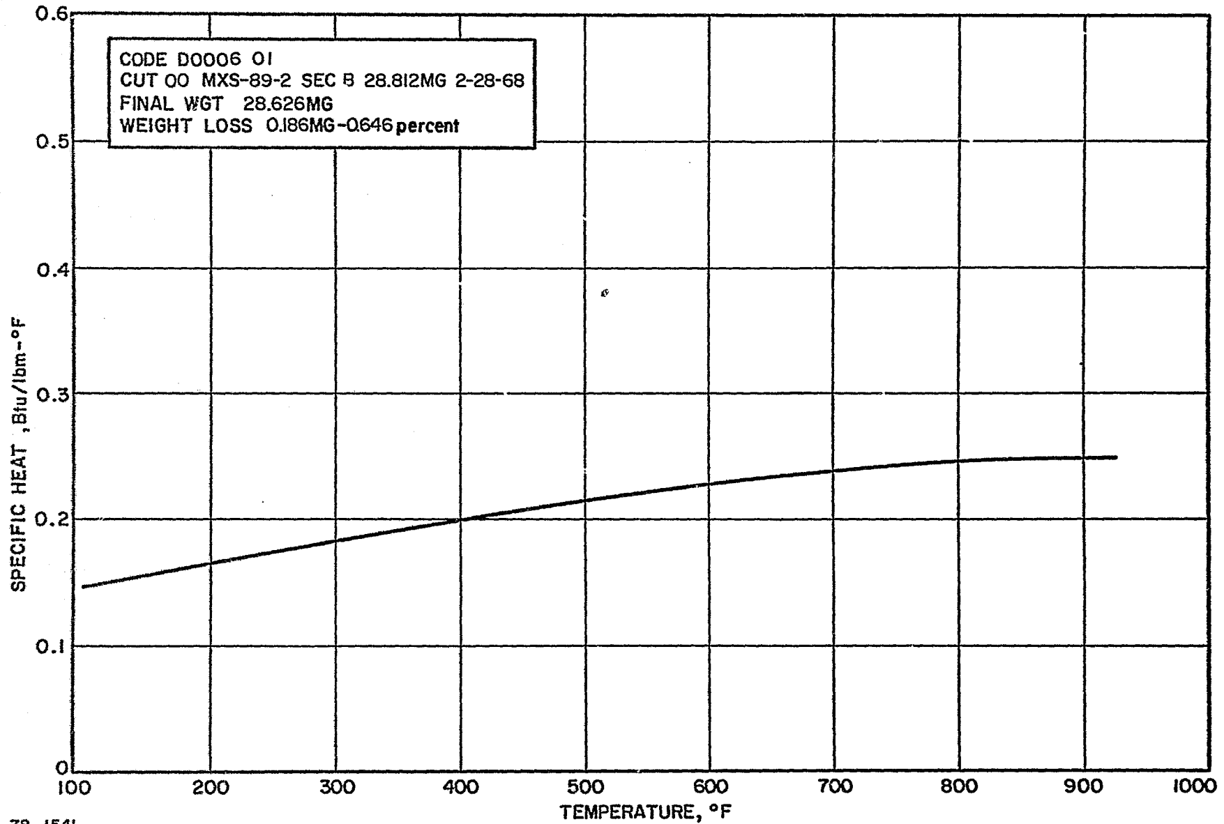
Figure 98 SILICA-PHENOLIC NOZZLE THROAT, SURFACE CHAR, SPECIFIC HEAT VERSUS TEMPERATURE
