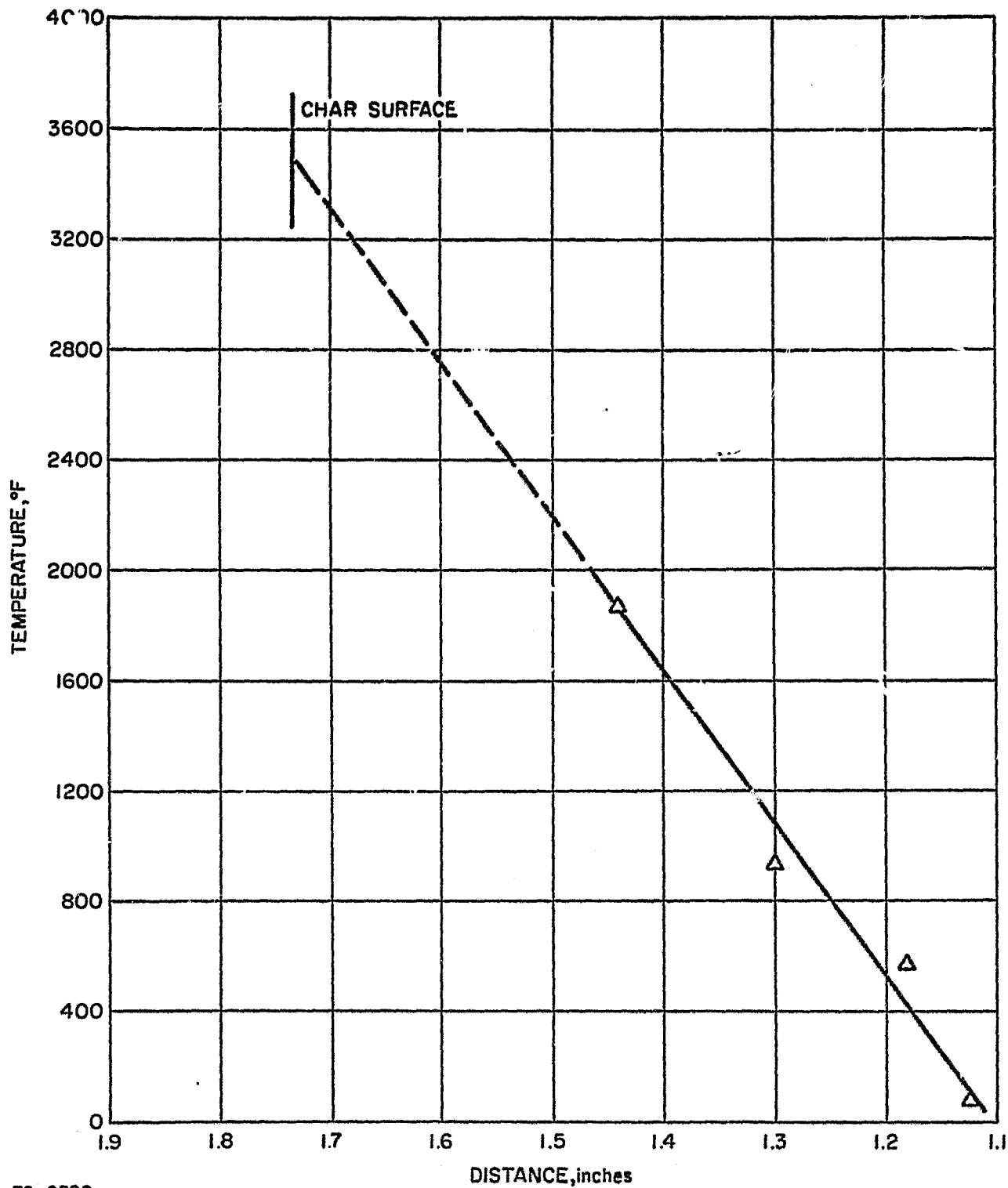
Figure 94 POSTULATED TEMPERATURE PROFILE FOR THROAT SECTION OF SILICA-PHENOLIC NOZZLE
