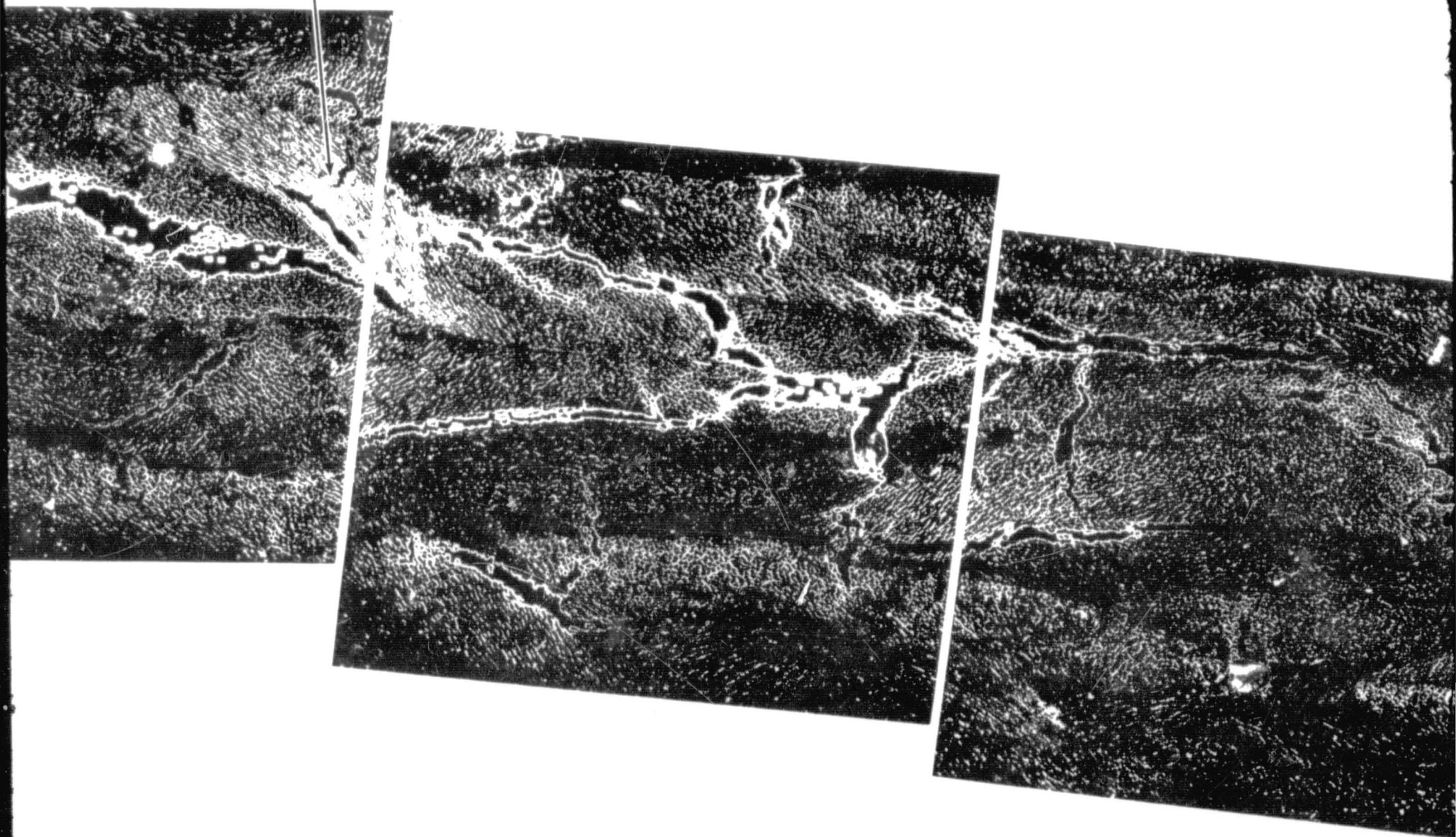
Figure 82 GRAPHITE-PHENOLIC MX4500 POST-FIRED ROCKET NOZZLE CHAR ZONE MONTAGE (100X MAGNIFICATION)
