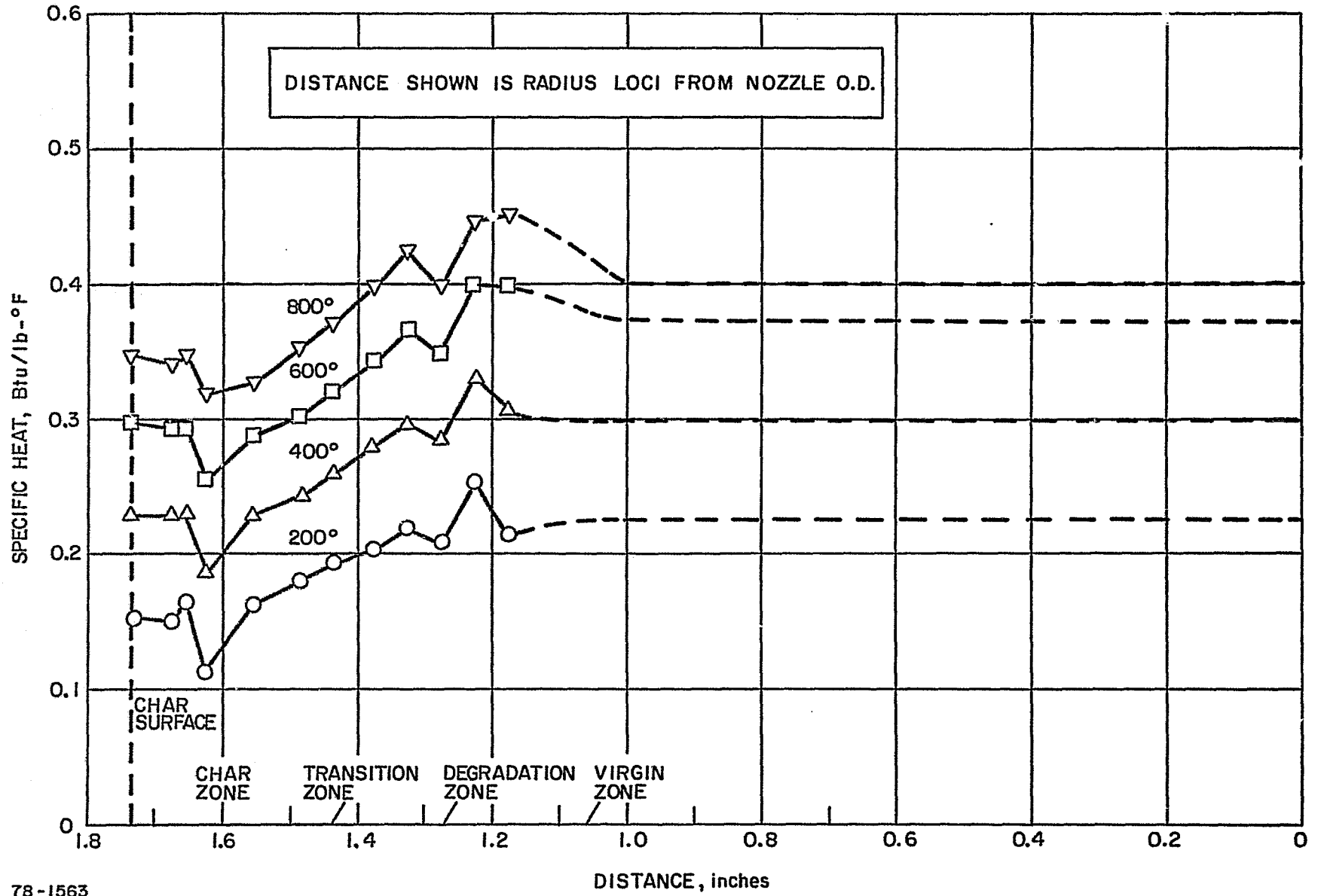
Figure 120 GRAPHITE PHENOLIC NOZZLE EXIT, SPECIFIC HEAT (AT TEMPERATURE) VERSUS CHAR LENGTH
