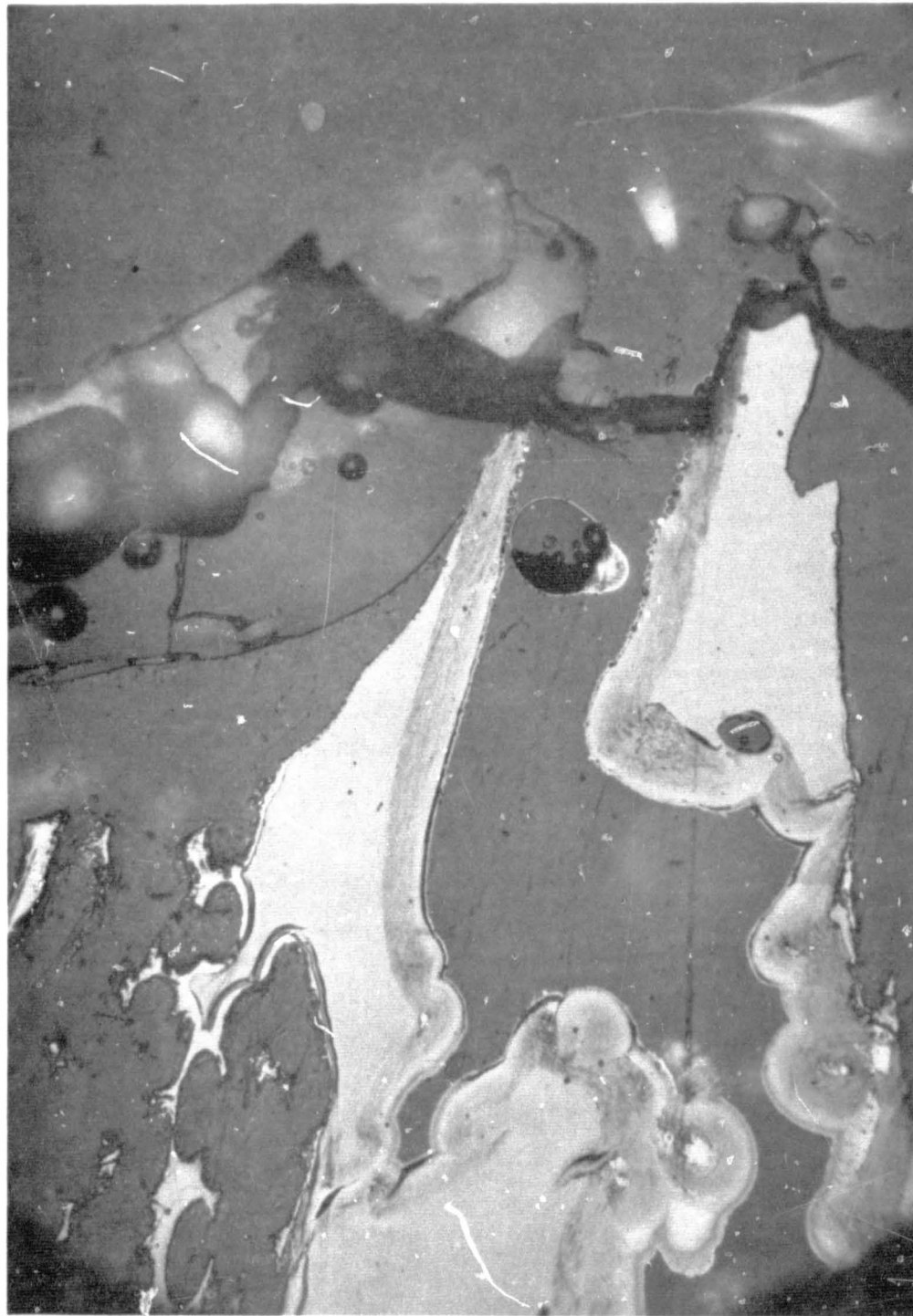
Figure 74 POST-FIRED SILICA-PHENOLIC MXS-89 NOZZLE SURFACE CHAR (500X MAGNIFICATION)
