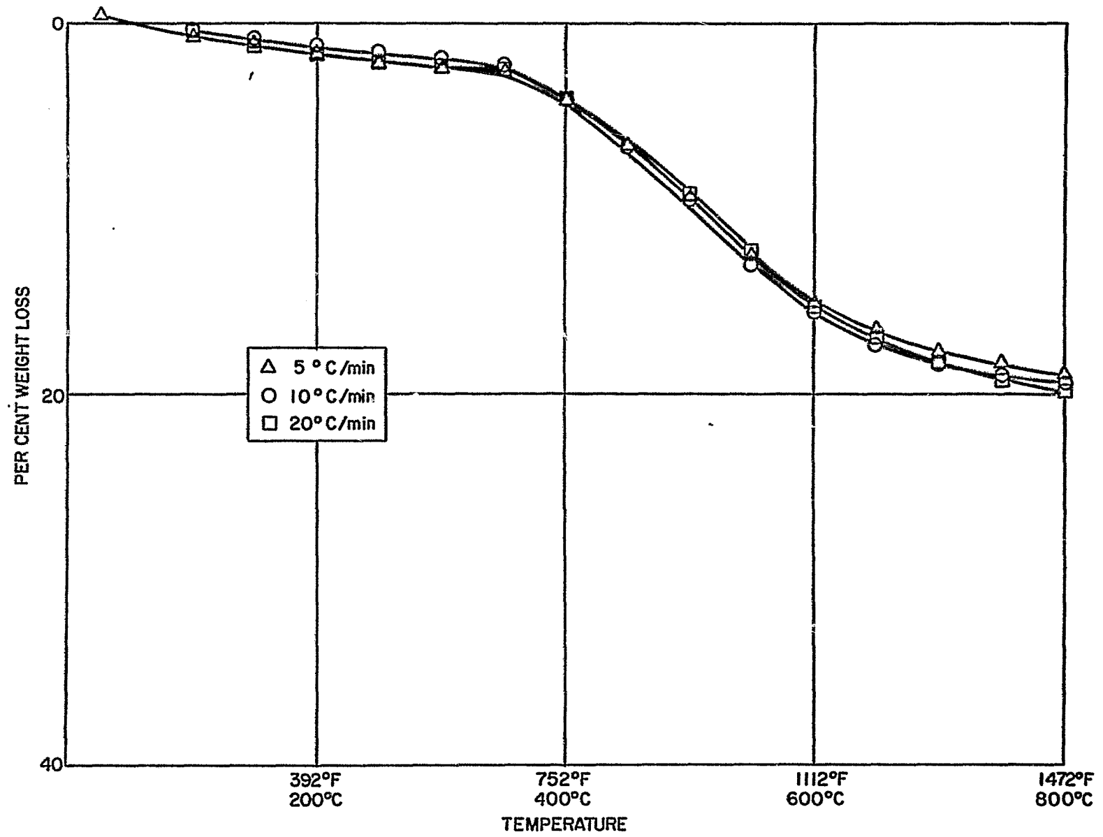
Figure 34 TGA CURVES FOR GRAPHITE-PHENOLIC IN HELIUM
