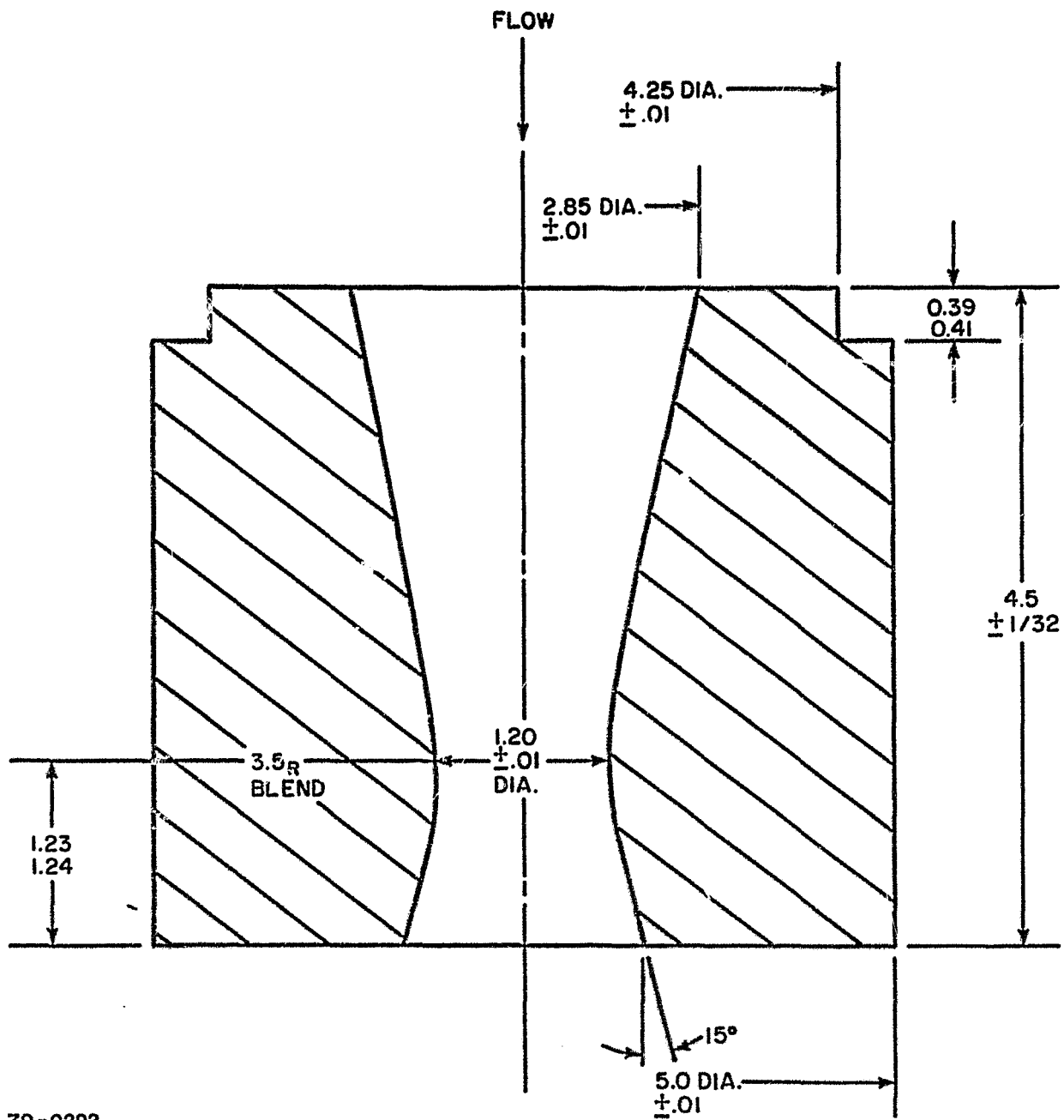
Figure 2 ORIGINAL GEOMETRY OF UNFIRED NOZZLES
