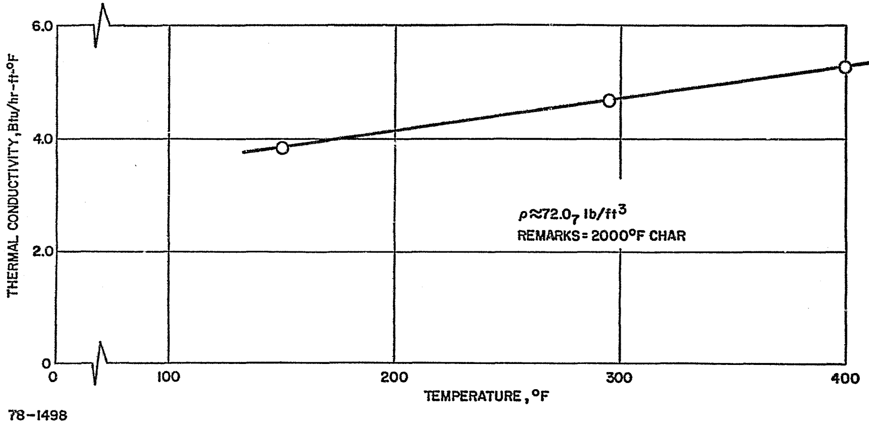
Figure 50 GRAPHITE-PHENOLIC MX4501, 2000°F PRECHARRED, THERMAL CONDUCTIVITY VERSUS TEMPERATURE
