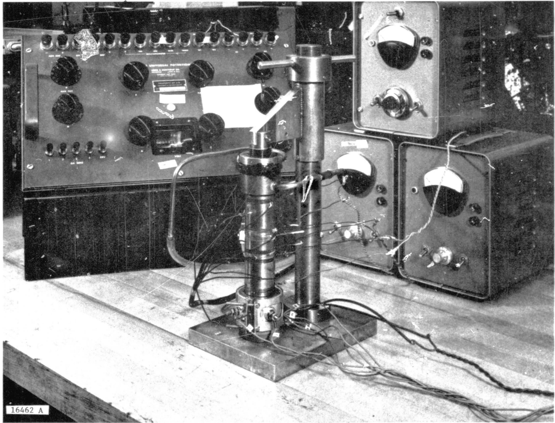
Figure C-1 STANDARD AVCO CUT-BAR APPARATUS
