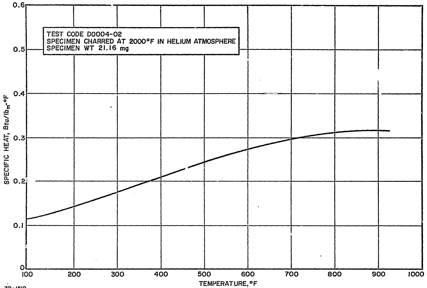
Figure 64 GRAPHITE-PHENOLIC MX4501, 2000°F PRECHARRED, SPECIFIC HEAT VERSUS TEMPERATURE
