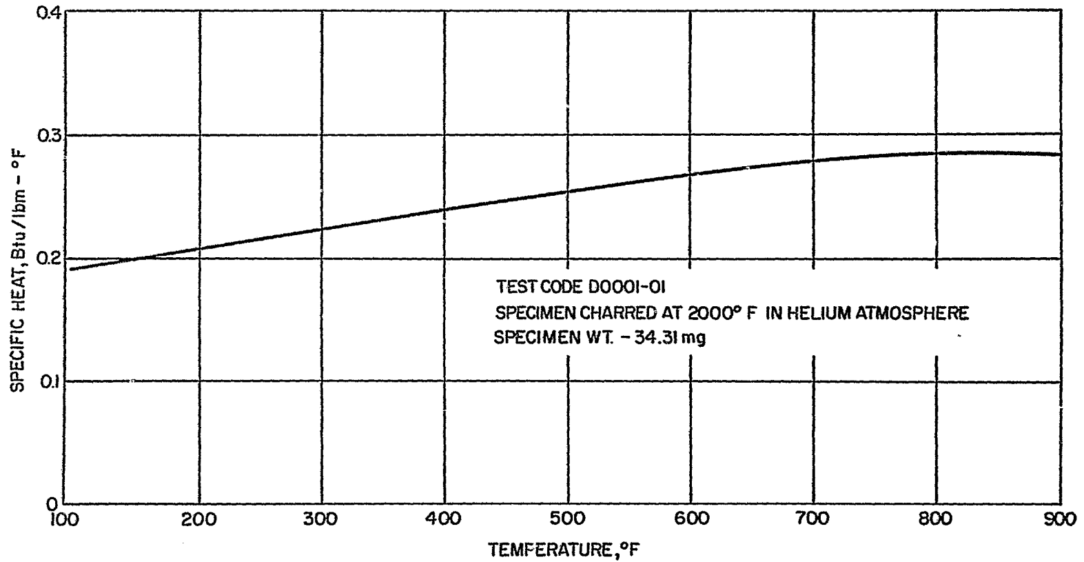
Figure 59 SILICA-PHENOLIC MXS-89, 2000°F PRECHARRED, SPECIFIC HEAT VERSUS TEMPERATURE
