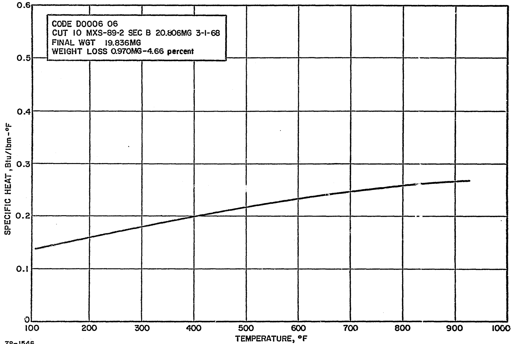
Figure 103 SILICA-PHENOLIC NOZZLE THROAT, 1.500-INCH CHAR LAYER, SPECIFIC HEAT VERSUS TEMPERATURE
