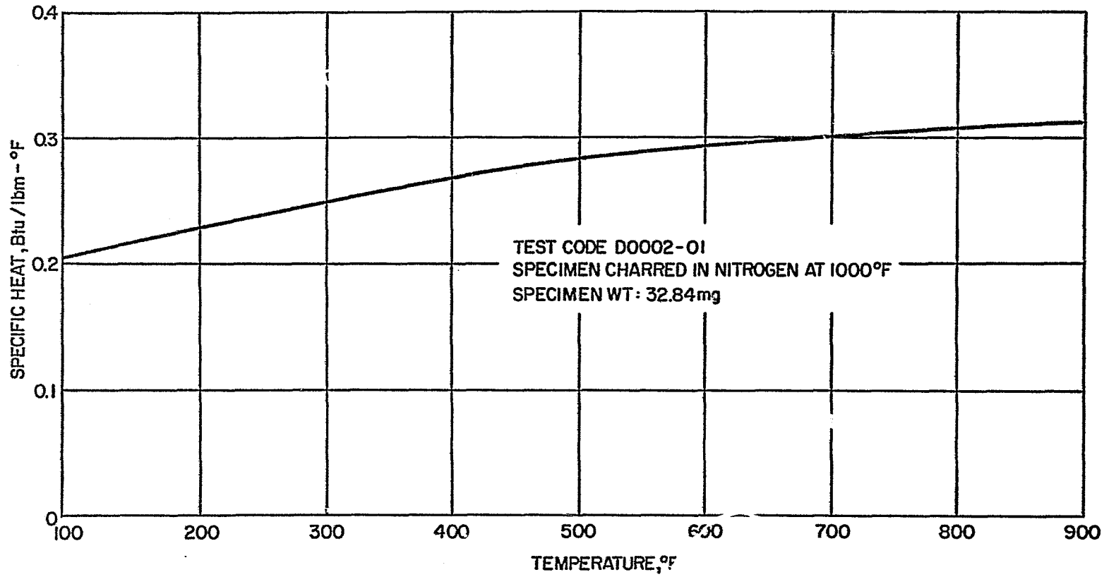
Figure 58 SILICA-PHENOLIC MXS-89, 1000°F PRECHARRED, SPECIFIC HEAT VERSUS TEMPERATURE
