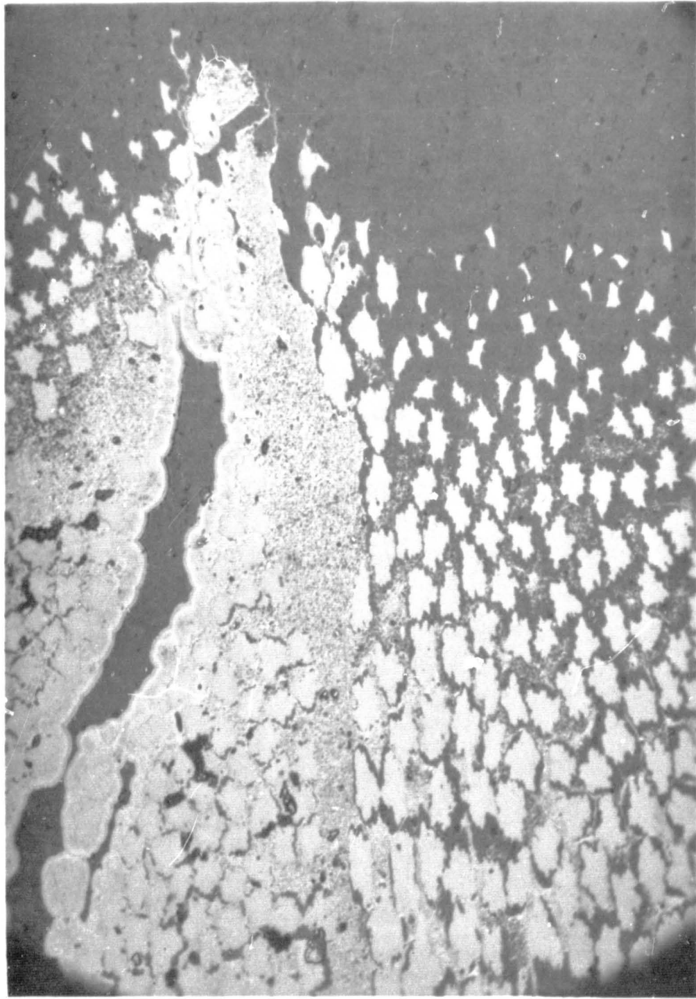
Figure 83 POST-FIRED GRAPHITE-PHENOLIC MX4500 NOZZLE CHAR (SURFACE CHAR) (500X MAGNIFICATION)
