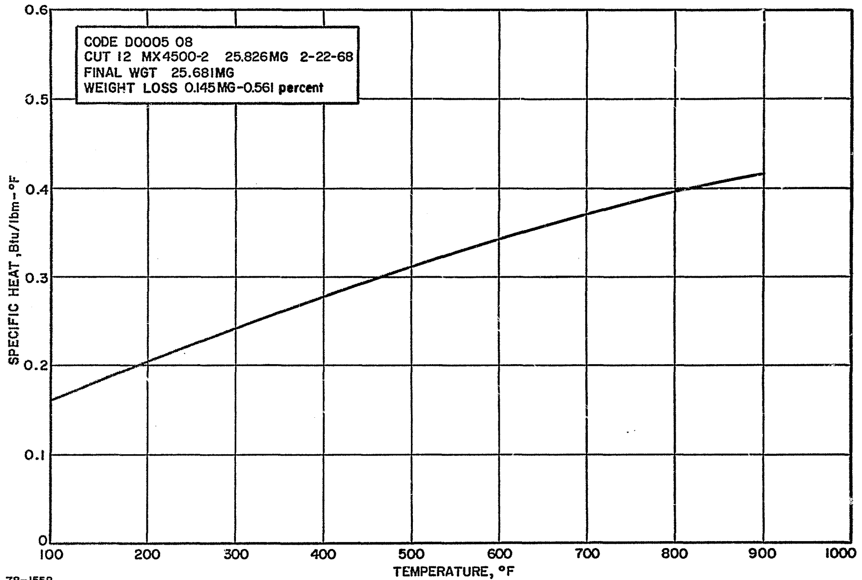
Figure 115 GRAPHITE-PHENOLIC NOZZLE EXIT, 1.377-INCH CHAR LAYER, SPECIFIC HEAT VERSUS TEMPERATURE
