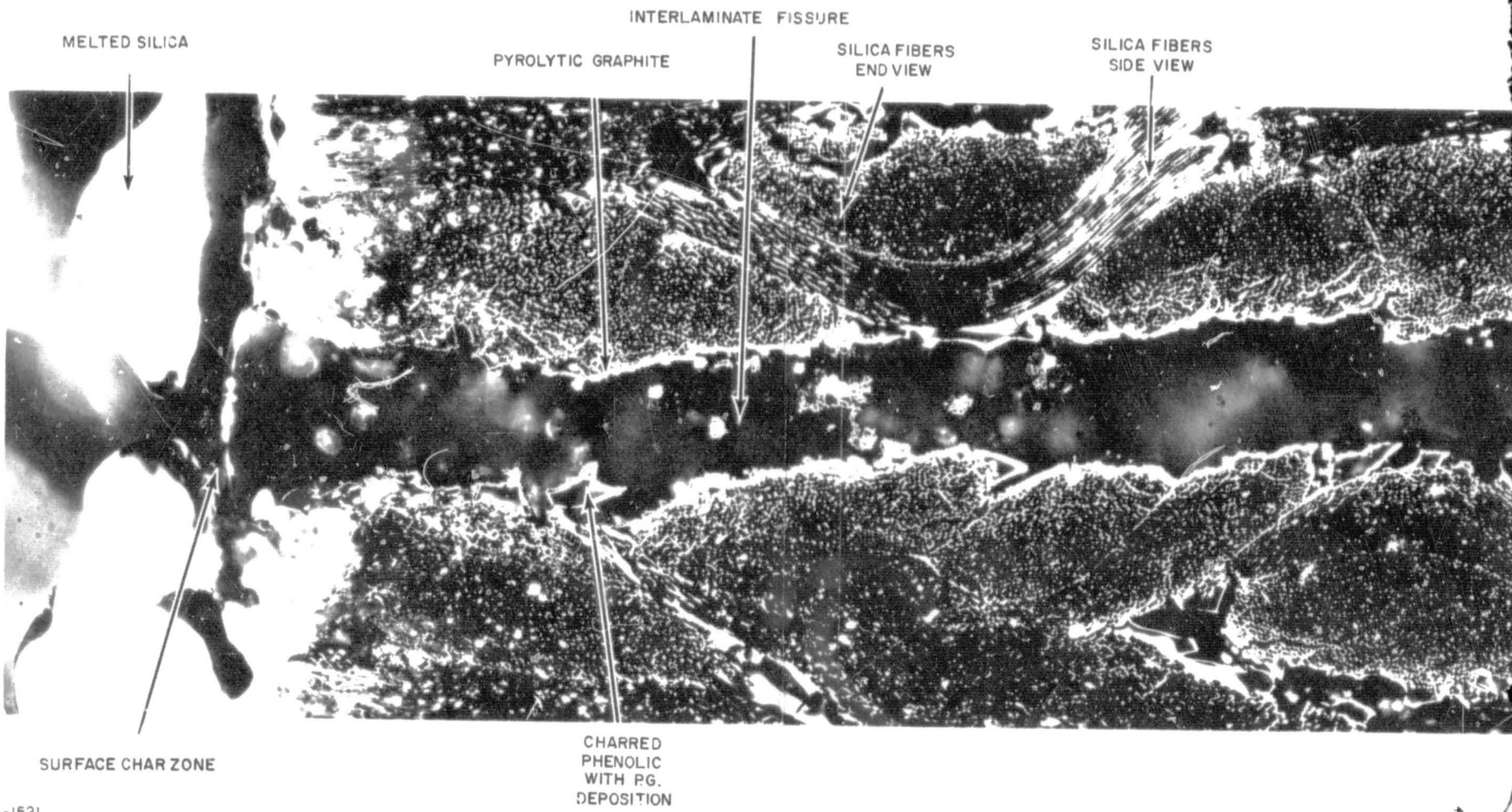
Figure 73 SILICA-PHENOLIC MXS-MONTAGE (
