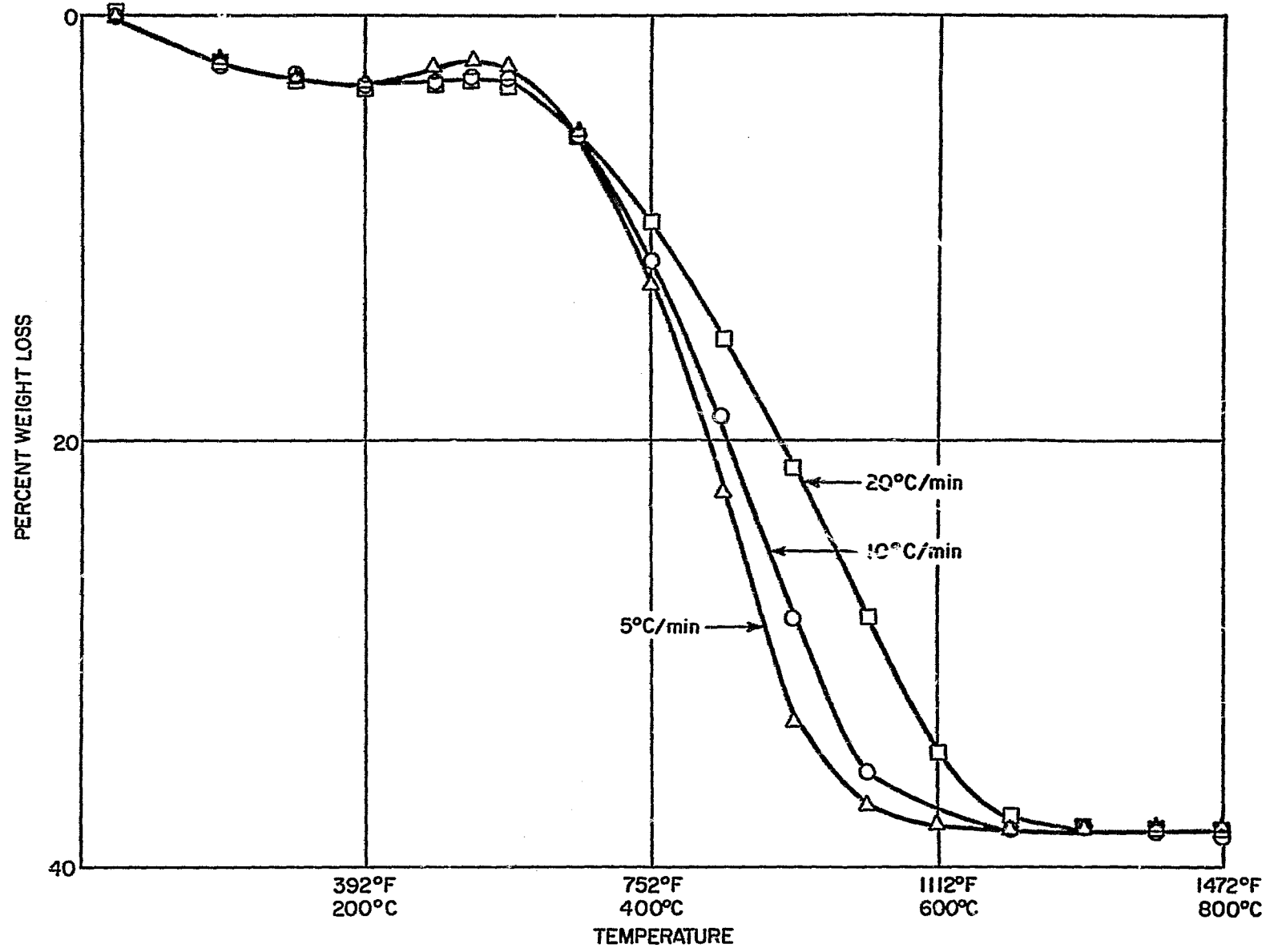
Figure 35 TGA CURVES FOR SILICA-PHENOLIC IN AIR
