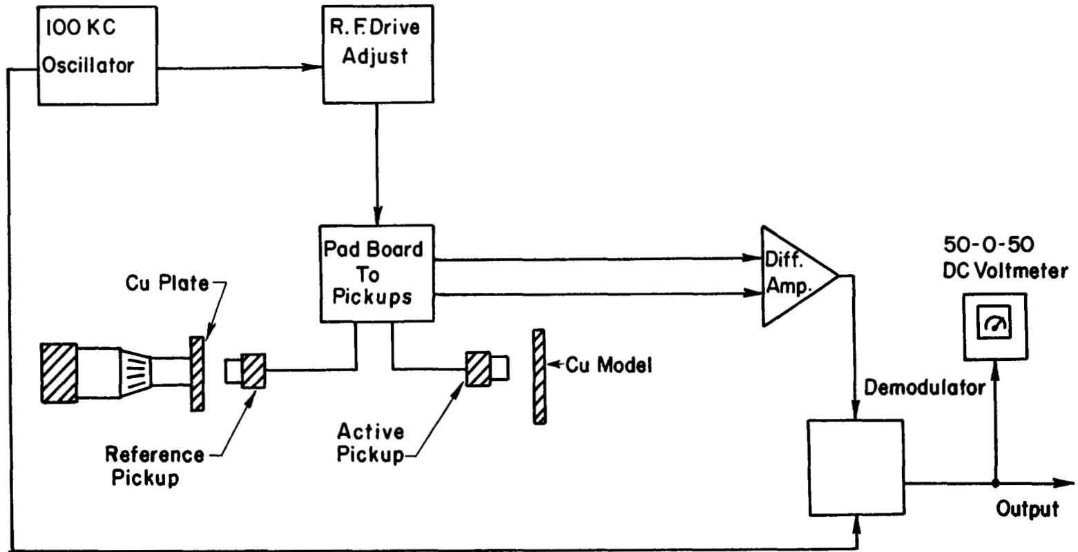
FIG. 6 PICKUP CIRCUIT
