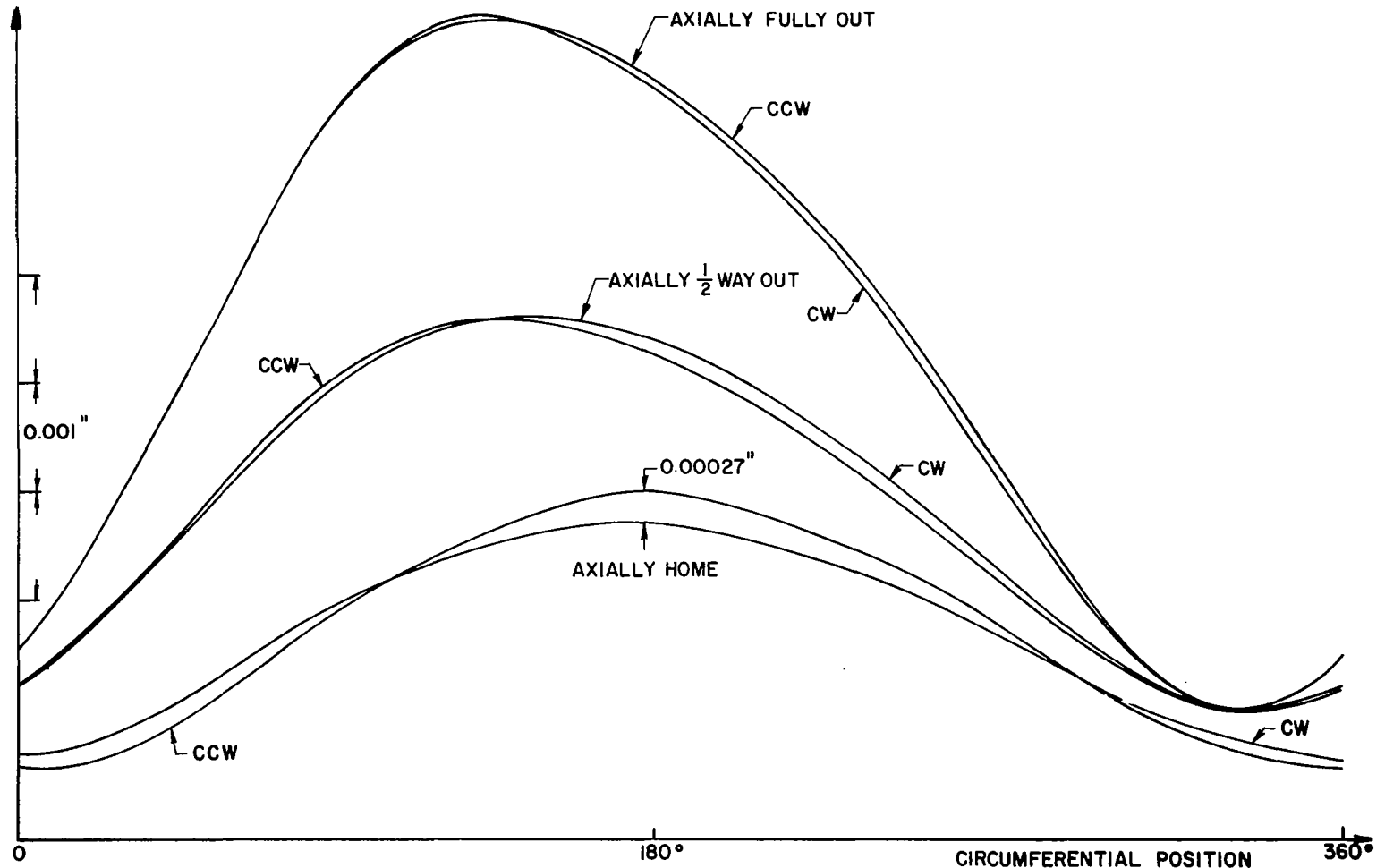
FIG. 12 HYSTERESIS CHECK
