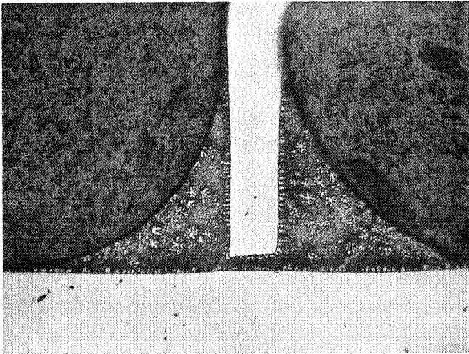
FIGURE 12. Cb-1Zr T-JOINT BRAZED WITH Zr-19Cb-6V-3Be; As-Brazed Condition
