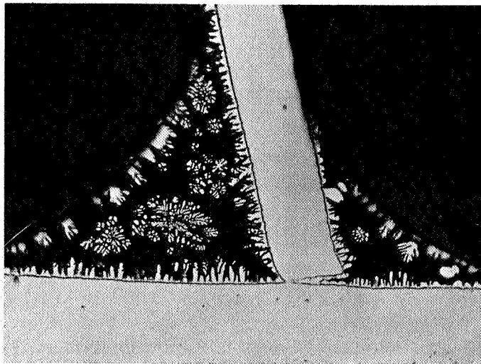
FIGURE 10. Cb-1Zr T-JOINT BRAZED WITH Ti-46.5Zr-4V-3Be; As-Brazed Condition
