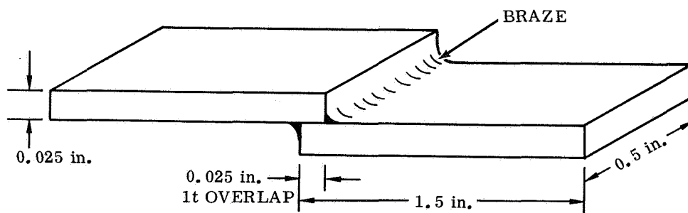
FIGURE 5. BRAZED SINGLE-LAP SHEAR SPECIMEN
