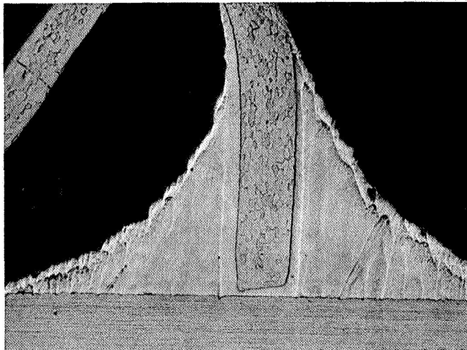
FIGURE 8. Cb-1Zr T-JOINT BRAZED WITH PURE GOLD FOIL; As-Brazed Condition
