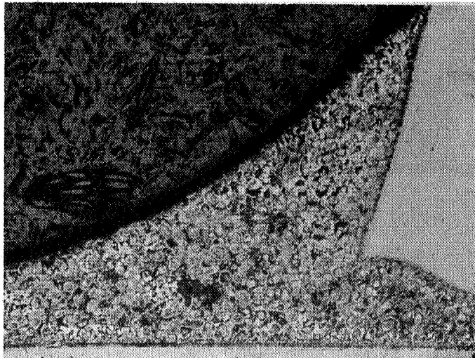
FIGURE 13. Cb-1Zr T-JOINT BRAZED WITH Zr-28V-16Ti; As-Brazed Condition
