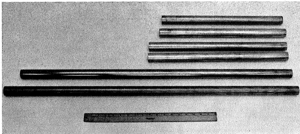
FIGURE 44. EXTERNAL SIDE VIEWS OF FOUR 18-INCH AND TWO 36-INCH HEAT RECEIVER TUBES; Post Brazing
