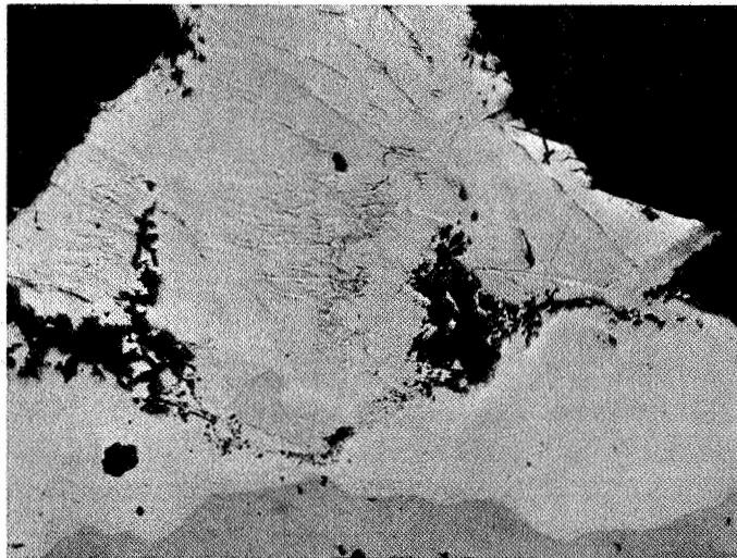
FIGURE 15. Cb-1Zr T-JOINT BRAZED WITH GOLD
