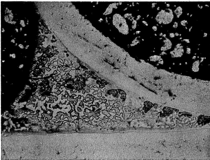
FIGURE 42. TRANSVERSE SECTIONS THROUGH TUBE/FIN BRAZEMENTS MADE WITH Zr-28V-16Ti BRAZE ALLOY; Fin Design A
