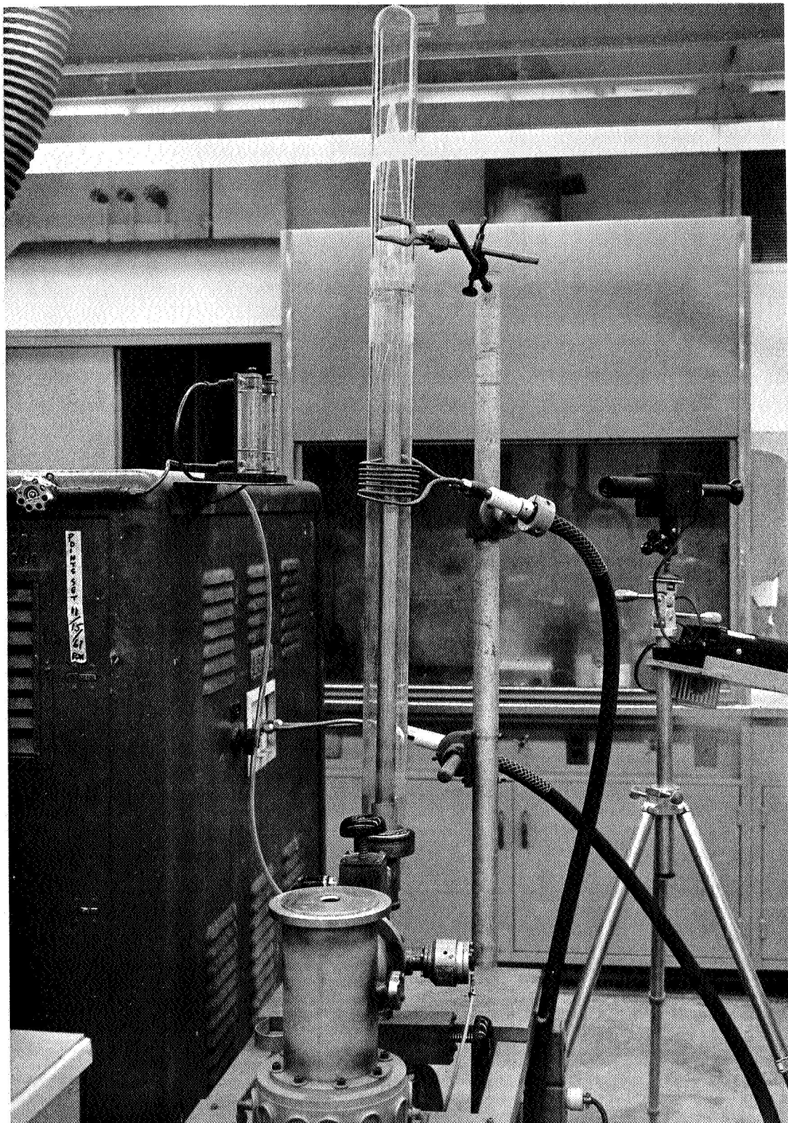
FIGURE 43. VACUUM INDUCTION BRAZING SETUP FOR 36-INCH HEAT RECEIVER TUBES
