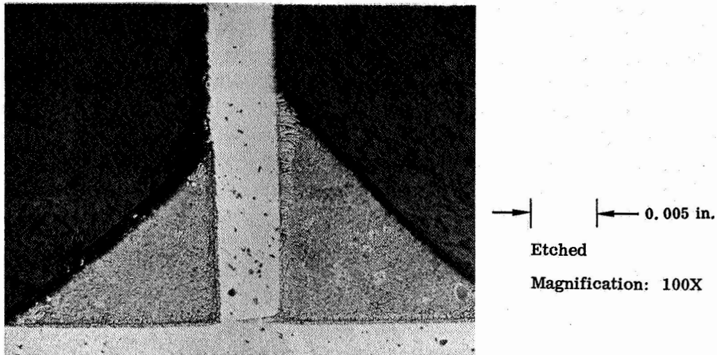
FIGURE 14. Cb-1Zr T-JOINT BRAZED WITH Zr-28V-16Ti-0.1Be; As-Brazed Condition
