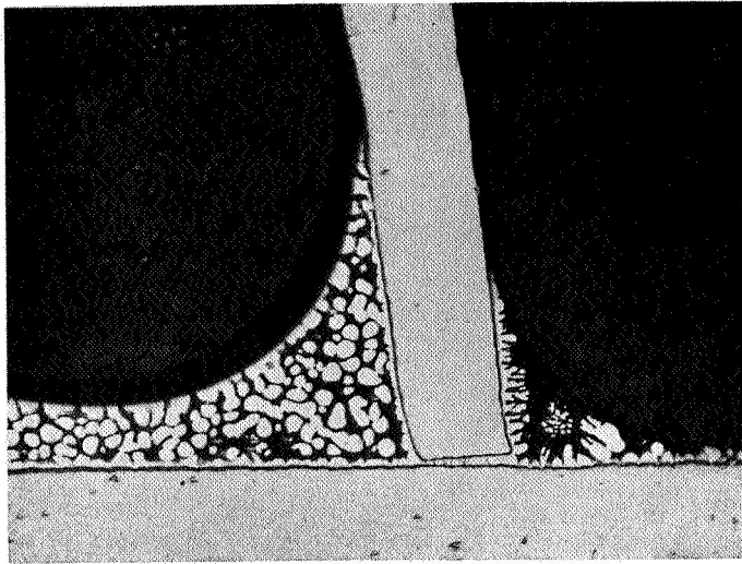
FIGURE 11. Cb-1Zr T-JOINT BRAZED WITH Ti-45Zr-7Cb-3Be; As-Brazed Condition
