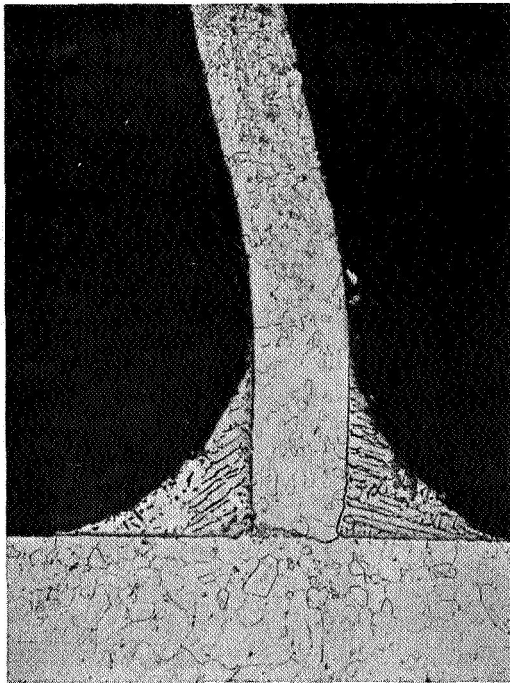
FIGURE 7. Cb-1Zr T-JOINT BRAZED WITH Cu-2Ni; As-Brazed Condition
