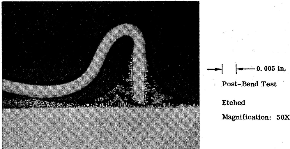
FIGURE 9. Cb-1Zr T-JOINT BRAZED WITH Ti-48Zr-4Be; As-Brazed Condition
