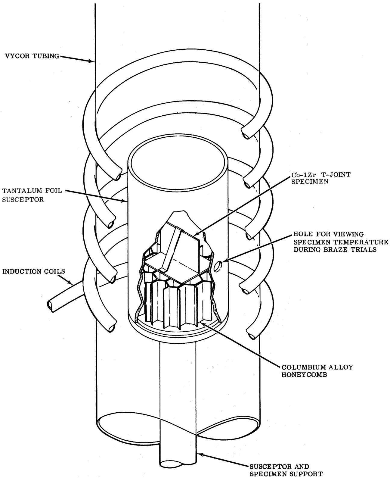
FIGURE 4. SCHEMATIC DIAGRAM OF THE LABORATORY BRAZING FURNACE
