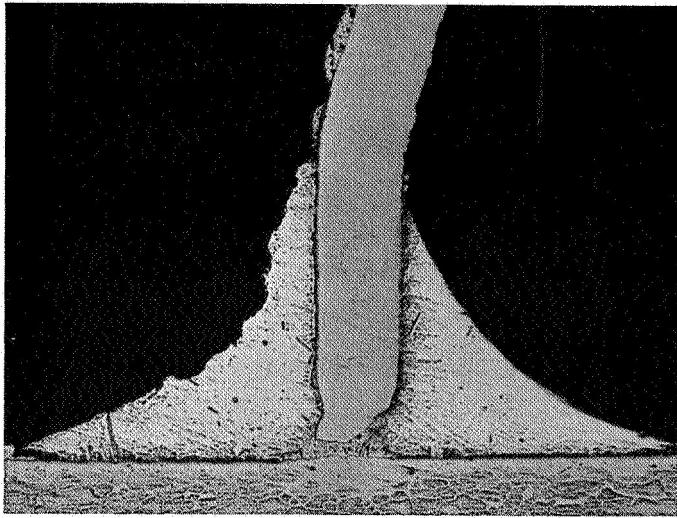
FIGURE 16. Cb-1Zr T-JOINT VACUUM BRAZED WITH Cu-2Ni ALLOY
