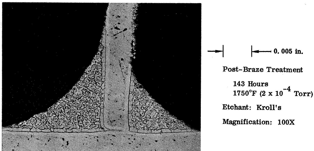
FIGURE 18. Cb-1Zr T-JOINT VACUUM BRAZED WITH Zr-28V-16Ti-0.1Be ALLOY
