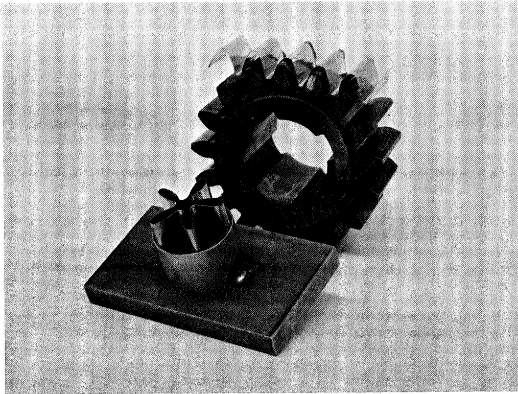
FIGURE 35. CORRUGATING GEAR AND SIZING FIXTURE FOR FABRICATING DESIGN B FIN MODULES
