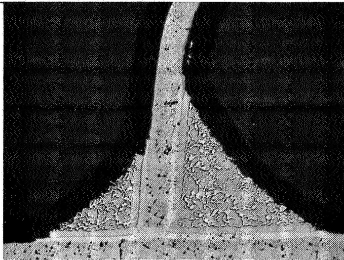
FIGURE 17. Cb-1Zr T-JOINT VACUUM BRAZED WITH Zr-28V-16Ti ALLOY
