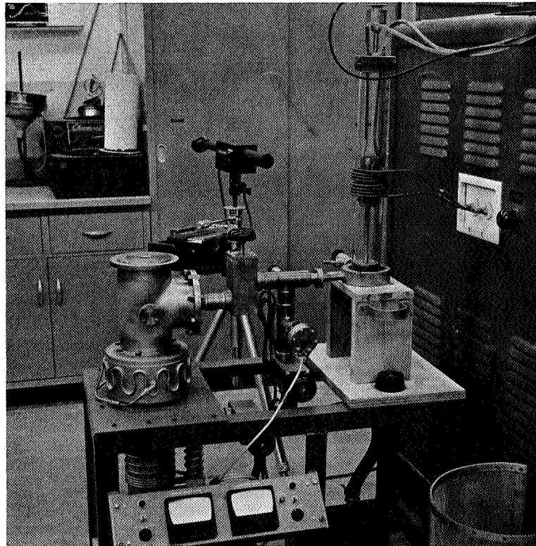
FIGURE 3. INDUCTION BRAZING FURNACE FOR BRAZING T-JOINTS
