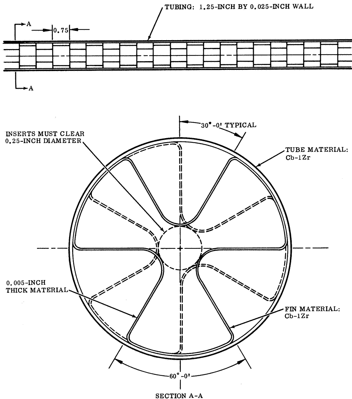
FIGURE 1. PRINCIPAL ELEMENTS OF AN INTERNALLY FINNED TUBE
