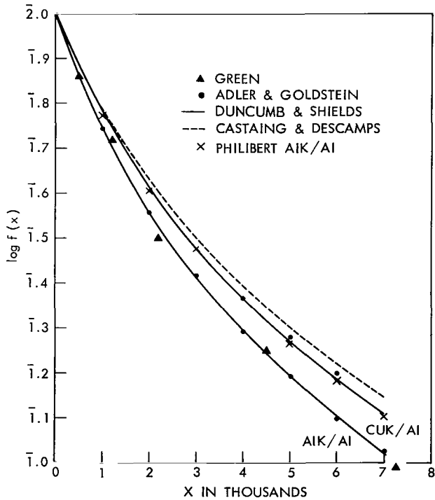
Figure 3—Plot of f(x) curves for Al.
