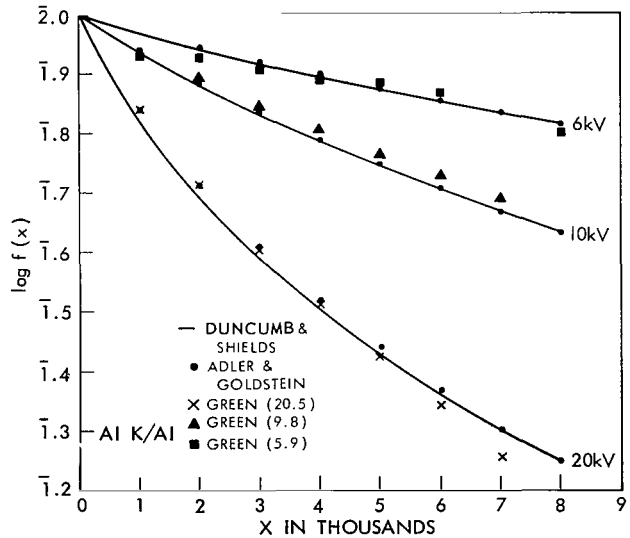
Figure 4—Plot of f(x) curves for Al K in Al with applied voltage.
