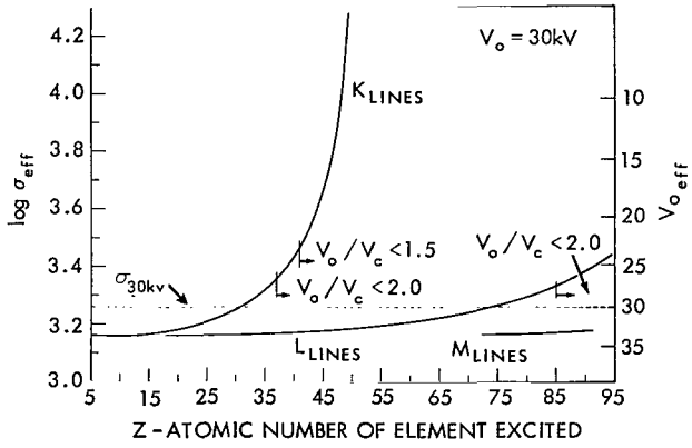
Figure 1—Overvoltage corrections, \sigma_{eff} and V_{0,eff} , plotted against the atomic number of the element excited.
