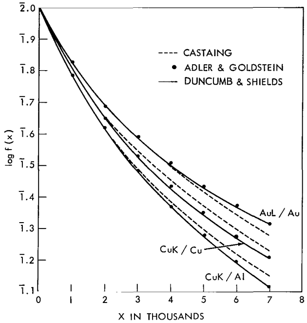
Figure 2—Plot of f(x) curves for Au L in Au, Cu K in Cu, and Cu K in Al at 29 kv.
