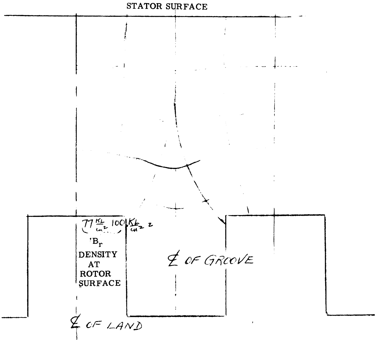
DISTRIBUTION OF SURFACE FLUX DENSITIES WHEN A ROTOR POLE-HEAD HAS 50% OF ITS SURFACE CUT AWAY BY GROOVING--ASSUME AN AIR-GAP DENSITY OF 50 KILOLINES PER INCH 2
