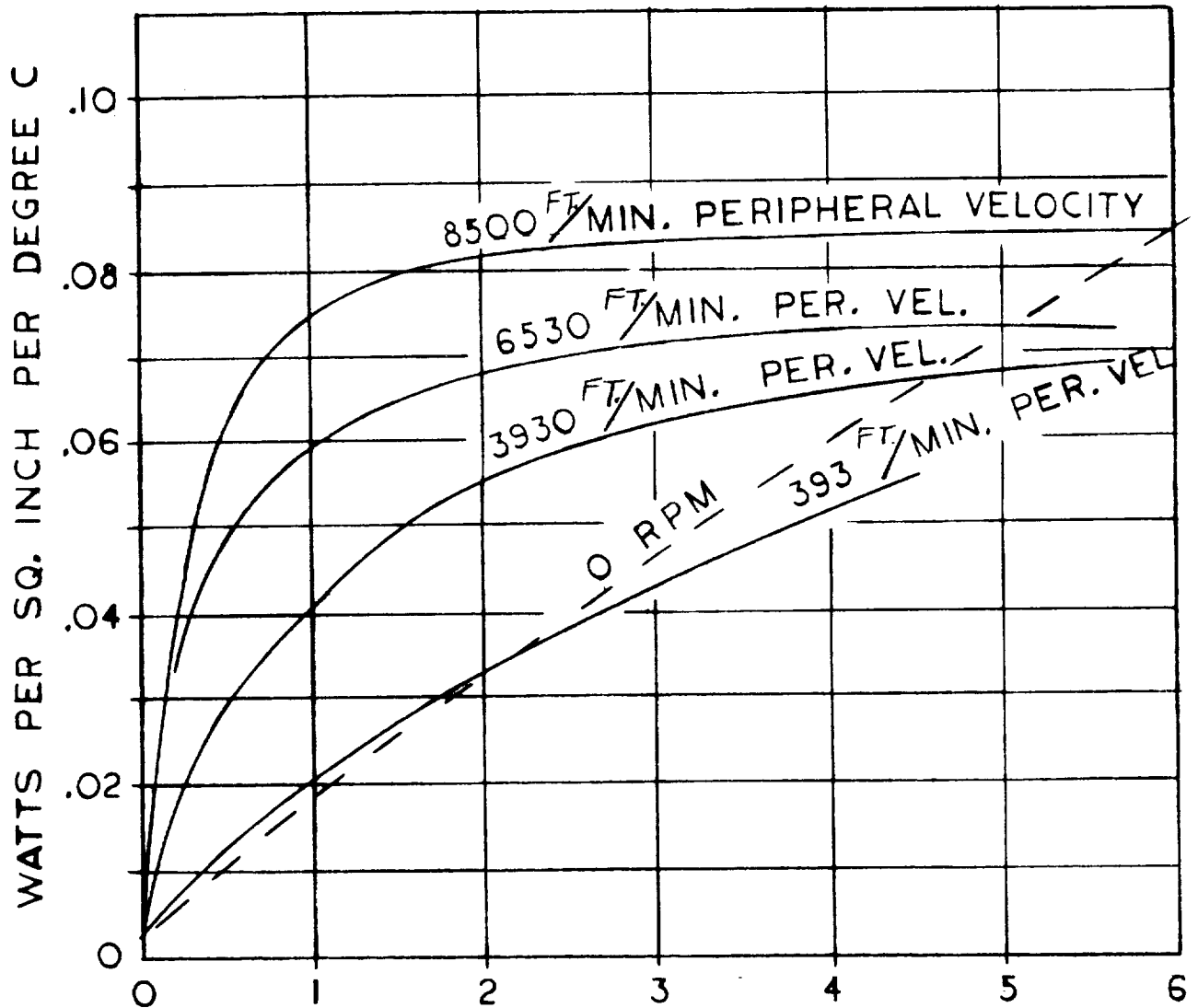
AVERAGE COOLING AIR VELOCITY THROUGH THE MACHINE AIR-GAP - THOUSANDS OF FEET PER MINUTE.
