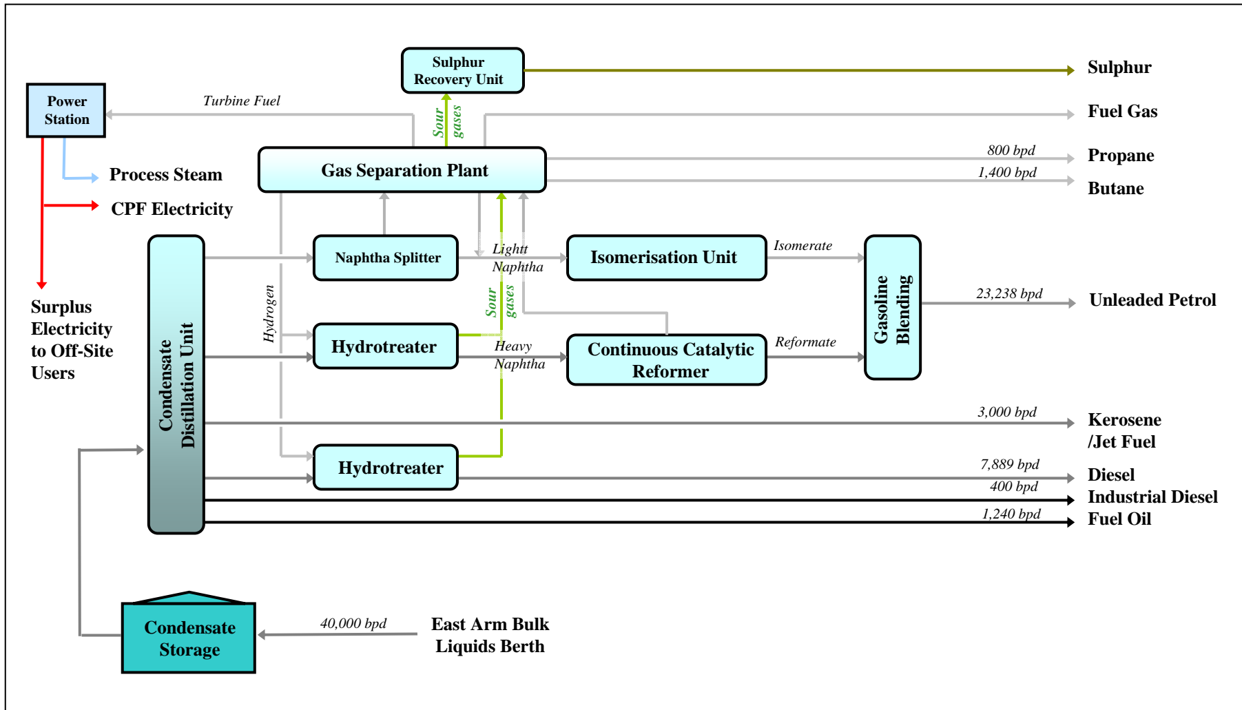
Figure 3 - Simplified Process Diagram Condensate Processing Facility - East Arm, Darwin NOTICE OF INTENT
