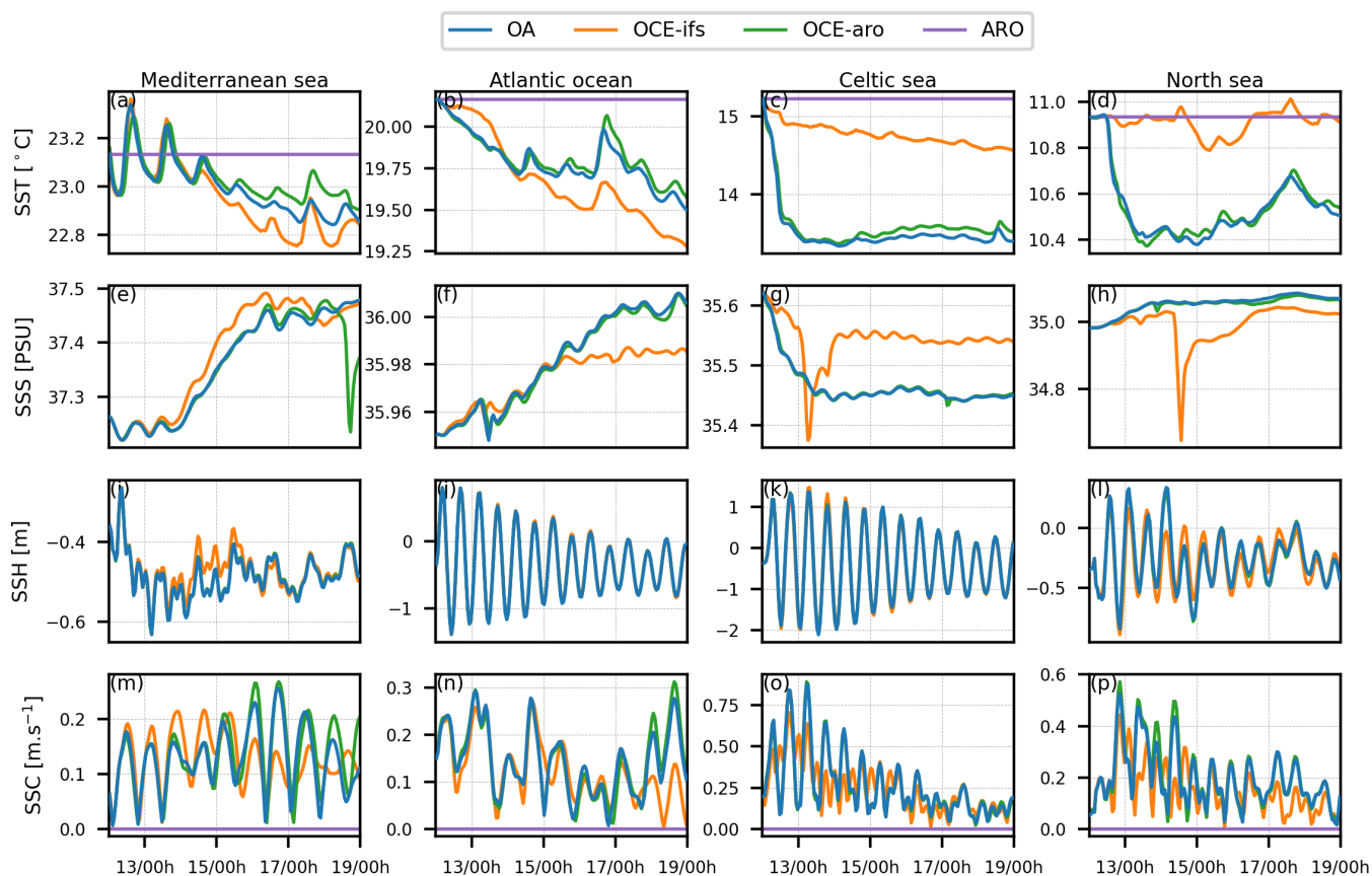
Figure 6. Temporal evolution of simulated sea surface temperature (SST, °C), salinity (SSS, psu), height (SSH, m) and current speed (SSC, m s -1 ) extracted in the four areas presented in Figure 3d. Note that ARO does not have SSS nor SSH.
