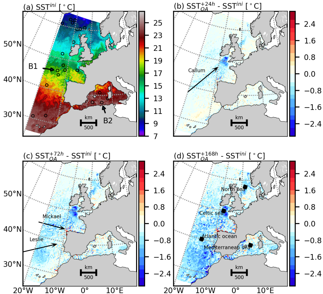
Figure 3. Initial [12 Oct. 2018 00 UTC] (a) and evolution of the SST ( ^{\circ}\text{C} ) after 1 day (b), 3 days (c) and 7 days (d) in the coupled simulation (OA; Table 2). In (a), the colour circles represent the SST measured by drifting buoys at that time ; B1 and B2 labels indicate the location of the two drifting buoys used in Figure 5. Black squares in (d) correspond to four extracted areas used for analyse in the next subsections.
