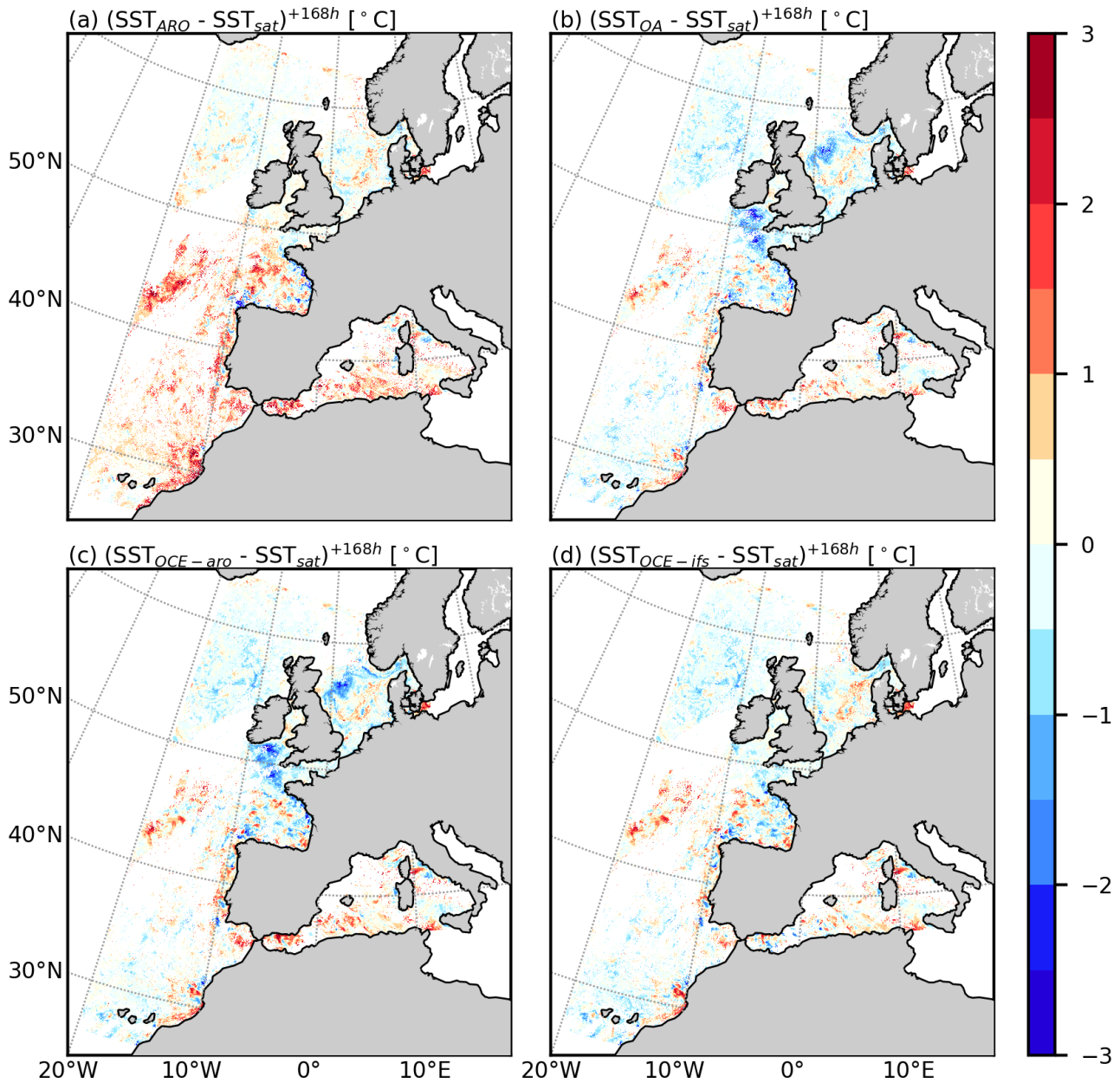
Figure 4. Comparison with L3 satellite SST observations at the end of the simulation (19 October 2018 00 UTC) : differences (in ^{\circ}C ) with (a) ARO SST, (b) OA simulated SST, (c) OCE-aro simulated SST and (d) OCE-ifs simulated SST.
