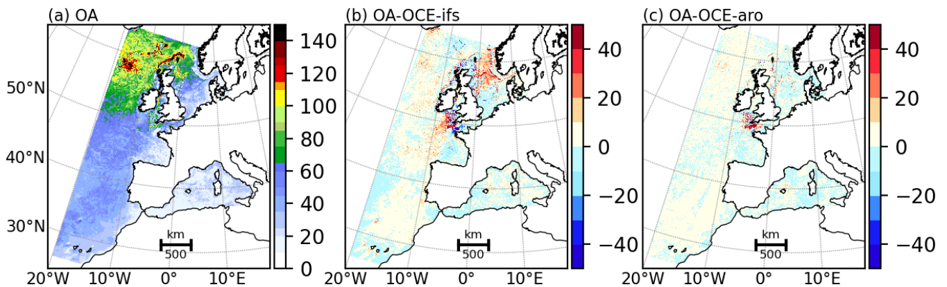
Figure 9. Daily-averaged oceanic mixed layer depth (m) simulated by OA simulation on the last day of simulation (a) and differences (in meters) with OCE-ifs and OCE-aro forced simulations (b, c).
