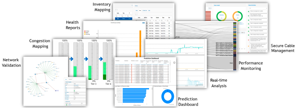
Robust UFM Cyber-AI Graphical User Interface
