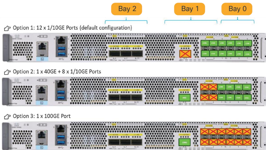
Figure 3. Bay 0 + bay 1 port options
