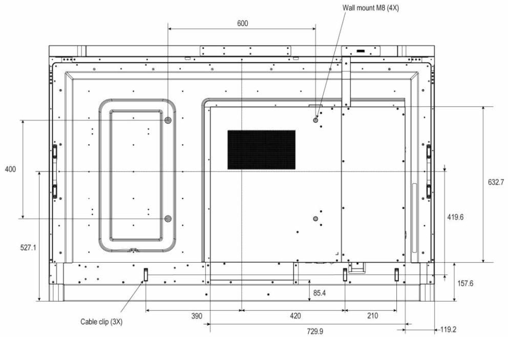
Figure 7-2. AVW-6555 Display Dimensions (mm)
