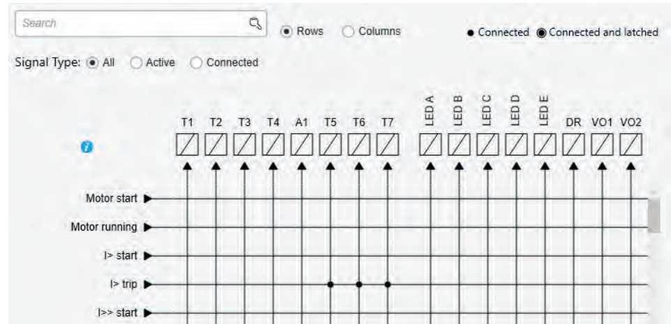
Figure 18 - Output matrix view
