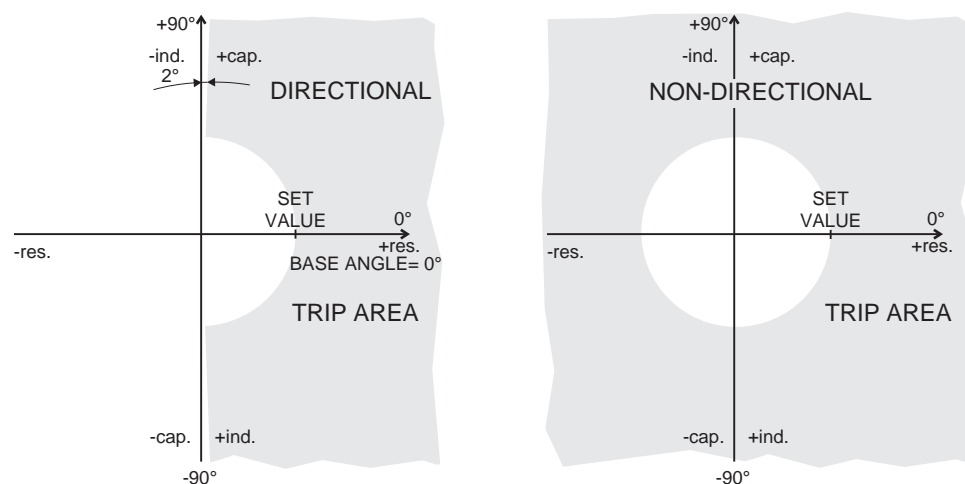
Figure 120 - Difference between directional mode and non-directional mode. The grey area is the trip region.
