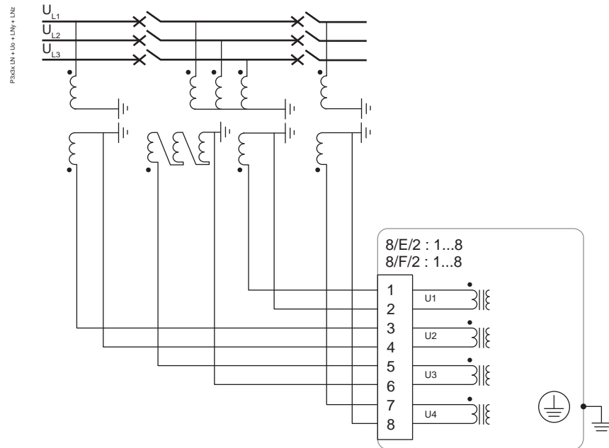
Figure 275 - LN+U 0 +LNy+LNz
