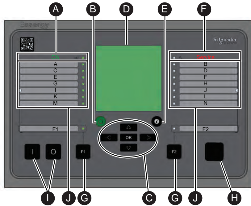
Figure 2 - Easergy P3M30 and P3M32 front panel
