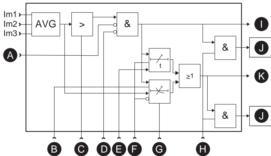
Figure 115 - Block diagram of the locked rotor protection stage I_{lr}>
