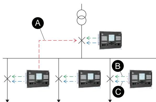
Figure 97 - CBFP implementation
