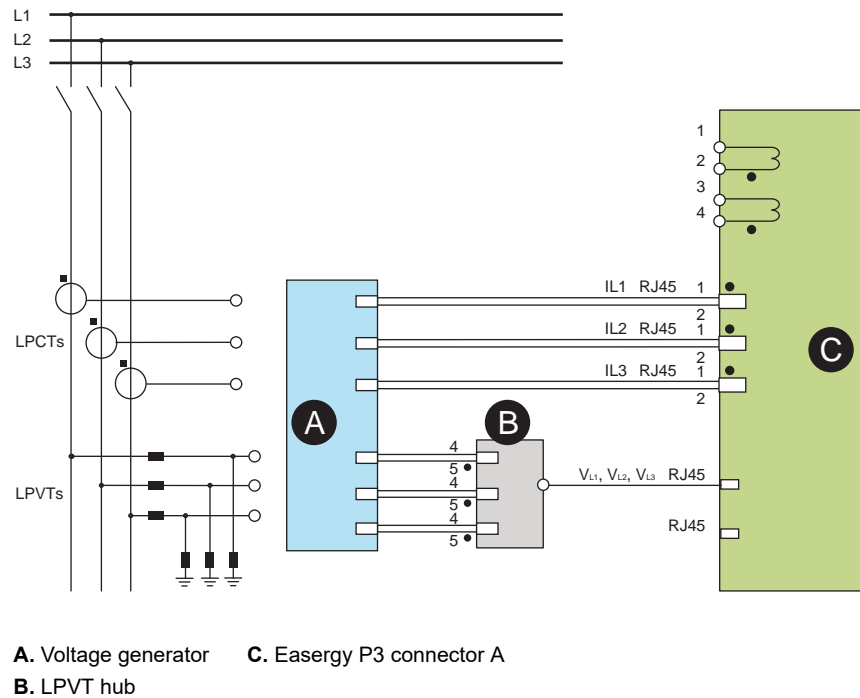
Figure 263 - Connection diagram for testing the LPIT
