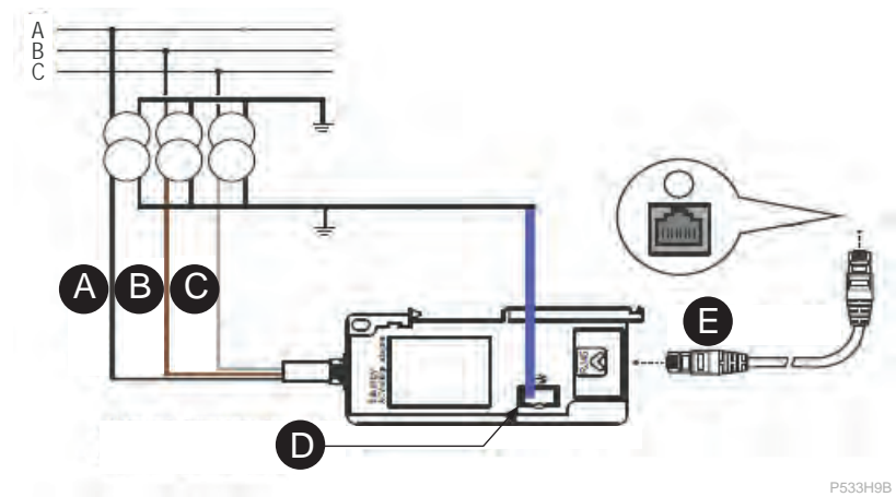
Figure 248 - 3 phase-to-neutral voltages connection
