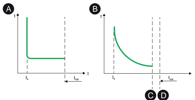
Figure 55 - Overcurrent characteristics
