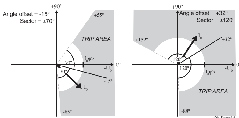
Figure 124 - Operation characteristics examples of the directional earth fault stages in the sector mode
