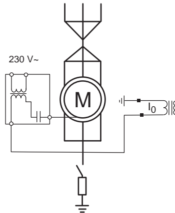
Figure 195 - Rotor earth-fault protection principle of field circuit by alternating current injection
