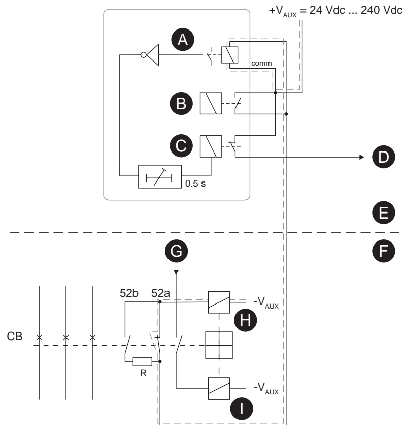
Figure 170 - Trip circuit supervision using a single digital input and an external resistor R
