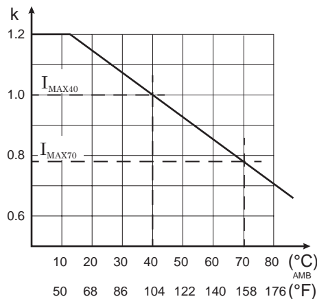
Figure 94 - Ambient temperature correction of the overload stage T>
