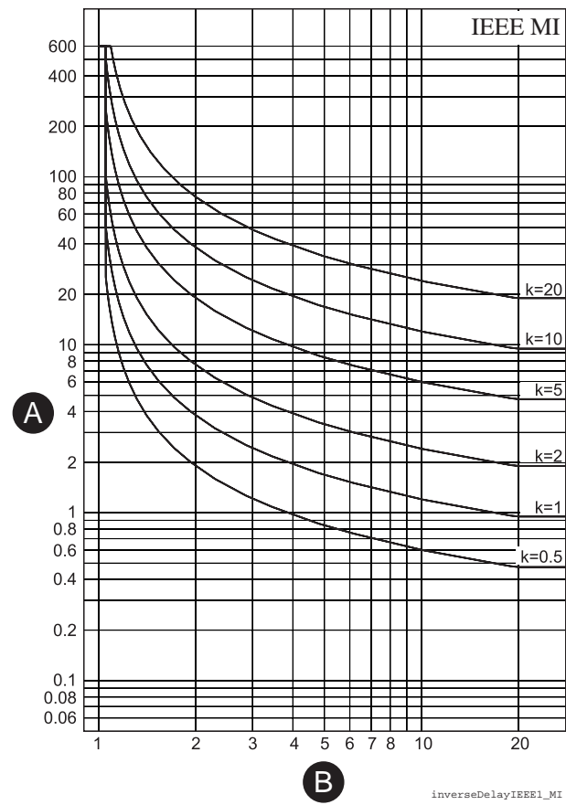
Figure 74 - ANSI/IEEE moderately inverse delay
