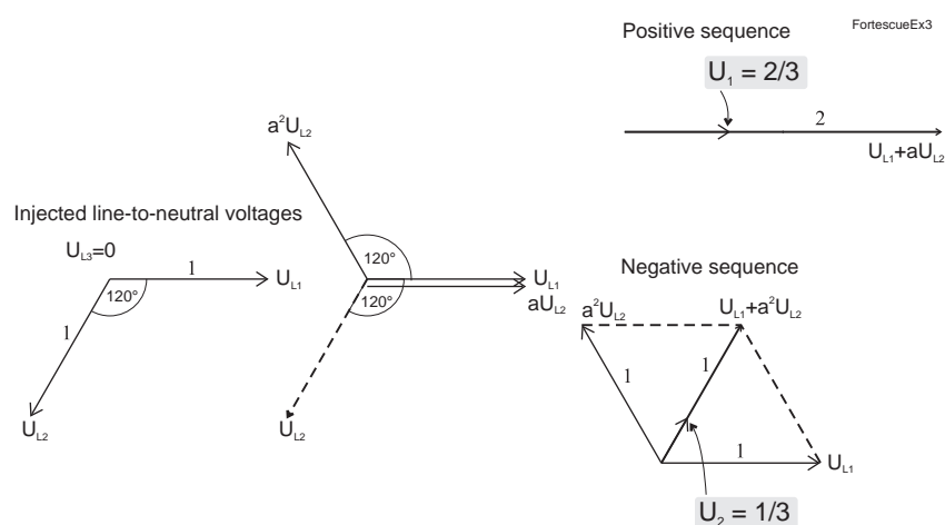
Figure 17 - Example of symmetrical component calculation using line-to-neutral voltages.
