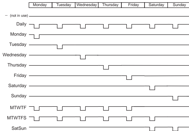
Figure 168 - Timer output sequence in different modes
