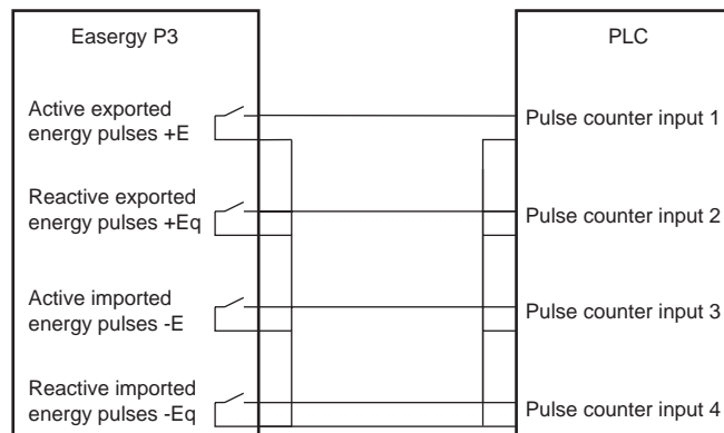
Figure 167 - Application example of wiring the energy pulse outputs to a PLC having common minus and an internal wetting voltage.
