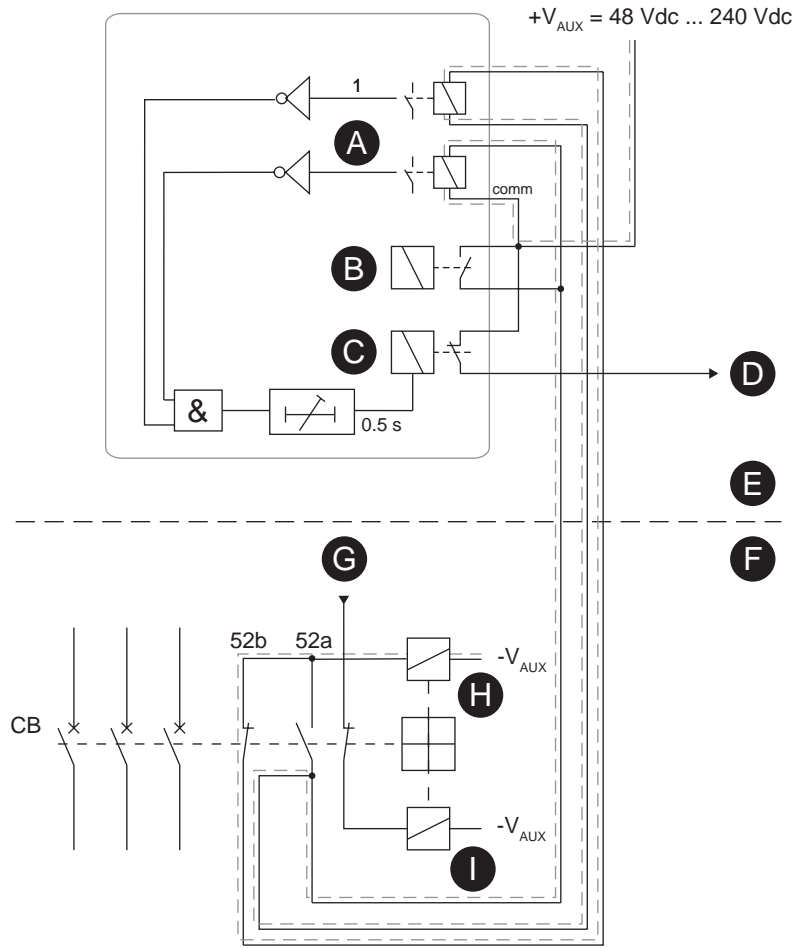
Figure 177 - Trip circuit supervision with two digital inputs and CB in open position
