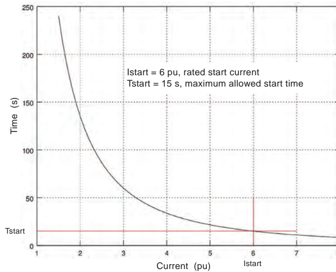
Figure 88 - Example of a dependent operate time delay of the motor start-up supervision stage
