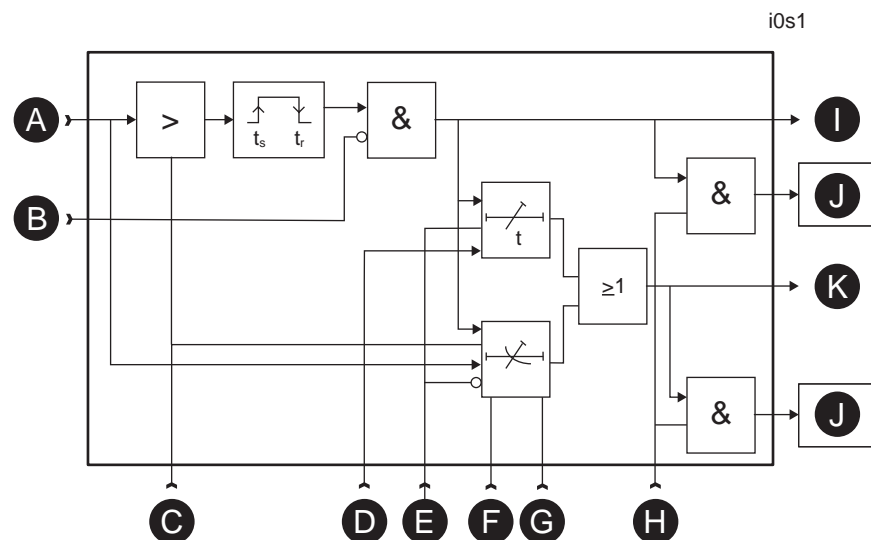
Figure 105 - Block diagram of the earth fault stage overcurrent I_0 >
