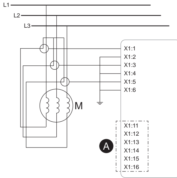
Figure 137 - Easergy P3M30 and P3M32 connected as a motor differential protection using 3 core balance CT's connected using flux balancing principle.
