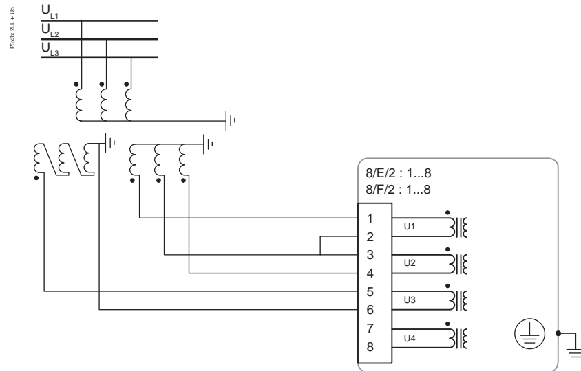
Figure 270 - 2LL+U 0
