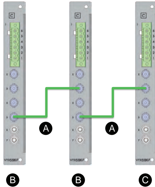
Figure 198 - Arc flash detection application example – fiber connections
