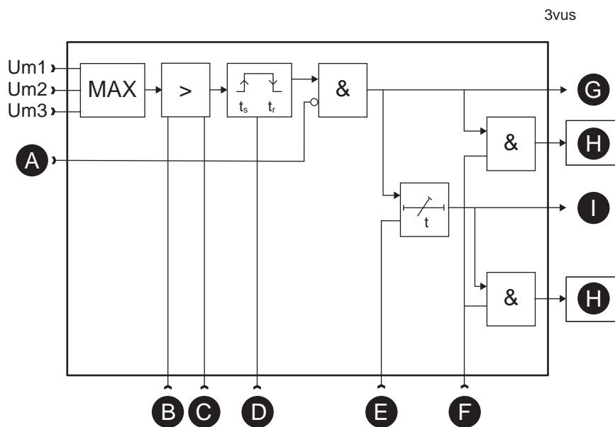
Figure 116 - Block diagram of the three-phase overvoltage stages U>, U>> and U>>>
