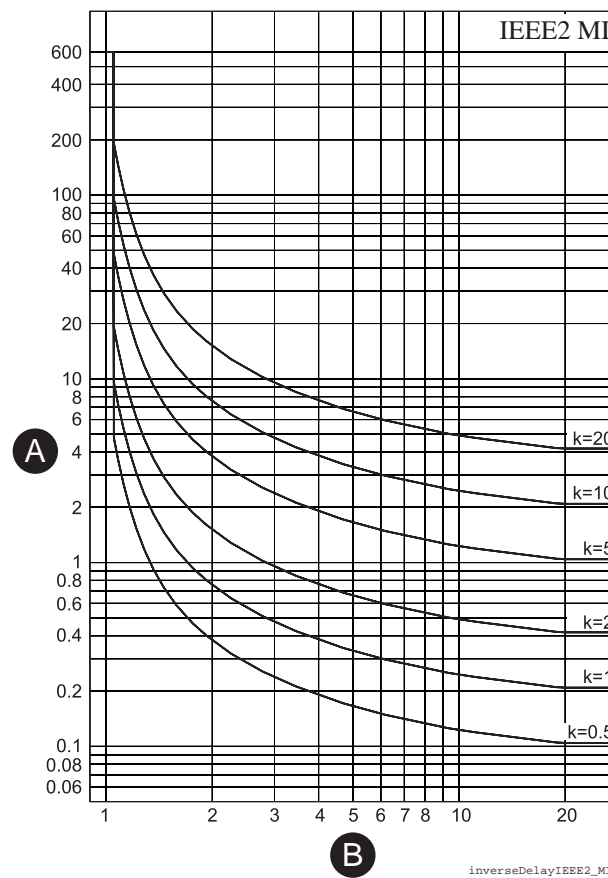
Figure 77 - IEEE2 moderately inverse delay
