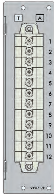
Figure 216 - Analog measurement card "T = 3xl (5/1A) + I_0 (5/1A)"
