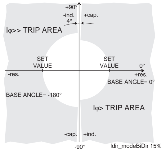
Figure 121 - Bi-directional application with two stages I_{\phi>} and I_{\phi>>}
