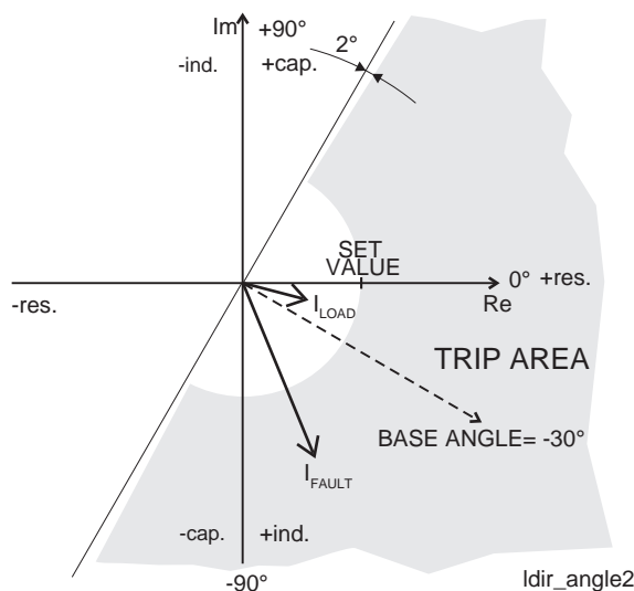
Figure 119 - Example of the directional overcurrent function's protection area
