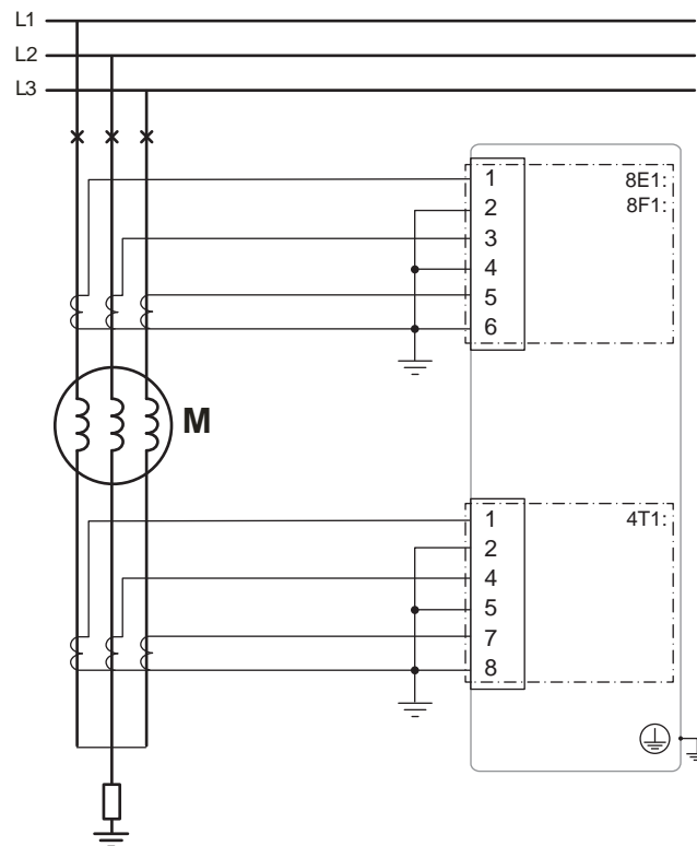
Figure 136 - Easergy P3M30 and P3M32 connected as a motor differential protection device using six CTs
