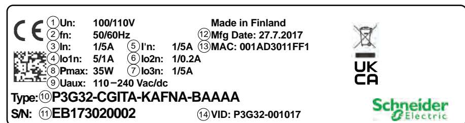
Figure 206 - Serial number label
