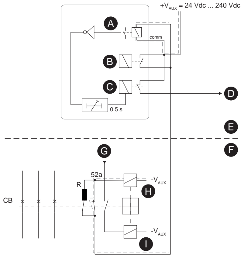
Figure 171 - Alternative connection without using circuit breaker 52b auxiliary contacts
