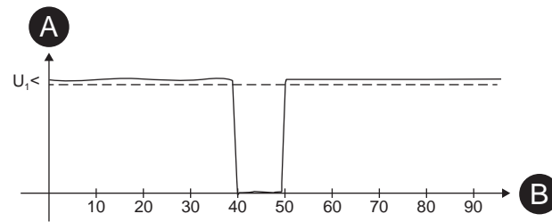
Figure 158 - A short voltage interrupt that will be recognized
