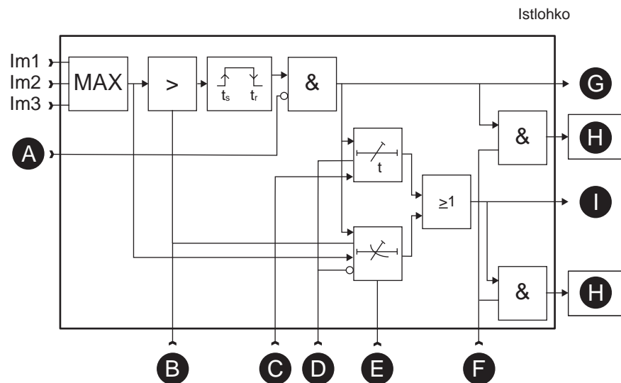
Figure 89 - Block diagram of motor start-up supervision I_{ST} >
