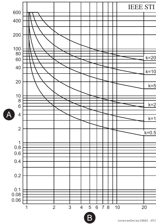
Figure 75 - ANSI/IEEE short time inverse delay
