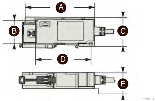
Figure 253 - Voltage adapter dimensions
