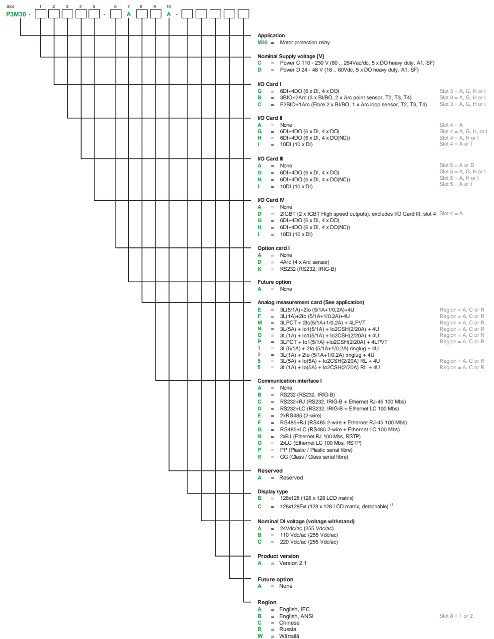
Figure 282 - P3M30 order code
