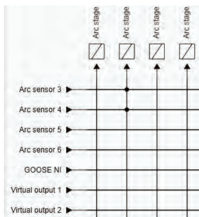
Figure 148 - Configuring the light arc matrix
