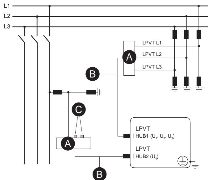
Figure 245 - Three line-to-neutral LPVTs + one line-to-neutral LPVT
