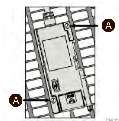
Figure 256 - Mounting on Telequick grid
