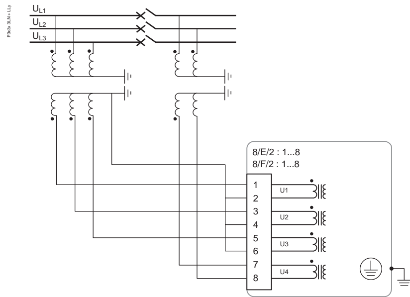
Figure 268 - 3LN+LLy
