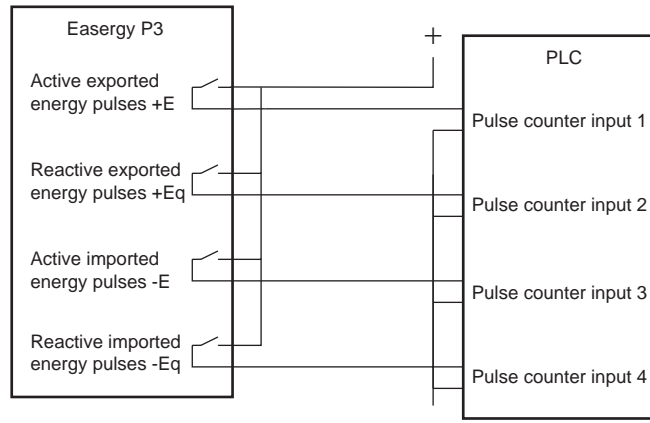
Figure 166 - Application example of wiring the energy pulse outputs to a PLC having common minus and using an external wetting voltage
