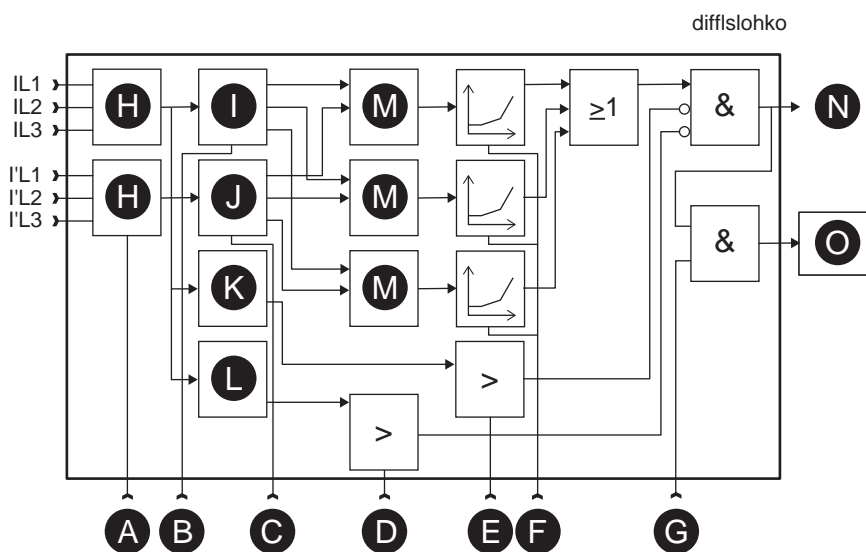
Figure 134 - Block diagram of the differential overcurrent stage \Delta I >
