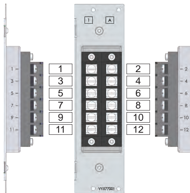
Figure 217 - Analog measurement card "1 = 3xl (5/1A) ring lug + I_0 (5/1A)"
