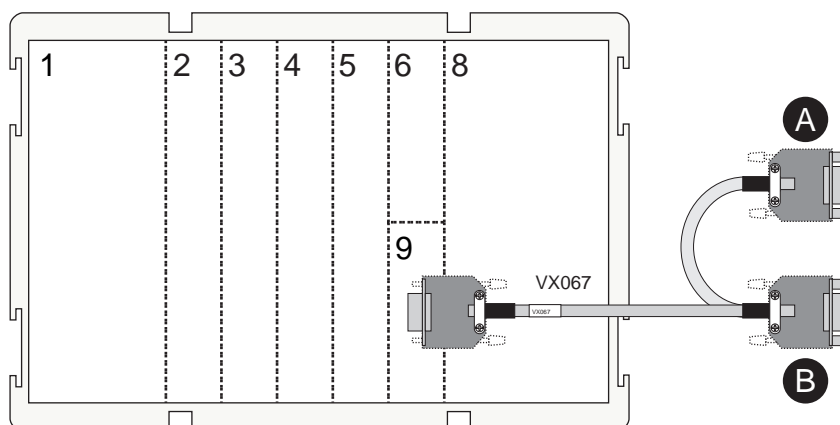
Figure 232 - VX067 cable on the D-connector of slot 9 option card
