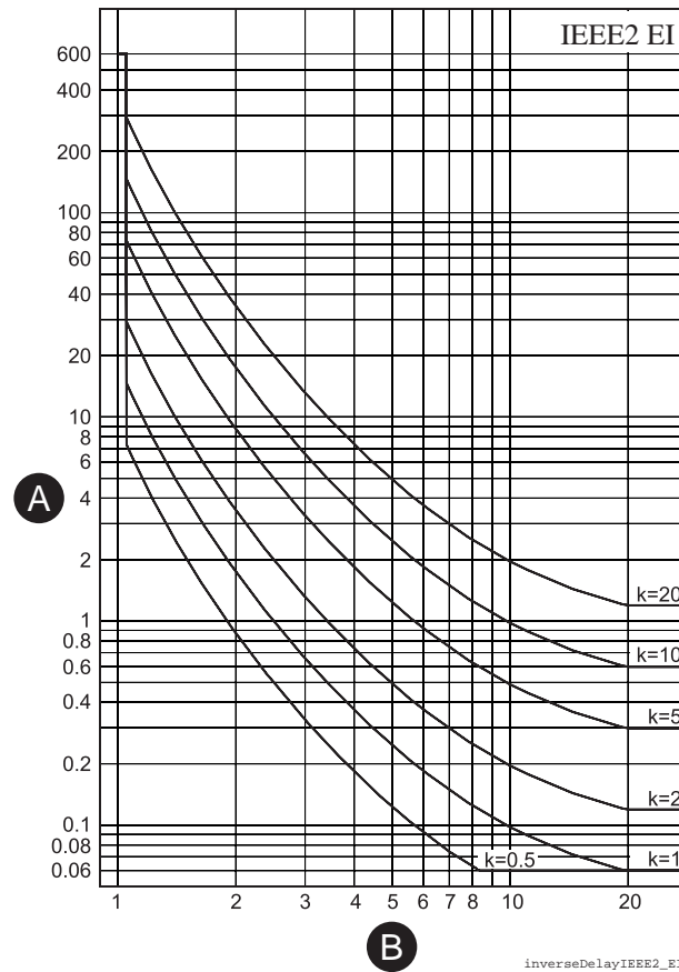
Figure 80 - IEEE2 extremely inverse delay
