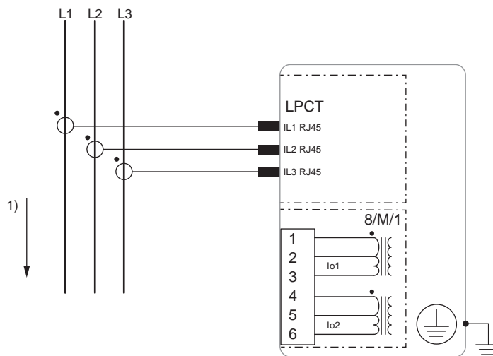
Figure 243 - Three-phase current measurement – LPCT
