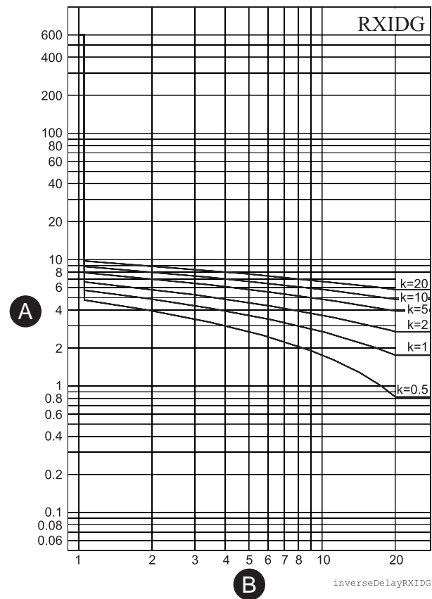
Figure 82 - RXIDG dependent delay
