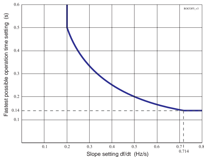
Figure 127 - At very sensitive slope settings the fastest possible operate time is limited.
