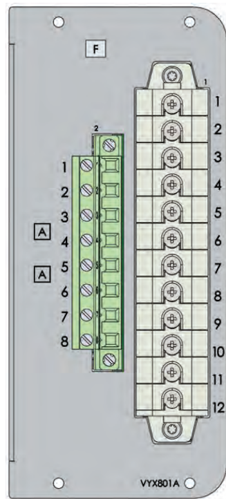
Figure 214 - Analog measurement card F or O (O only for P3x30 models)
