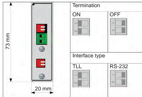
Figure 236 - RS-232 and TTL interface
