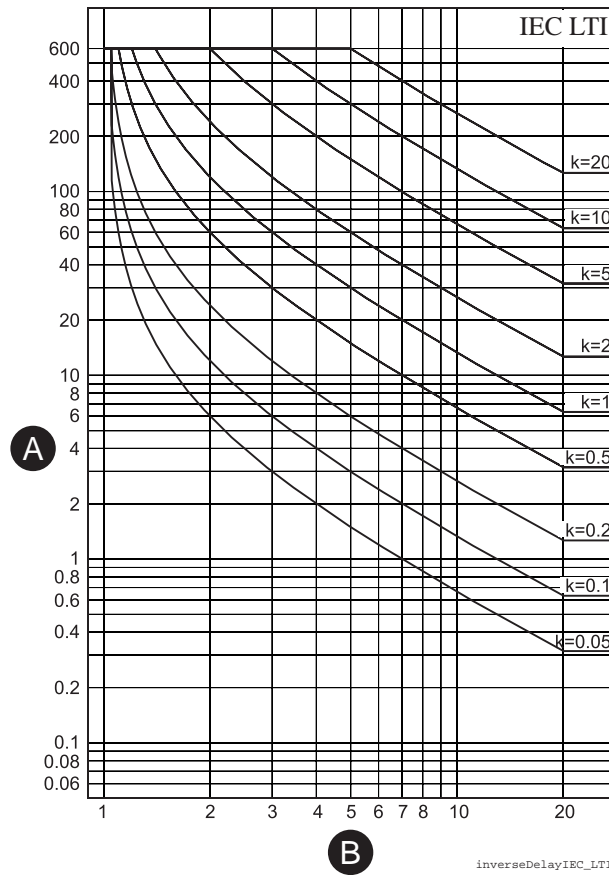
Figure 70 - IEC long time inverse delay
