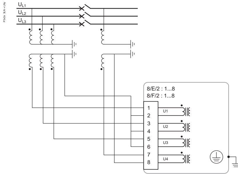
Figure 269 - 3LN+LNy
