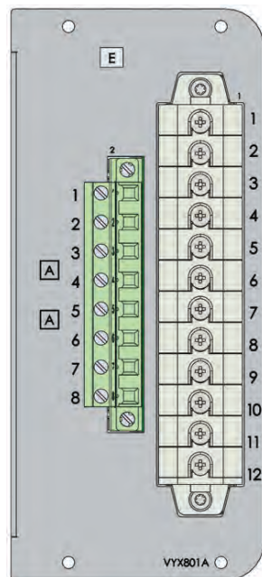
Figure 212 - Analog measurement card E / N (N only for P3x30 models)
