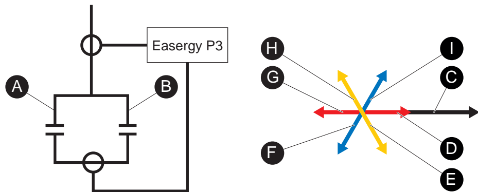
Figure 109 - How a failure in different branches of the bank affects the I_0 measurement
