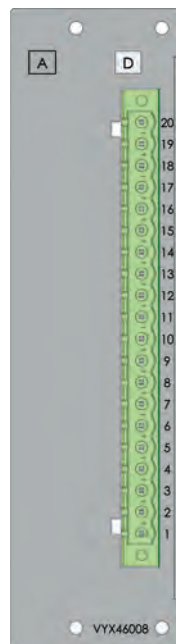
Figure 220 - I/O card “D = 2IGBT”
