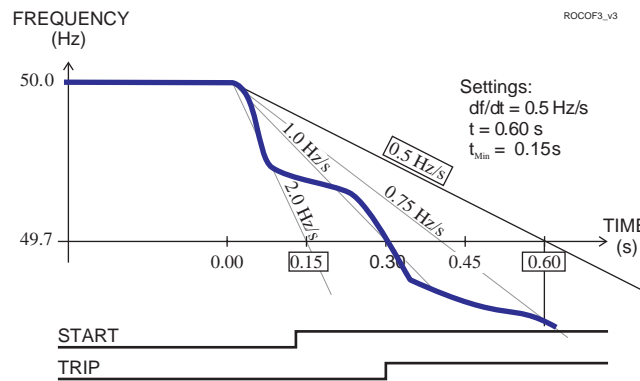
Figure 129 - An example of dependent df/dt operate time. The time to trip will be 0.3 s, although the setting is 0.6 s, because the average slope 1 Hz/s is steeper than the setting value 0.5 Hz/s.
