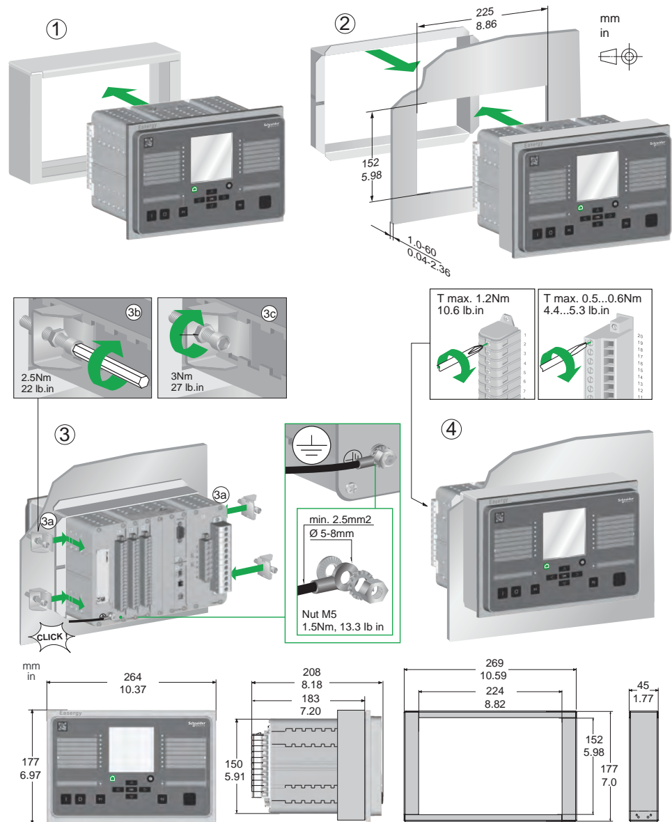
Figure 210 - Projection mounting
