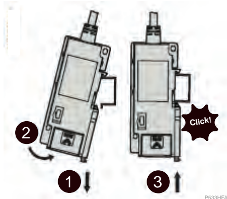
Figure 254 - Mounting on DIN rail
