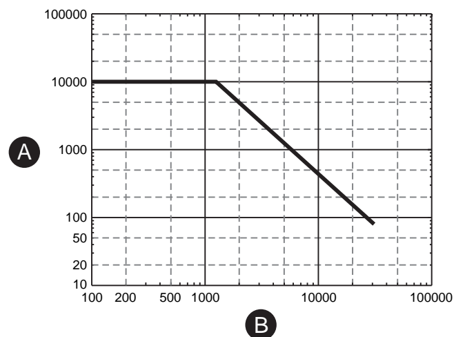
Figure 159 - Example permissible cycle diagram
