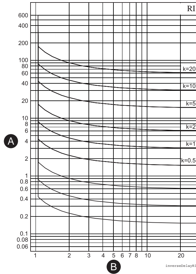
Figure 81 - RI dependent delay
