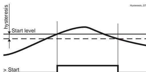
Figure 60 - Behavior of a greater than comparator (for example, the hysteresis (dead band) in overvoltage stages)
