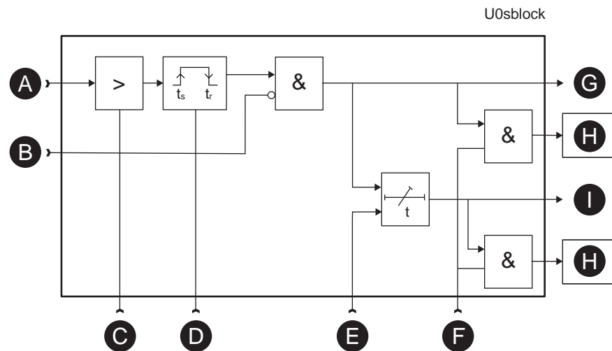
Figure 117 - Block diagram of the neutral voltage displacement stages U_0> , U_0>>
