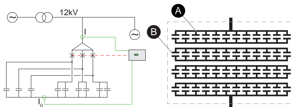
Figure 110 - 131.43 \mu\text{F} Y-Y connected capacitor bank with internal fuses
