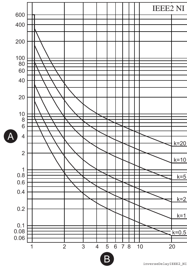
Figure 78 - IEEE2 normal inverse delay
