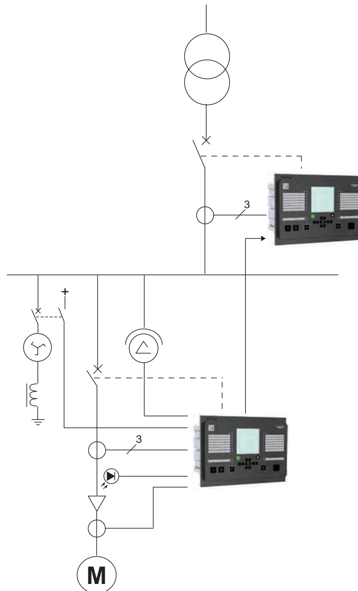
Figure 194 - Easergy P3M30 and P3M32 used in cable protection of an industry plant network
