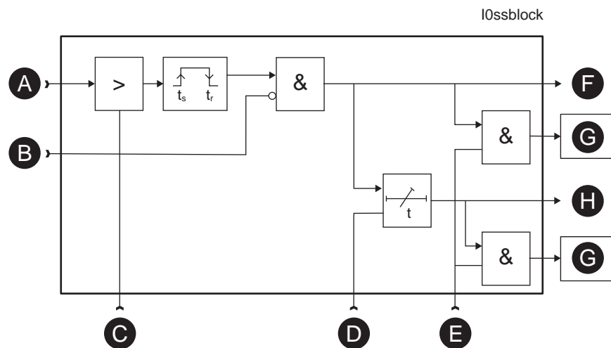
Figure 106 - Block diagram of the earth fault stages overcurrent I_0>> , I_0>>> , I_0>>>>
