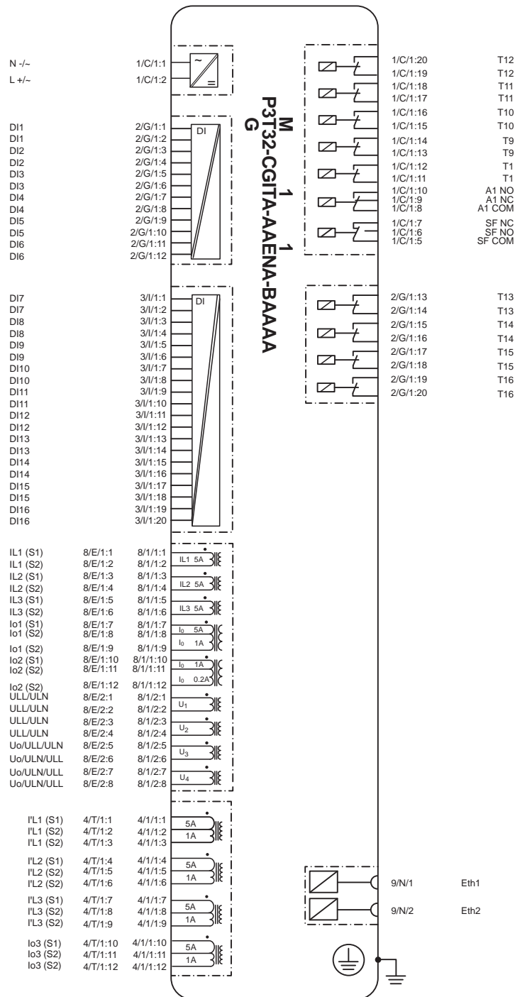
Figure 240 - Typical block diagram for P3M32, P3T32 and P3G32 relays
