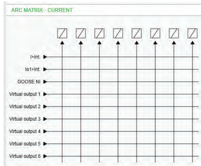
Figure 147 - Configuring the current matrix – an example
