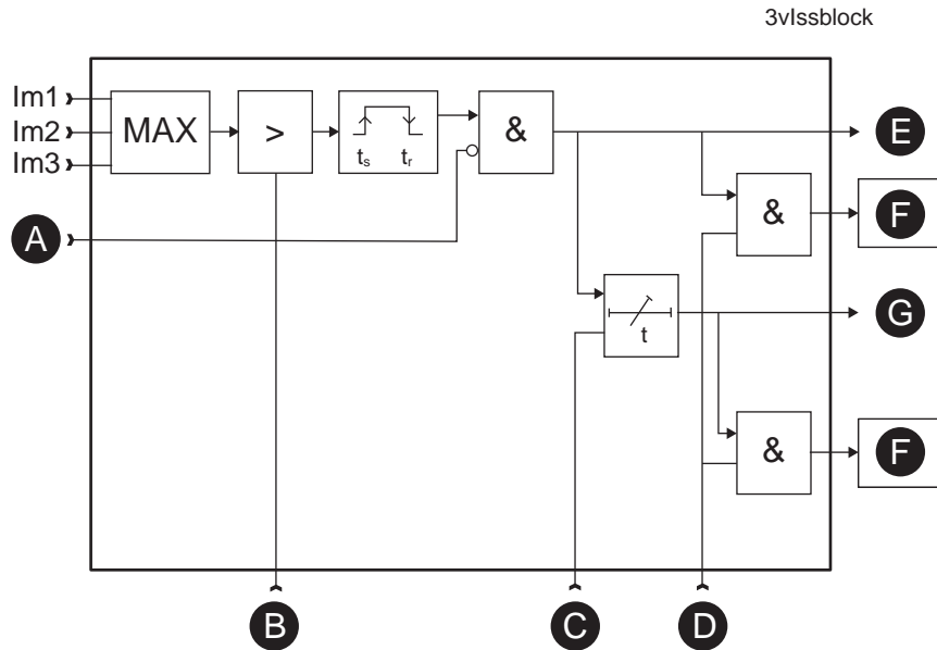
Figure 104 - Block diagram of the three-phase overcurrent stage I>> and I>>>
