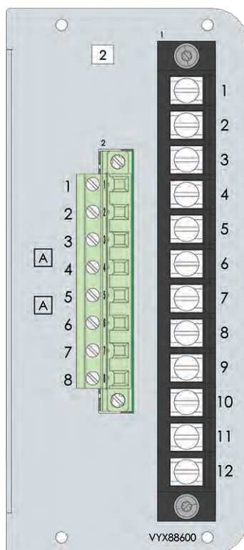
Figure 215 - Analog measurement card 2 or 6 (6 only for P3x30 models)
