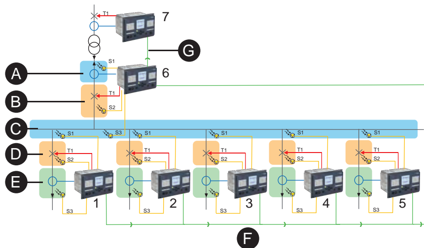
Figure 196 - Typical arc flash detection scheme with integrated arc flash option card
