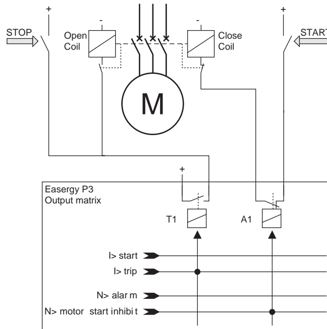
Figure 118 - Application for preventing too frequent starting using the N> stage
