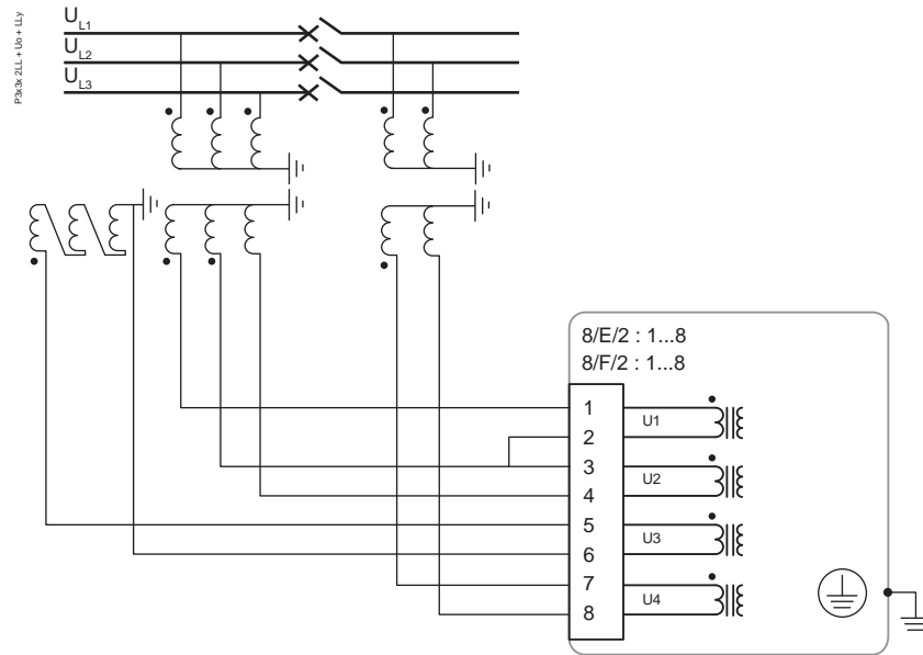
Figure 271 - 2LL+U 0 +LLy
