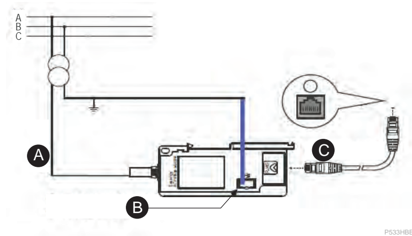
Figure 250 - 1 additional line-to-line voltage connection
