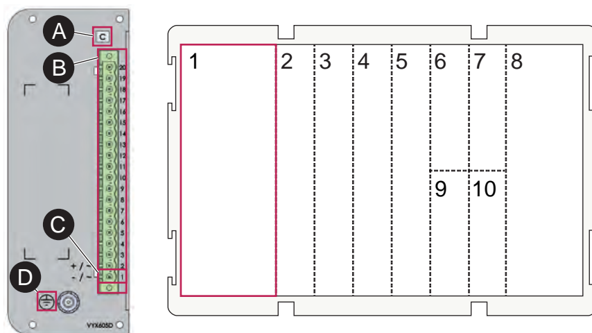
Figure 5 - Slot numbering and card options in the Easergy P3M30 and P3M32 rear panel and an example of defining the pin address 1/C/1:1
