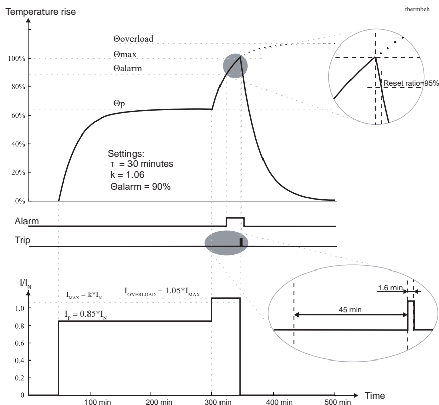
Figure 95 - Example of the thermal model behavior
