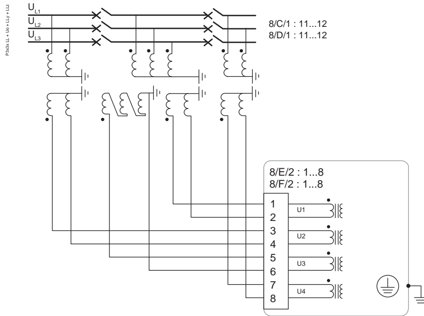
Figure 273 - LL+U 0 +LLy+LLz
