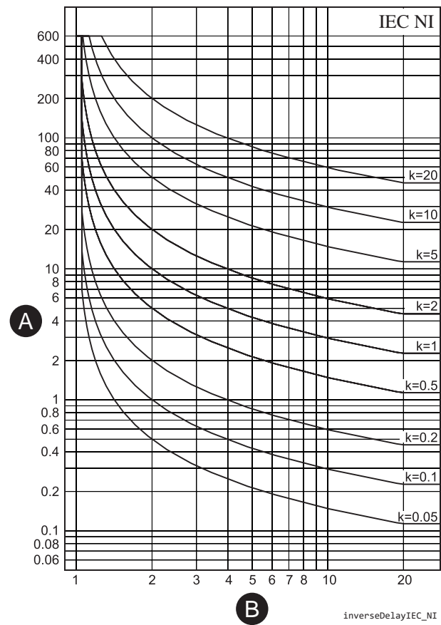
Figure 67 - IEC normal inverse delay
