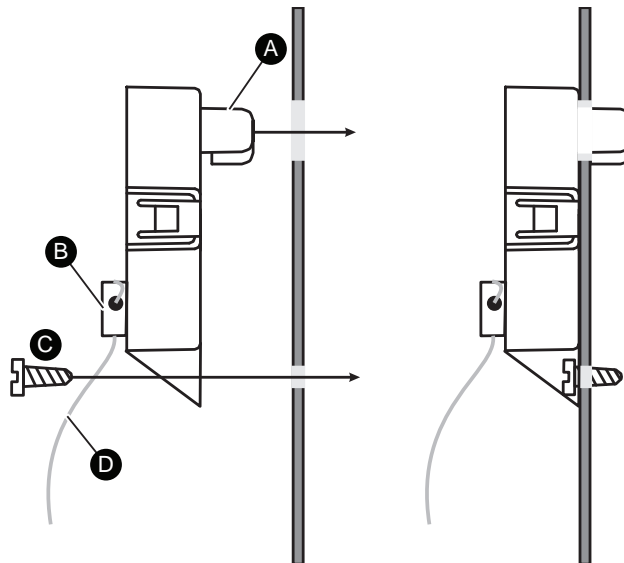
Figure 228 - Mounting the sensor
