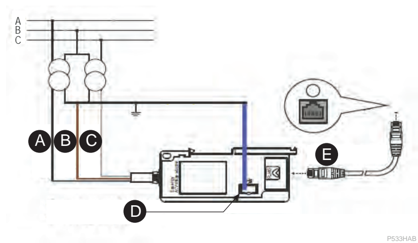
Figure 249 - 2 line-to-line voltages connection
