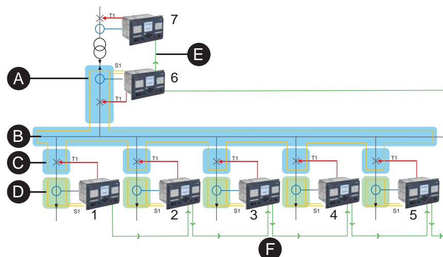
Figure 197 - Arc flash detection application example – fiber
