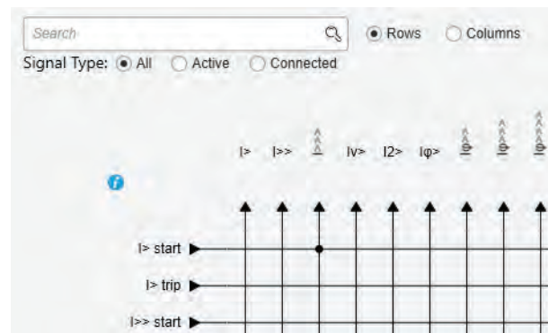
Figure 39 - Block matrix view
