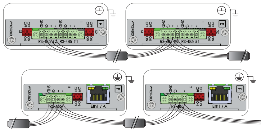
Figure 229 - All shields connected through and grounded at one end
