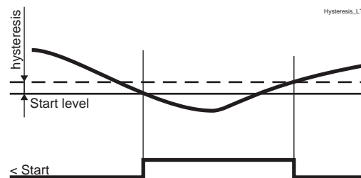
Figure 65 - Example behavior of an under-protection with hysteresis
