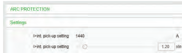
Figure 146 - Example of defining the I start setting value
