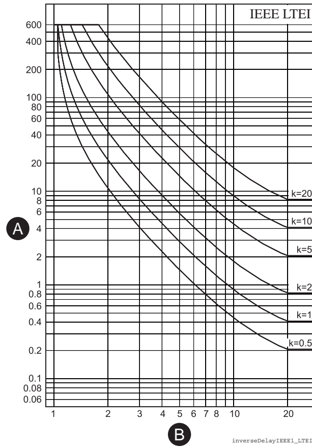
Figure 73 - ANSI/IEEE long time extremely inverse delay
