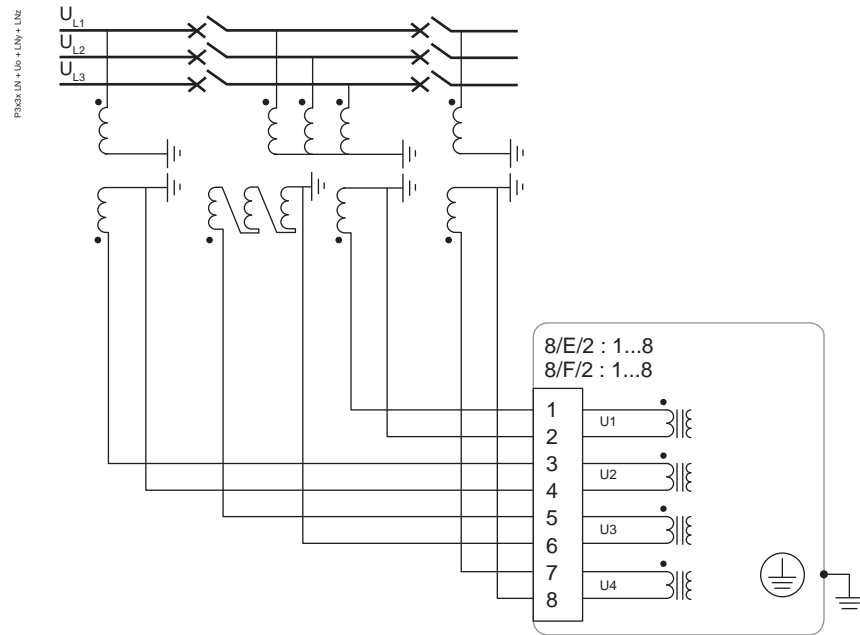
Figure 274 - LN+U 0 +LNy+LNz
