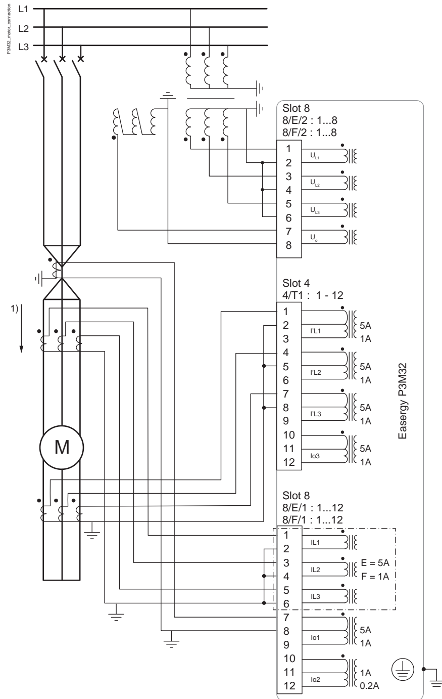
Figure 242 - P3M32 connection for motor differential application
