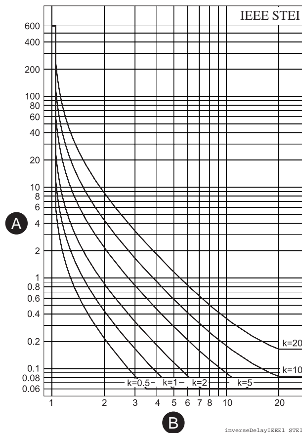
Figure 76 - ANSI/IEEE short time extremely inverse delay
