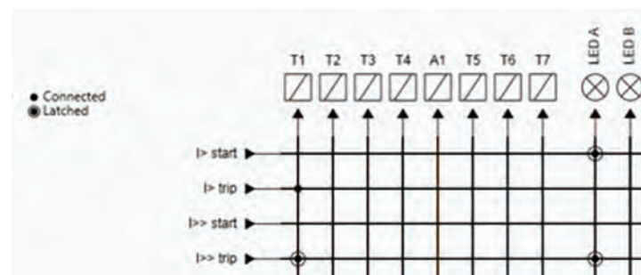
Figure 130 - The lockout programmed for LED A and I>> trip signals
