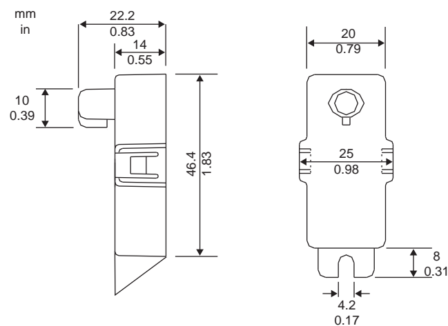
Figure 225 - Sensor dimensions
