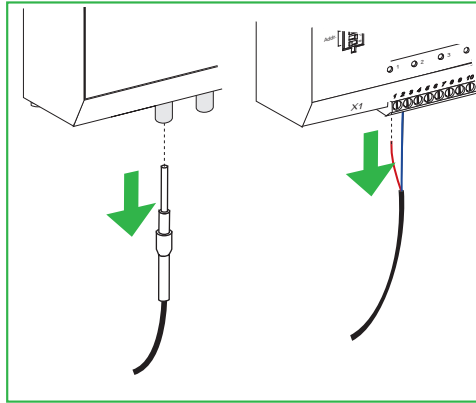
Figure 261 - Testing the sensor's self-supervision
