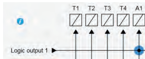
Figure 180 - An example of output matrix configuration for trip circuit supervision with two digital inputs
