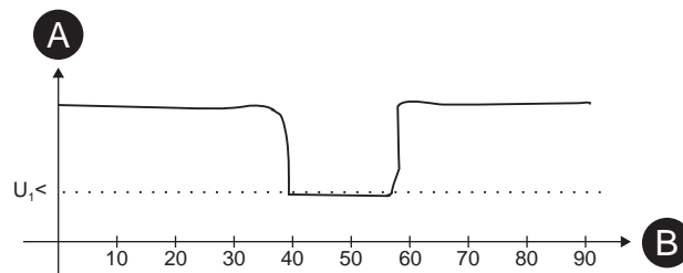
Figure 157 - A short voltage interruption which is probably not recognized
