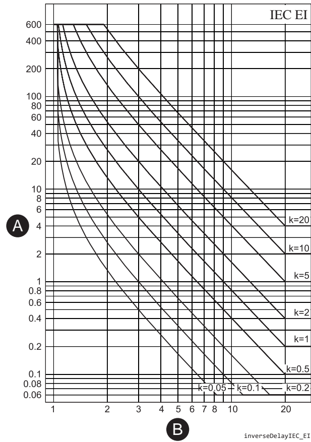
Figure 68 - IEC extremely inverse delay
