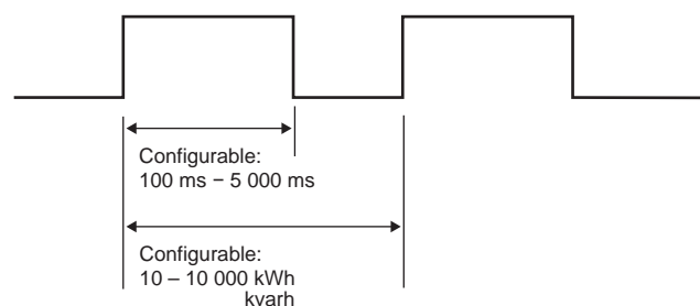
Figure 164 - Principle of energy pulses
