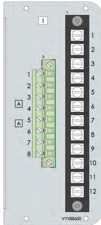
Figure 213 - Analog measurement card 1 / 5 (5 only for P3x30 models)
