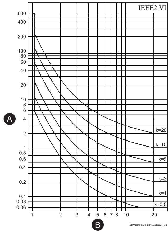
Figure 79 - IEEE2 very inverse delay
