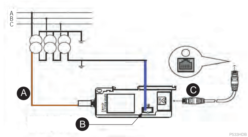
Figure 252 - Open-delta connection 2
