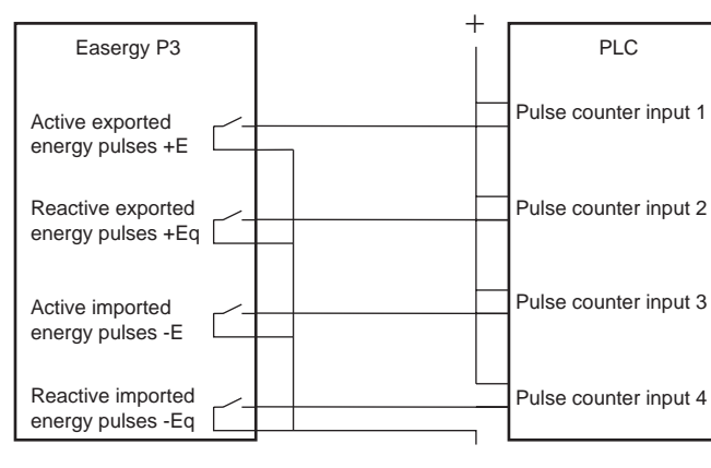
Figure 165 - Application example of wiring the energy pulse outputs to a PLC having common plus and using an external wetting voltage
