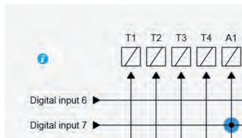
Figure 175 - Example of output matrix configuration for trip circuit supervision with one digital input
