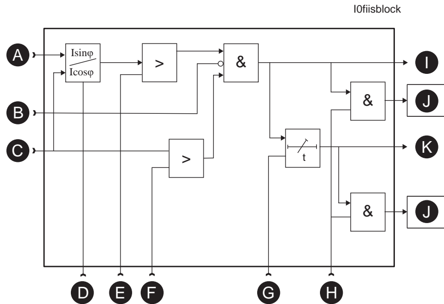
Figure 122 - Block diagram of the directional earth fault overcurrent stages I_{0\phi} > , I_{0\phi} >>
