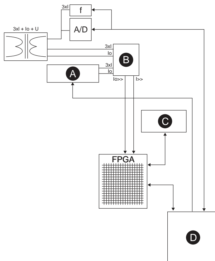
Figure 10 - Measurement logic for the arc flash detection function
