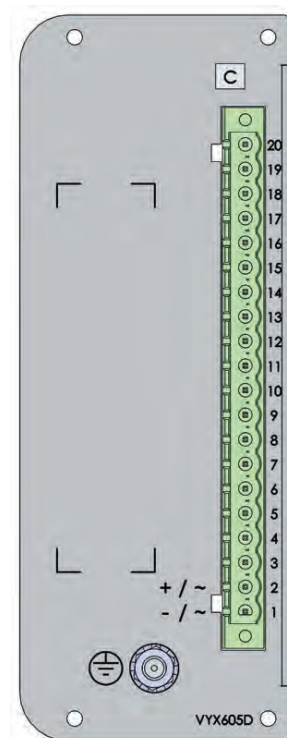
Figure 211 - Example of supply voltage card Power C 110-240
