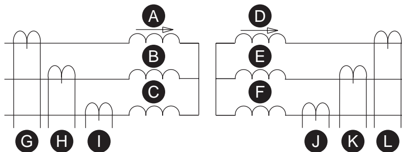
Figure 133 - Winding currents in connection group Yy0
