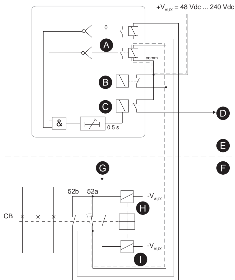
Figure 176 - Trip circuit supervision with two digital inputs and closed CB
