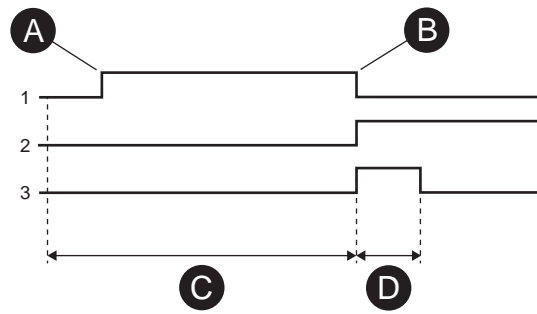
Figure 85 - Synchrocheck function principle
