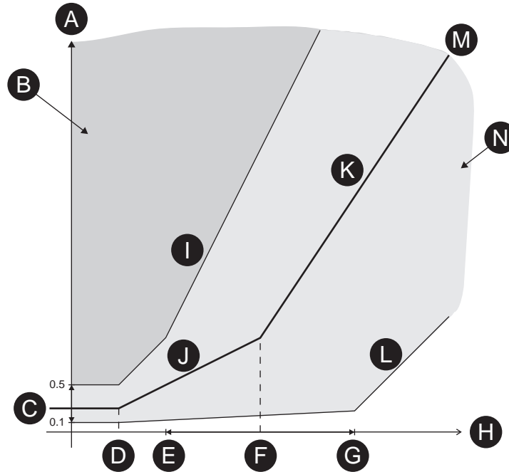
Figure 135 - Example of differential overcurrent characteristics
