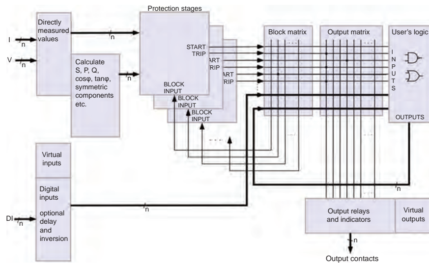
Figure 37 - Blocking matrix and output matrix
