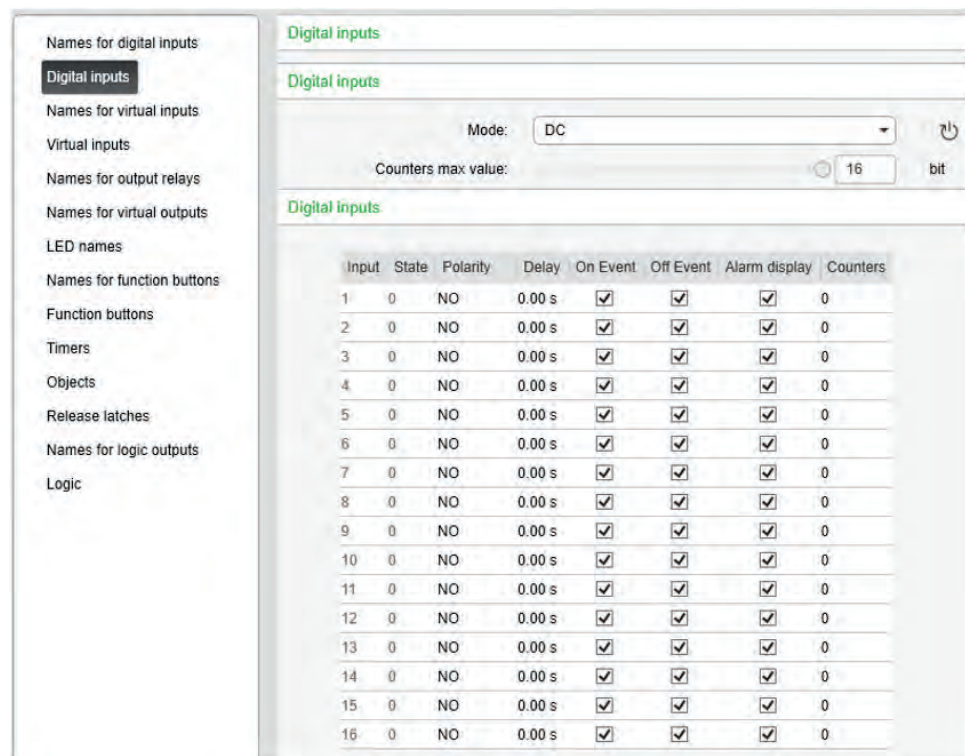
Figure 27 - Digital inputs view
