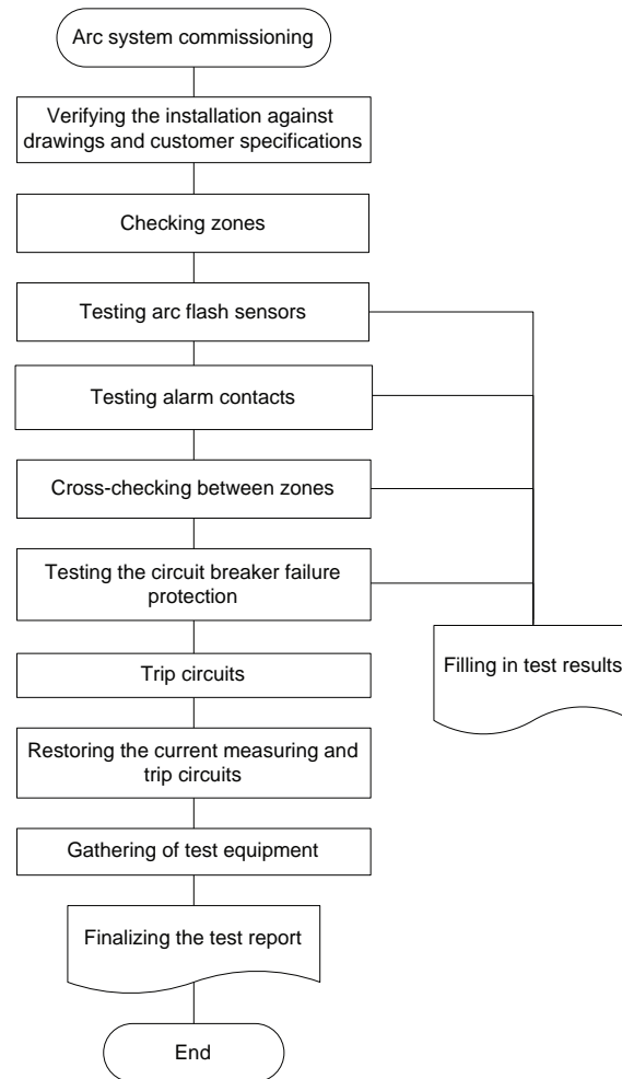
Figure 259 - Testing sequence
