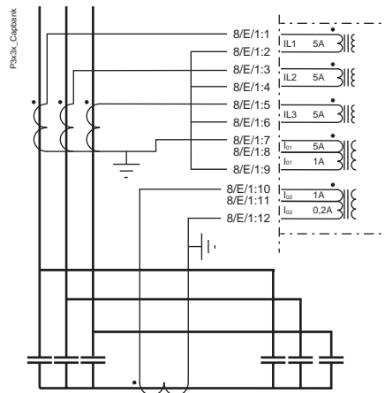
Figure 107 - Typical capacitor bank protection application with Easergy P3 relays
