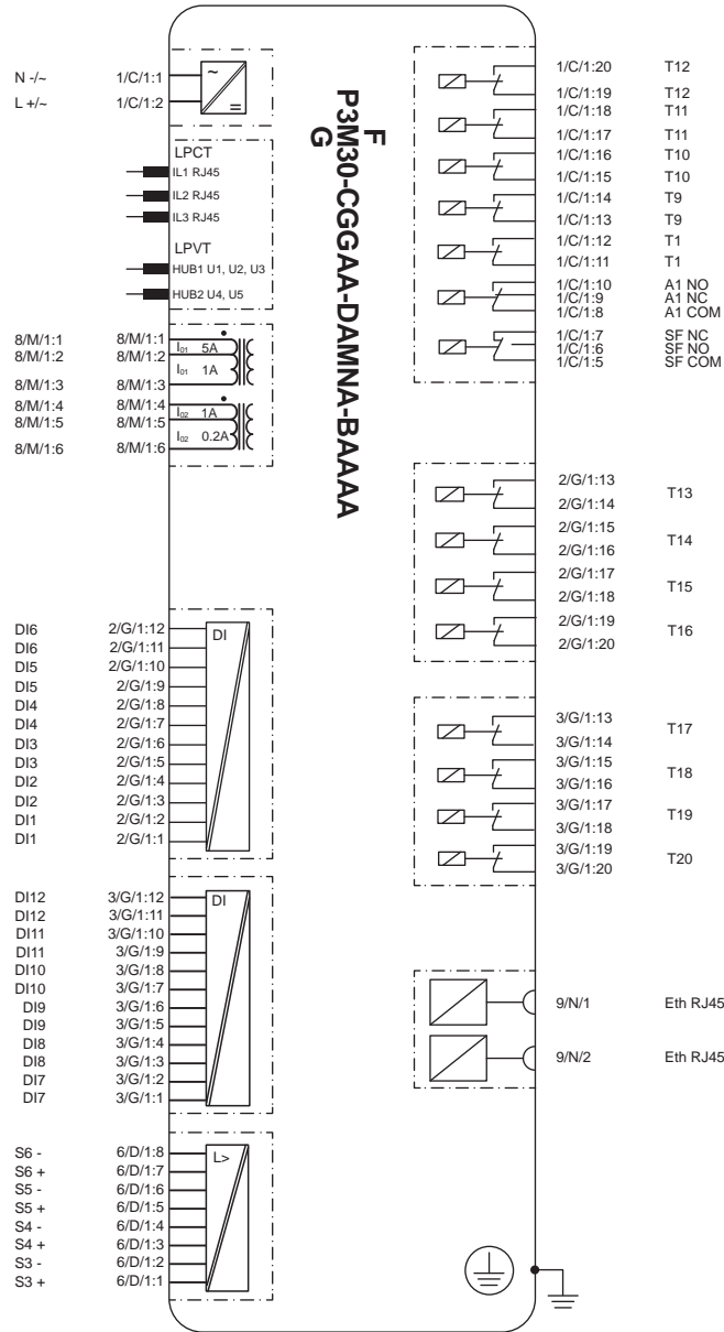
Figure 239 - P3F30 and P3M30 block diagram – LPIT
