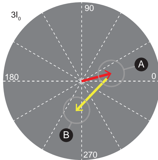
Figure 108 - Natural unbalance compensation and a single capacitor fault
