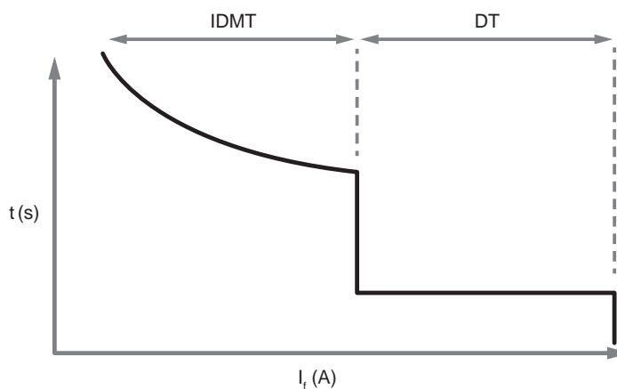
Figure 61 - Dependent time and definite time operation curves
