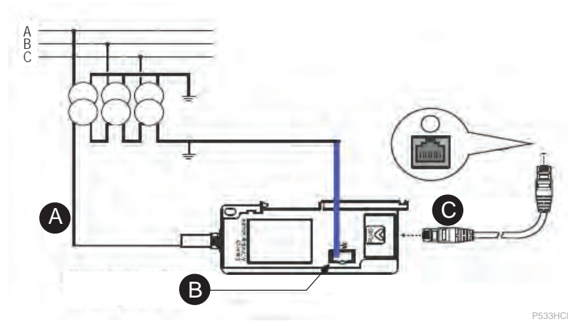
Figure 251 - Open-delta connection 1
