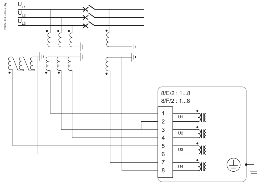
Figure 272 - 2LL+U 0 +LNy
