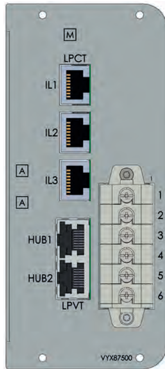
Figure 265 - Terminals 8/M/Hub 1 and 8/M/Hub 2 – LPVT
