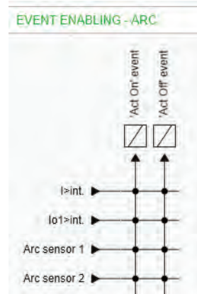
Figure 150 - Configuring the arc events – an example
