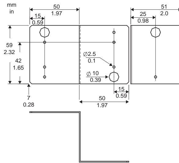
Figure 226 - VYX 001 mounting plate for sensor
