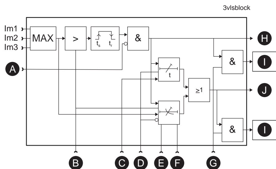
Figure 103 - Block diagram of the three-phase overcurrent stage I>
