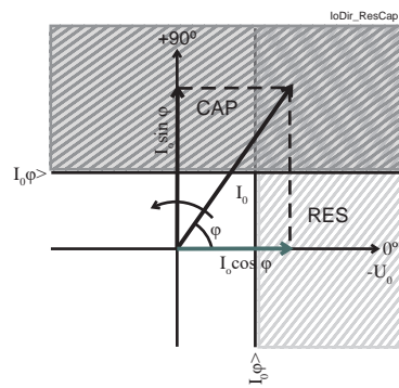
Figure 123 - Operation characteristics of the directional earth fault protection in Res and Cap mode
