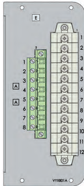
Figure 264 - Example of terminal 8/E/1 and 8/E/2
