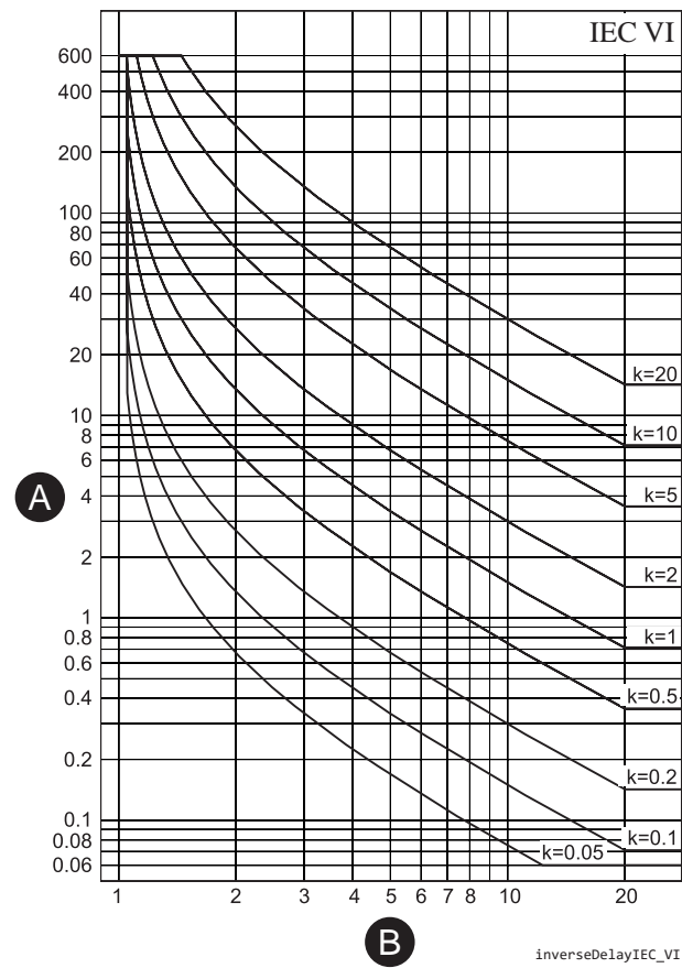
Figure 69 - IEC very inverse delay
