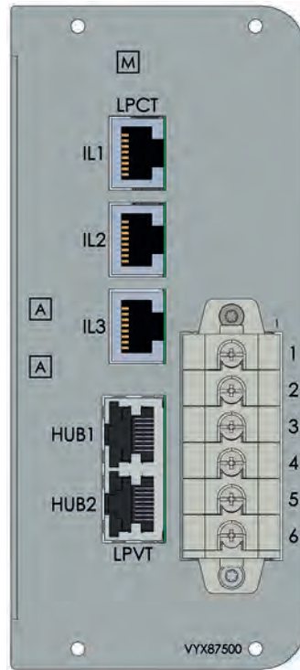
Figure 246 - LPIT measurement card M / P (P only for P3x30 models)
