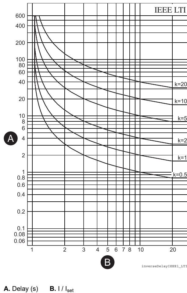
Figure 71 - ANSI/IEEE long time inverse delay
