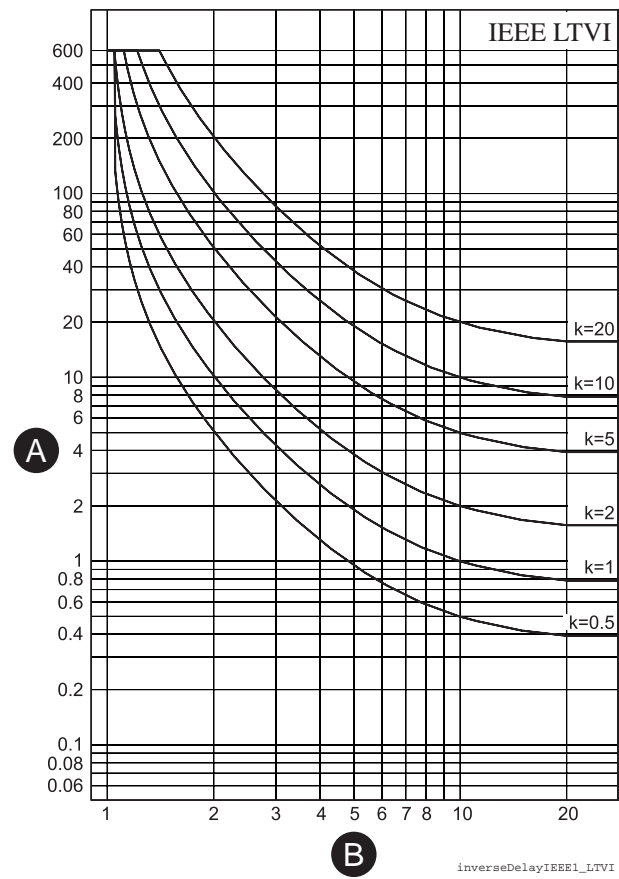
Figure 72 - ANSI/IEEE long time very inverse delay
