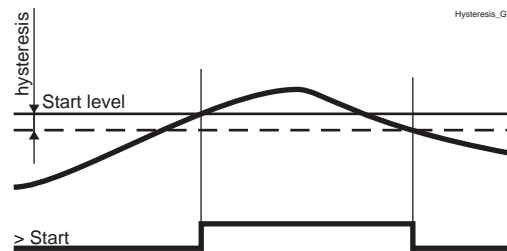
Figure 64 - Example behavior of an over-protection with hysteresis
