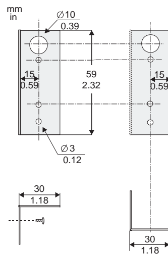
Figure 227 - VYX 002 mounting plate for sensor
