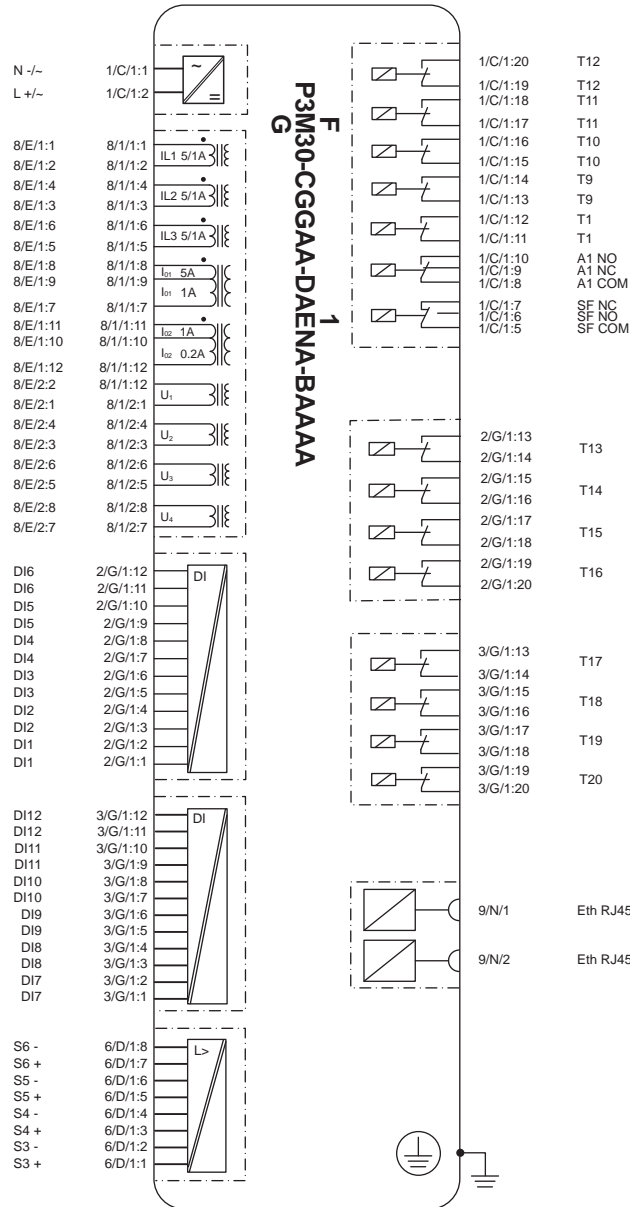
Figure 238 - Typical block diagram for P3F30, P3M30 and P3G30 relays
