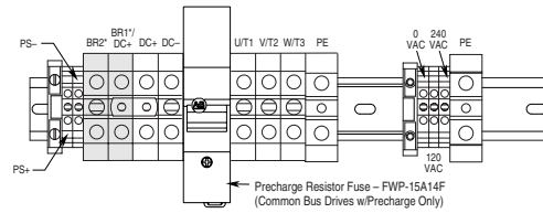
Frame 5 - 75 HP Normal Duty 650V DC Input
