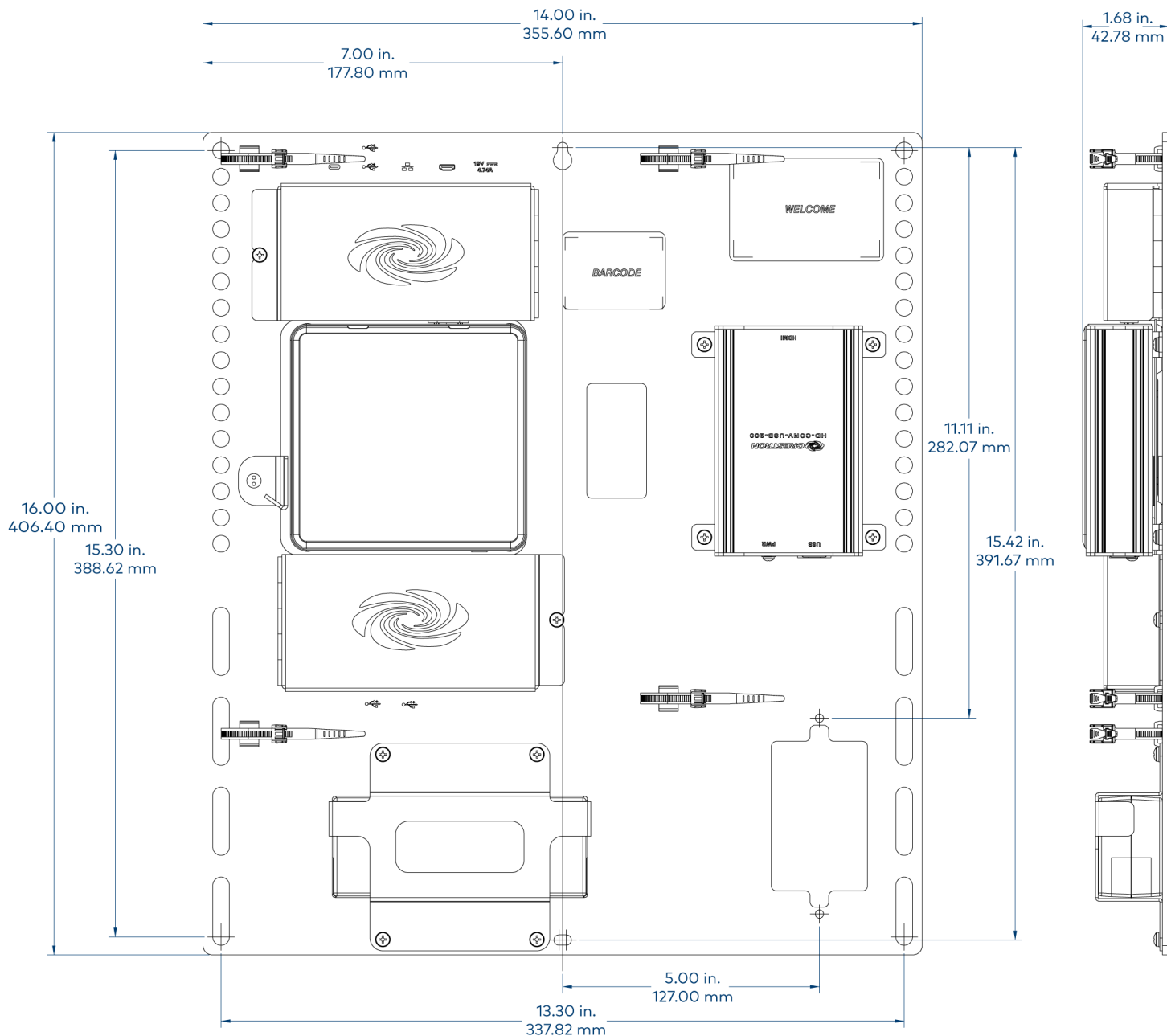
UC-BRKT-100-SD-Z-ASSY
