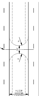
DETAIL OF TEMPORARY CROSSOVER
