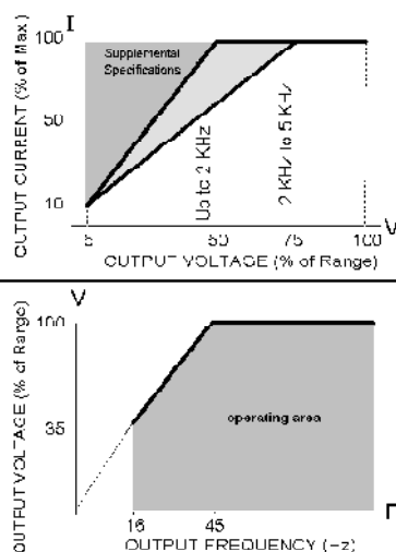
Voltage, Current and Frequency rating charts
